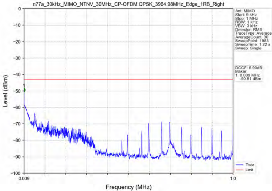
n77a_30kHz_MIMO_NTNV_30MHz_CP-OFDM QPSK_3964.98MHz_Edge_1RB_Right
