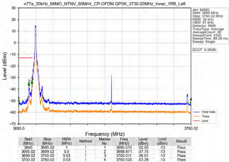
n77a_30kHz_MIMO_NTNV_60MHz_CP-OFDM QPSK_3730.02MHz_Inner_1RB_Left
