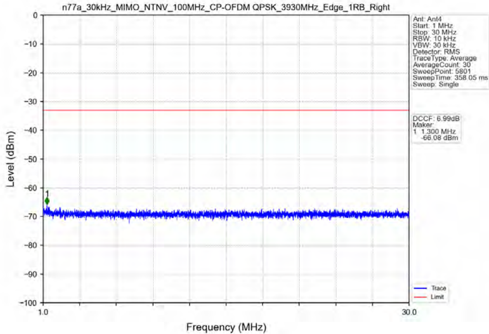
n77a_30kHz_MIMO_NTNV_100MHz_CP-OFDM_QPSK_3930MHz_Edge_1RB_Right
