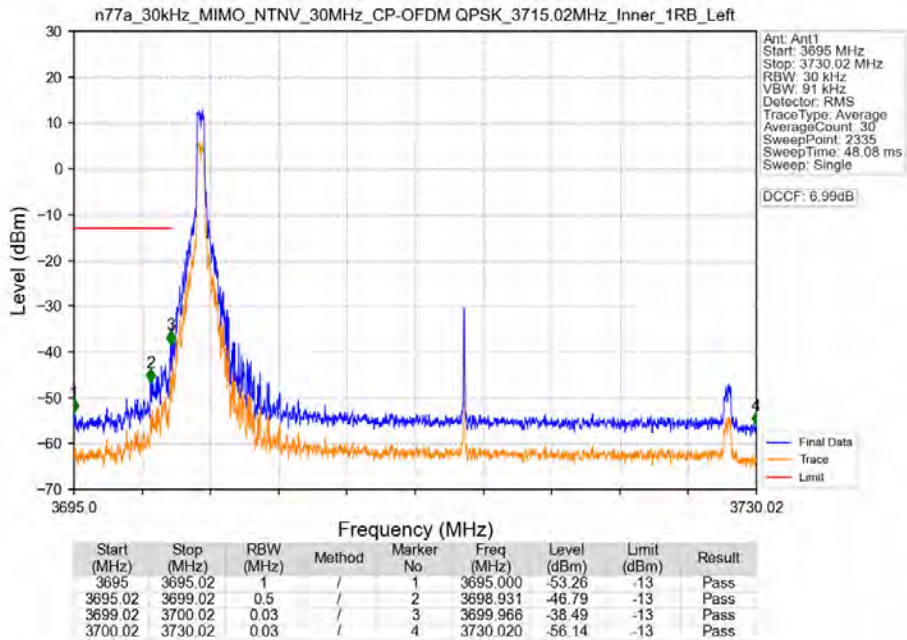
n77a_30kHz_MIMO_NTNV_30MHz_CP-OFDM QPSK_3715.02MHz_Inner_1RB_Left
