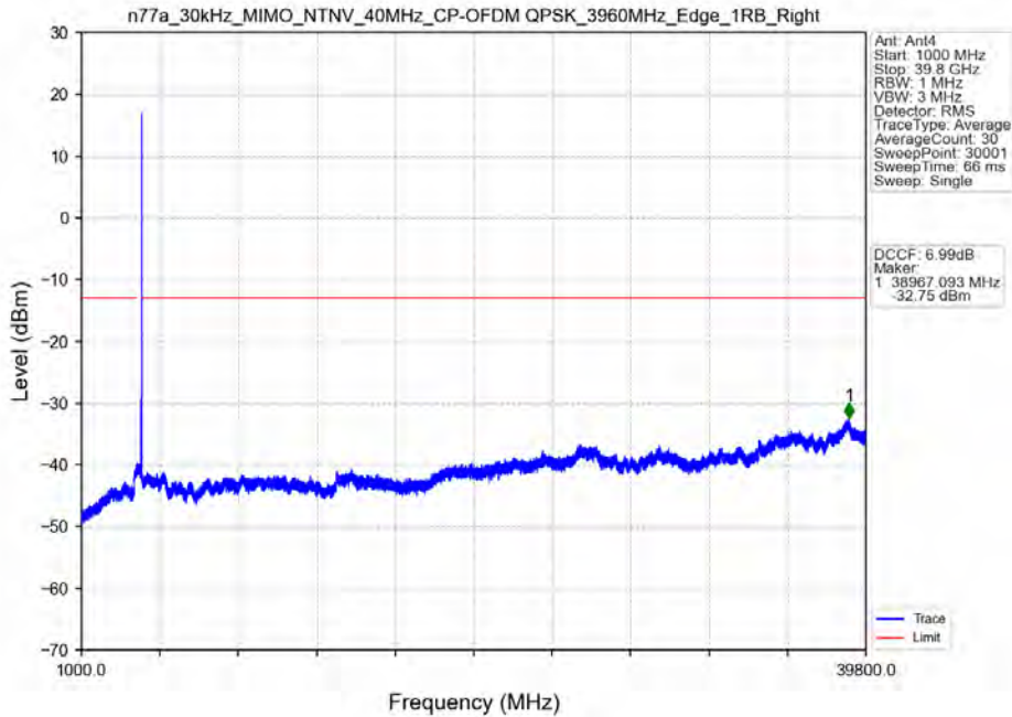
n77a_30kHz_MIMO_NTNV_40MHz_CP-OFDM QPSK_3960MHz_Edge_1RB_Right
