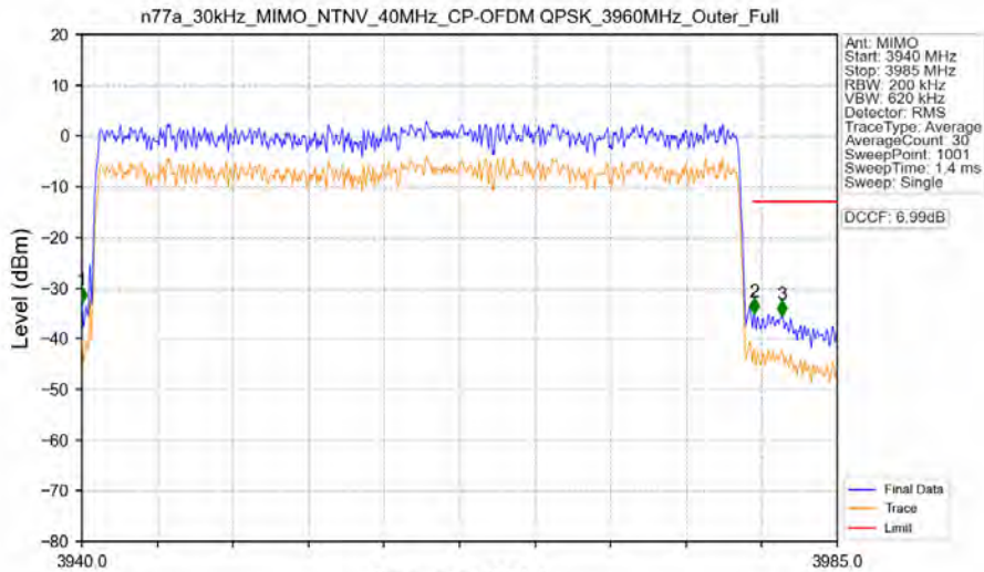
n77a_30kHz_MIMO_NTNV_40MHz_CP-OFDM QPSK_3960MHz_Outer_Full
