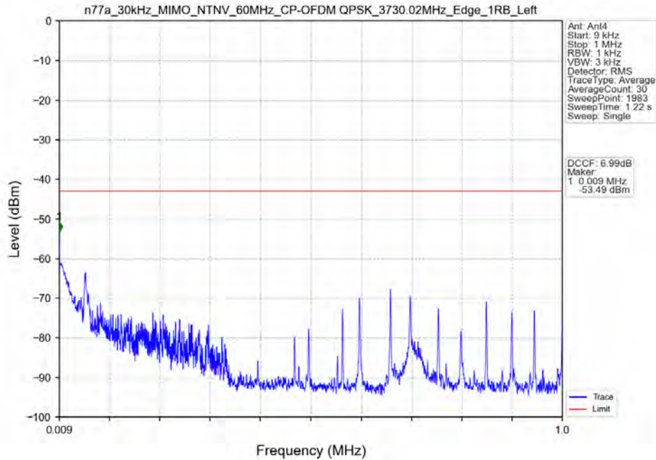
n77a_30kHz_MIMO_NTNV_60MHz_CP-OFDM QPSK_3730.02MHz_Edge_1RB_Left
