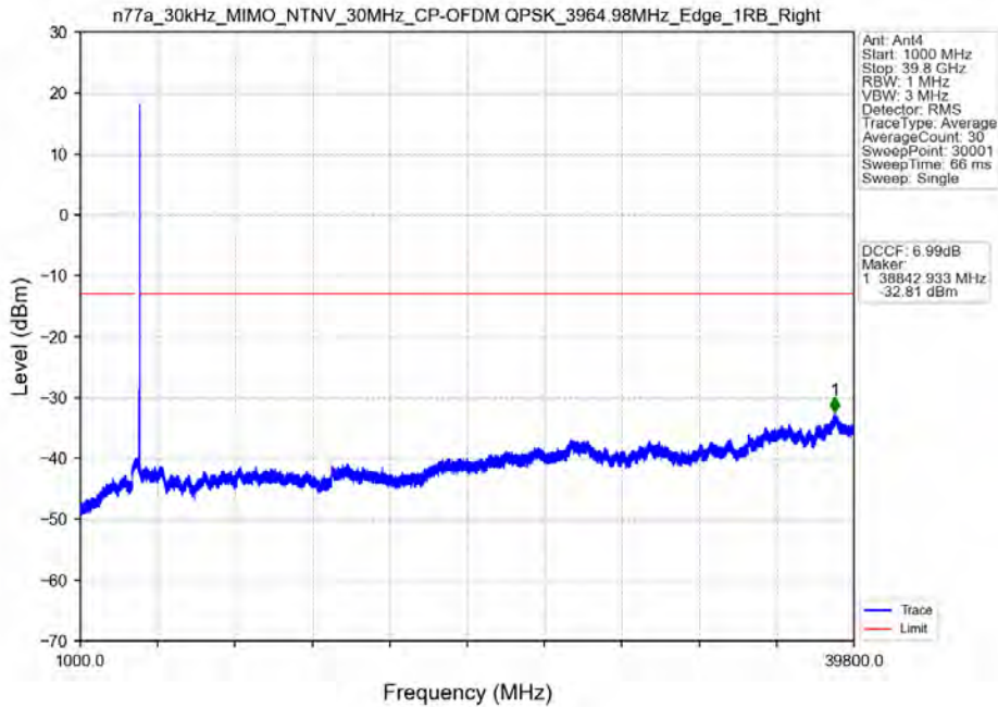
n77a_30kHz_MIMO_NTNV_30MHz_CP-OFDM QPSK_3964.98MHz_Edge_1RB_Right
