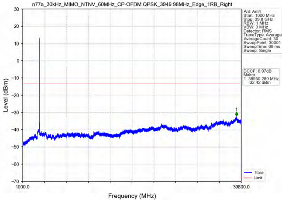
n77a_30kHz_MIMO_NTNV_60MHz_CP-OFDM_QPSK_3949.98MHz_Edge_1RB_Right
