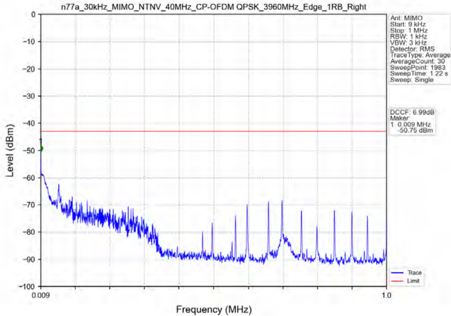
n77a_30kHz_MIMO_NTNV_40MHz_CP-OFDM QPSK_3960MHz_Edge_1RB_Right
