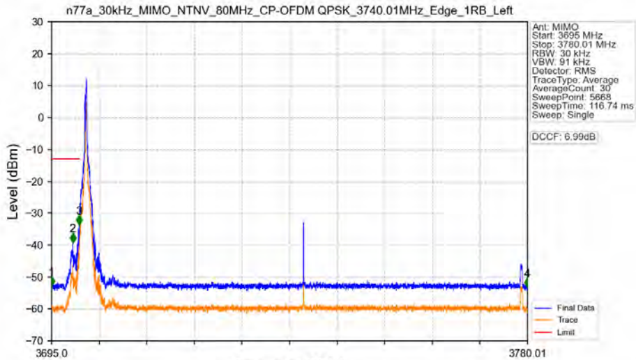
n77a_30kHz_MIMO_NTNV_80MHz_CP-OFDM QPSK_3740.01MHz_Edge_1RB_Left
