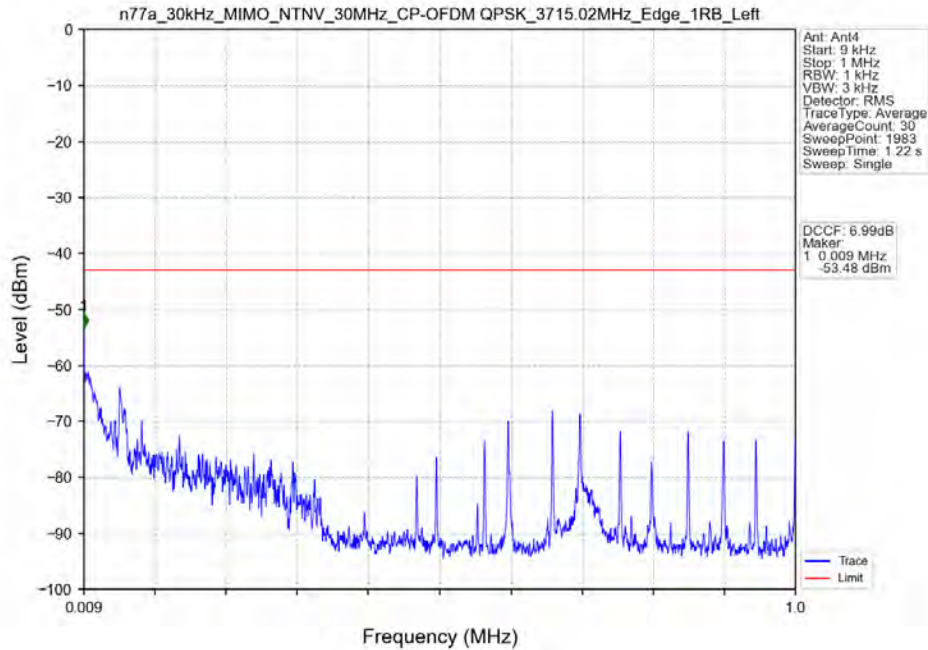
n77a_30kHz_MIMO_NTNV_30MHz_CP-OFDM QPSK_3715.02MHz_Edge_1RB_Left
