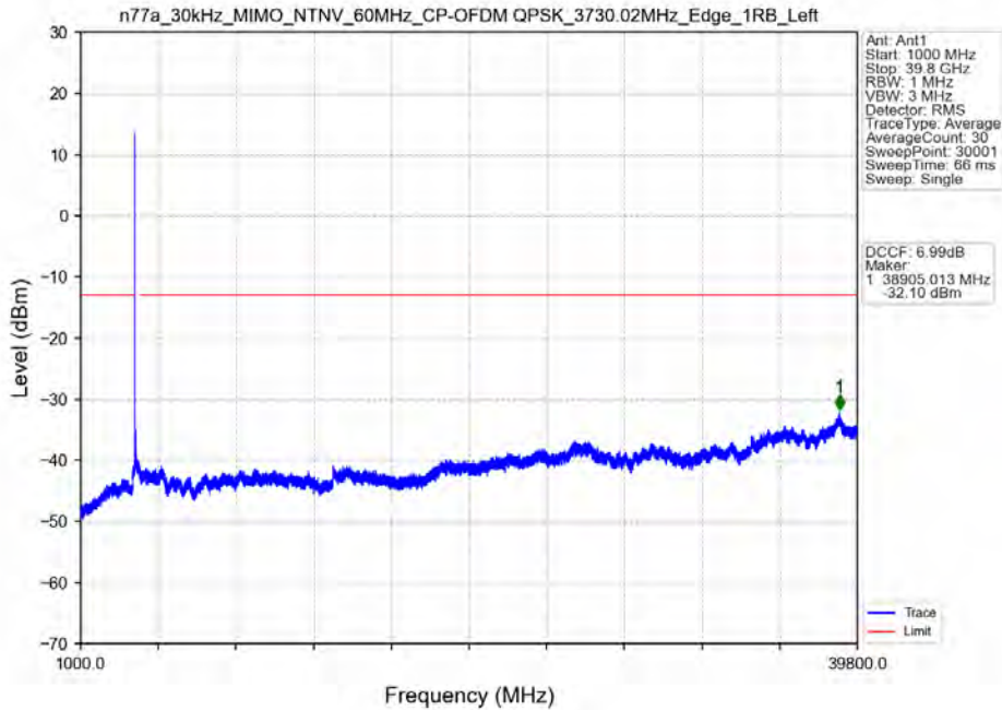
n77a_30kHz_MIMO_NTNV_60MHz_CP-OFDM QPSK_3730.02MHz_Edge_1RB_Left
