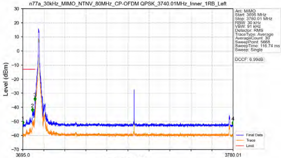
n77a_30kHz_MIMO_NTNV_80MHz_CP-OFDM QPSK_3740.01MHz_Inner_1RB_Left
