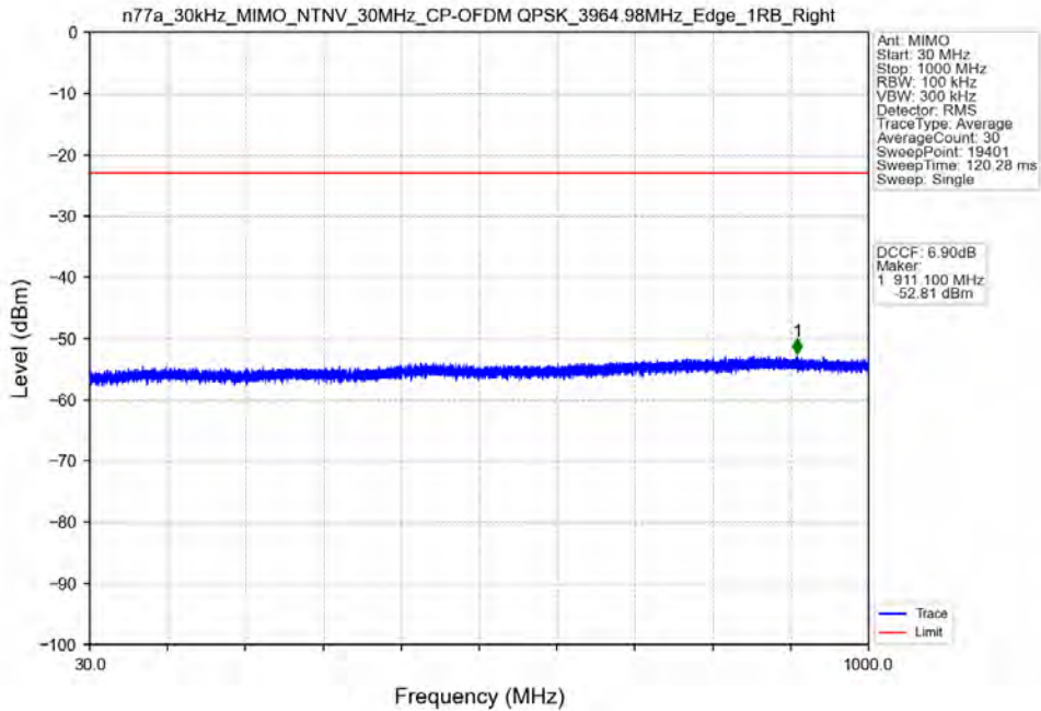
n77a_30kHz_MIMO_NTNV_30MHz_CP-OFDM QPSK_3964.98MHz_Edge_1RB_Right
