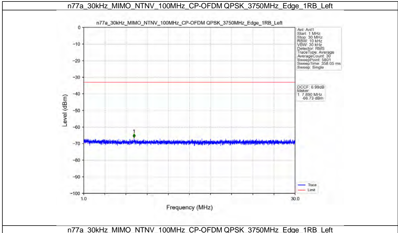
n77a_30kHz_MIMO_NTNV_100MHz_CP-OFDM QPSK_3750MHz_Edge_1RB_Left
