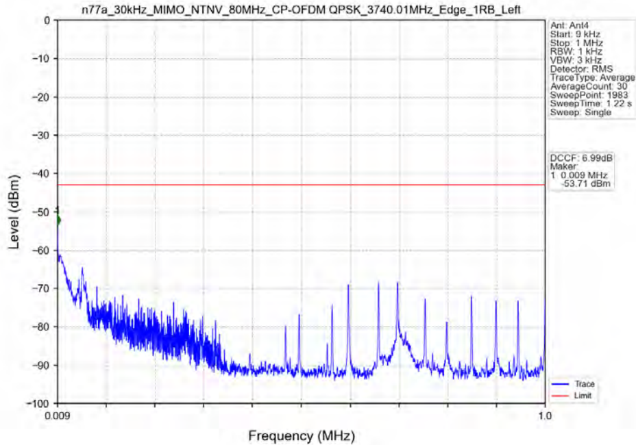
n77a_30kHz_MIMO_NTNV_80MHz_CP-OFDM QPSK_3740.01MHz_Edge_1RB_Left
