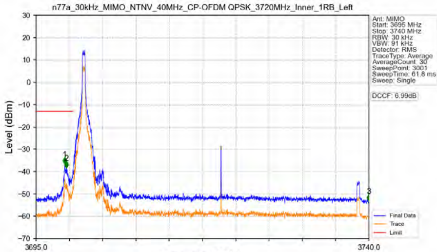
n77a_30kHz_MIMO_NTNV_40MHz_CP-OFDM QPSK_3720MHz_Inner_1RB_Left
