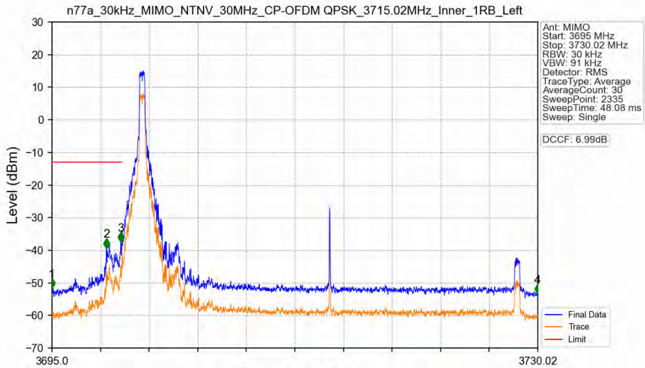
n77a_30kHz_MIMO_NTNV_30MHz_CP-OFDM QPSK_3715.02MHz_Inner_1RB_Left
