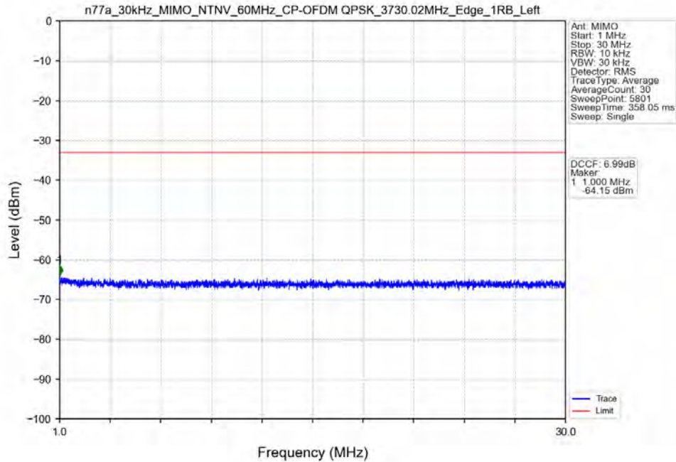
n77a_30kHz_MIMO_NTNV_60MHz_CP-OFDM QPSK_3730.02MHz_Edge_1RB_Left
