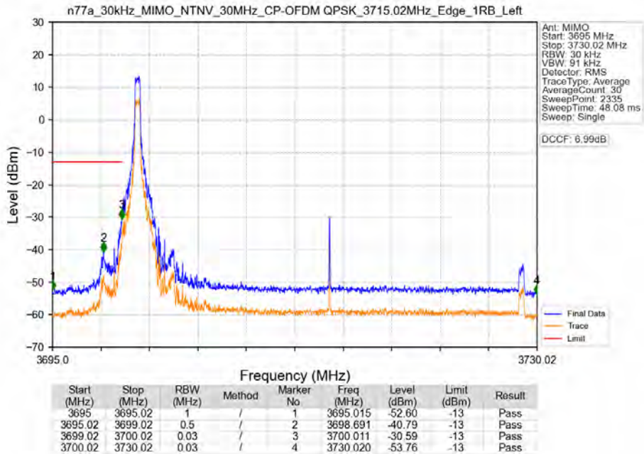
n77a_30kHz_MIMO_NTNV_30MHz_CP-OFDM QPSK_3715.02MHz_Edge_1RB_Left
