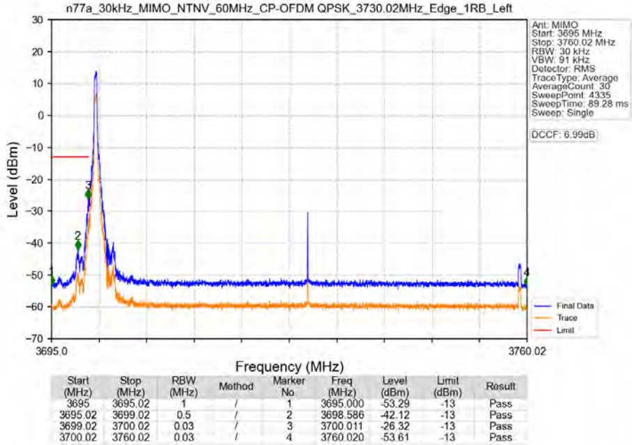
n77a_30kHz_MIMO_NTNV_60MHz_CP-OFDM QPSK_3730.02MHz_Edge_1RB_Left
