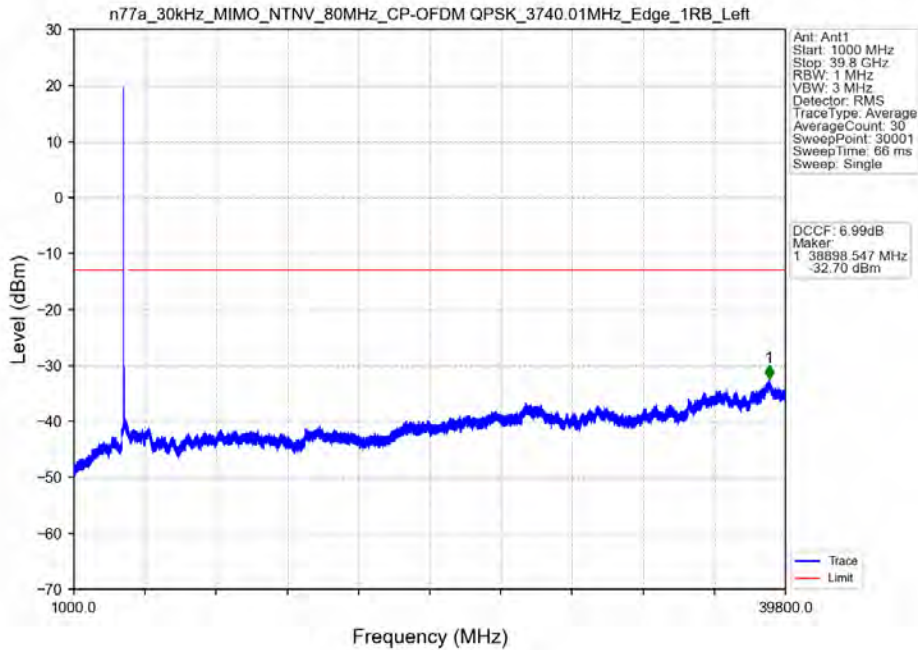
n77a_30kHz_MIMO_NTNV_80MHz_CP-OFDM QPSK_3740.01MHz_Edge_1RB_Left
