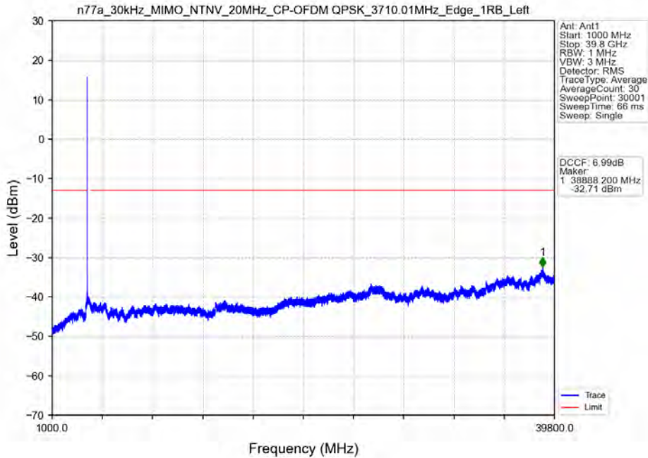
n77a_30kHz_MIMO_NTNV_20MHz_CP-OFDM QPSK_3710.01MHz_Edge_1RB_Left
