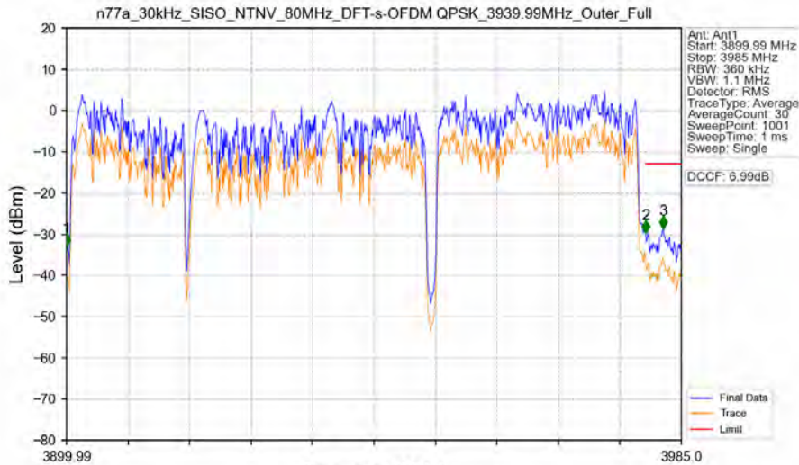
n77a_30kHz_SISO_NTNV_80MHz_DFT-s-OFDM QPSK_3939.99MHz_Outer_Full
