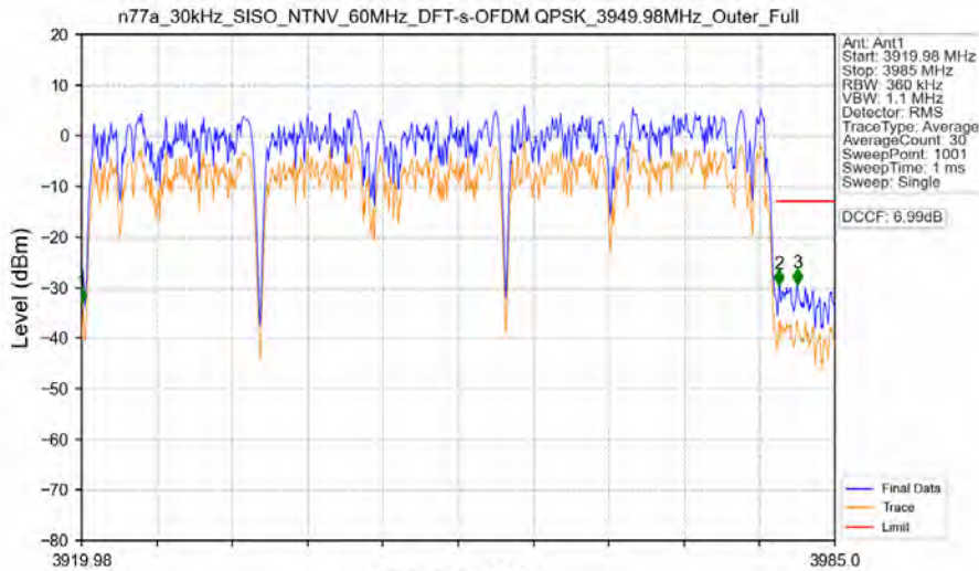
n77a_30kHz_SISO_NTNV_60MHz_DFT-s-OFDM QPSK_3949.98MHz_Outer_Full
