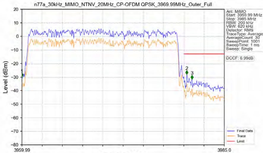
n77a_30kHz_MIMO_NTNV_20MHz_CP-OFDM QPSK_3969.99MHz_Outer_Full
