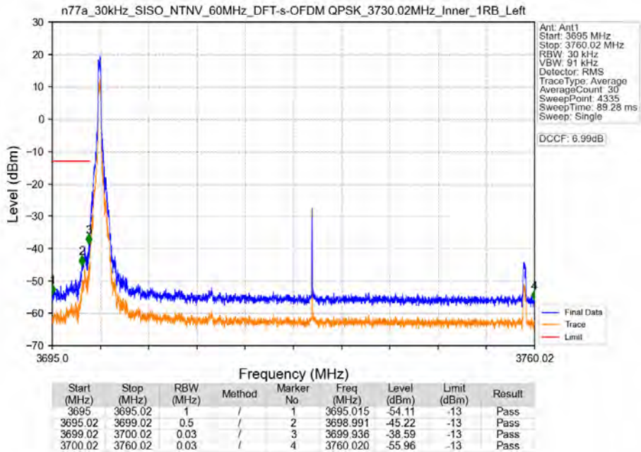
n77a_30kHz_SISO_NTNV_60MHz_DFT-s-OFDM_QPSK_3730.02MHz_Inner_1RB_Left
