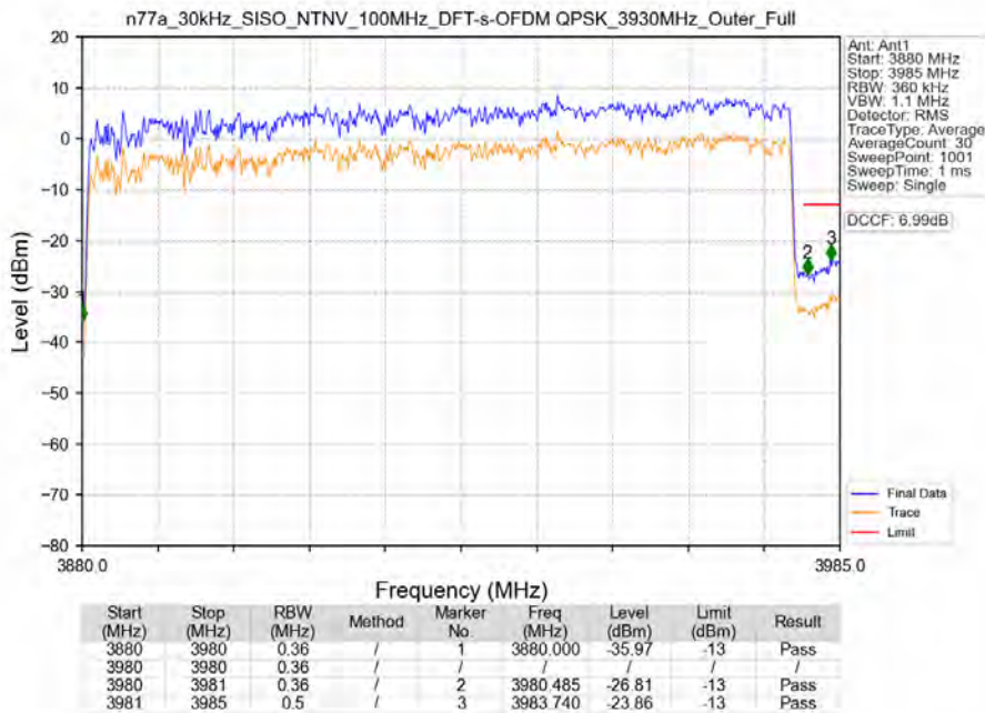
n77a_30kHz_SISO_NTNV_100MHz_DFT-s-OFDM QPSK_3930MHz_Outer_Full
