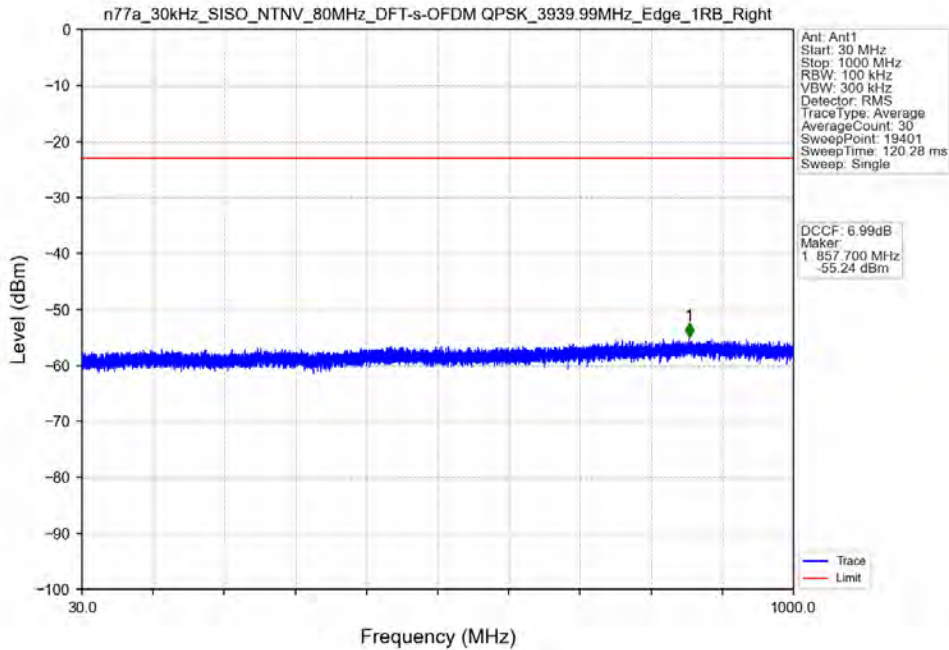
n77a_30kHz_SISO_NTNV_80MHz_DFT-s-OFDM QPSK_3939.99MHz_Edge_1RB_Right
