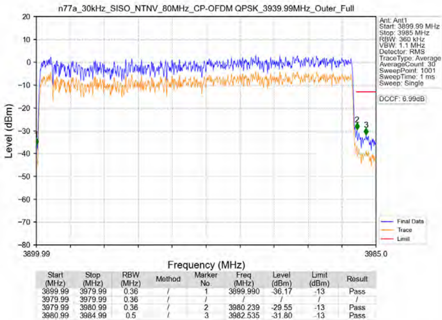
n77a_30kHz_SISO_NTNV_80MHz_CP-OFDM QPSK_3939.99MHz_Outer_Full
