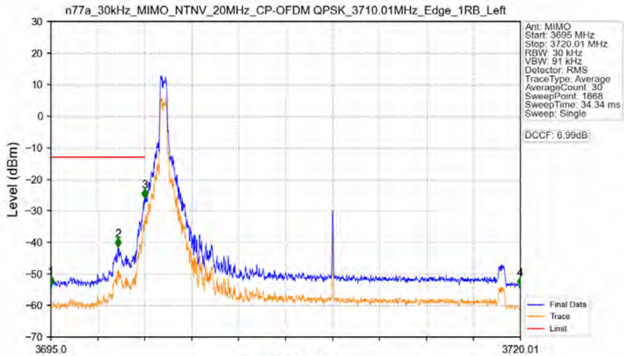
n77a_30kHz_MIMO_NTNV_20MHz_CP-OFDM QPSK_3710.01MHz_Edge_1RB_Left
