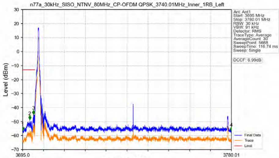
n77a_30kHz_SISO_NTNV_80MHz_CP-OFDM QPSK_3740.01MHz_Inner_1RB_Left
