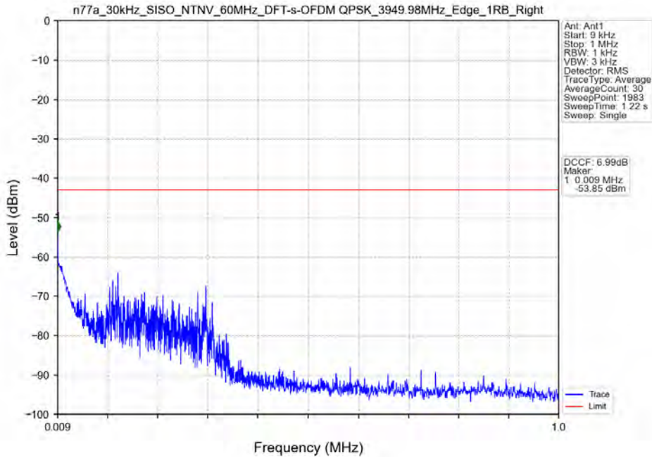
n77a_30kHz_SISO_NTNV_60MHz_DFT-s-OFDM QPSK_3949.98MHz_Edge_1RB_Right
