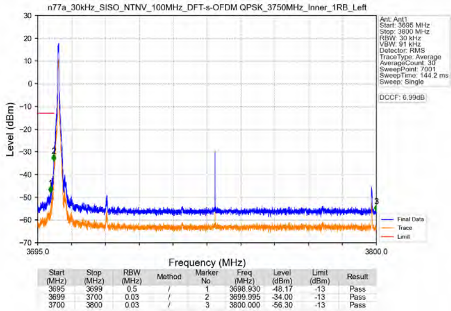
n77a_30kHz_SISO_NTNV_100MHz_DFT-s-OFDM_QPSK_3750MHz_Inner_1RB_Left
