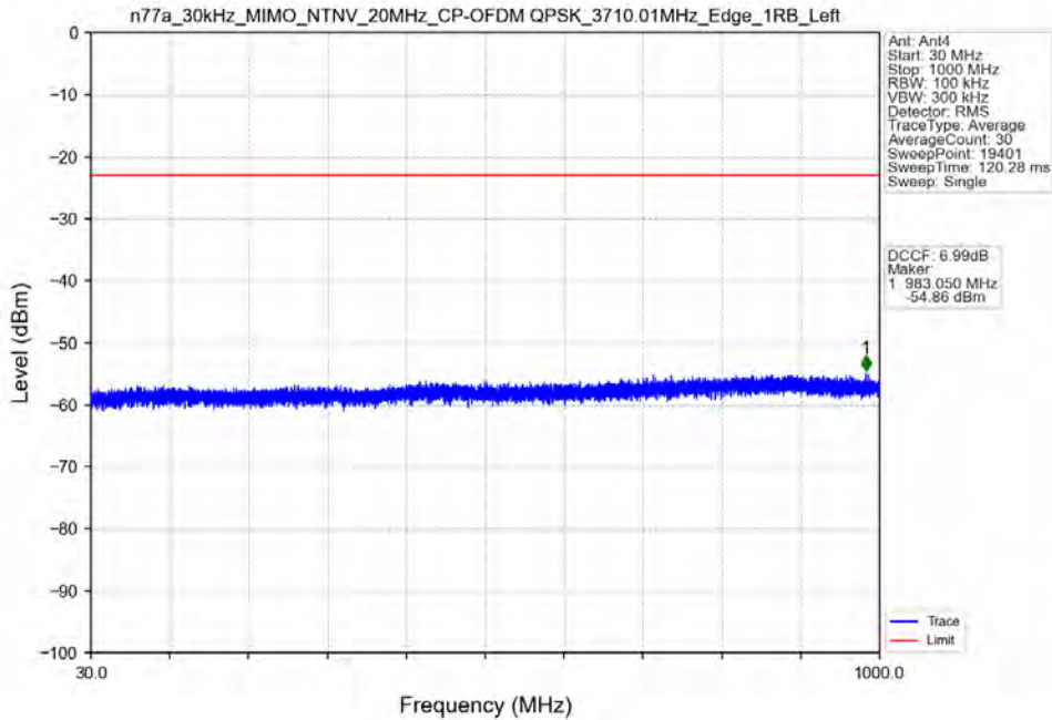
n77a_30kHz_MIMO_NTNV_20MHz_CP-OFDM QPSK_3710.01MHz_Edge_1RB_Left
