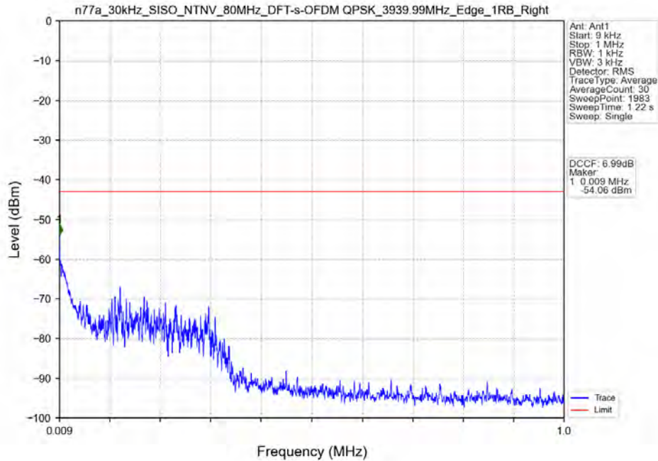
n77a_30kHz_SISO_NTNV_80MHz_DFT-s-OFDM QPSK_3939.99MHz_Edge_1RB_Right
