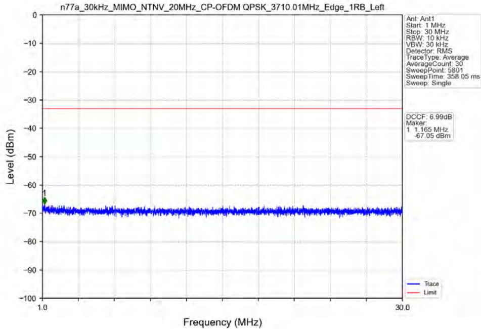
n77a_30kHz_MIMO_NTNV_20MHz_CP-OFDM QPSK_3710.01MHz_Edge_1RB_Left
