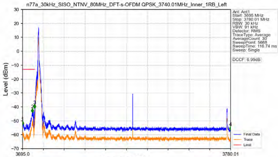
n77a_30kHz_SISO_NTNV_80MHz_DFT-s-OFDM_QPSK_3740.01MHz_Inner_1RB_Left
