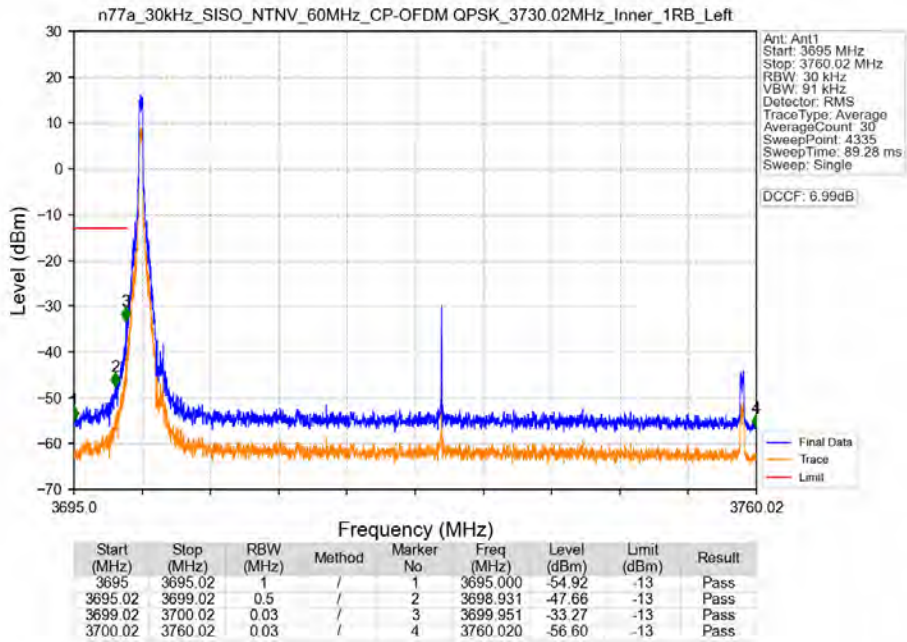
n77a_30kHz_SISO_NTNV_60MHz_CP-OFDM QPSK_3730.02MHz_Inner_1RB_Left
