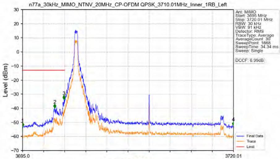
n77a_30kHz_MIMO_NTNV_20MHz_CP-OFDM QPSK_3710.01MHz_Inner_1RB_Left
