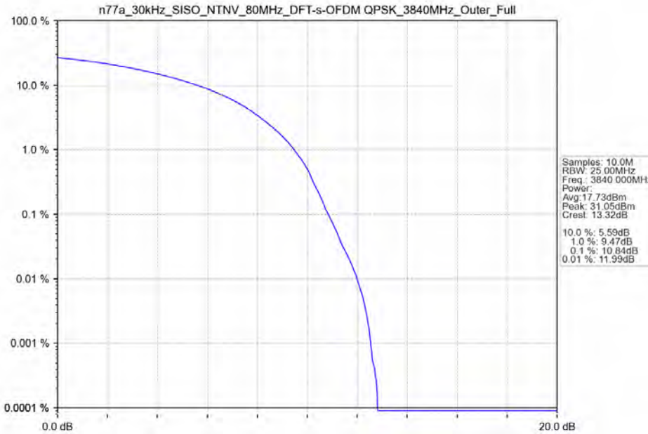
n77a_30kHz_SISO_NTNV_80MHz_DFT-s-OFDM QPSK_3840MHz_Outer_Full
