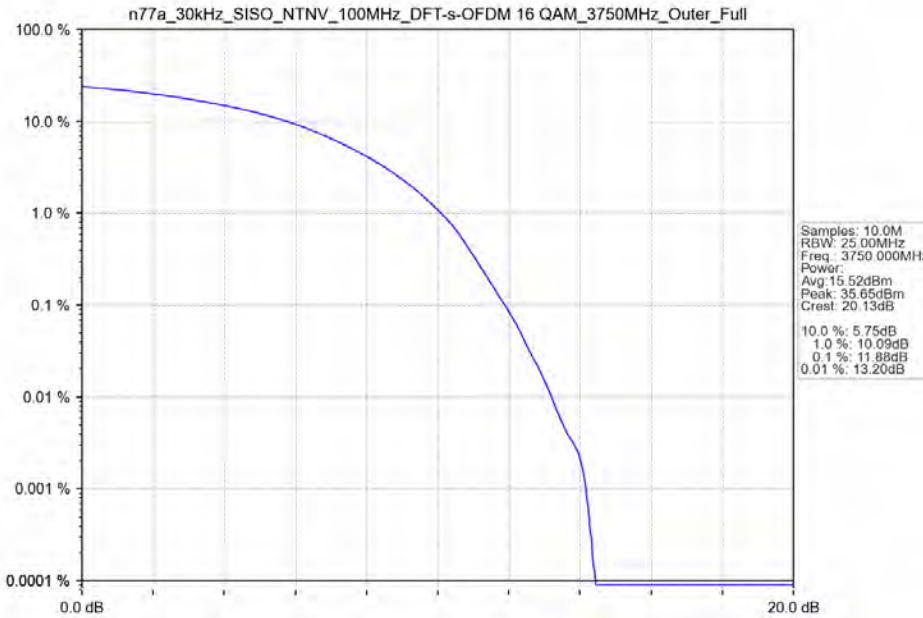
n77a_30kHz_SISO_NTNV_100MHz_DFT-s-OFDM 16 QAM_3750MHz_Outer_Full
