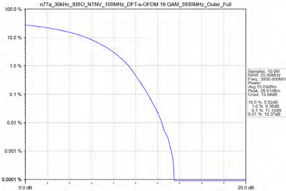
n77a_30kHz_SISO_NTNV_100MHz_DFT-s-OFDM 16 QAM_3930MHz_Outer_Full
