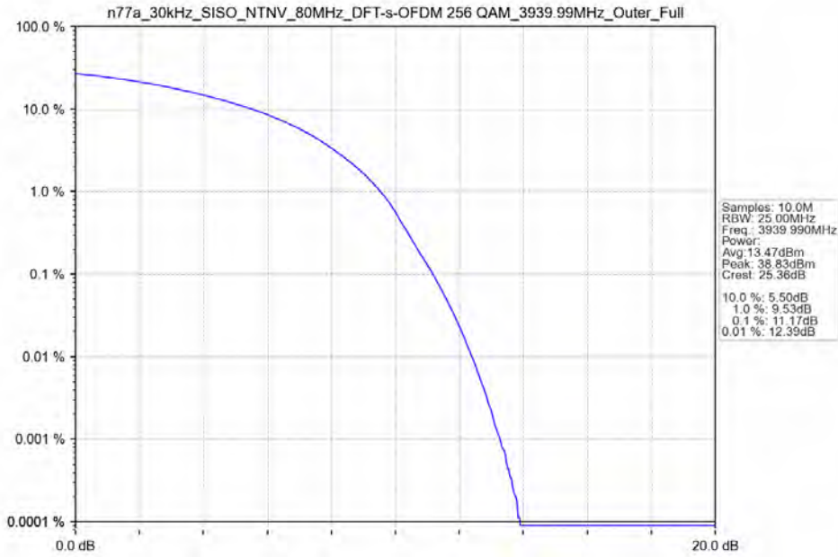
n77a_30kHz_SISO_NTNV_80MHz_DFT-s-OFDM 256 QAM_3939.99MHz_Outer_Full
