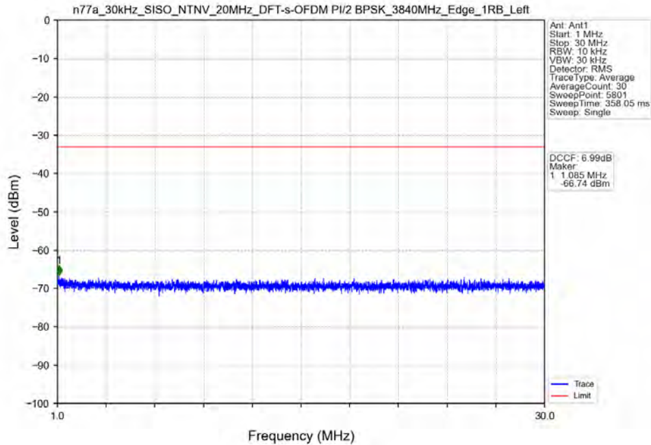
n77a_30kHz_SISO_NTNV_20MHz_DFT-s-OFDM PI/2 BPSK_3840MHz_Edge_1RB_Left
