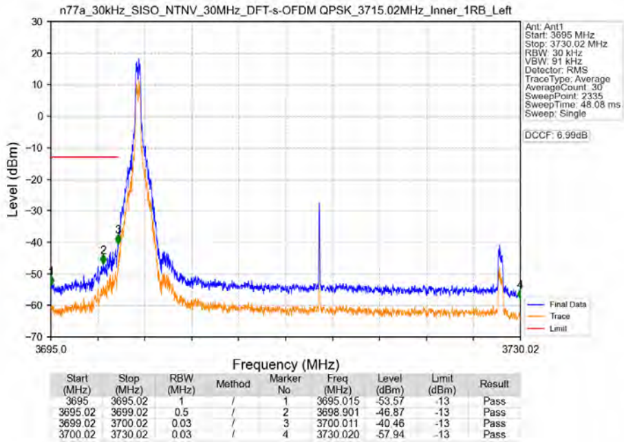
n77a_30kHz_SISO_NTNV_30MHz_DFT-s-OFDM_QPSK_3715.02MHz_Inner_1RB_Left
