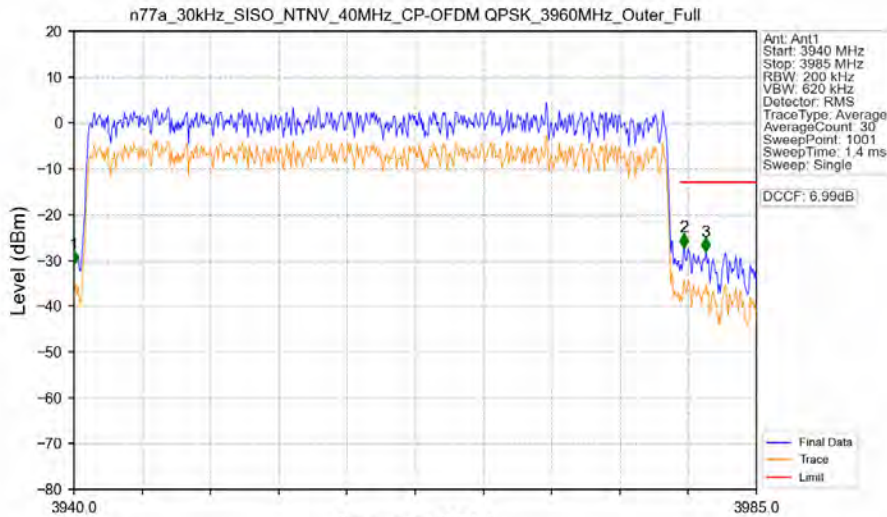
n77a_30kHz_SISO_NTNV_40MHz_CP-OFDM QPSK_3960MHz_Outer_Full
