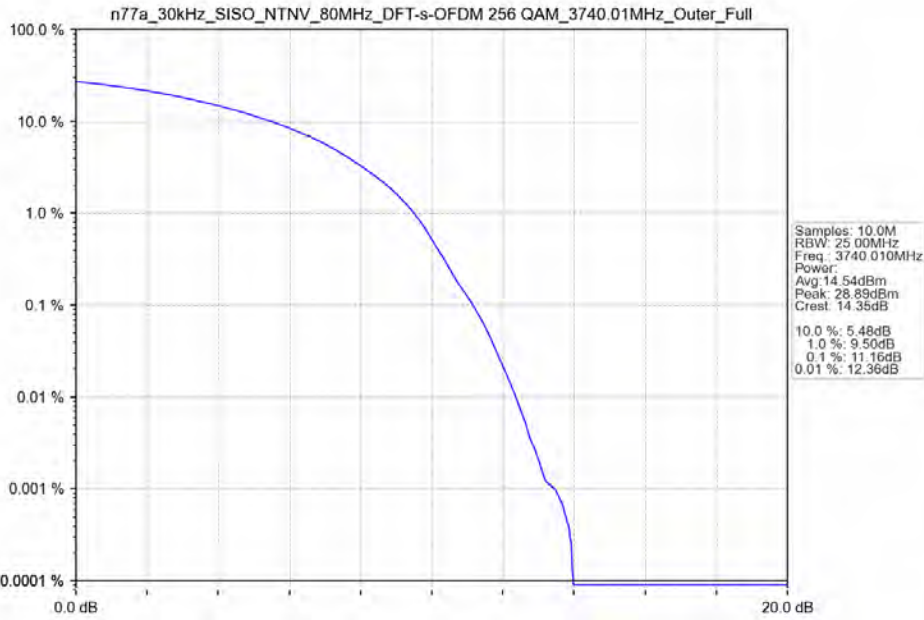
n77a_30kHz_SISO_NTNV_80MHz_DFT-s-OFDM 256 QAM_3740.01MHz_Outer_Full
