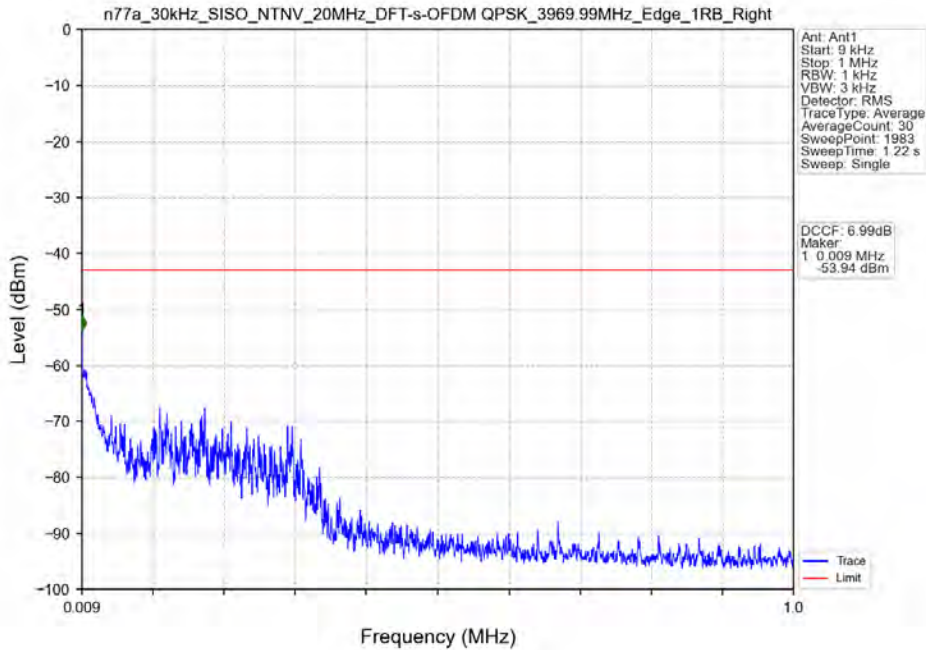
n77a_30kHz_SISO_NTNV_20MHz_DFT-s-OFDM QPSK_3969.99MHz_Edge_1RB_Right
