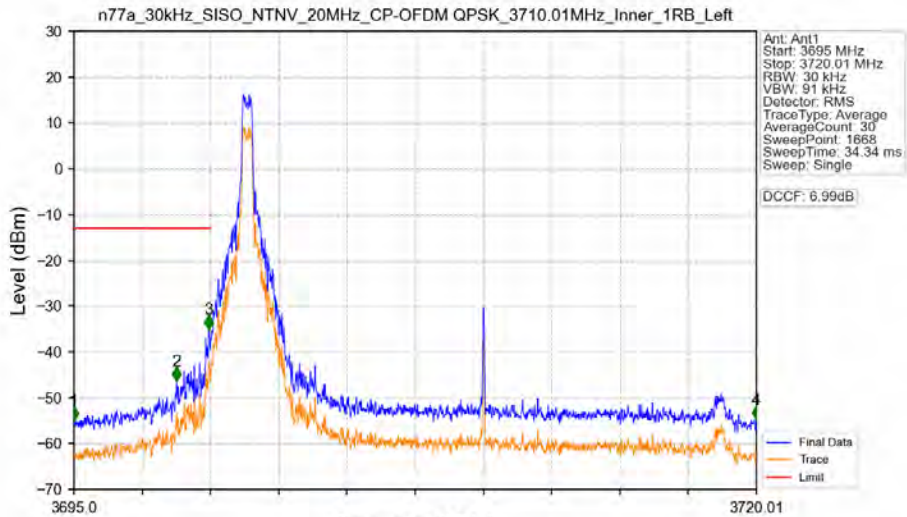
n77a_30kHz_SISO_NTNV_20MHz_CP-OFDM QPSK_3710.01MHz_Inner_1RB_Left
