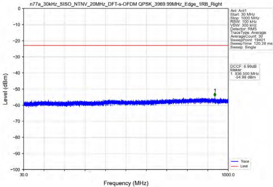
n77a_30kHz_SISO_NTNV_20MHz_DFT-s-OFDM QPSK_3969.99MHz_Edge_1RB_Right
