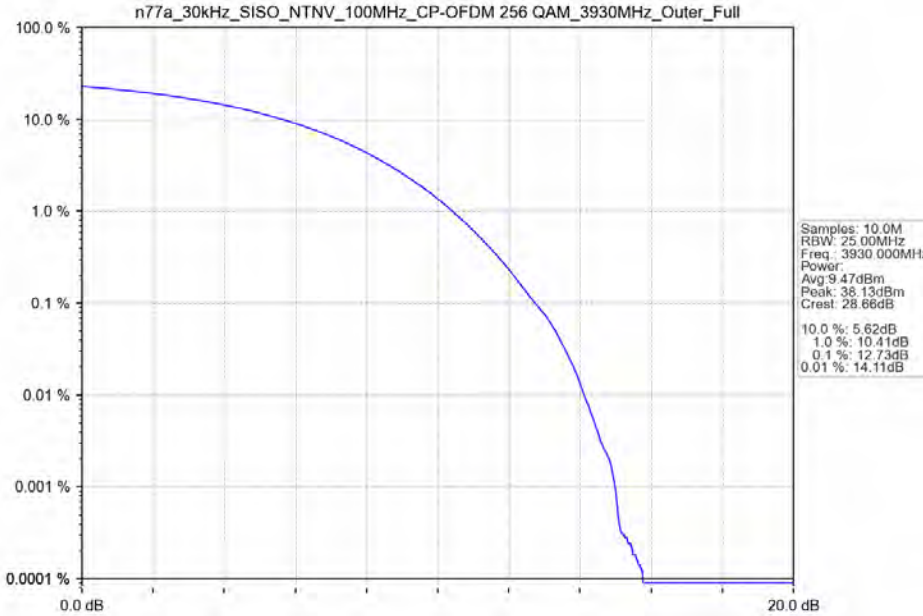
n77a_30kHz_SISO_NTNV_100MHz_CP-OFDM 256 QAM_3930MHz_Outer_Full
