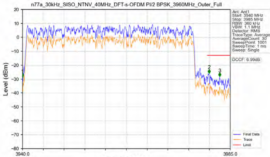
n77a_30kHz_SISO_NTNV_40MHz_DFT-s-OFDM PI/2 BPSK_3960MHz_Outer_Full
