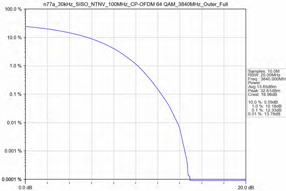
n77a_30kHz_SISO_NTNV_100MHz_CP-OFDM 64 QAM_3840MHz_Outer_Full
