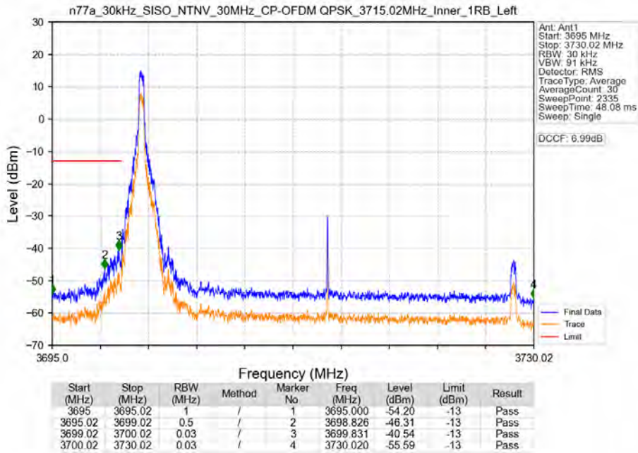
n77a_30kHz_SISO_NTNV_30MHz_CP-OFDM QPSK_3715.02MHz_Inner_1RB_Left
