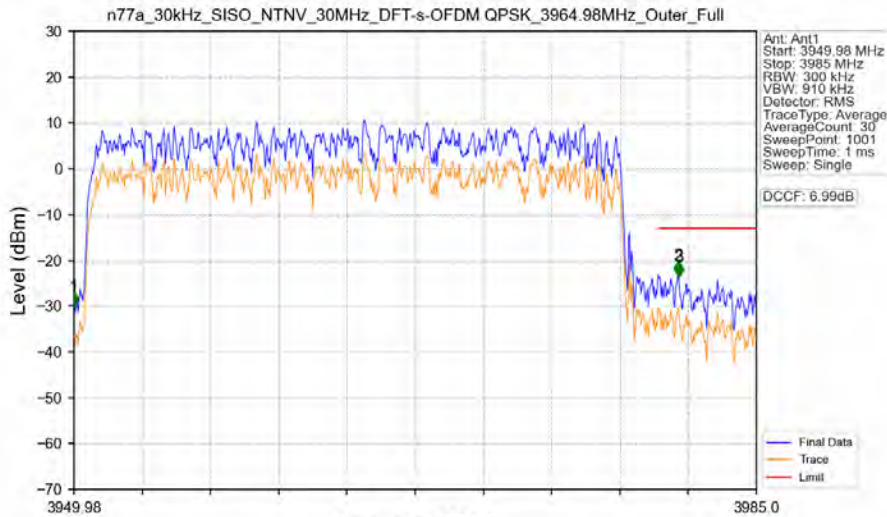
n77a_30kHz_SISO_NTNV_30MHz_DFT-s-OFDM QPSK_3964.98MHz_Outer_Full
