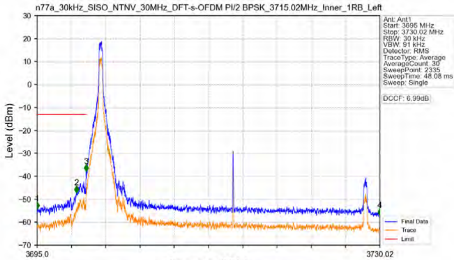
n77a_30kHz_SISO_NTNV_30MHz_DFT-s-OFDM PI/2 BPSK_3715.02MHz_Inner_1RB_Left
