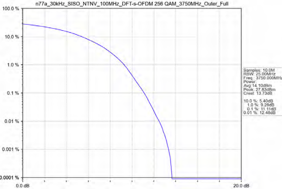
n77a_30kHz_SISO_NTNV_100MHz_DFT-s-OFDM_256_QAM_3750MHz_Outer_Full
