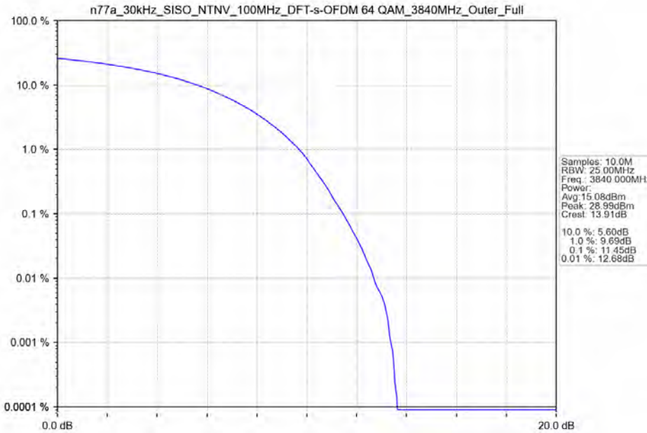
n77a_30kHz_SISO_NTNV_100MHz_DFT-s-OFDM 64 QAM_3840MHz_Outer_Full
