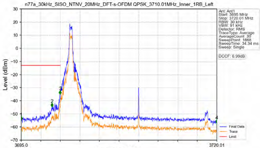
n77a_30kHz_SISO_NTNV_20MHz_DFT-s-OFDM_QPSK_3710.01MHz_Inner_1RB_Left
