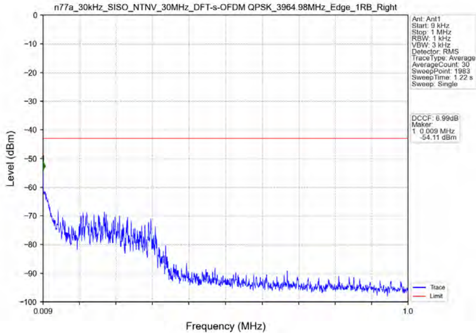
n77a_30kHz_SISO_NTNV_30MHz_DFT-s-OFDM QPSK_3964.98MHz_Edge_1RB_Right
