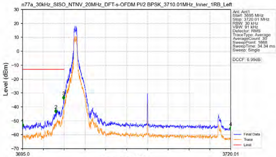
n77a_30kHz_SISO_NTNV_20MHz_DFT-s-OFDM PI/2 BPSK_3710.01MHz_Inner_1RB_Left
