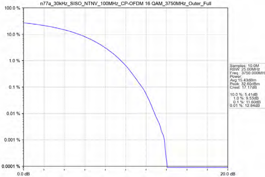
n77a_30kHz_SISO_NTNV_100MHz_CP-OFDM 16 QAM_3750MHz_Outer_Full
