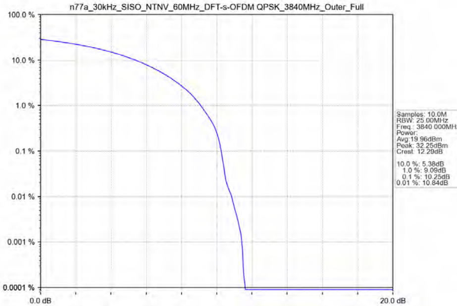
n77a_30kHz_SISO_NTNV_60MHz_DFT-s-OFDM QPSK_3840MHz_Outer_Full
