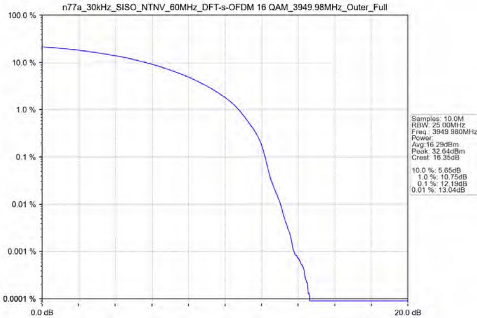
n77a_30kHz_SISO_NTNV_60MHz_DFT-s-OFDM 16 QAM_3949.98MHz_Outer_Full
