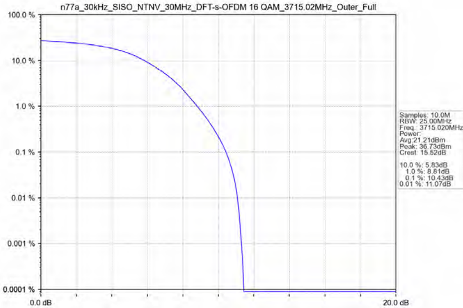
n77a_30kHz_SISO_NTNV_30MHz_DFT-s-OFDM 16 QAM_3715.02MHz_Outer_Full
