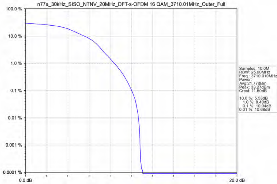
n77a_30kHz_SISO_NTNV_20MHz_DFT-s-OFDM 16 QAM_3710.01MHz_Outer_Full
