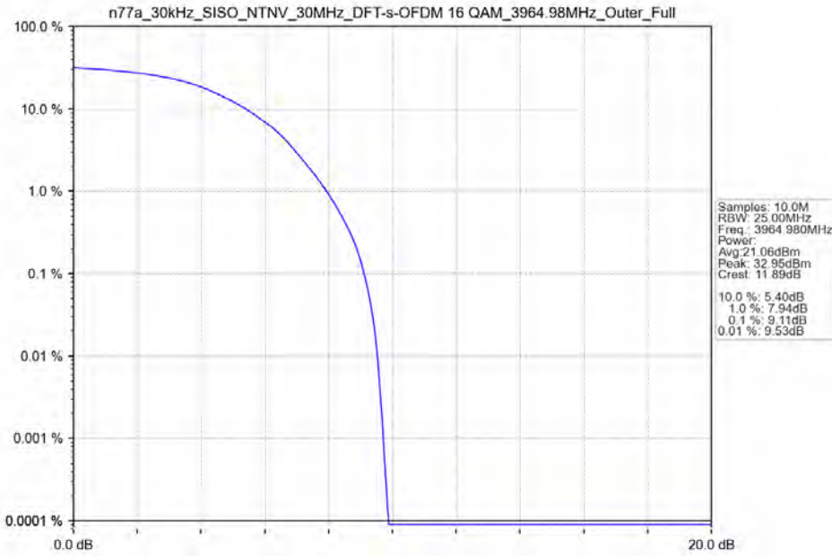
n77a_30kHz_SISO_NTNV_30MHz_DFT-s-OFDM 16 QAM_3964.98MHz_Outer_Full
