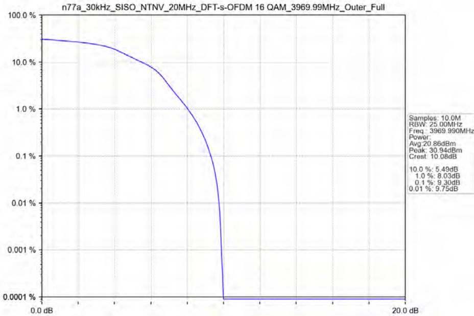
n77a_30kHz_SISO_NTNV_20MHz_DFT-s-OFDM 16 QAM_3969.99MHz_Outer_Full
