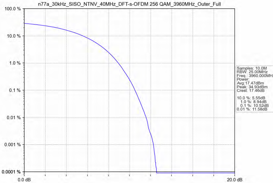
n77a_30kHz_SISO_NTNV_40MHz_DFT-s-OFDM 256 QAM_3960MHz_Outer_Full
