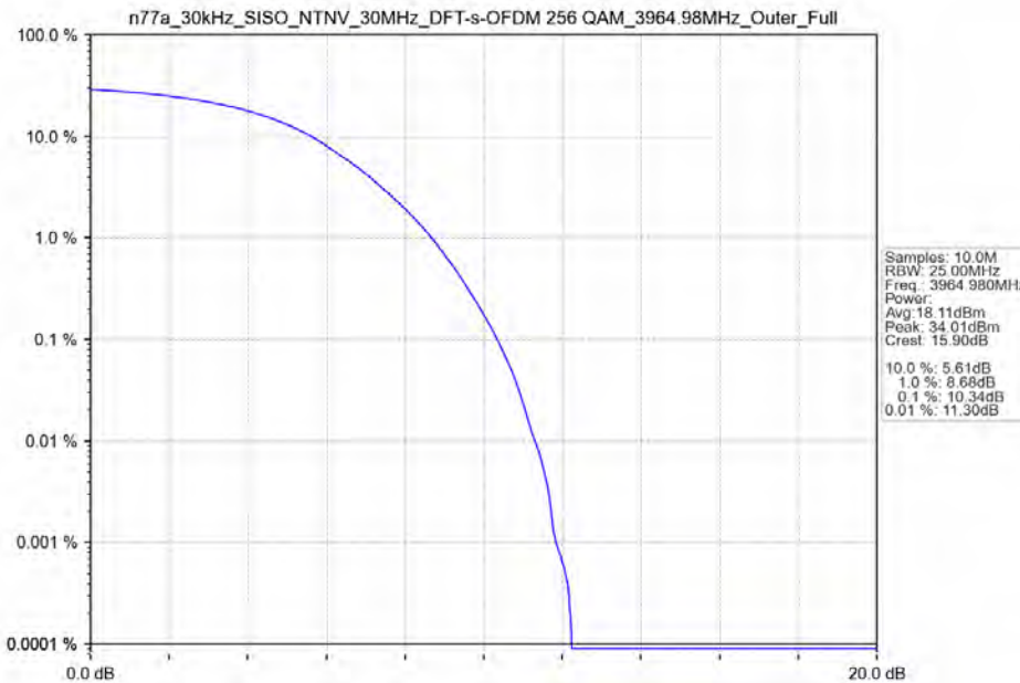
n77a_30kHz_SISO_NTNV_30MHz_DFT-s-OFDM 256 QAM_3964.98MHz_Outer_Full
