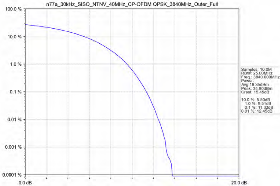
n77a_30kHz_SISO_NTNV_40MHz_CP-OFDM QPSK_3840MHz_Outer_Full
