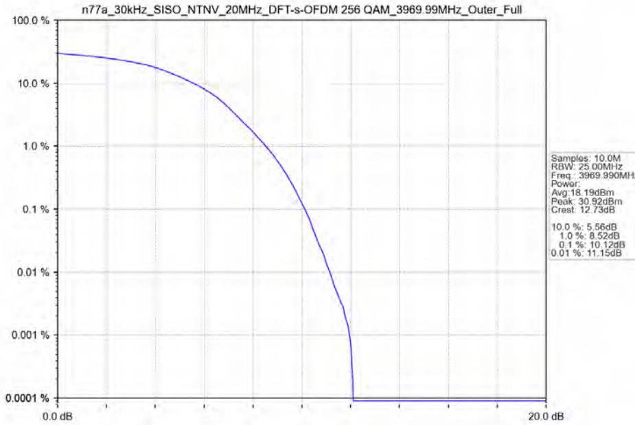
n77a_30kHz_SISO_NTNV_20MHz_DFT-s-OFDM 256 QAM_3969.99MHz_Outer_Full
