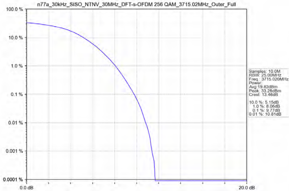
n77a_30kHz_SISO_NTNV_30MHz_DFT-s-OFDM 256 QAM_3715.02MHz_Outer_Full
