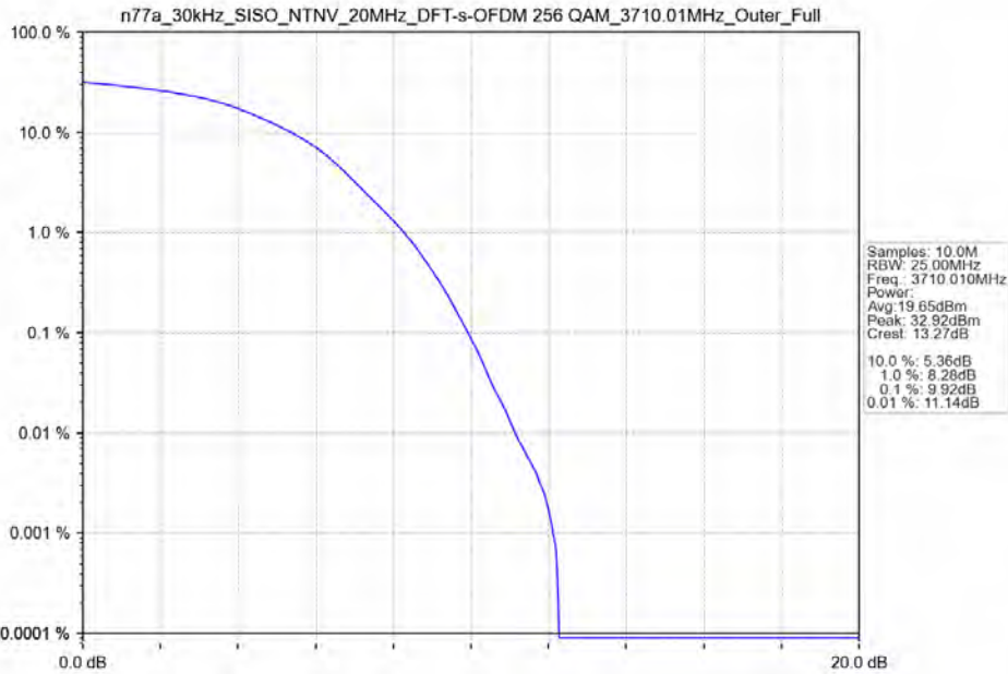
n77a_30kHz_SISO_NTNV_20MHz_DFT-s-OFDM 256 QAM_3710.01MHz_Outer_Full
