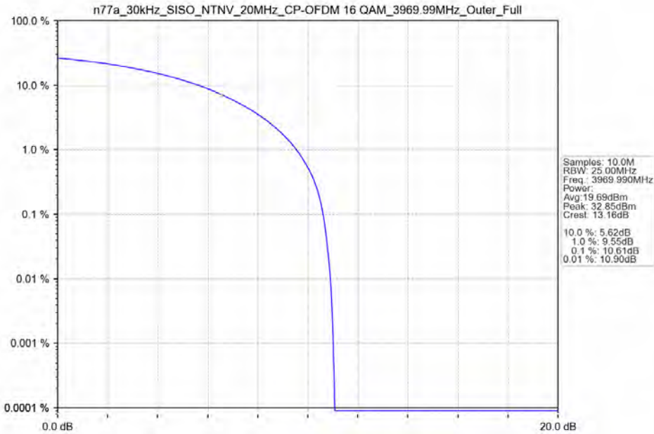
n77a_30kHz_SISO_NTNV_20MHz_CP-OFDM 16 QAM_3969.99MHz_Outer_Full
