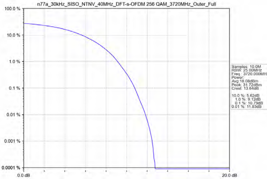
n77a_30kHz_SISO_NTNV_40MHz_DFT-s-OFDM 256 QAM_3720MHz_Outer_Full
