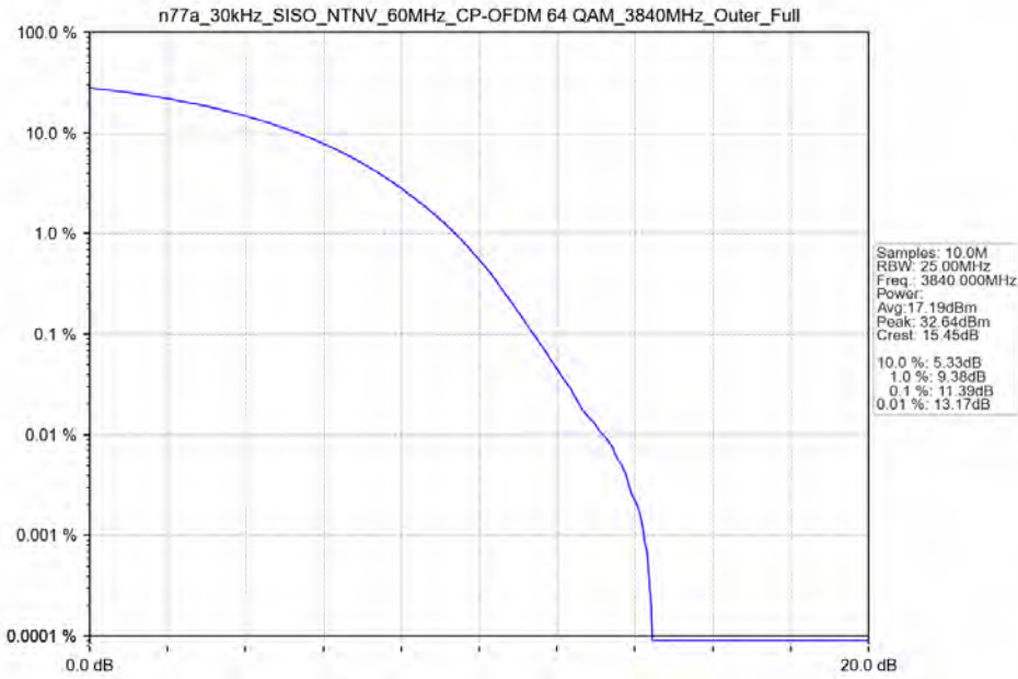
n77a_30kHz_SISO_NTNV_60MHz_CP-OFDM 64 QAM_3840MHz_Outer_Full
