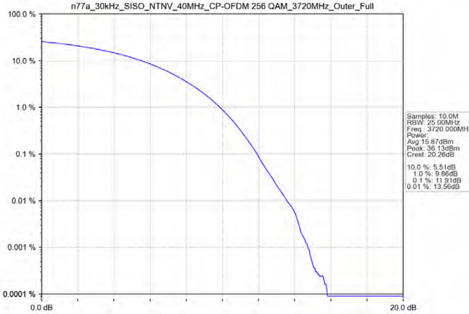
n77a_30kHz_SISO_NTNV_40MHz_CP-OFDM 256 QAM_3720MHz_Outer_Full
