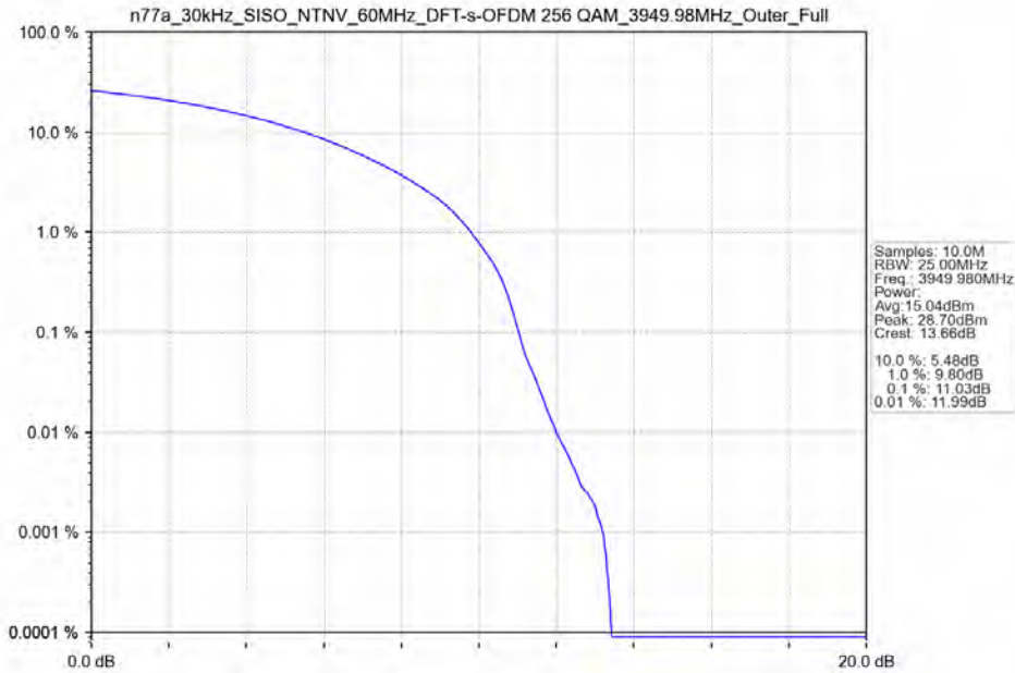
n77a_30kHz_SISO_NTNV_60MHz_DFT-s-OFDM 256 QAM_3949.98MHz_Outer_Full
