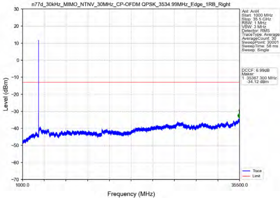
n77d_30kHz_MIMO_NTNV_30MHz_CP-OFDM QPSK_3534.99MHz_Edge_1RB_Right
