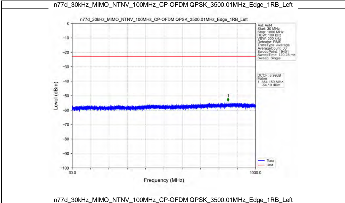
n77d_30kHz_MIMO_NTNV_100MHz_CP-OFDM QPSK_3500.01MHz_Edge_1RB_Left
