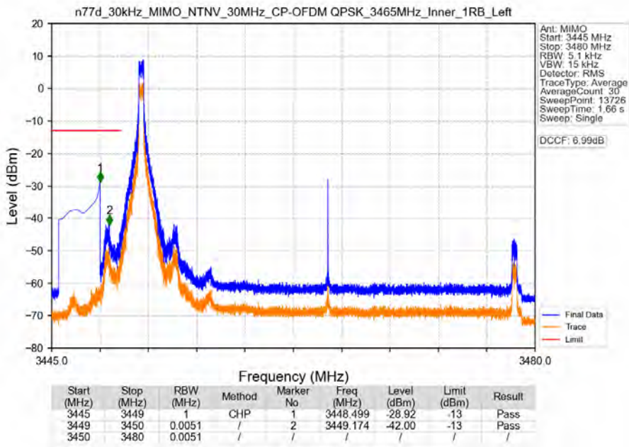
n77d_30kHz_MIMO_NTNV_30MHz_CP-OFDM QPSK_3465MHz_Inner_1RB_Left
