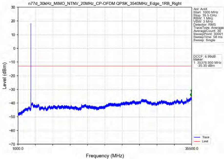
n77d_30kHz_MIMO_NTNV_20MHz_CP-OFDM QPSK_3540MHz_Edge_1RB_Right
