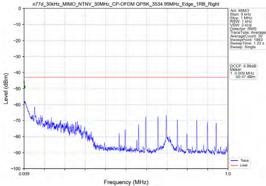
n77d_30kHz_MIMO_NTNV_30MHz_CP-OFDM QPSK_3534.99MHz_Edge_1RB_Right
