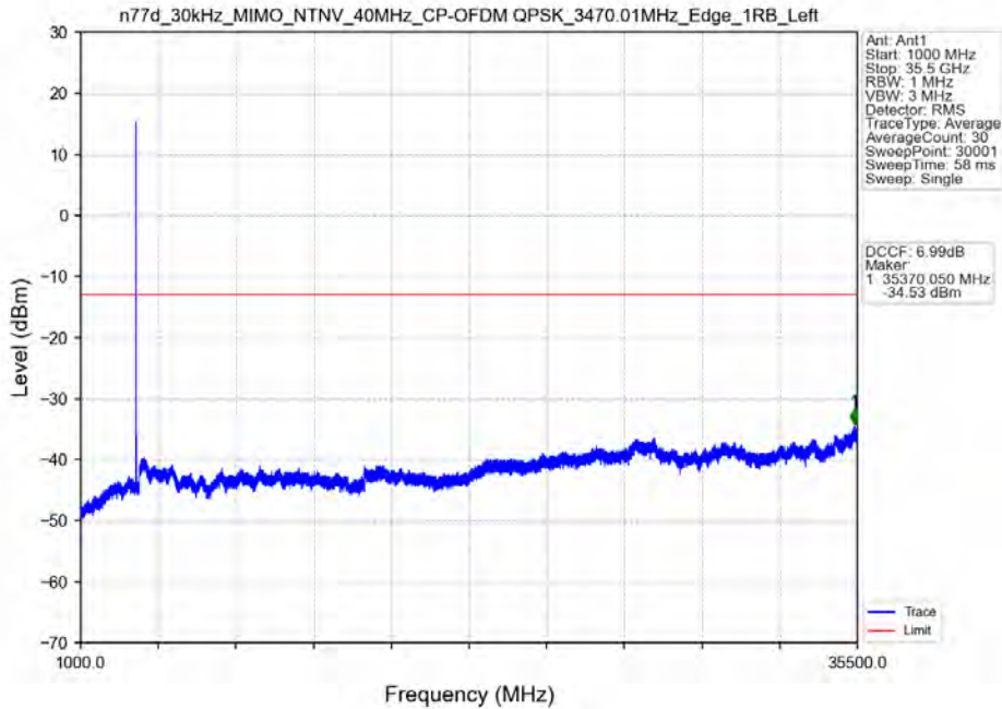
n77d_30kHz_MIMO_NTNV_40MHz_CP-OFDM QPSK_3470.01MHz_Edge_1RB_Left
