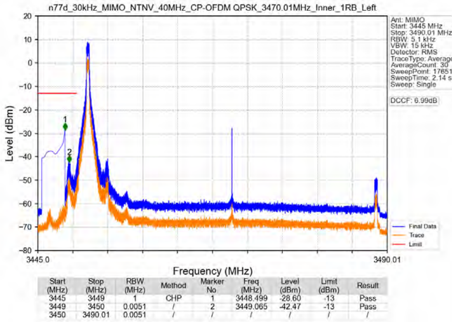
n77d_30kHz_MIMO_NTNV_40MHz_CP-OFDM QPSK_3470.01MHz_Inner_1RB_Left
