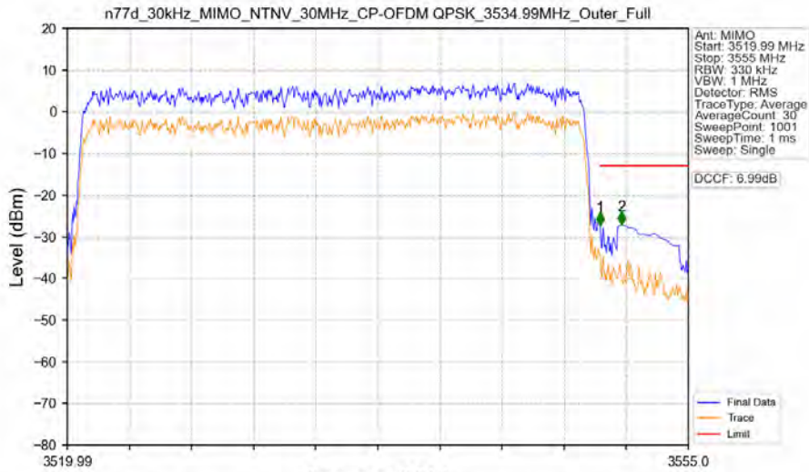
n77d_30kHz_MIMO_NTNV_30MHz_CP-OFDM QPSK_3534.99MHz_Outer_Full
