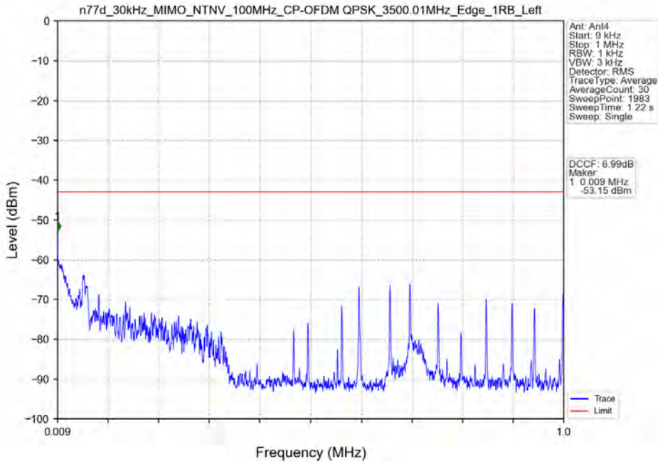
n77d_30kHz_MIMO_NTNV_100MHz_CP-OFDM QPSK_3500.01MHz_Edge_1RB_Left
