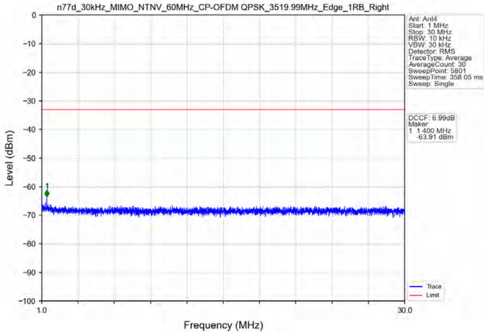
n77d_30kHz_MIMO_NTNV_60MHz_CP-OFDM QPSK_3519.99MHz_Edge_1RB_Right
