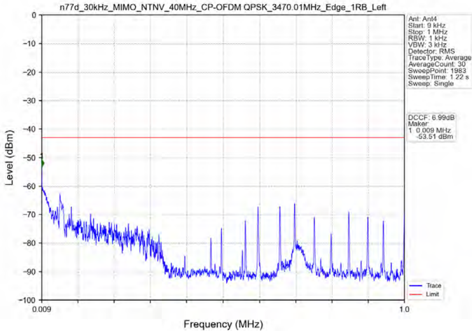
n77d_30kHz_MIMO_NTNV_40MHz_CP-OFDM QPSK_3470.01MHz_Edge_1RB_Left
