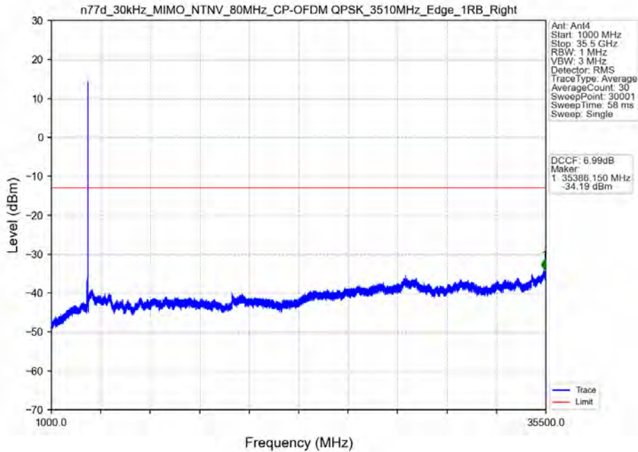
n77d_30kHz_MIMO_NTNV_80MHz_CP-OFDM QPSK_3510MHz_Edge_1RB_Right
