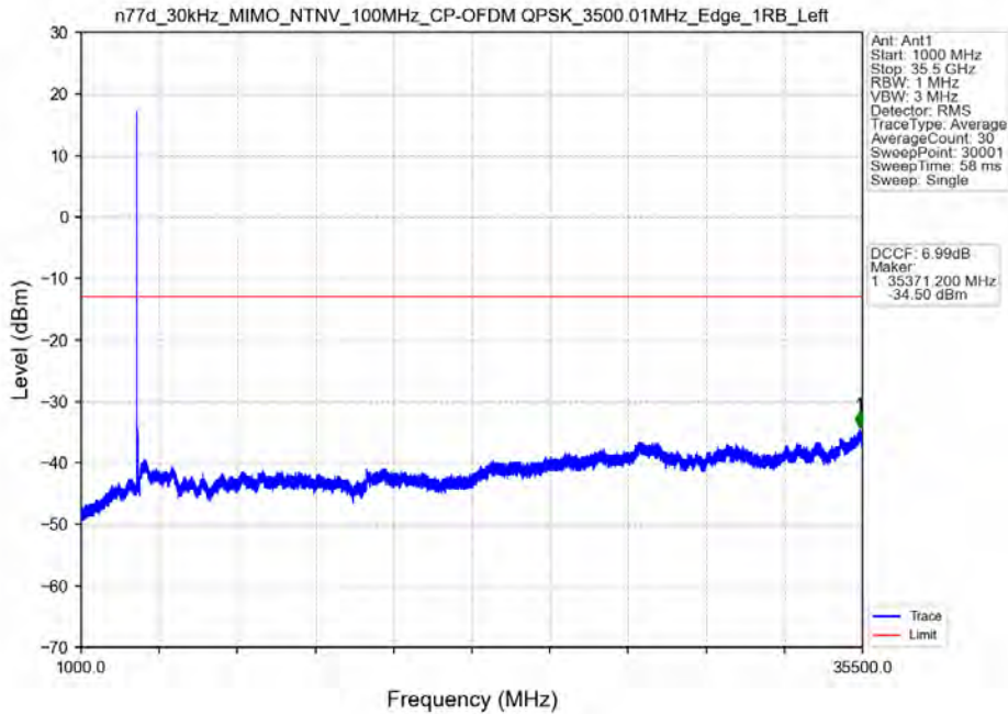
n77d_30kHz_MIMO_NTNV_100MHz_CP-OFDM QPSK_3500.01MHz_Edge_1RB_Left
