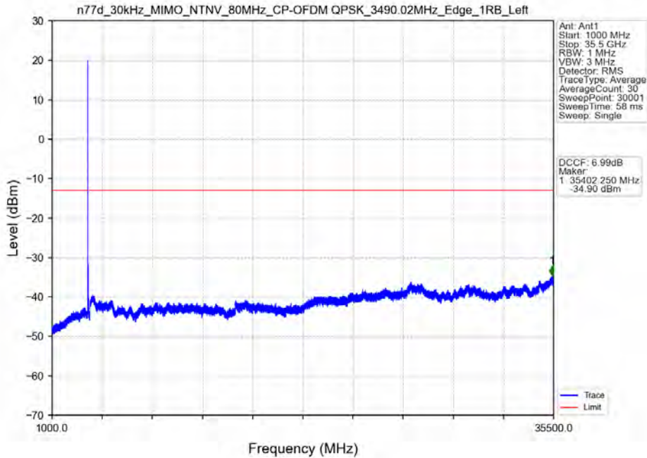
n77d_30kHz_MIMO_NTNV_80MHz_CP-OFDM QPSK_3490.02MHz_Edge_1RB_Left
