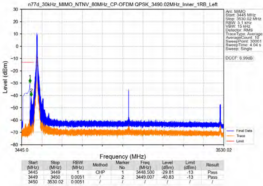
n77d_30kHz_MIMO_NTNV_80MHz_CP-OFDM QPSK_3490.02MHz_Inner_1RB_Left
