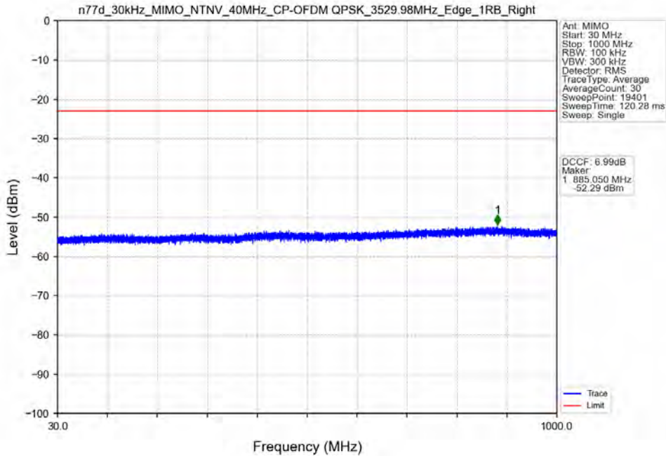
n77d_30kHz_MIMO_NTNV_40MHz_CP-OFDM QPSK_3529.98MHz_Edge_1RB_Right
