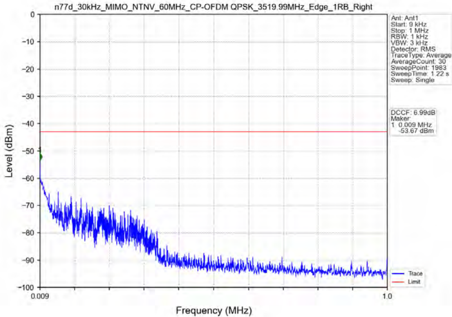
n77d_30kHz_MIMO_NTNV_60MHz_CP-OFDM QPSK_3519.99MHz_Edge_1RB_Right
