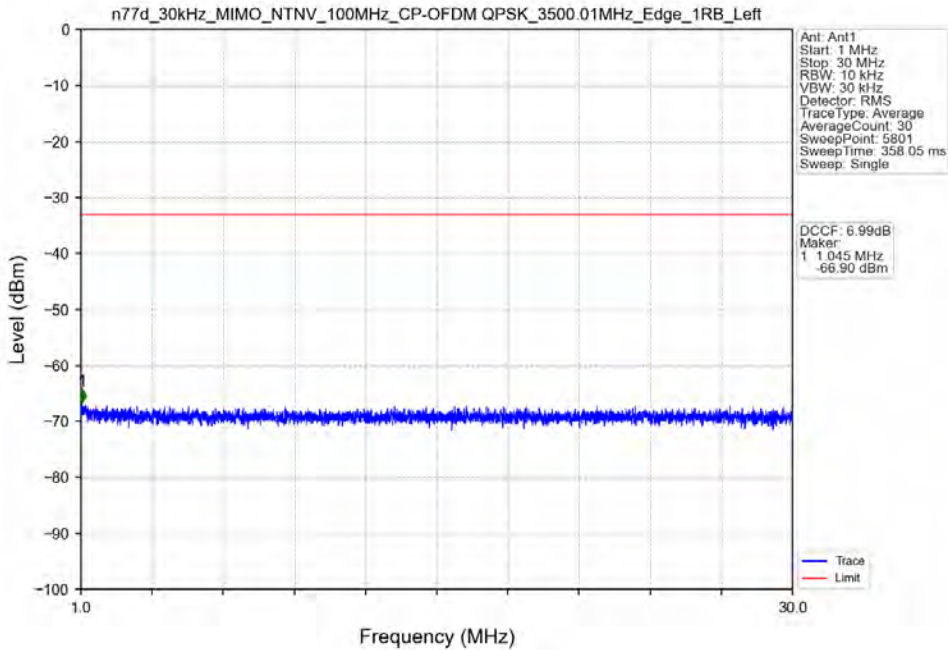
n77d_30kHz_MIMO_NTNV_100MHz_CP-OFDM QPSK_3500.01MHz_Edge_1RB_Left
