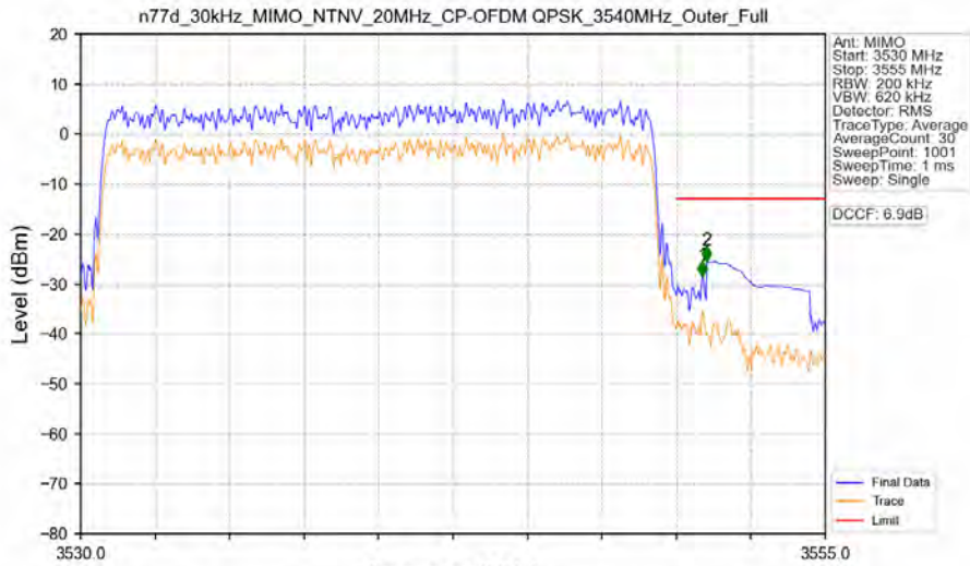
n77d_30kHz_MIMO_NTNV_20MHz_CP-OFDM QPSK_3540MHz_Outer_Full
