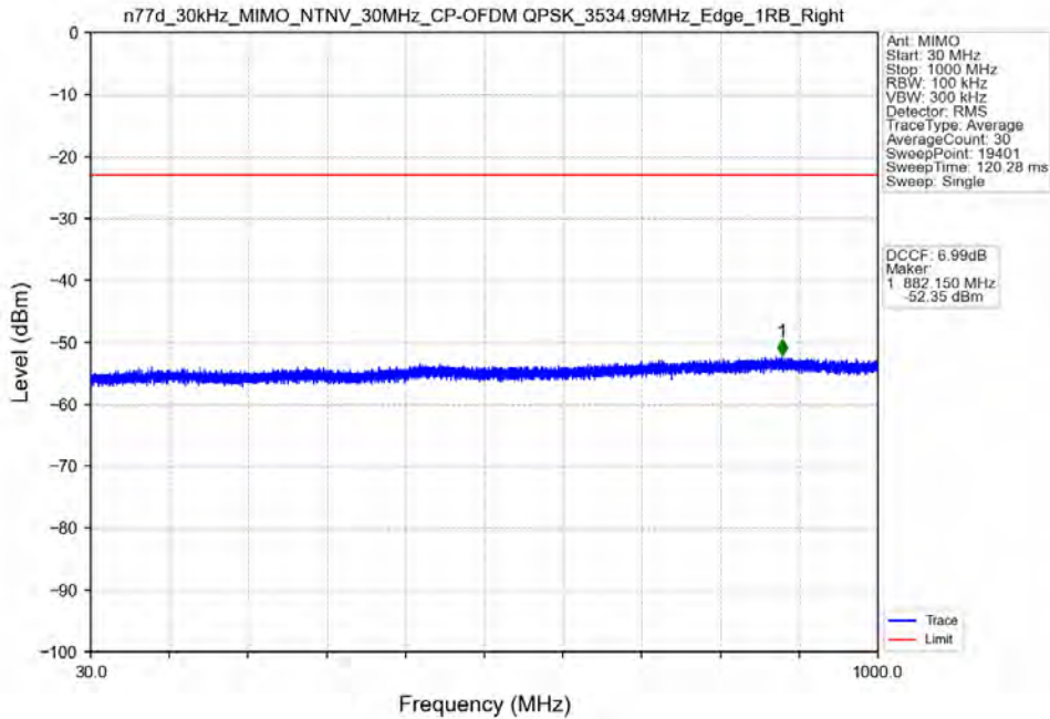
n77d_30kHz_MIMO_NTNV_30MHz_CP-OFDM QPSK_3534.99MHz_Edge_1RB_Right
