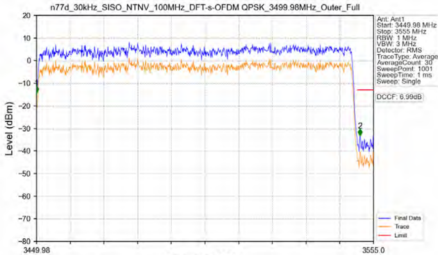
n77d_30kHz_SISO_NTNV_100MHz_DFT-s-OFDM_QPSK_3499.98MHz_Outer_Full
