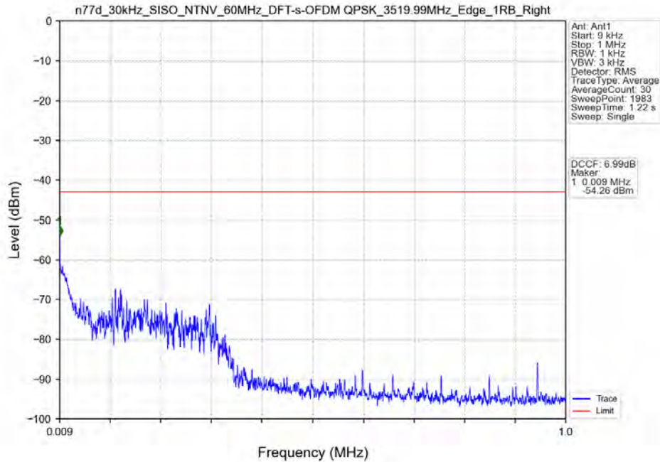
n77d_30kHz_SISO_NTNV_60MHz_DFT-s-OFDM QPSK_3519.99MHz_Edge_1RB_Right
