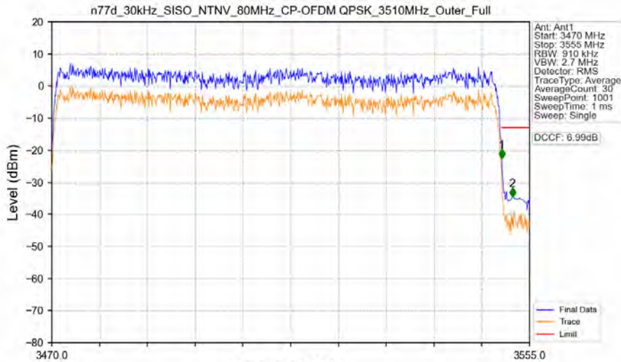
n77d_30kHz_SISO_NTNV_80MHz_CP-OFDM QPSK_3510MHz_Outer_Full
