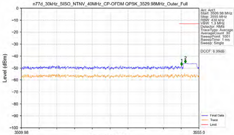
n77d_30kHz_SISO_NTNV_40MHz_CP-OFDM QPSK_3529.98MHz_Outer_Full
