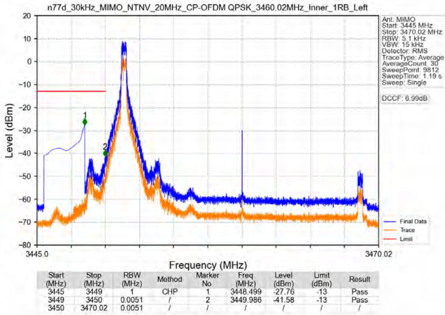
n77d_30kHz_MIMO_NTNV_20MHz_CP-OFDM QPSK_3460.02MHz_Inner_1RB_Left
