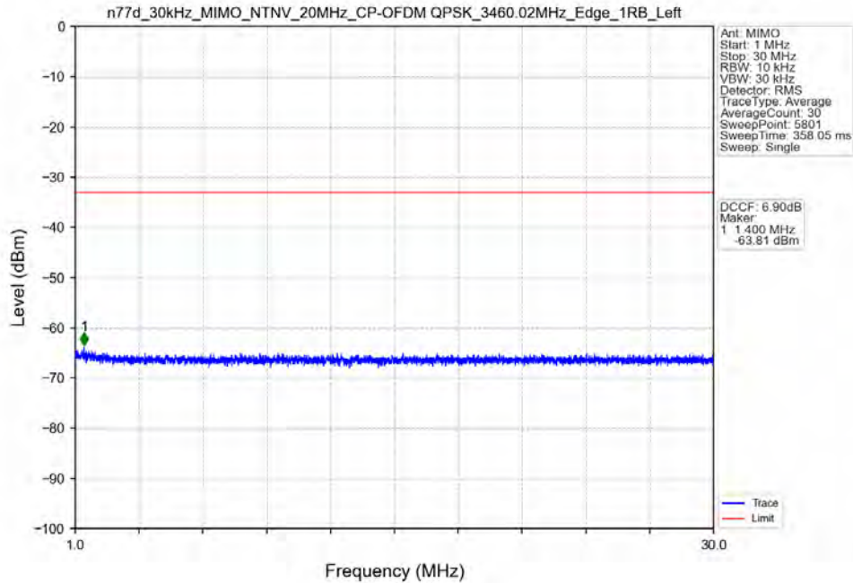
n77d_30kHz_MIMO_NTNV_20MHz_CP-OFDM QPSK_3460.02MHz_Edge_1RB_Left
