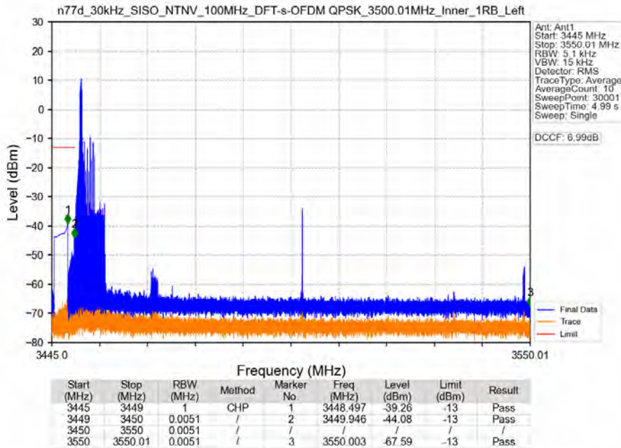
n77d_30kHz_SISO_NTNV_100MHz_DFT-s-OFDM_QPSK_3500.01MHz_Inner_1RB_Left
