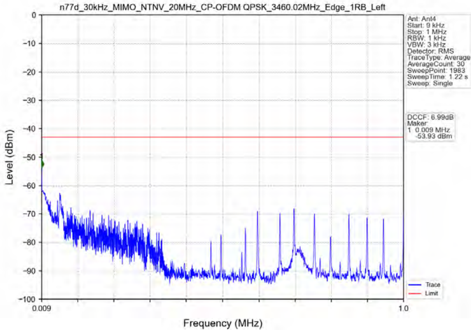
n77d_30kHz_MIMO_NTNV_20MHz_CP-OFDM QPSK_3460.02MHz_Edge_1RB_Left
