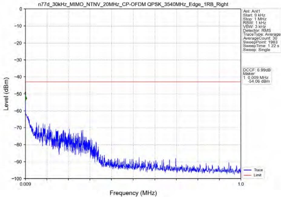
n77d_30kHz_MIMO_NTNV_20MHz_CP-OFDM QPSK_3540MHz_Edge_1RB_Right
