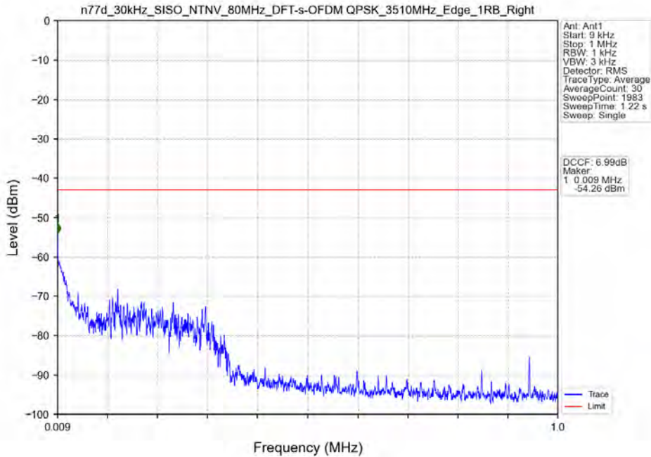
n77d_30kHz_SISO_NTNV_80MHz_DFT-s-OFDM_QPSK_3510MHz_Edge_1RB_Right
