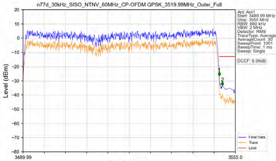
n77d_30kHz_SISO_NTNV_60MHz_CP-OFDM QPSK_3519.99MHz_Outer_Full
