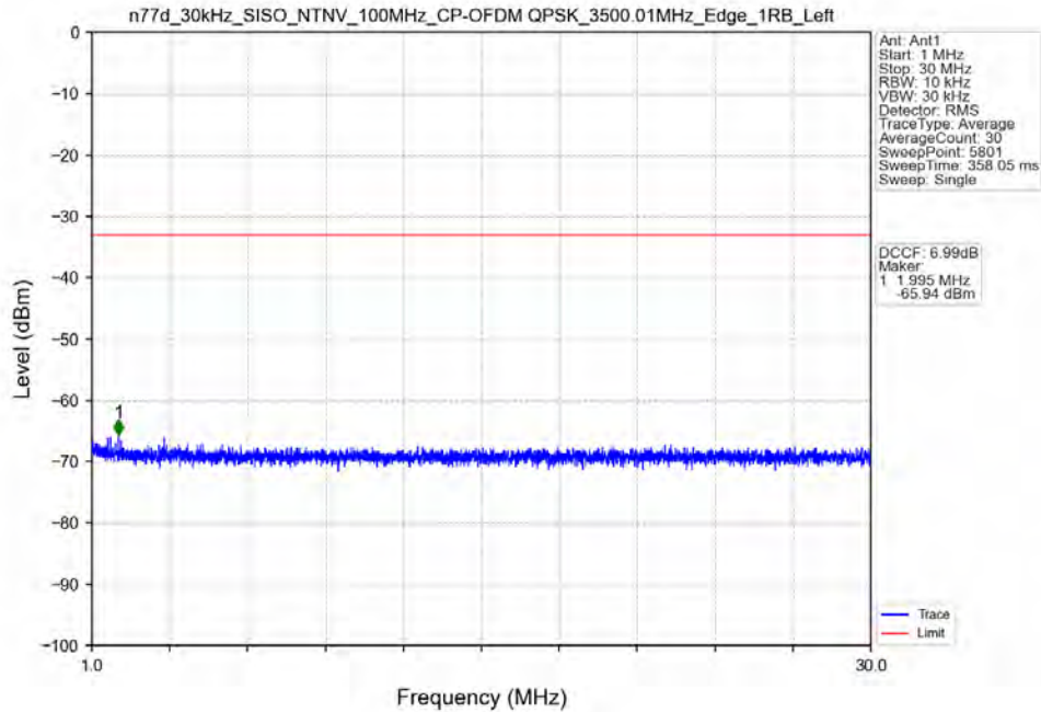
n77d_30kHz_SISO_NTNV_100MHz_CP-OFDM QPSK_3500.01MHz_Edge_1RB_Left
