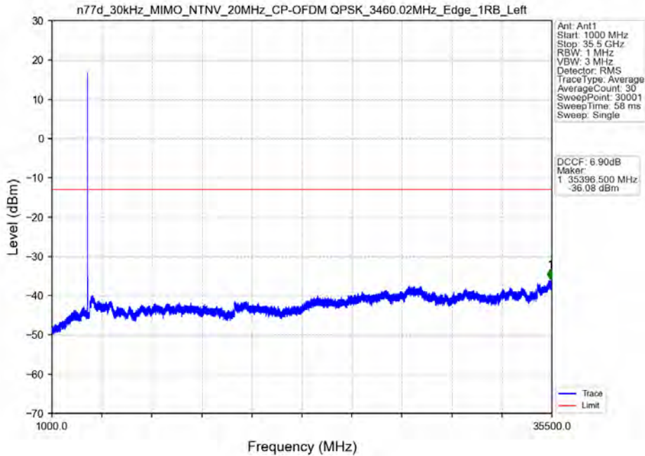
n77d_30kHz_MIMO_NTNV_20MHz_CP-OFDM QPSK_3460.02MHz_Edge_1RB_Left
