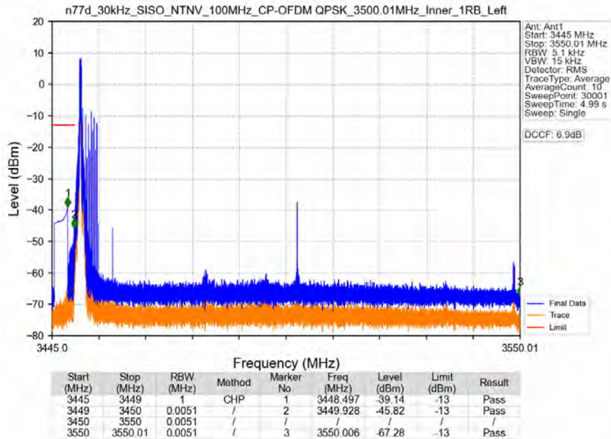
n77d_30kHz_SISO_NTNV_100MHz_CP-OFDM QPSK_3500.01MHz_Inner_1RB_Left
