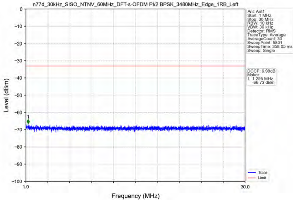
n77d_30kHz_SISO_NTNV_60MHz_DFT-s-OFDM PI/2 BPSK_3480MHz_Edge_1RB_Left
