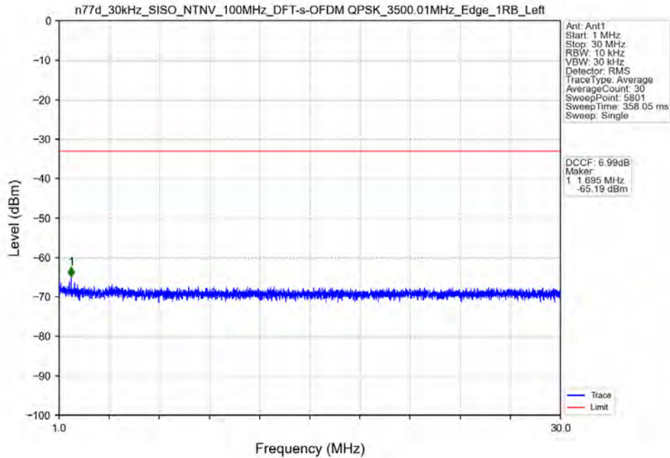
n77d_30kHz_SISO_NTNV_100MHz_DFT-s-OFDM_QPSK_3500.01MHz_Edge_1RB_Left
