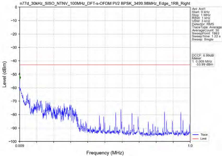
n77d_30kHz_SISO_NTNV_100MHz_DFT-s-OFDM PI/2 BPSK_3499.98MHz_Edge_1RB_Right
