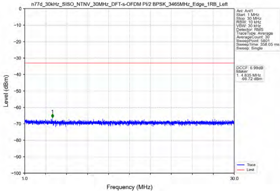
n77d_30kHz_SISO_NTNV_30MHz_DFT-s-OFDM PI/2 BPSK_3465MHz_Edge_1RB_Left
