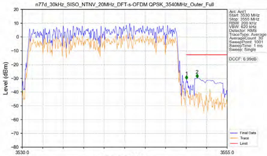
n77d_30kHz_SISO_NTNV_20MHz_DFT-s-OFDM QPSK_3540MHz_Outer_Full
