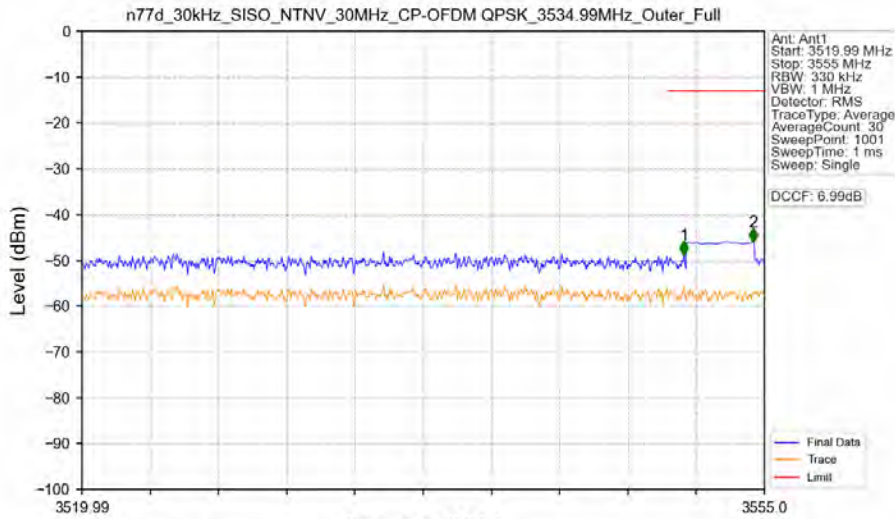
n77d_30kHz_SISO_NTNV_30MHz_CP-OFDM QPSK_3534.99MHz_Outer_Full
