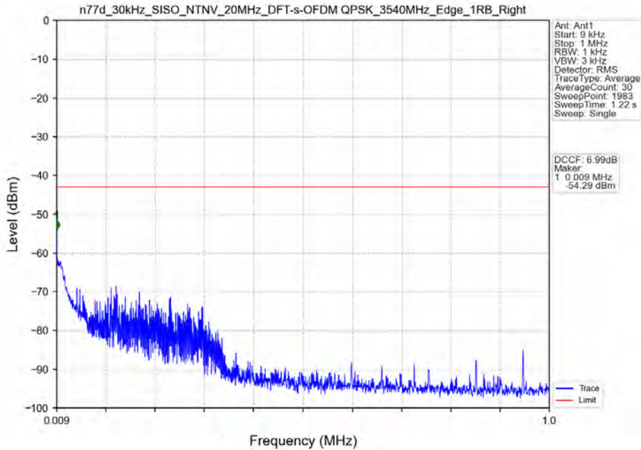
n77d_30kHz_SISO_NTNV_20MHz_DFT-s-OFDM_QPSK_3540MHz_Edge_1RB_Right
