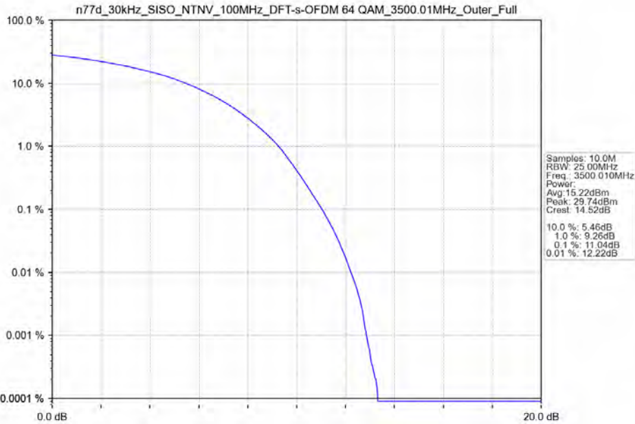
n77d_30kHz_SISO_NTNV_100MHz_DFT-s-OFDM 64 QAM_3500.01MHz_Outer_Full
