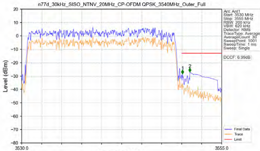
n77d_30kHz_SISO_NTNV_20MHz_CP-OFDM QPSK_3540MHz_Outer_Full
