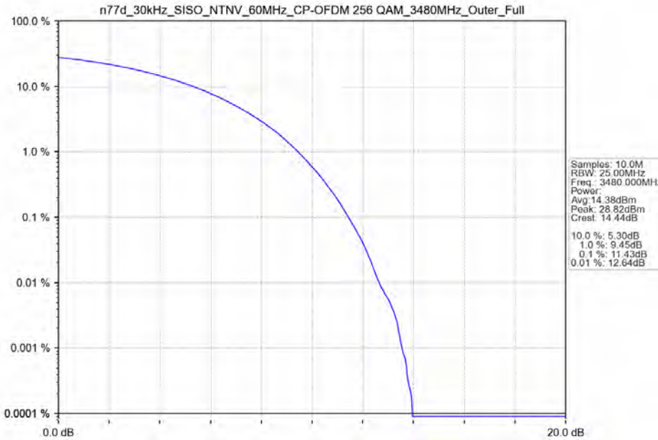
n77d_30kHz_SISO_NTNV_60MHz_CP-OFDM 256 QAM_3480MHz_Outer_Full
