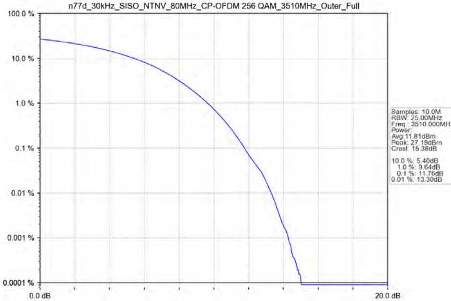
n77d_30kHz_SISO_NTNV_80MHz_CP-OFDM 256 QAM_3510MHz_Outer_Full
