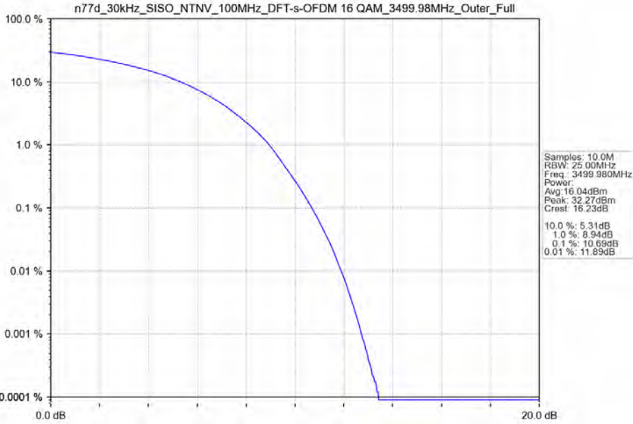
n77d_30kHz_SISO_NTNV_100MHz_DFT-s-OFDM 16 QAM_3499.98MHz_Outer_Full
