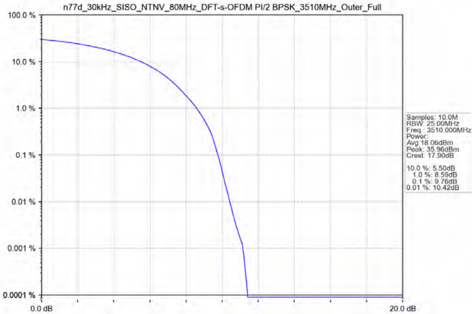
n77d_30kHz_SISO_NTNV_80MHz_DFT-s-OFDM PI/2 BPSK_3510MHz_Outer_Full
