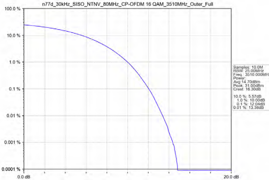
n77d_30kHz_SISO_NTNV_80MHz_CP-OFDM 16 QAM_3510MHz_Outer_Full
