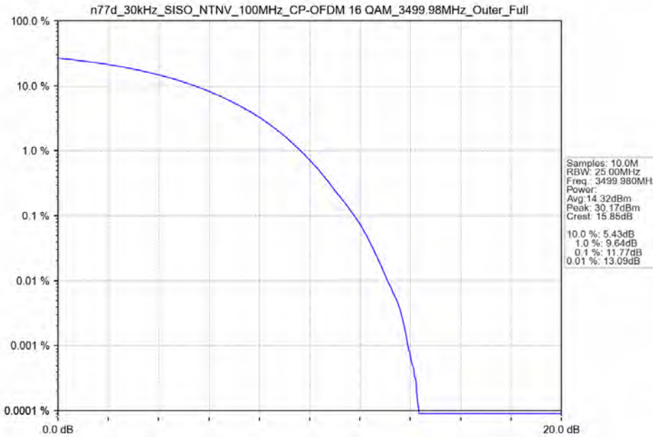
n77d_30kHz_SISO_NTNV_100MHz_CP-OFDM 16 QAM_3499.98MHz_Outer_Full
