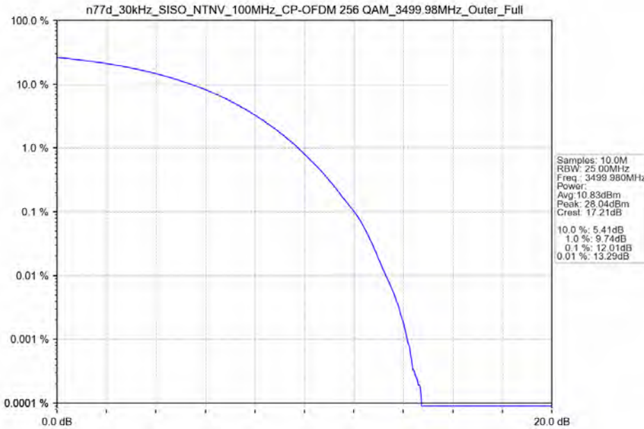
n77d_30kHz_SISO_NTNV_100MHz_CP-OFDM 256 QAM_3499.98MHz_Outer_Full
