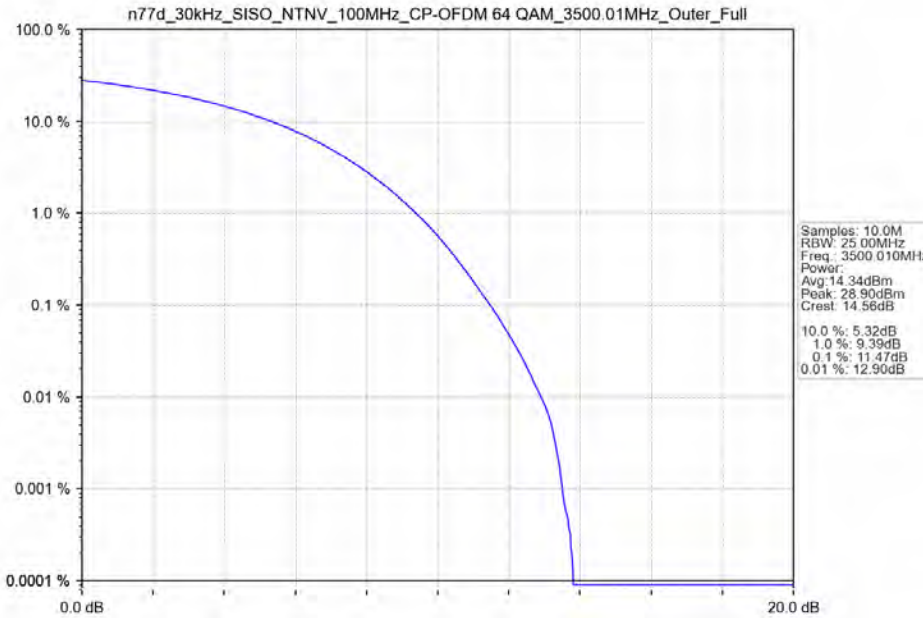
n77d_30kHz_SISO_NTNV_100MHz_CP-OFDM 64 QAM_3500.01MHz_Outer_Full
