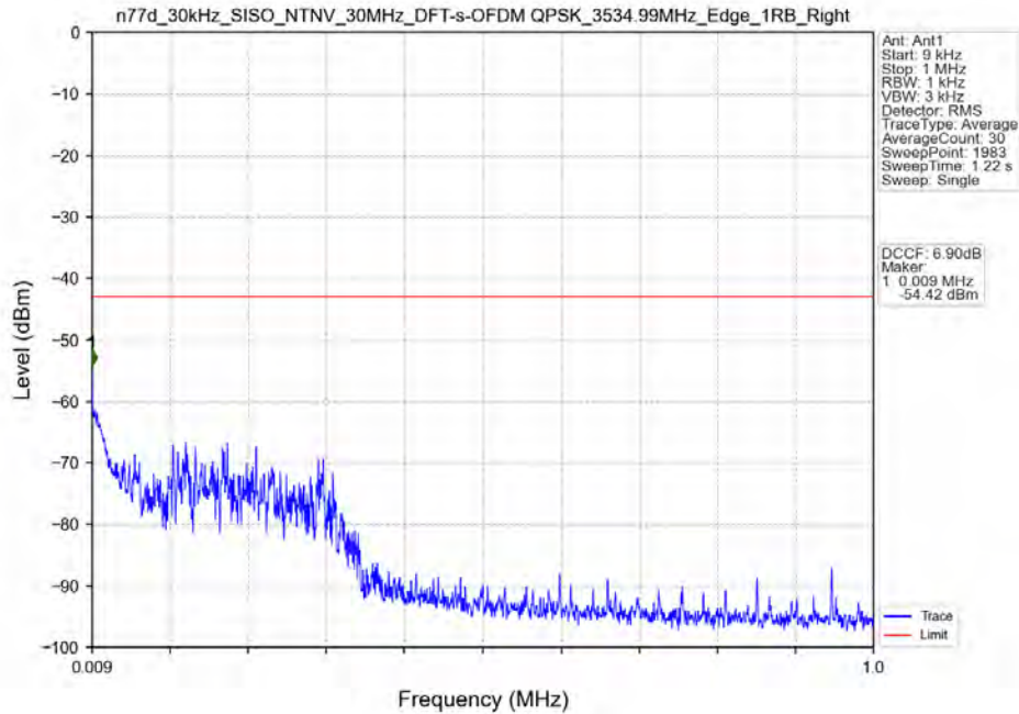
n77d_30kHz_SISO_NTNV_30MHz_DFT-s-OFDM QPSK_3534.99MHz_Edge_1RB_Right
