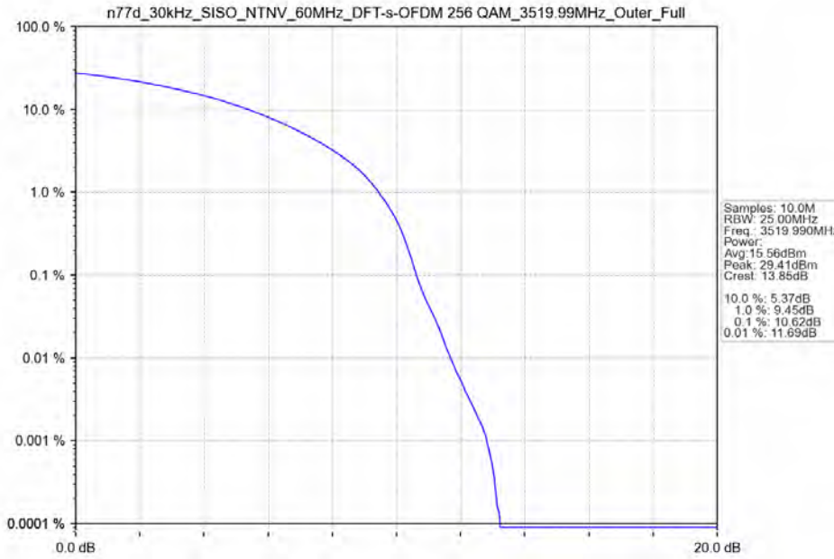
n77d_30kHz_SISO_NTNV_60MHz_DFT-s-OFDM 256 QAM_3519.99MHz_Outer_Full
