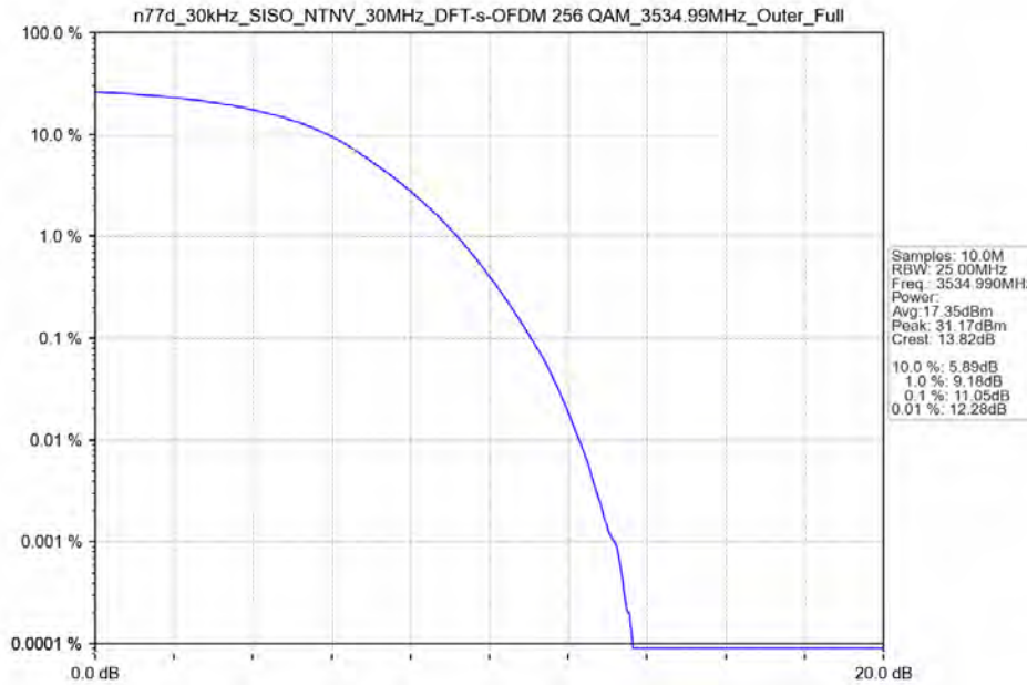
n77d_30kHz_SISO_NTNV_30MHz_DFT-s-OFDM 256 QAM_3534.99MHz_Outer_Full
