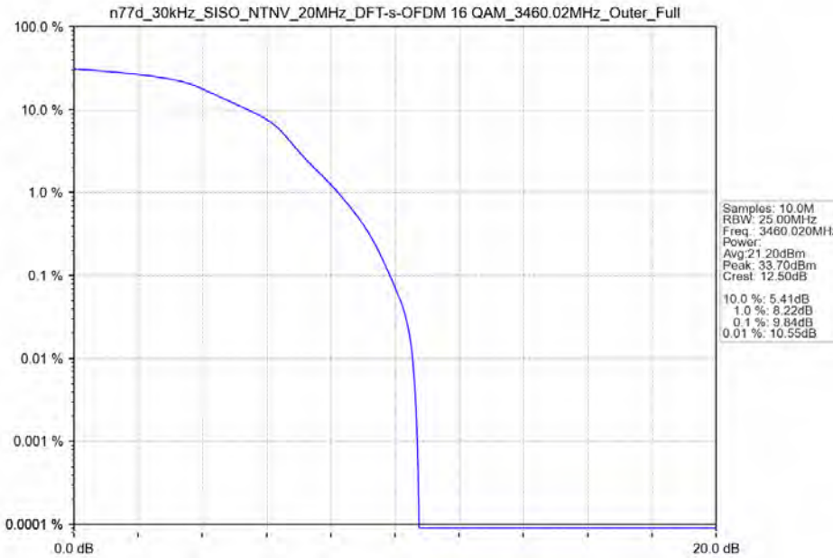
n77d_30kHz_SISO_NTNV_20MHz_DFT-s-OFDM 16 QAM_3460.02MHz_Outer_Full
