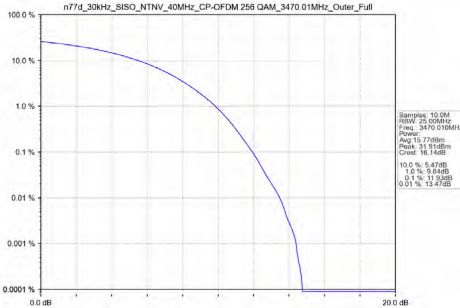
n77d_30kHz_SISO_NTNV_40MHz_CP-OFDM 256 QAM_3470.01MHz_Outer_Full
