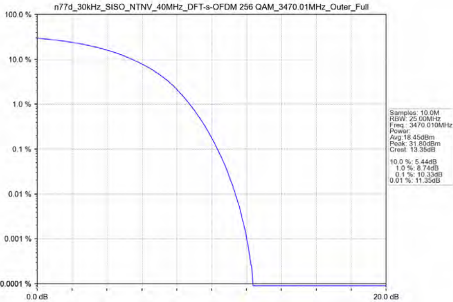
n77d_30kHz_SISO_NTNV_40MHz_DFT-s-OFDM_256_QAM_3470.01MHz_Outer_Full
