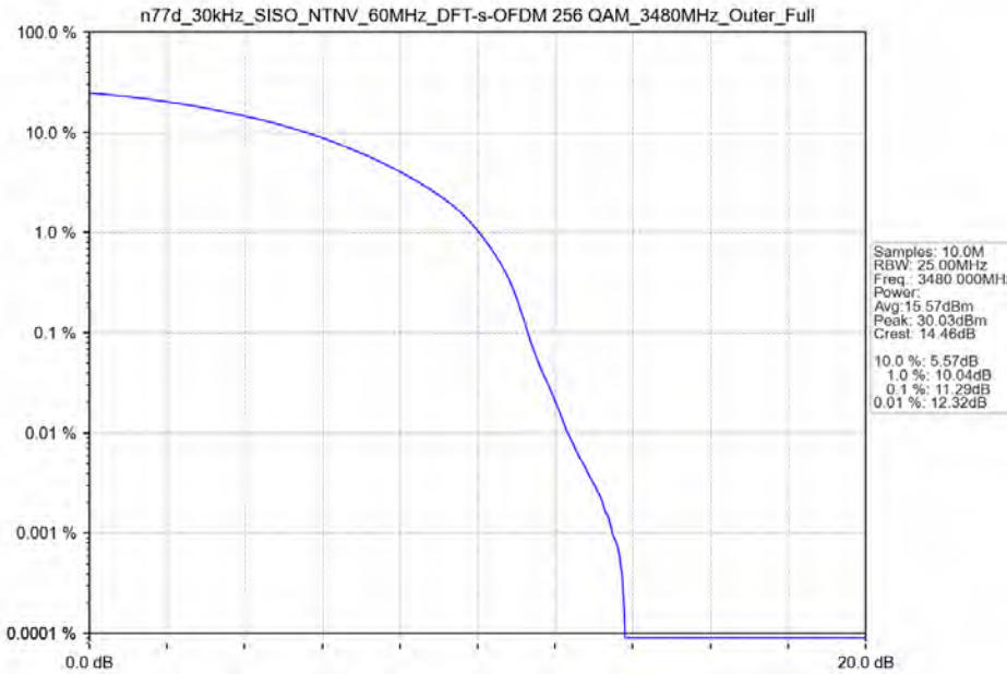
n77d_30kHz_SISO_NTNV_60MHz_DFT-s-OFDM 256 QAM_3480MHz_Outer_Full
