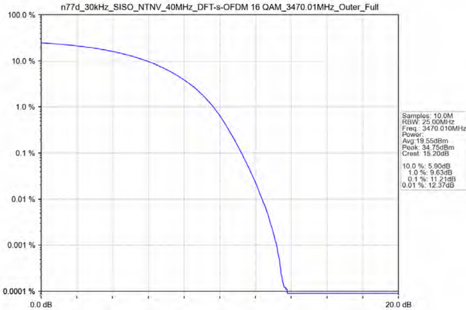
n77d_30kHz_SISO_NTNV_40MHz_DFT-s-OFDM 16 QAM_3470.01MHz_Outer_Full
