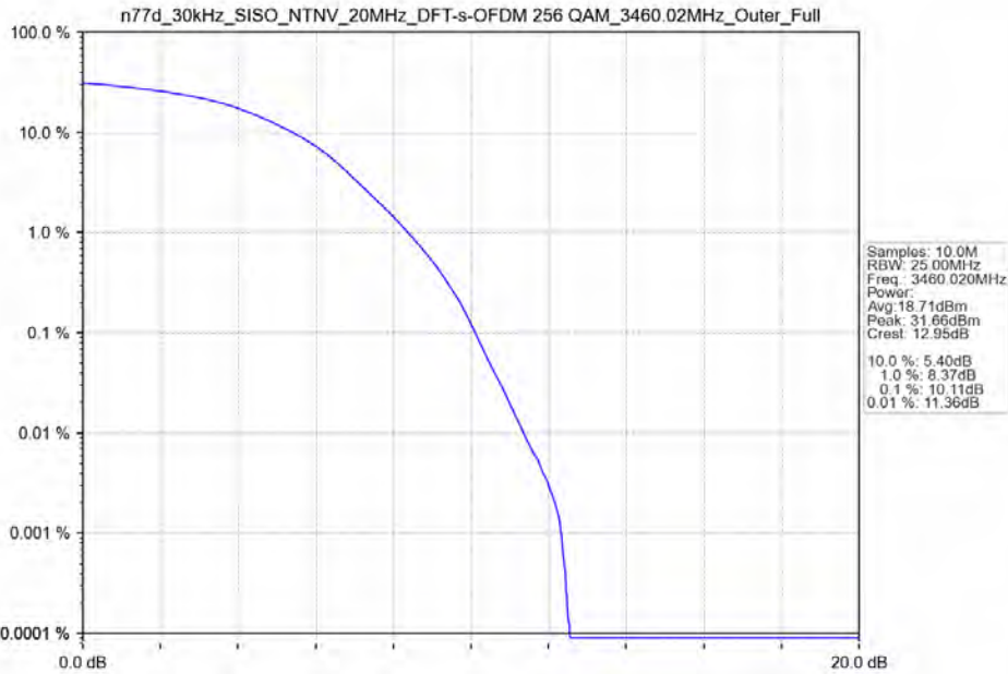
n77d_30kHz_SISO_NTNV_20MHz_DFT-s-OFDM_256_QAM_3460.02MHz_Outer_Full
