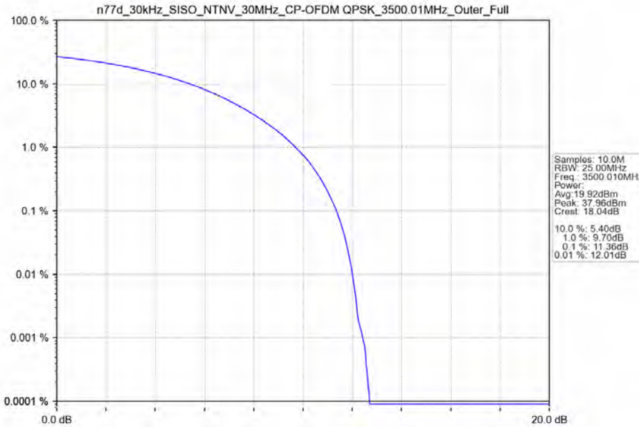
n77d_30kHz_SISO_NTNV_30MHz_CP-OFDM QPSK_3500.01MHz_Outer_Full
