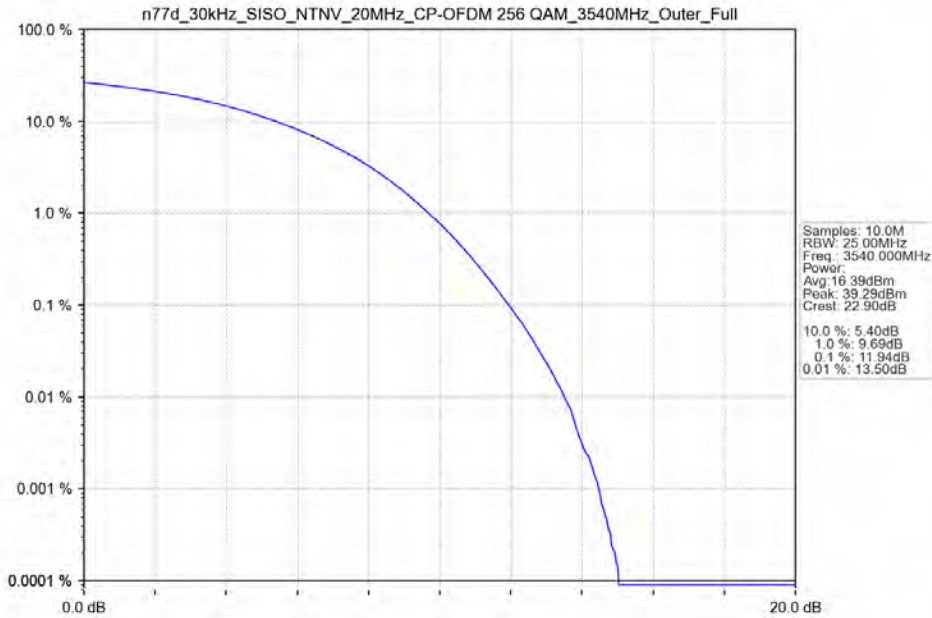
n77d_30kHz_SISO_NTNV_20MHz_CP-OFDM 256 QAM_3540MHz_Outer_Full
