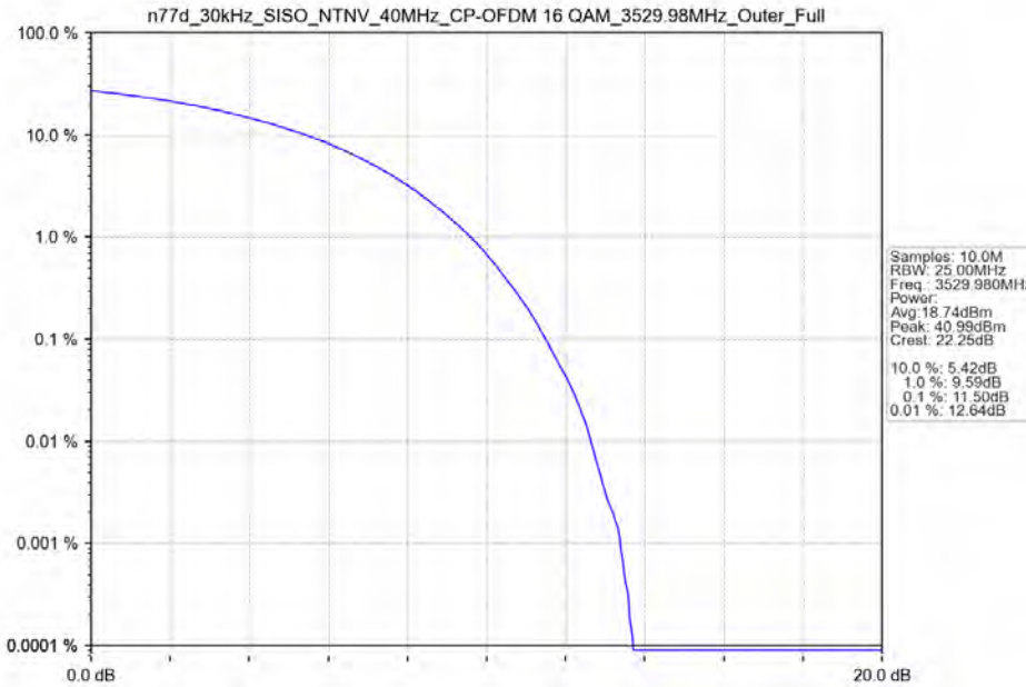
n77d_30kHz_SISO_NTNV_40MHz_CP-OFDM 16 QAM_3529.98MHz_Outer_Full
