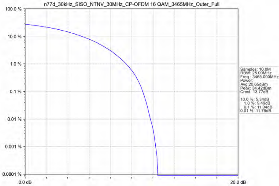
n77d_30kHz_SISO_NTNV_30MHz_CP-OFDM 16 QAM_3465MHz_Outer_Full
