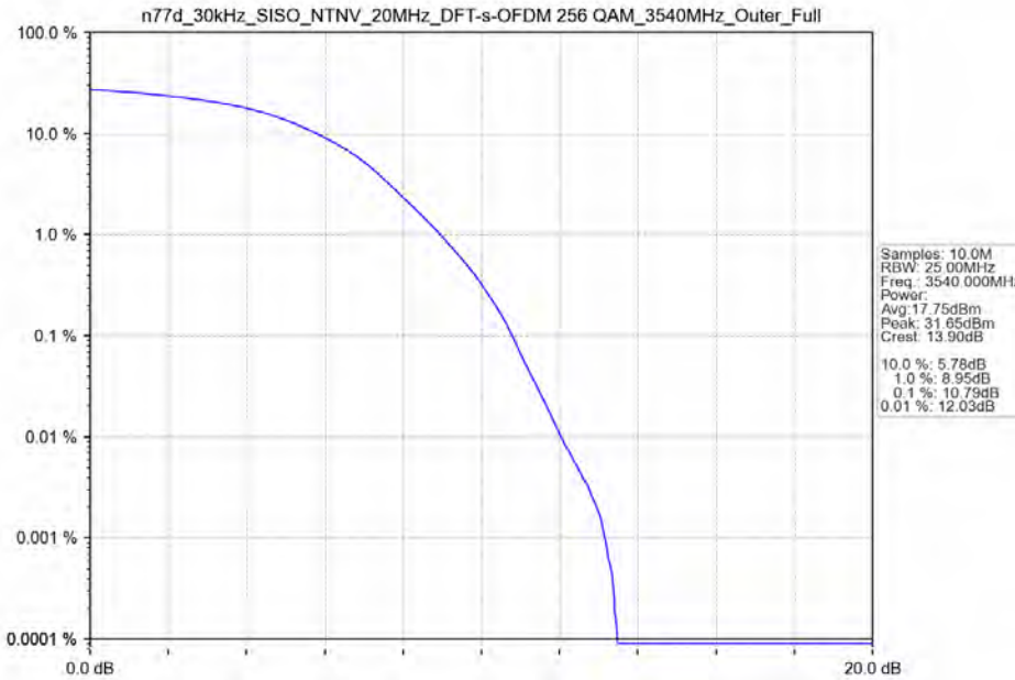
n77d_30kHz_SISO_NTNV_20MHz_DFT-s-OFDM 256 QAM_3540MHz_Outer_Full
