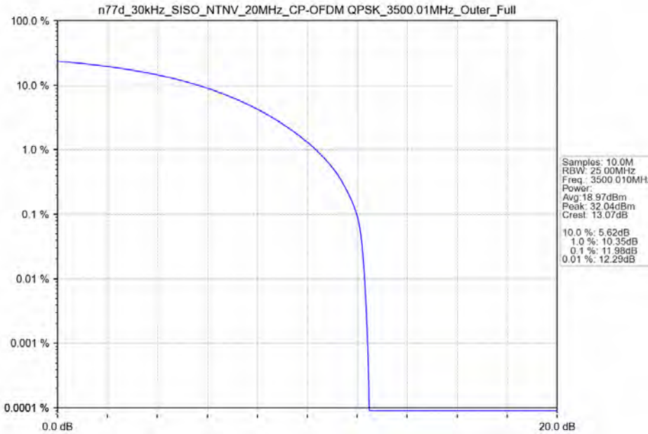
n77d_30kHz_SISO_NTNV_20MHz_CP-OFDM QPSK_3500.01MHz_Outer_Full
