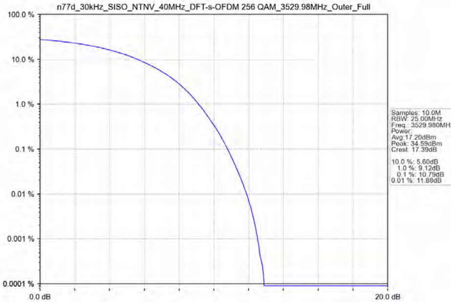
n77d_30kHz_SISO_NTNV_40MHz_DFT-s-OFDM 256 QAM_3529.98MHz_Outer_Full
