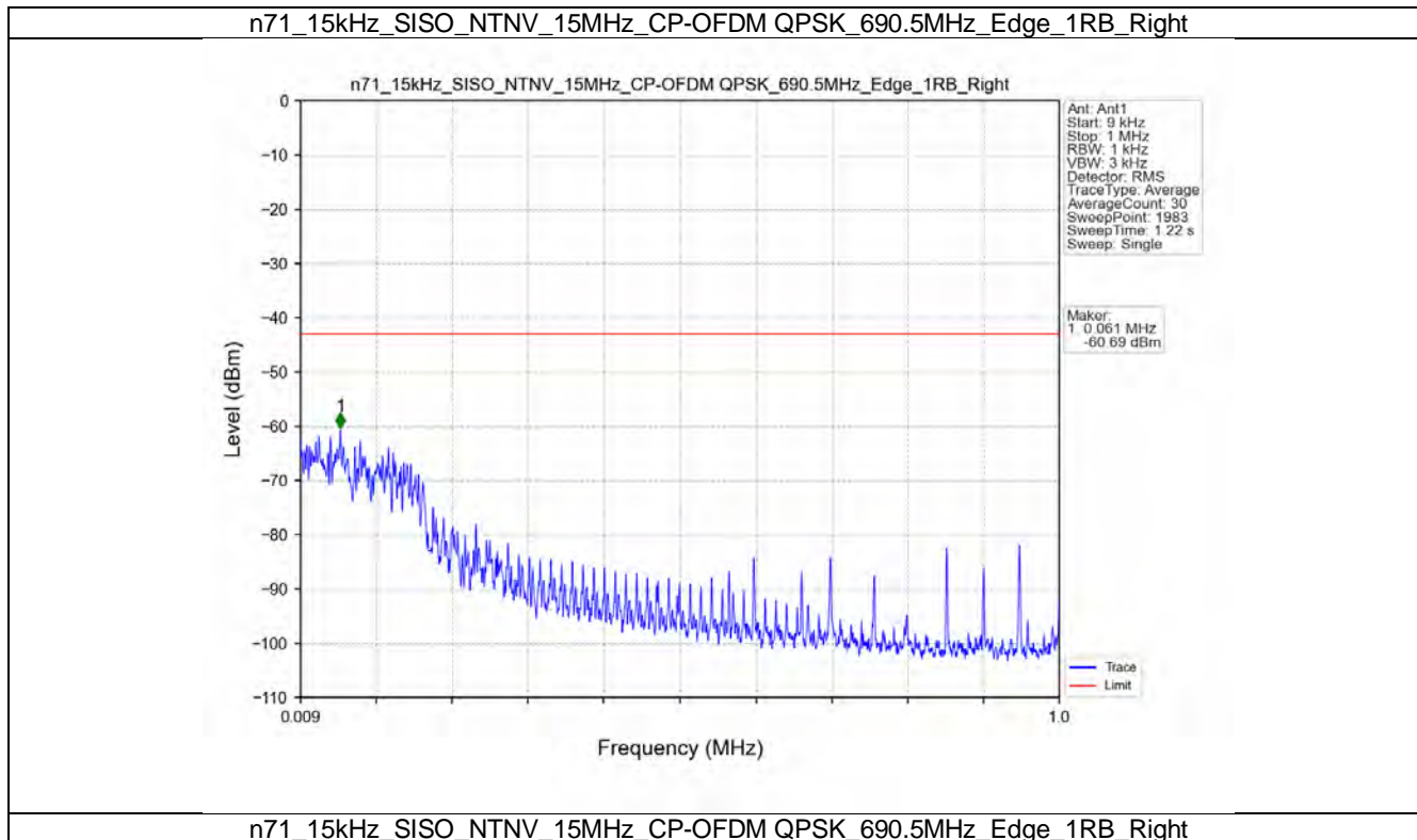
n71_15kHz_SISO_NTNV_15MHz_CP-OFDM QPSK_690.5MHz_Edge_1RB_Right
