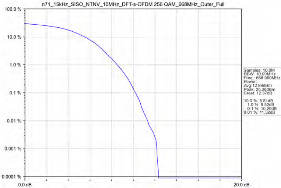
n71_15kHz_SISO_NTNV_10MHz_DFT-s-OFDM 256 QAM_668MHz_Outer_Full
