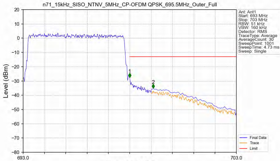
n71_15kHz_SISO_NTNV_5MHz_CP-OFDM QPSK_695.5MHz_Outer_Full
