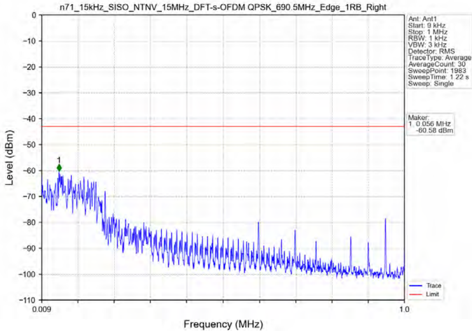
n71_15kHz_SISO_NTNV_15MHz_DFT-s-OFDM QPSK_690.5MHz_Edge_1RB_Right
