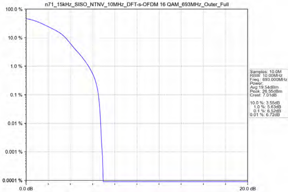
n71_15kHz_SISO_NTNV_10MHz_DFT-s-OFDM 16 QAM_693MHz_Outer_Full
