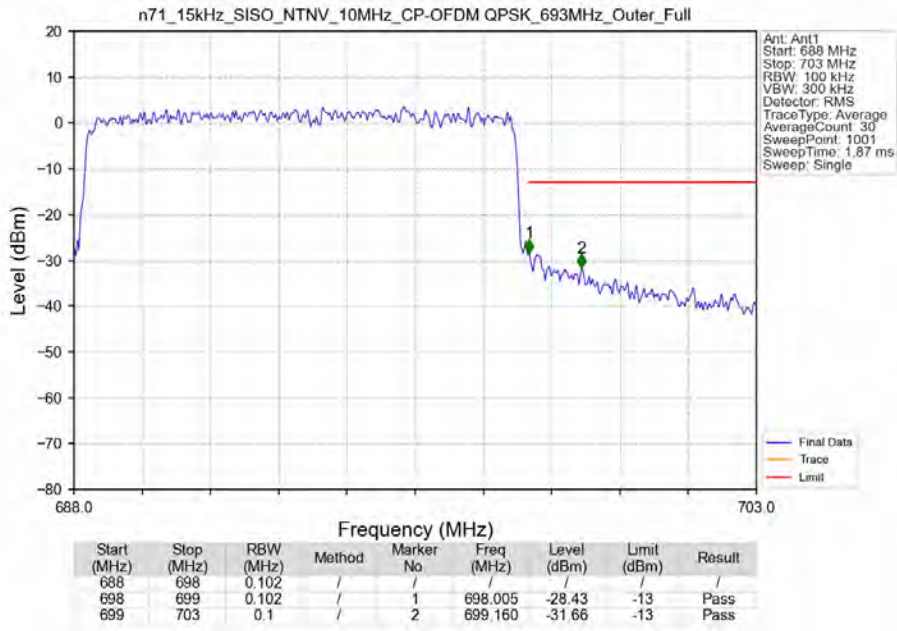
n71_15kHz_SISO_NTNV_10MHz_CP-OFDM QPSK_693MHz_Outer_Full
