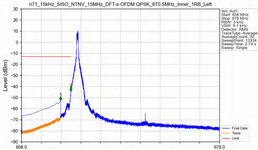
n71_15kHz_SISO_NTNV_15MHz_DFT-s-OFDM_QPSK_670.5MHz_Inner_1RB_Left
