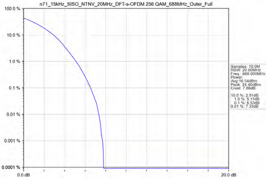
n71_15kHz_SISO_NTNV_20MHz_DFT-s-OFDM 256 QAM_688MHz_Outer_Full
