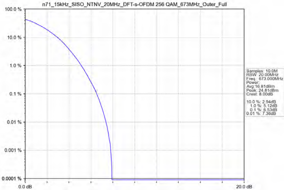
n71_15kHz_SISO_NTNV_20MHz_DFT-s-OFDM 256 QAM_673MHz_Outer_Full
