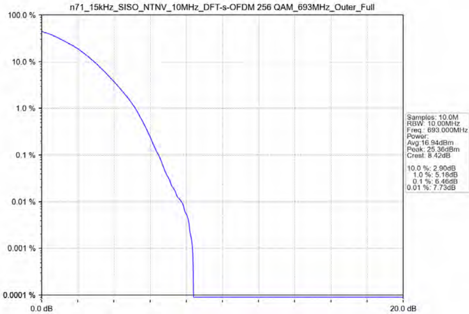
n71_15kHz_SISO_NTNV_10MHz_DFT-s-OFDM 256 QAM_693MHz_Outer_Full
