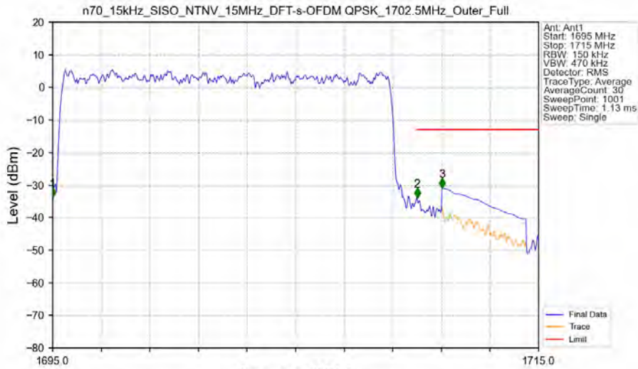
n70_15kHz_SISO_NTNV_15MHz_DFT-s-OFDM QPSK_1702.5MHz_Outer_Full
