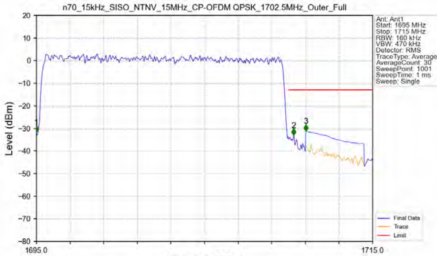
n70_15kHz_SISO_NTNV_15MHz_CP-OFDM QPSK_1702.5MHz_Outer_Full
