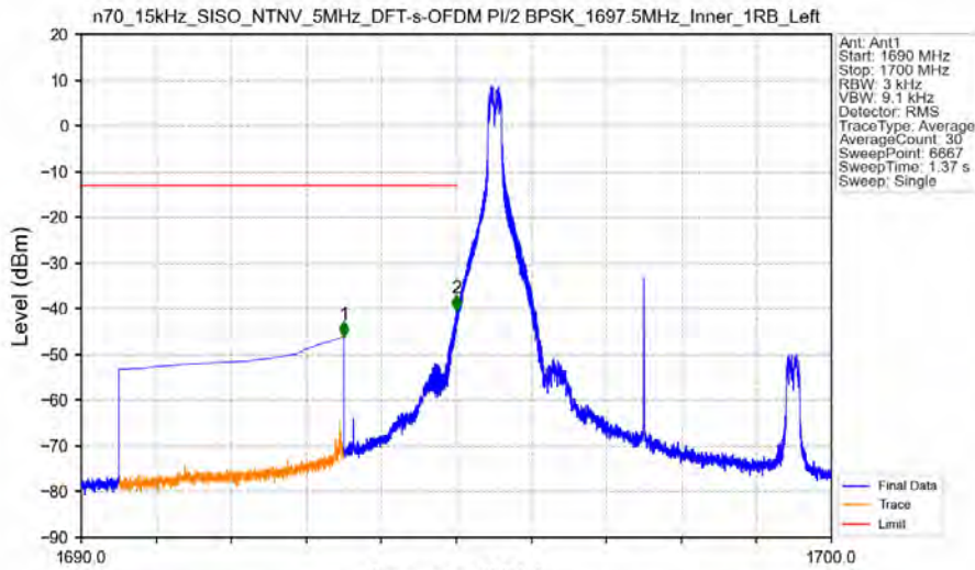
n70_15kHz_SISO_NTNV_5MHz_DFT-s-OFDM PI/2 BPSK_1697.5MHz_Inner_1RB_Left
