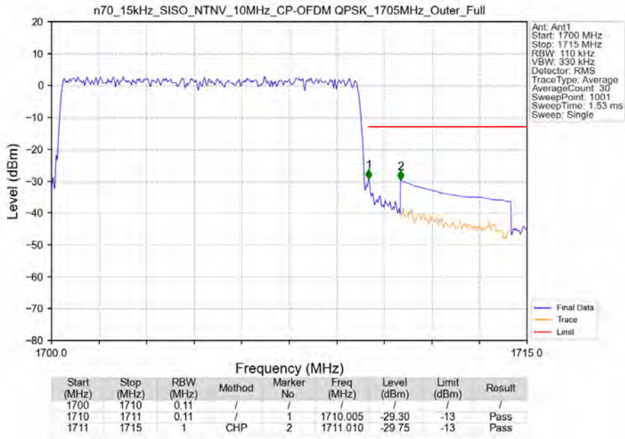
n70_15kHz_SISO_NTNV_10MHz_CP-OFDM QPSK_1705MHz_Outer_Full
