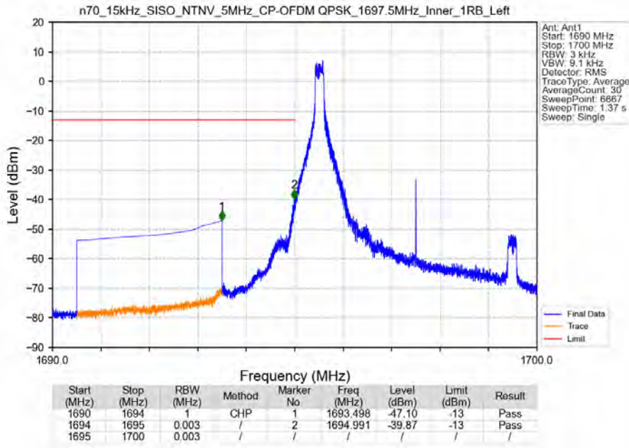
n70_15kHz_SISO_NTNV_5MHz_CP-OFDM QPSK_1697.5MHz_Inner_1RB_Left
