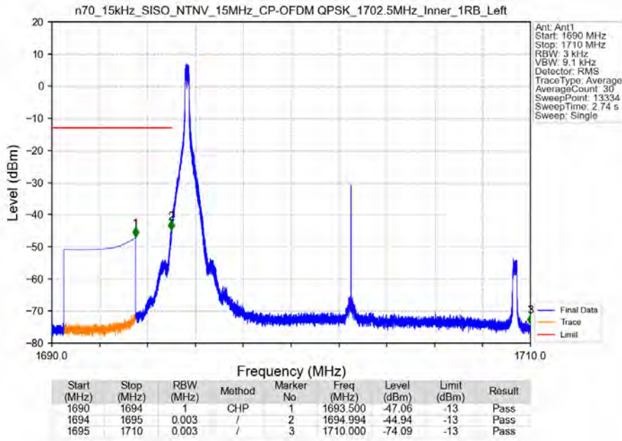
n70_15kHz_SISO_NTNV_15MHz_CP-OFDM QPSK_1702.5MHz_Inner_1RB_Left
