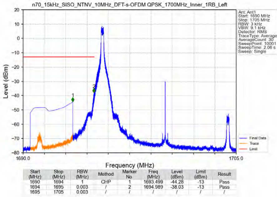
n70_15kHz_SISO_NTNV_10MHz_DFT-s-OFDM QPSK_1700MHz_Inner_1RB_Left
