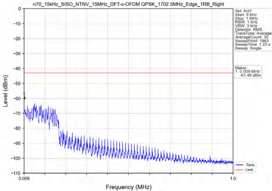
n70_15kHz_SISO_NTNV_15MHz_DFT-s-OFDM QPSK_1702.5MHz_Edge_1RB_Right
