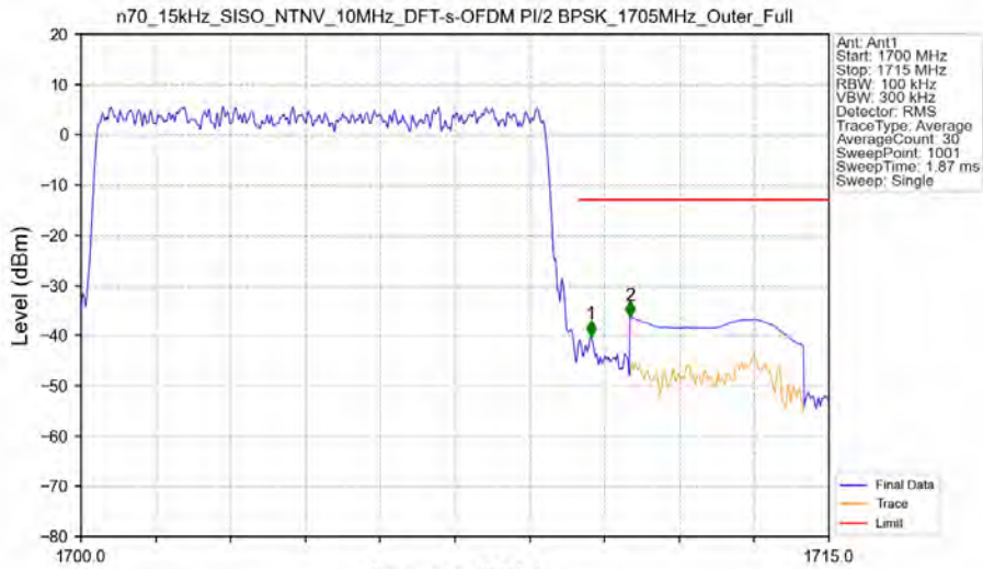
n70_15kHz_SISO_NTNV_10MHz_DFT-s-OFDM PI/2 BPSK_1705MHz_Outer_Full
