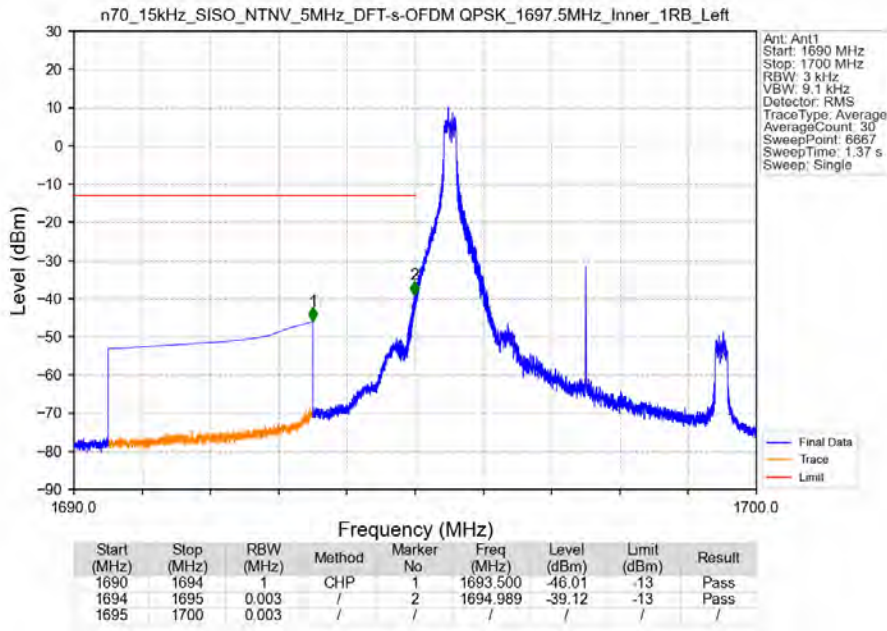
n70_15kHz_SISO_NTNV_5MHz_DFT-s-OFDM QPSK_1697.5MHz_Inner_1RB_Left
