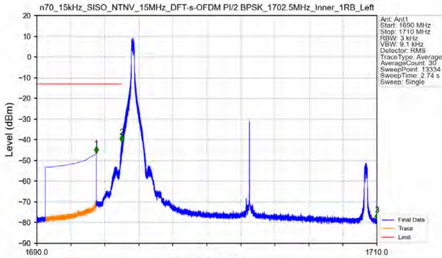
n70_15kHz_SISO_NTNV_15MHz_DFT-s-OFDM PI/2 BPSK_1702.5MHz_Inner_1RB_Left
