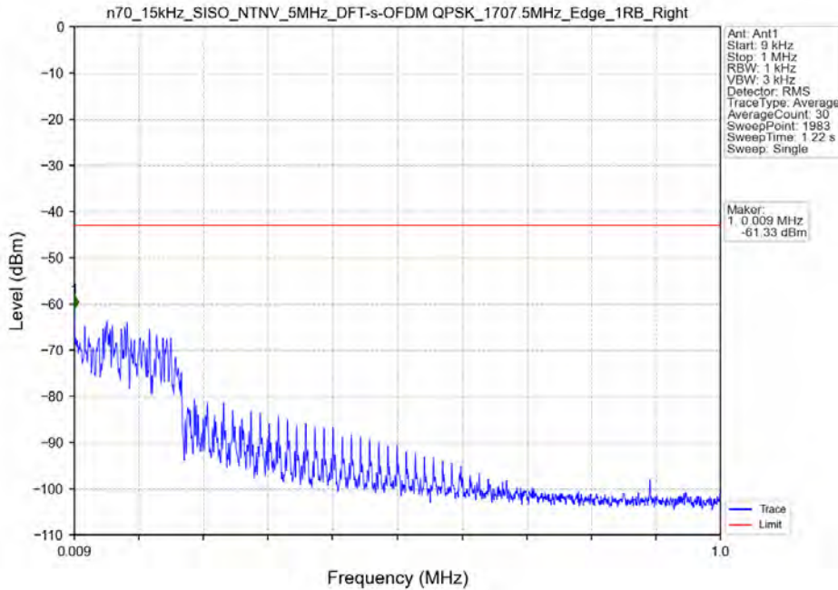
n70_15kHz_SISO_NTNV_5MHz_DFT-s-OFDM QPSK_1707.5MHz_Edge_1RB_Right
