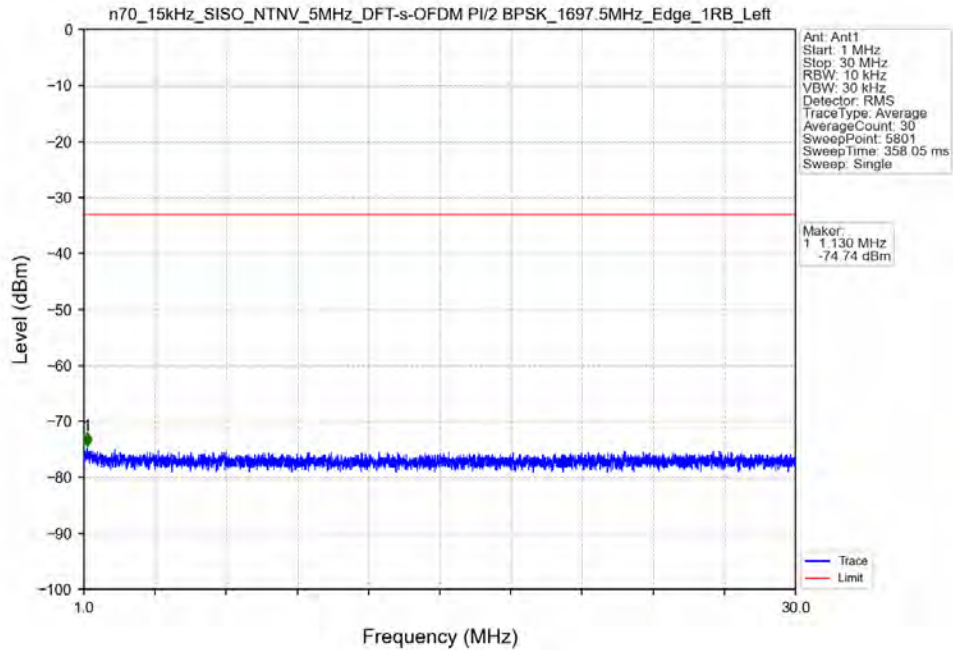
n70_15kHz_SISO_NTNV_5MHz_DFT-s-OFDM PI/2 BPSK_1697.5MHz_Edge_1RB_Left
