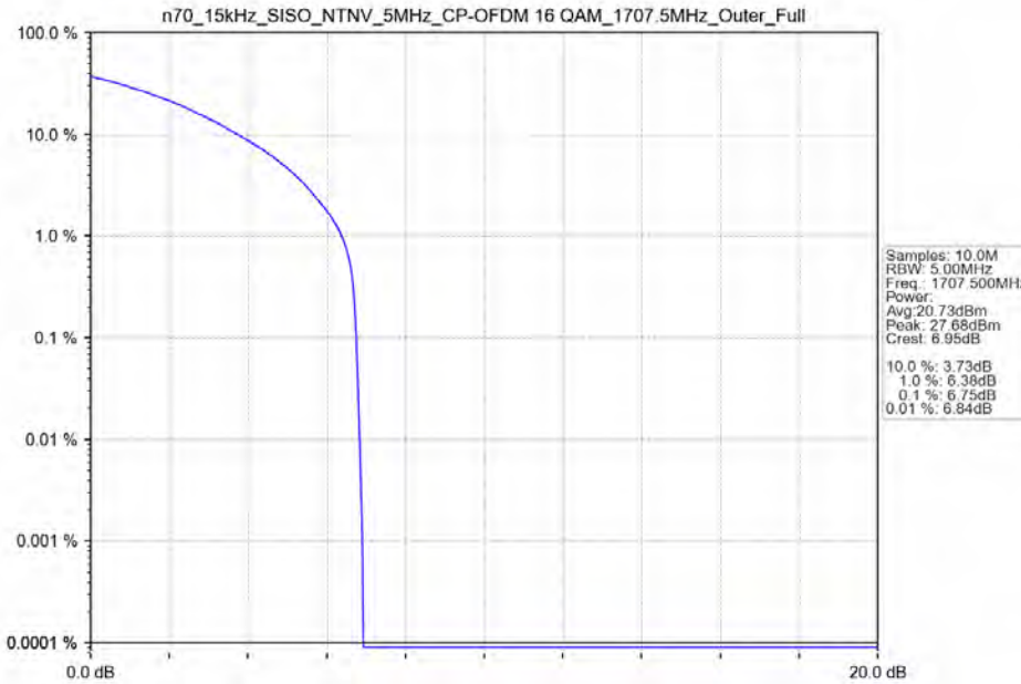
n70_15kHz_SISO_NTNV_5MHz_CP-OFDM 16 QAM_1707.5MHz_Outer_Full
