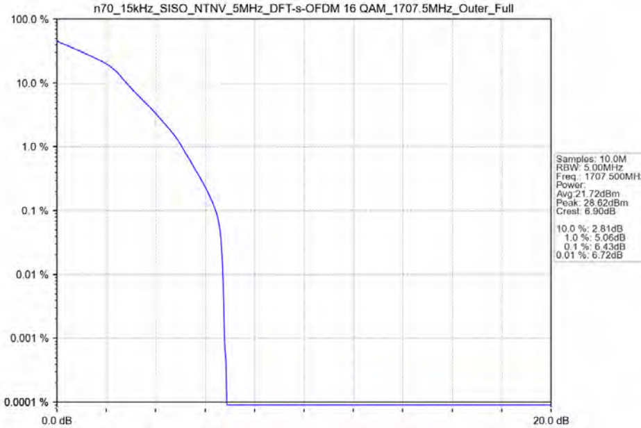
n70_15kHz_SISO_NTNV_5MHz_DFT-s-OFDM 16 QAM_1707.5MHz_Outer_Full
