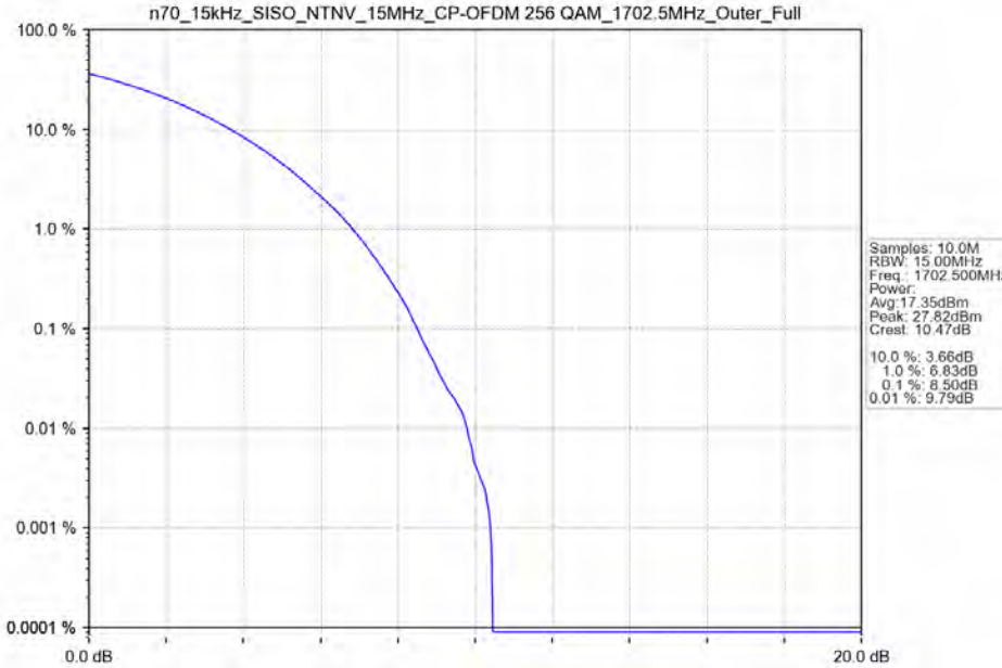
n70_15kHz_SISO_NTNV_15MHz_CP-OFDM 256 QAM_1702.5MHz_Outer_Full
