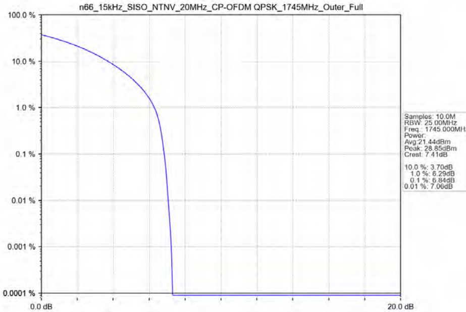
n66_15kHz_SISO_NTNV_20MHz_CP-OFDM QPSK_1745MHz_Outer_Full
