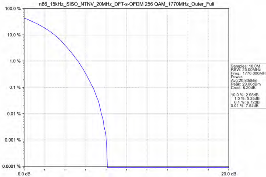
n66_15kHz_SISO_NTNV_20MHz_DFT-s-OFDM 256 QAM_1770MHz_Outer_Full
