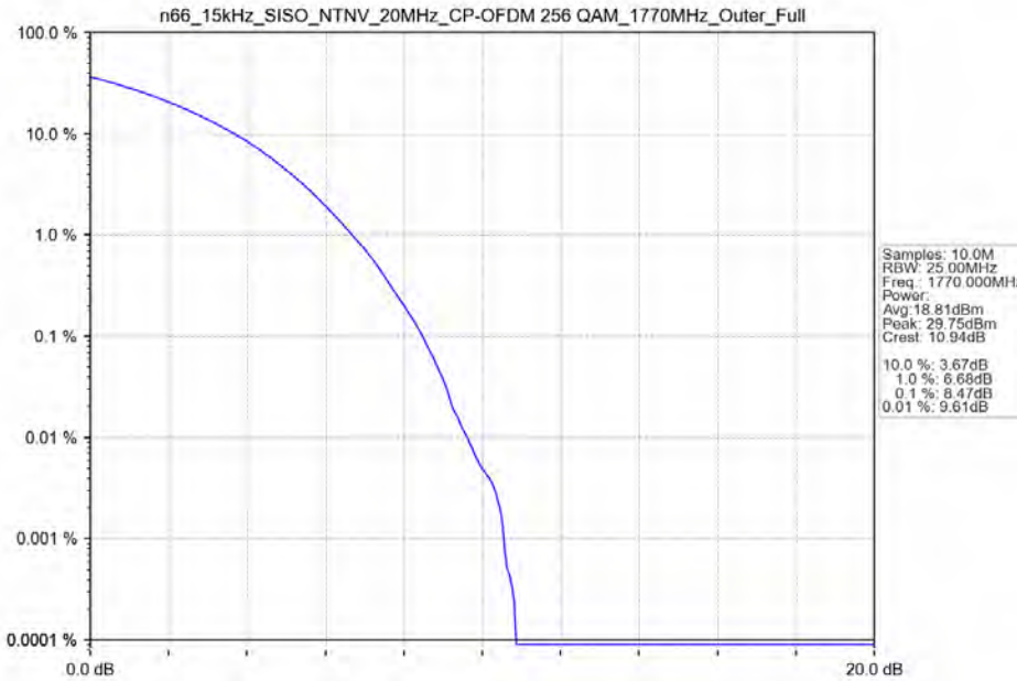
n66_15kHz_SISO_NTNV_20MHz_CP-OFDM 256 QAM_1770MHz_Outer_Full
