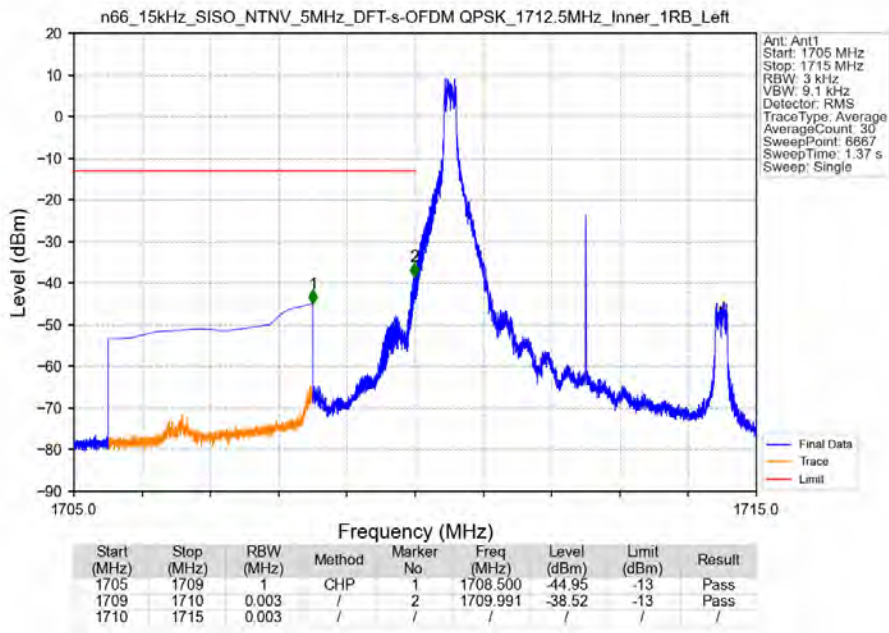
n66_15kHz_SISO_NTNV_5MHz_DFT-s-OFDM QPSK_1712.5MHz_Inner_1RB_Left
