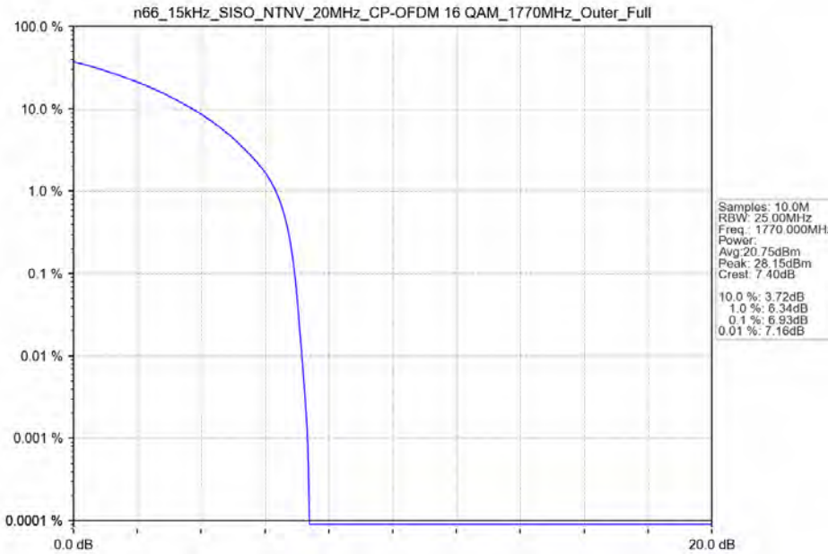
n66_15kHz_SISO_NTNV_20MHz_CP-OFDM 16 QAM_1770MHz_Outer_Full
