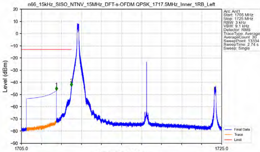
n66_15kHz_SISO_NTNV_15MHz_DFT-s-OFDM_QPSK_1717.5MHz_Inner_1RB_Left
