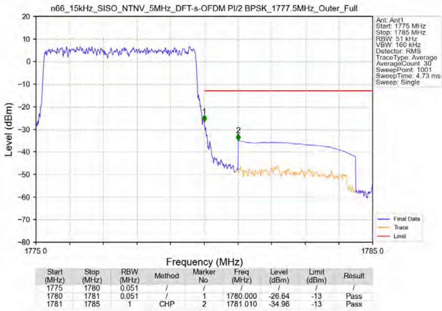
n66_15kHz_SISO_NTNV_5MHz_DFT-s-OFDM PI/2 BPSK_1777.5MHz_Outer_Full
