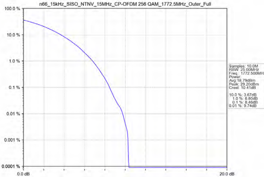
n66_15kHz_SISO_NTNV_15MHz_CP-OFDM 256 QAM_1772.5MHz_Outer_Full
