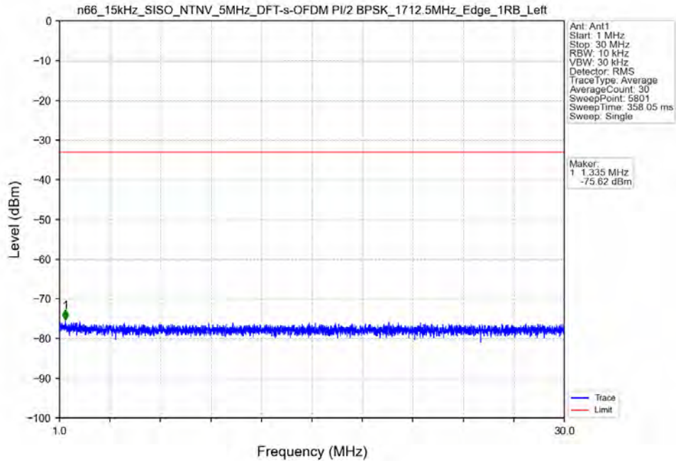
n66_15kHz_SISO_NTNV_5MHz_DFT-s-OFDM PI/2 BPSK_1712.5MHz_Edge_1RB_Left
