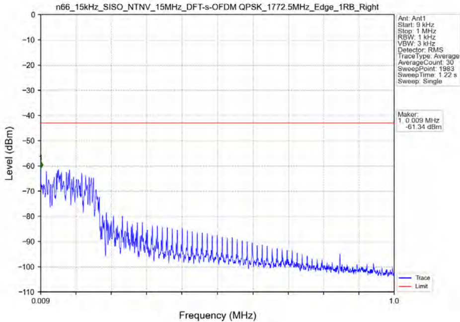
n66_15kHz_SISO_NTNV_15MHz_DFT-s-OFDM QPSK_1772.5MHz_Edge_1RB_Right
