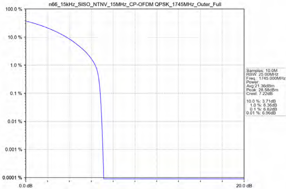
n66_15kHz_SISO_NTNV_15MHz_CP-OFDM QPSK_1745MHz_Outer_Full
