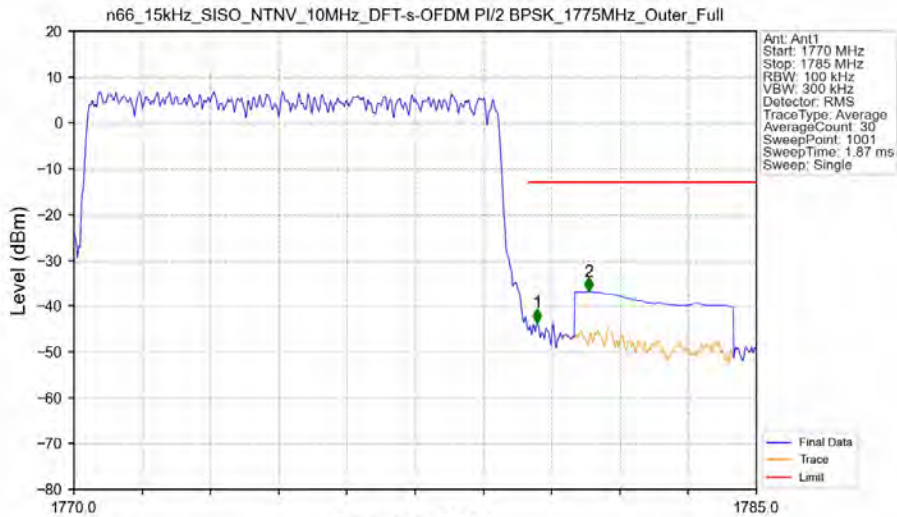
n66_15kHz_SISO_NTNV_10MHz_DFT-s-OFDM PI/2 BPSK_1775MHz_Outer_Full
