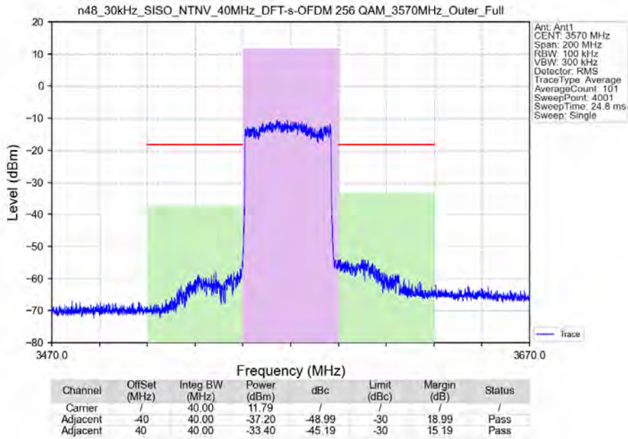
n48_30kHz_SISO_NTNV_40MHz_DFT-s-OFDM 256 QAM_3570MHz_Outer_Full
