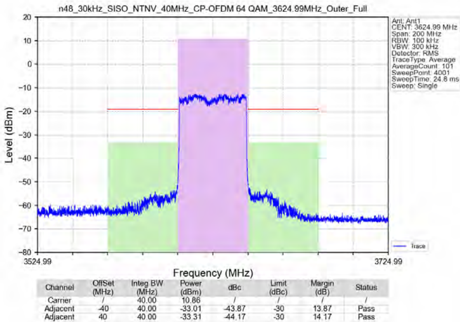
n48_30kHz_SISO_NTNV_40MHz_CP-OFDM 64 QAM_3624.99MHz_Outer_Full
