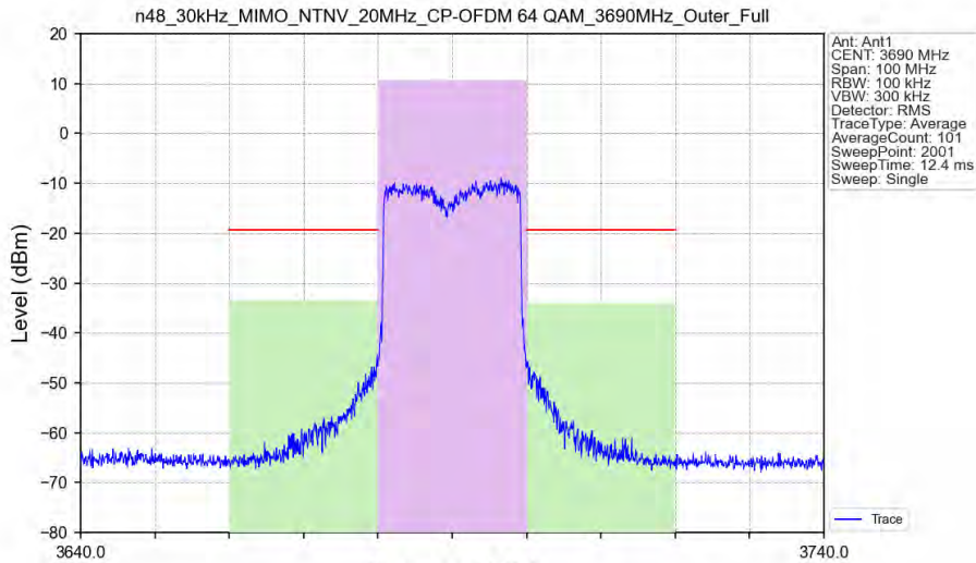
n48_30kHz_MIMO_NTNV_20MHz_CP-OFDM 64 QAM_3690MHz_Outer_Full
