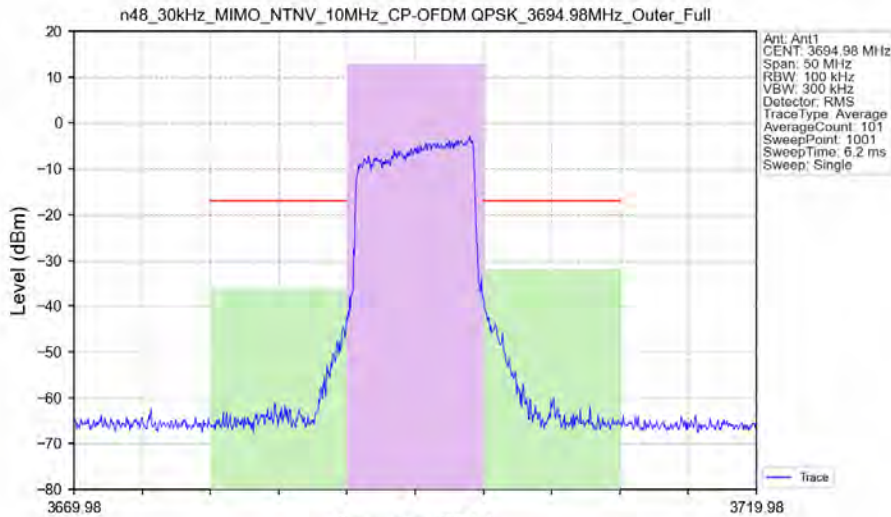
n48_30kHz_MIMO_NTNV_10MHz_CP-OFDM QPSK_3694.98MHz_Outer_Full
