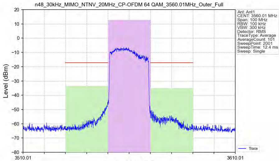
n48_30kHz_MIMO_NTNV_20MHz_CP-OFDM 64 QAM_3560.01MHz_Outer_Full
