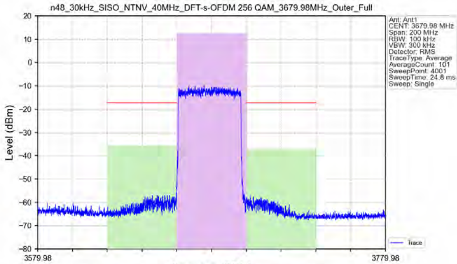
n48_30kHz_SISO_NTNV_40MHz_DFT-s-OFDM 256 QAM_3679.98MHz_Outer_Full
