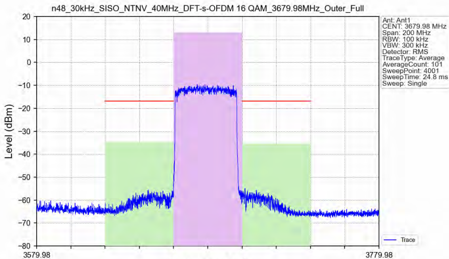
n48_30kHz_SISO_NTNV_40MHz_DFT-s-OFDM 16 QAM_3679.98MHz_Outer_Full
