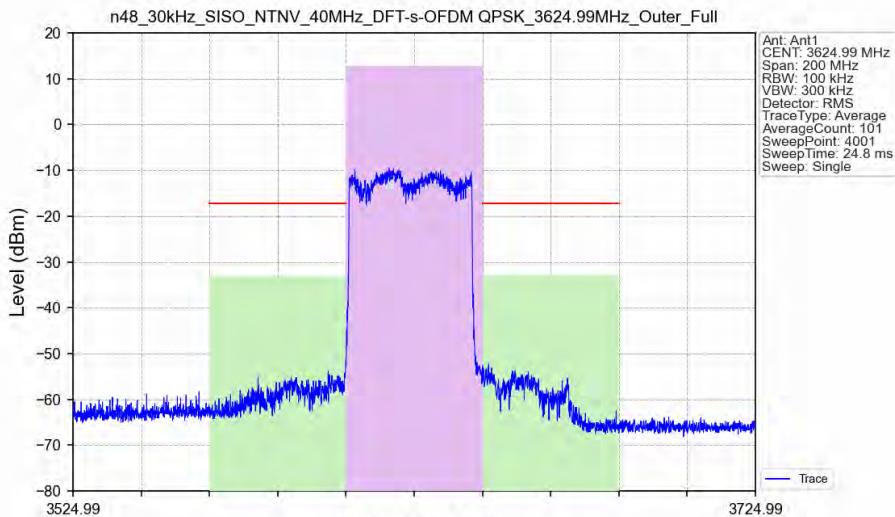
n48_30kHz_SISO_NTNV_40MHz_DFT-s-OFDM QPSK_3624.99MHz_Outer_Full
