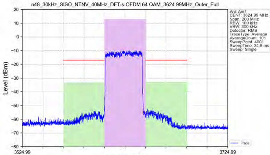
n48_30kHz_SISO_NTNV_40MHz_DFT-s-OFDM 64 QAM_3624.99MHz_Outer_Full
