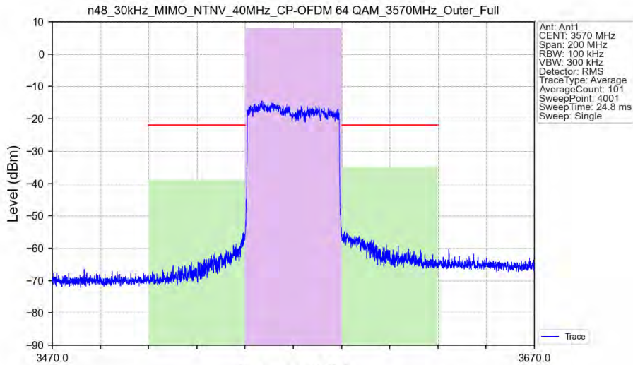
n48_30kHz_MIMO_NTNV_40MHz_CP-OFDM 64 QAM_3570MHz_Outer_Full
