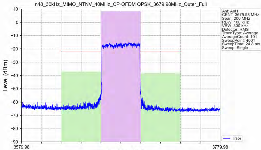
n48_30kHz_MIMO_NTNV_40MHz_CP-OFDM QPSK_3679.98MHz_Outer_Full
