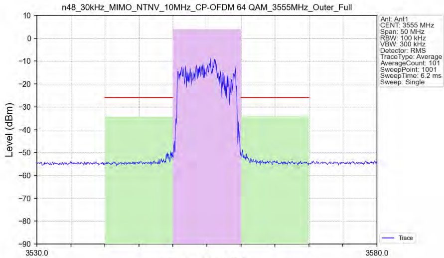
n48_30kHz_MIMO_NTNV_10MHz_CP-OFDM 64 QAM_3555MHz_Outer_Full
