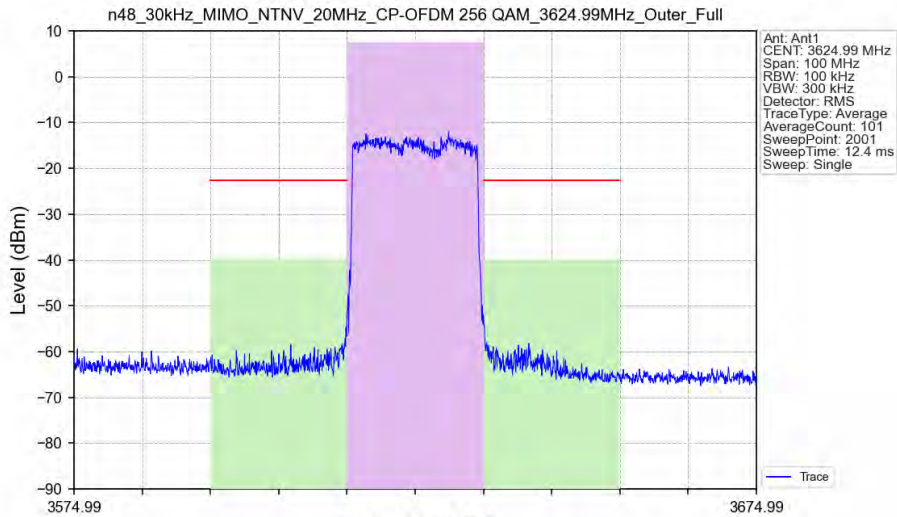
n48_30kHz_MIMO_NTNV_20MHz_CP-OFDM 256 QAM_3624.99MHz_Outer_Full
