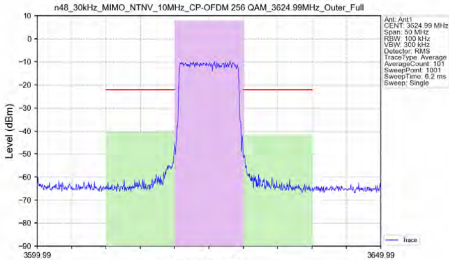
n48_30kHz_MIMO_NTNV_10MHz_CP-OFDM 256 QAM_3624.99MHz_Outer_Full
