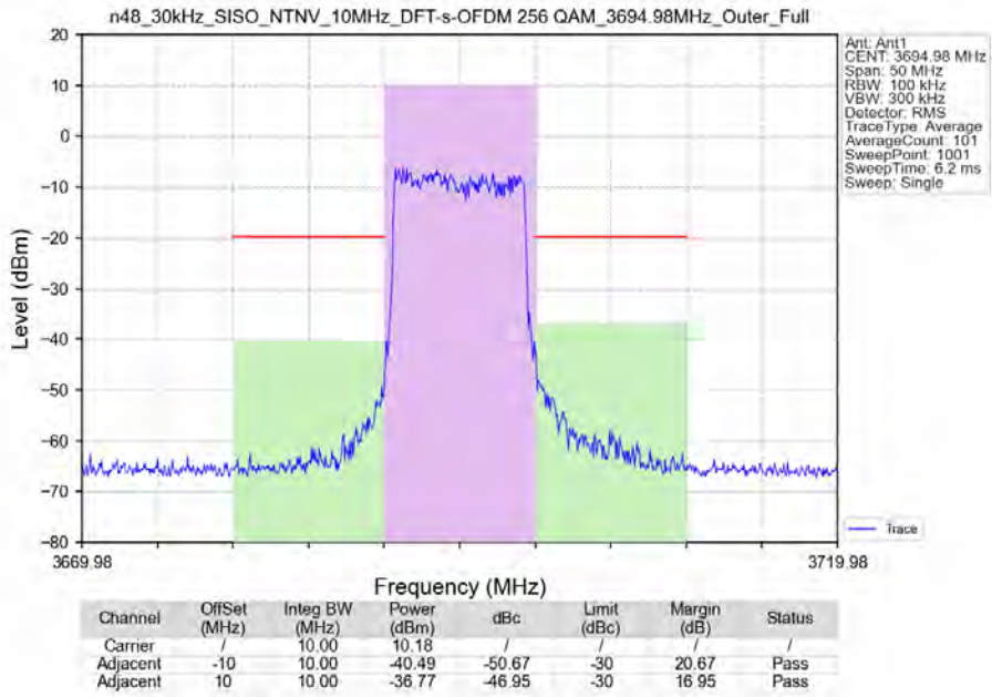
n48_30kHz_SISO_NTNV_10MHz_DFT-s-OFDM 256 QAM_3694.98MHz_Outer_Full
