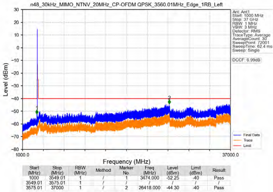
n48_30kHz_MIMO_NTNV_20MHz_CP-OFDM_QPSK_3560.01MHz_Edge_1RB_Left
