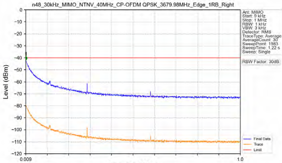
n48_30kHz_MIMO_NTNV_40MHz_CP-OFDM QPSK_3679.98MHz_Edge_1RB_Right
