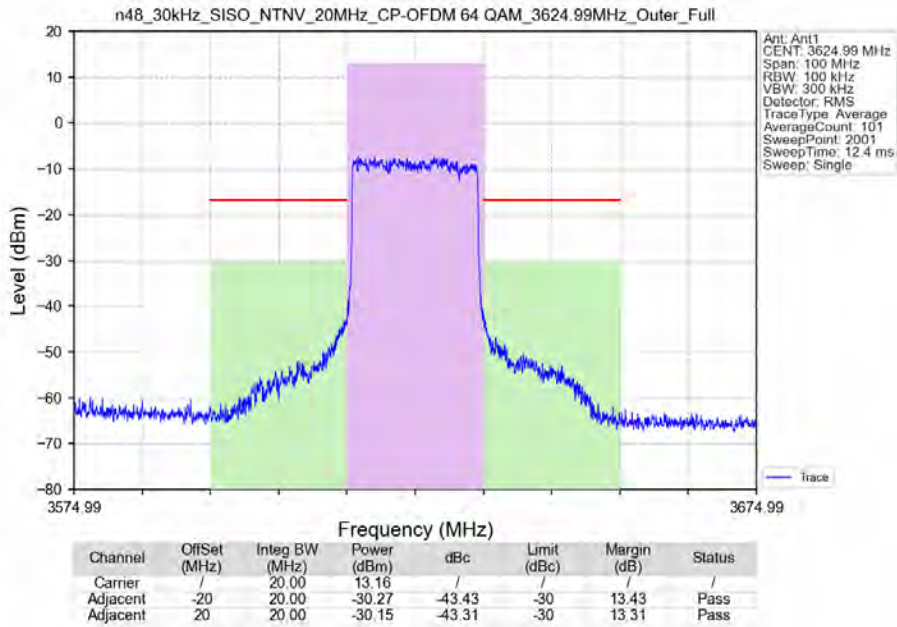
n48_30kHz_SISO_NTNV_20MHz_CP-OFDM 64 QAM_3624.99MHz_Outer_Full
