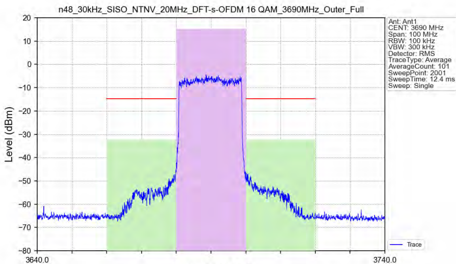
n48_30kHz_SISO_NTNV_20MHz_DFT-s-OFDM 16 QAM_3690MHz_Outer_Full
