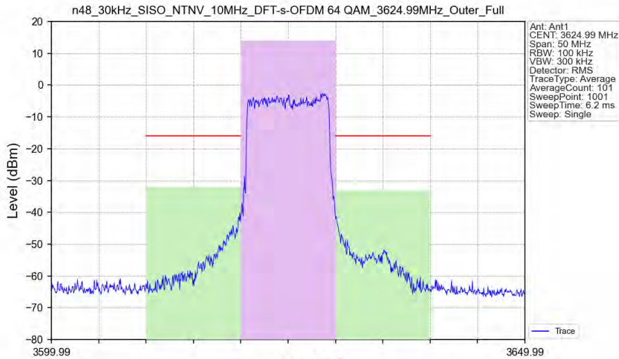
n48_30kHz_SISO_NTNV_10MHz_DFT-s-OFDM 64 QAM_3624.99MHz_Outer_Full
