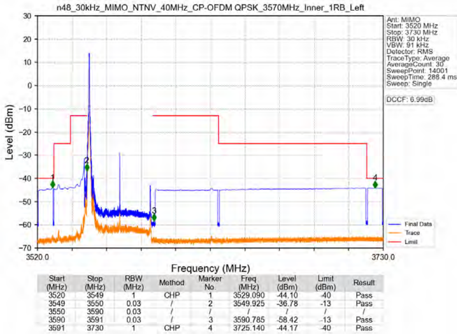
n48_30kHz_MIMO_NTNV_40MHz_CP-OFDM QPSK_3570MHz_Inner_1RB_Left
