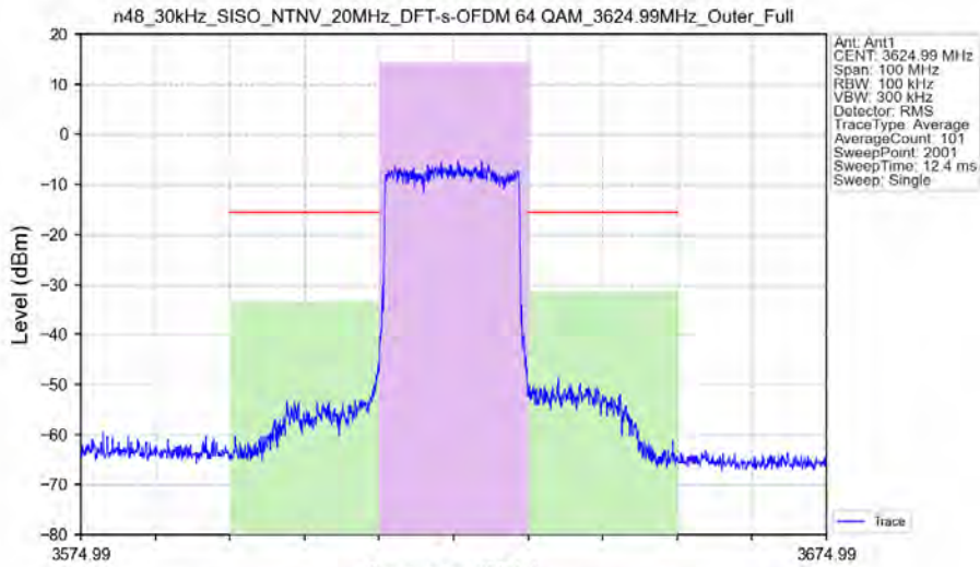
n48_30kHz_SISO_NTNV_20MHz_DFT-s-OFDM 64 QAM_3624.99MHz_Outer_Full
