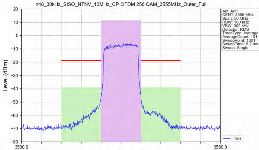
n48_30kHz_SISO_NTNV_10MHz_CP-OFDM 256 QAM_3555MHz_Outer_Full
