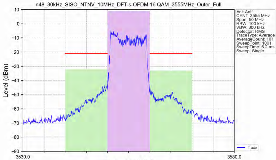
n48_30kHz_SISO_NTNV_10MHz_DFT-s-OFDM 16 QAM_3555MHz_Outer_Full
