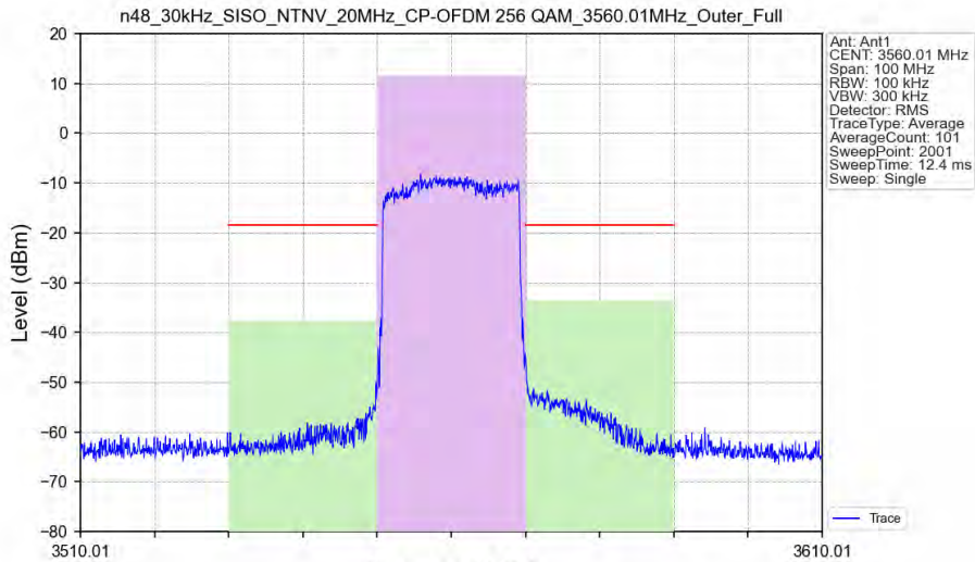
n48_30kHz_SISO_NTNV_20MHz_CP-OFDM 256 QAM_3560.01MHz_Outer_Full
