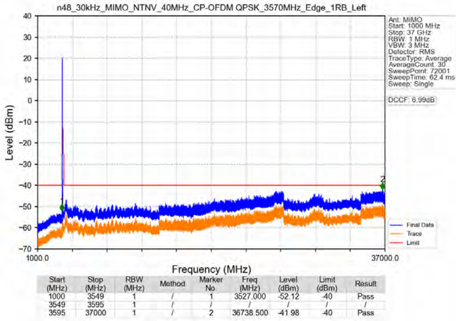
n48_30kHz_MIMO_NTNV_40MHz_CP-OFDM QPSK_3570MHz_Edge_1RB_Left
