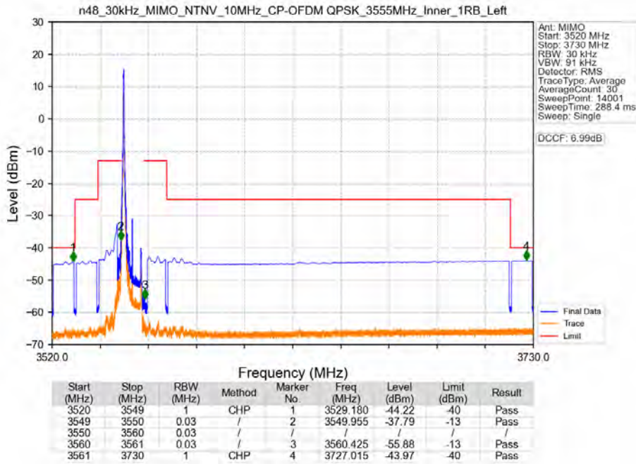
n48_30kHz_MIMO_NTNV_10MHz_CP-OFDM QPSK_3555MHz_Inner_1RB_Left
