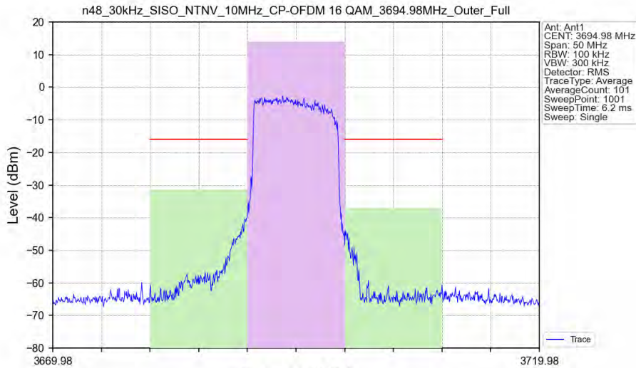
n48_30kHz_SISO_NTNV_10MHz_CP-OFDM 16 QAM_3694.98MHz_Outer_Full
