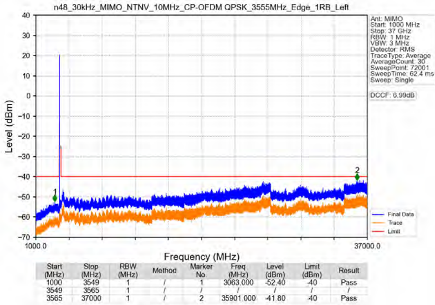
n48_30kHz_MIMO_NTNV_10MHz_CP-OFDM QPSK_3555MHz_Edge_1RB_Left
