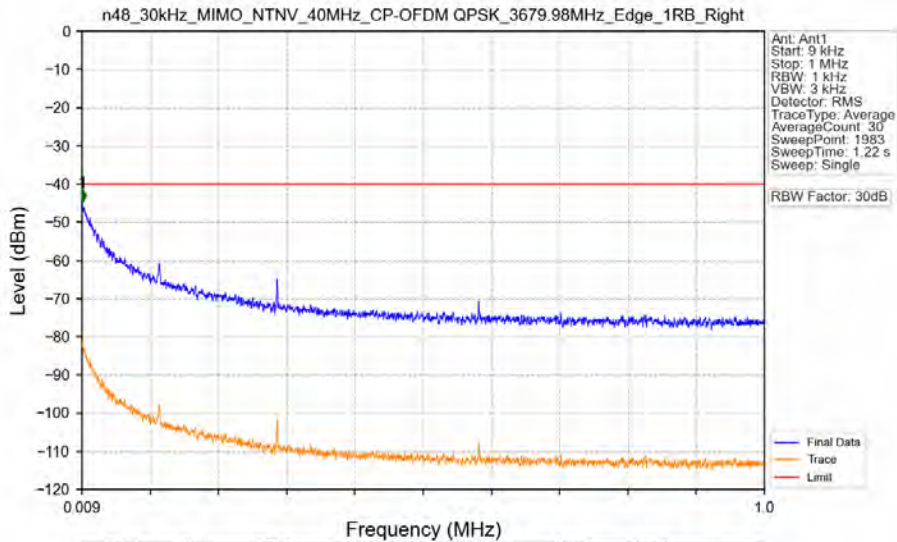
n48_30kHz_MIMO_NTNV_40MHz_CP-OFDM QPSK_3679.98MHz_Edge_1RB_Right
