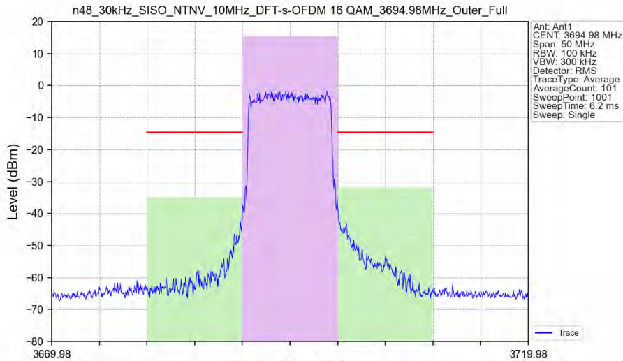
n48_30kHz_SISO_NTNV_10MHz_DFT-s-OFDM 16 QAM_3694.98MHz_Outer_Full
