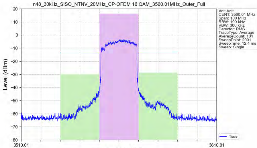
n48_30kHz_SISO_NTNV_20MHz_CP-OFDM 16 QAM_3560.01MHz_Outer_Full
