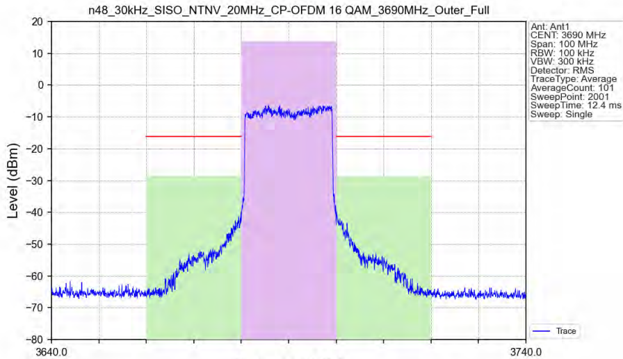
n48_30kHz_SISO_NTNV_20MHz_CP-OFDM 16 QAM_3690MHz_Outer_Full
