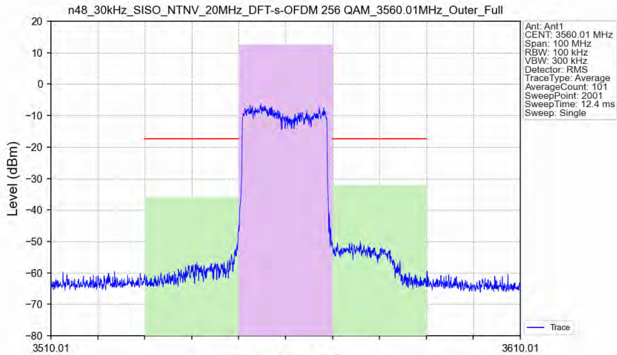
n48_30kHz_SISO_NTNV_20MHz_DFT-s-OFDM_256_QAM_3560.01MHz_Outer_Full
