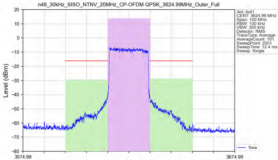
n48_30kHz_SISO_NTNV_20MHz_CP-OFDM QPSK_3624.99MHz_Outer_Full
