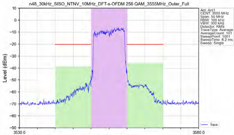
n48_30kHz_SISO_NTNV_10MHz_DFT-s-OFDM 256 QAM_3555MHz_Outer_Full
