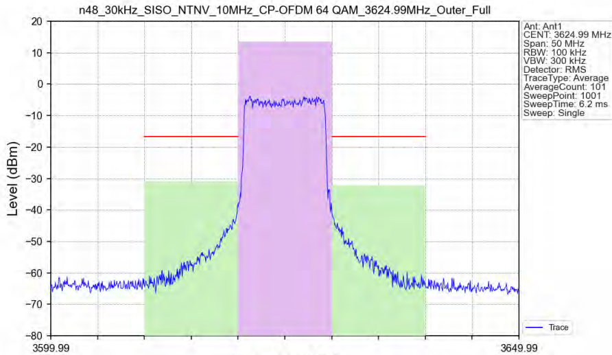
n48_30kHz_SISO_NTNV_10MHz_CP-OFDM 64 QAM_3624.99MHz_Outer_Full
