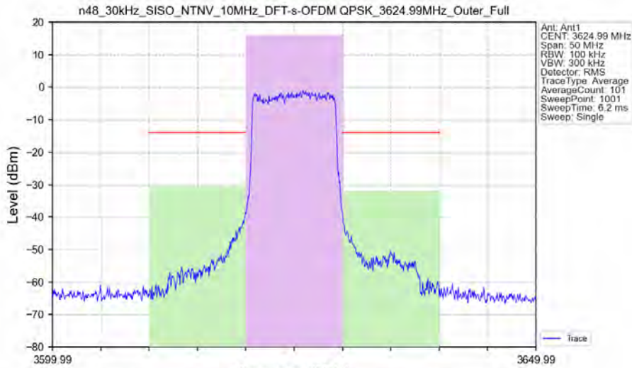
n48_30kHz_SISO_NTNV_10MHz_DFT-s-OFDM QPSK_3624.99MHz_Outer_Full
