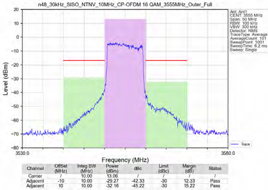
n48_30kHz_SISO_NTNV_10MHz_CP-OFDM 16 QAM_3555MHz_Outer_Full
