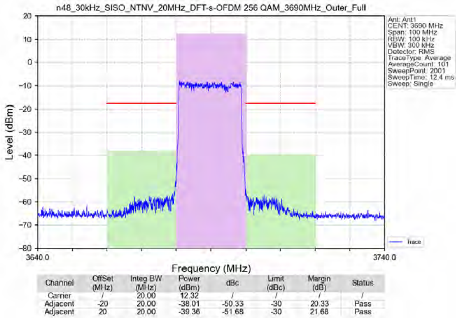
n48_30kHz_SISO_NTNV_20MHz_DFT-s-OFDM 256 QAM_3690MHz_Outer_Full
