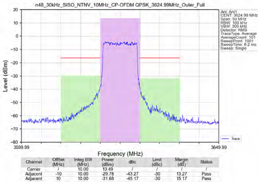
n48_30kHz_SISO_NTNV_10MHz_CP-OFDM QPSK_3624.99MHz_Outer_Full
