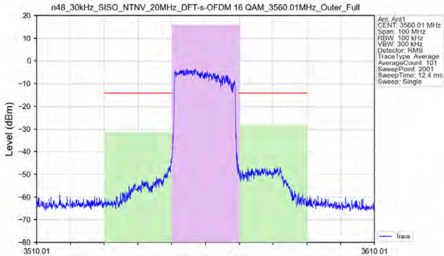
n48_30kHz_SISO_NTNV_20MHz_DFT-s-OFDM 16 QAM_3560.01MHz_Outer_Full
