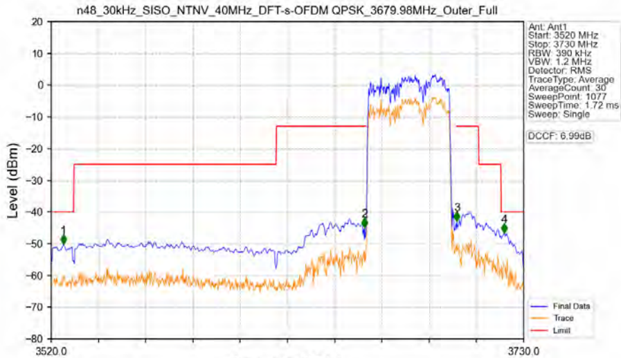
n48_30kHz_SISO_NTNV_40MHz_DFT-s-OFDM QPSK_3679.98MHz_Outer_Full
