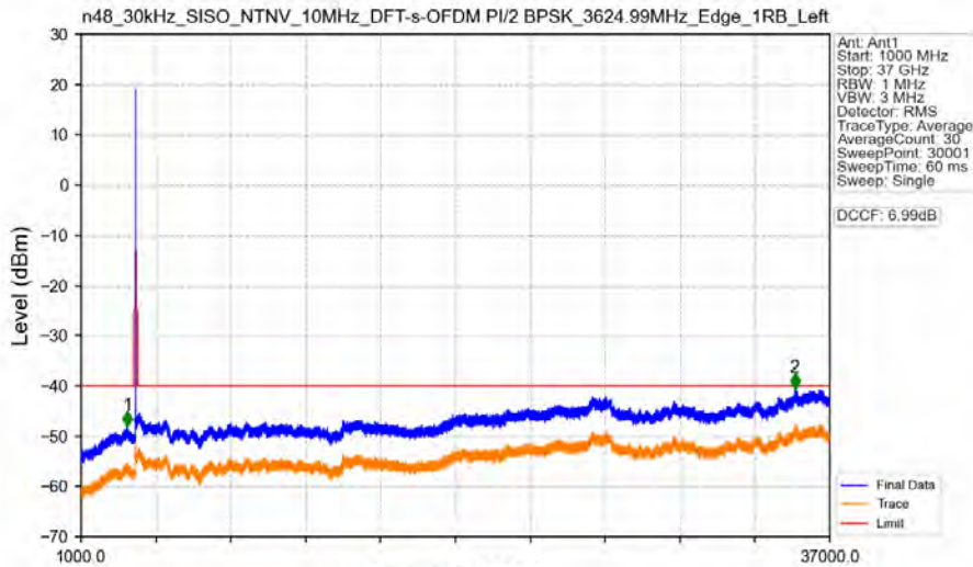
n48_30kHz_SISO_NTNV_10MHz_DFT-s-OFDM PI/2 BPSK_3624.99MHz_Edge_1RB_Left
