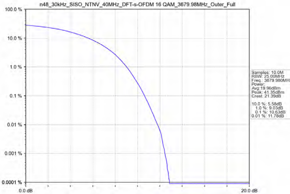
n48_30kHz_SISO_NTNV_40MHz_DFT-s-OFDM 16 QAM_3679.98MHz_Outer_Full
