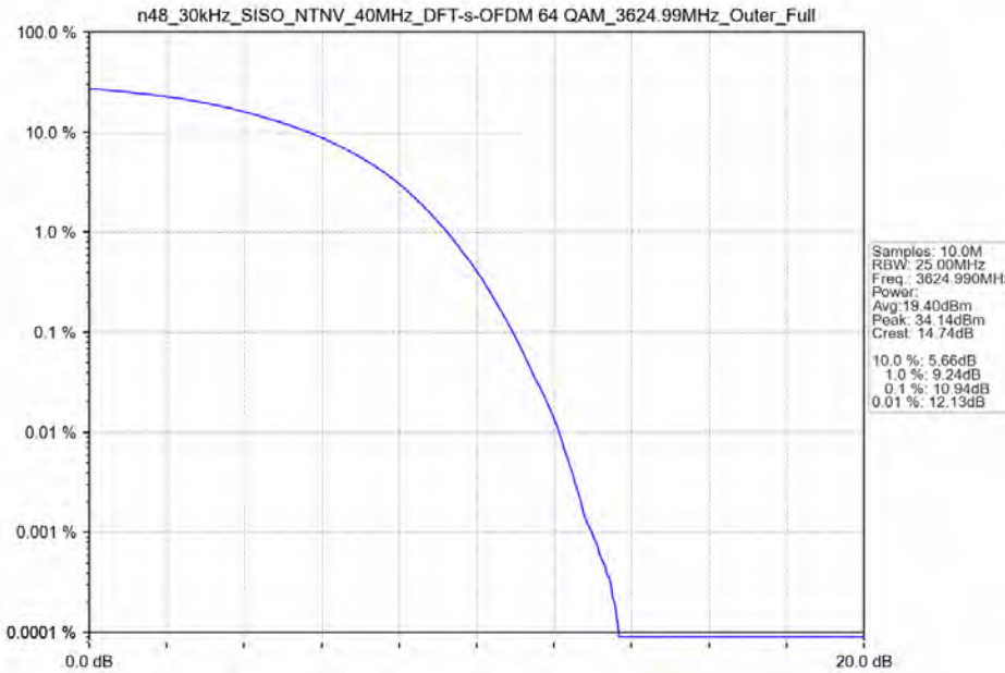
n48_30kHz_SISO_NTNV_40MHz_DFT-s-OFDM 64 QAM_3624.99MHz_Outer_Full
