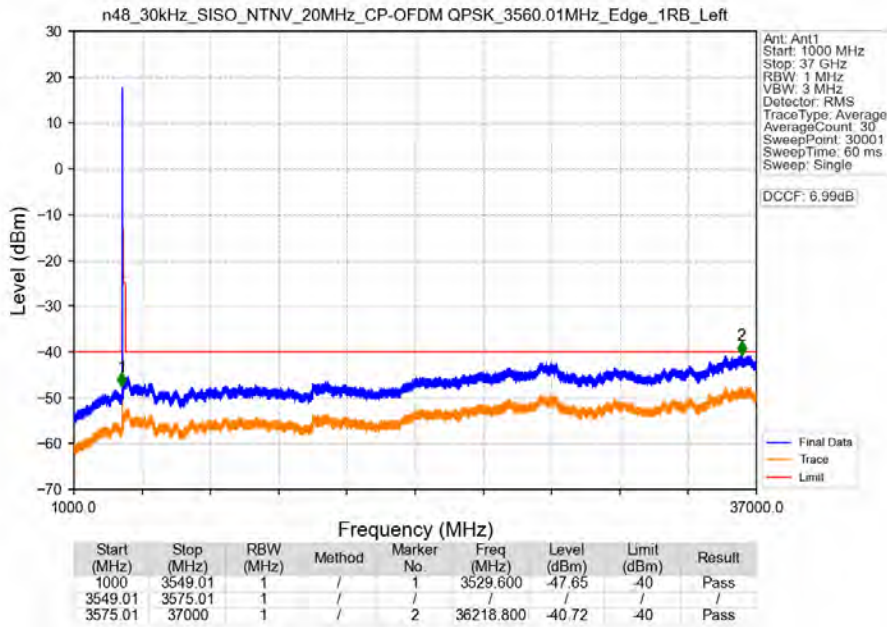
n48_30kHz_SISO_NTNV_20MHz_CP-OFDM QPSK_3560.01MHz_Edge_1RB_Left
