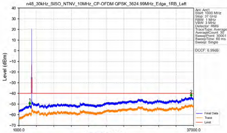
n48_30kHz_SISO_NTNV_10MHz_CP-OFDM QPSK_3624.99MHz_Edge_1RB_Left
