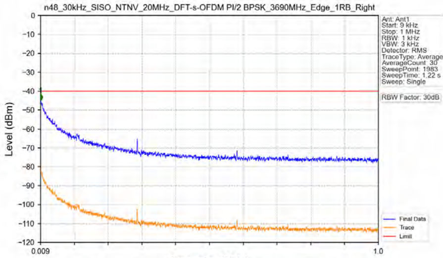
n48_30kHz_SISO_NTNV_20MHz_DFT-s-OFDM PI/2 BPSK_3690MHz_Edge_1RB_Right
