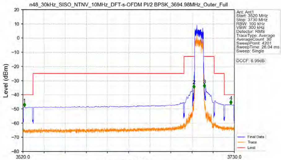
n48_30kHz_SISO_NTNV_10MHz_DFT-s-OFDM PI/2 BPSK_3694.98MHz_Outer_Full
