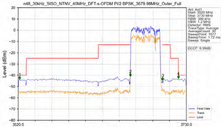
n48_30kHz_SISO_NTNV_40MHz_DFT-s-OFDM PI/2 BPSK_3679.98MHz_Outer_Full
