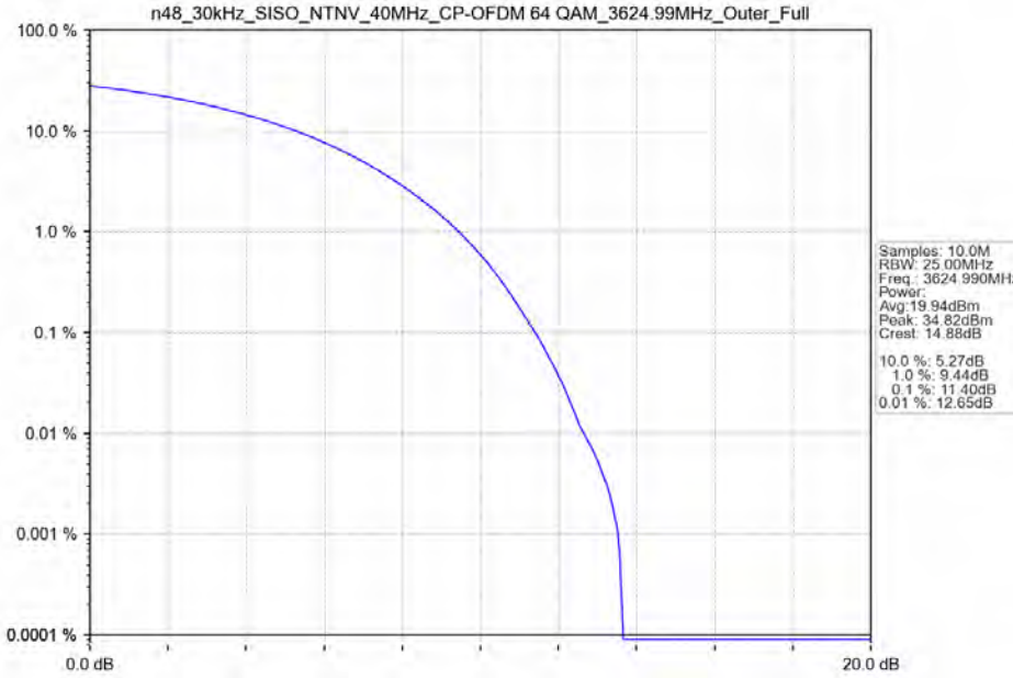
n48_30kHz_SISO_NTNV_40MHz_CP-OFDM 64 QAM_3624.99MHz_Outer_Full
