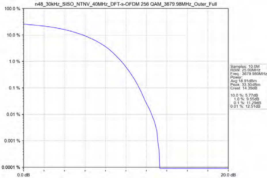
n48_30kHz_SISO_NTNV_40MHz_DFT-s-OFDM 256 QAM_3679.98MHz_Outer_Full
