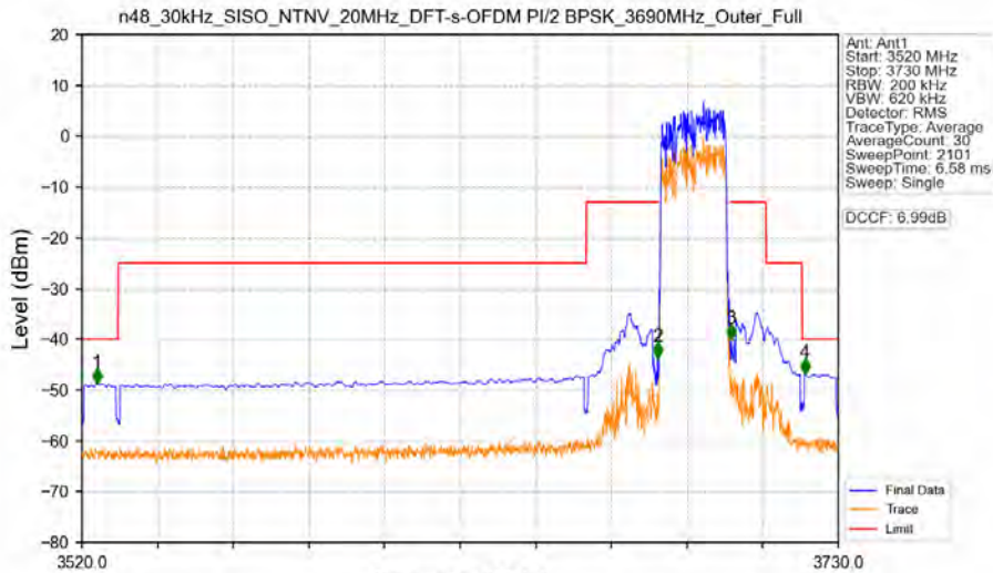
n48_30kHz_SISO_NTNV_20MHz_DFT-s-OFDM PI/2 BPSK_3690MHz_Outer_Full
