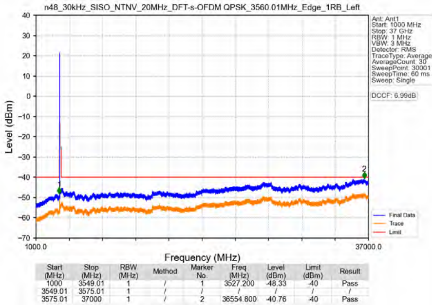
n48_30kHz_SISO_NTNV_20MHz_DFT-s-OFDM QPSK_3560.01MHz_Edge_1RB_Left
