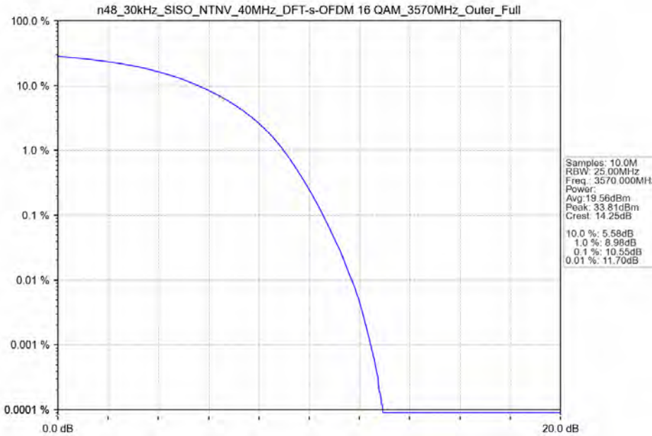
n48_30kHz_SISO_NTNV_40MHz_DFT-s-OFDM 16 QAM_3570MHz_Outer_Full
