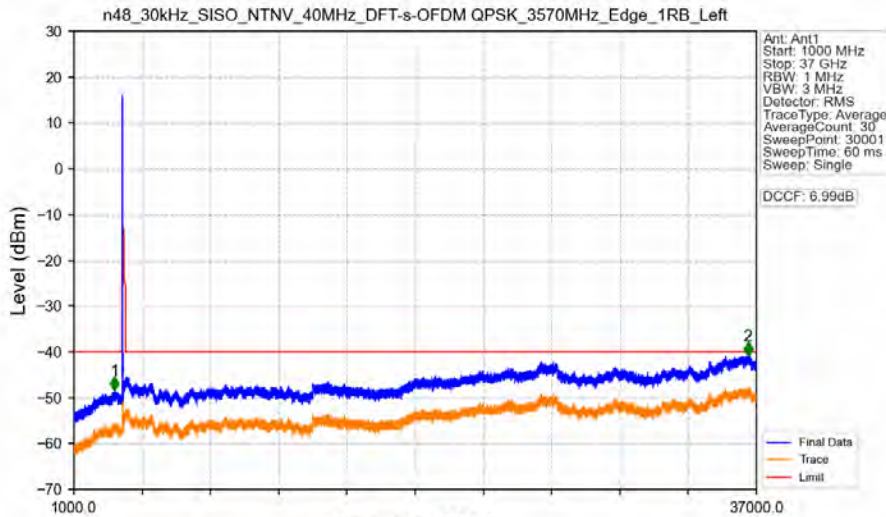
n48_30kHz_SISO_NTNV_40MHz_DFT-s-OFDM QPSK_3570MHz_Edge_1RB_Left
