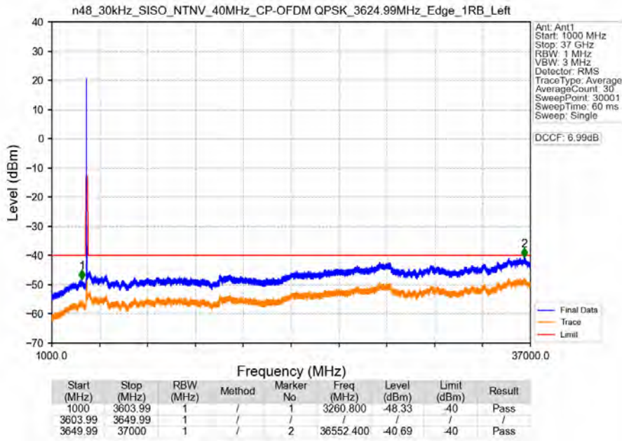
n48_30kHz_SISO_NTNV_40MHz_CP-OFDM QPSK_3624.99MHz_Edge_1RB_Left
