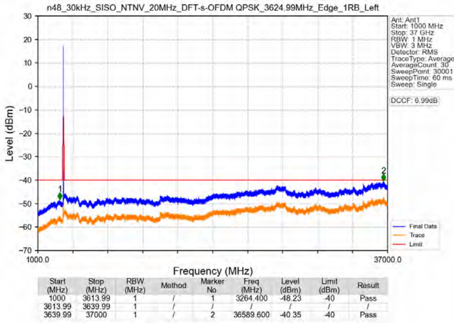
n48_30kHz_SISO_NTNV_20MHz_DFT-s-OFDM_QPSK_3624.99MHz_Edge_1RB_Left
