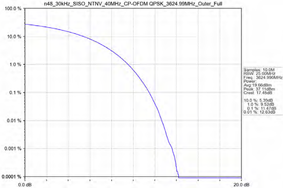
n48_30kHz_SISO_NTNV_40MHz_CP-OFDM QPSK_3624.99MHz_Outer_Full
