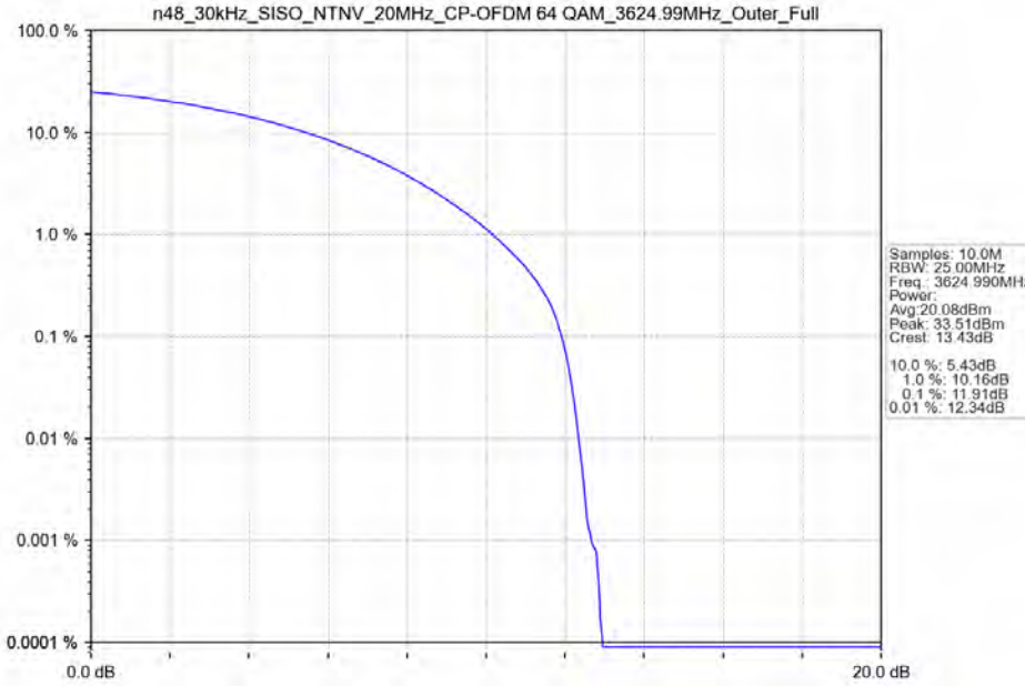
n48_30kHz_SISO_NTNV_20MHz_CP-OFDM 64 QAM_3624.99MHz_Outer_Full
