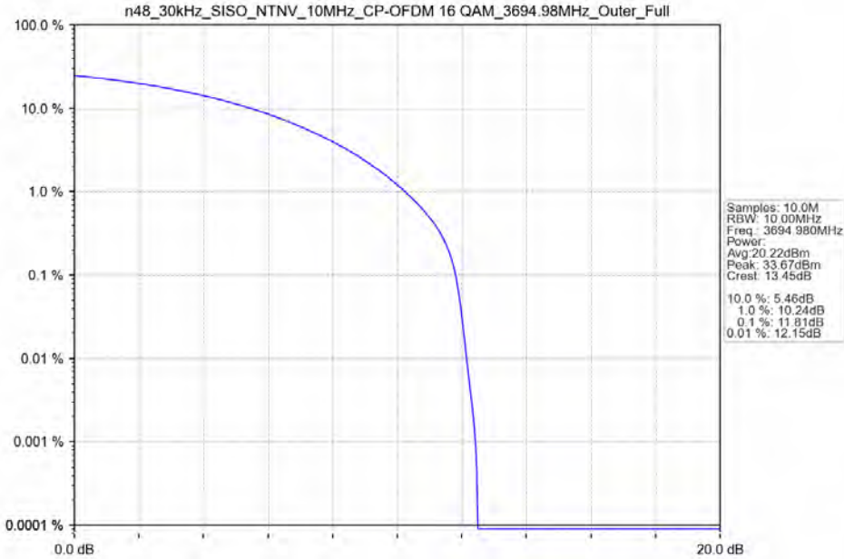
n48_30kHz_SISO_NTNV_10MHz_CP-OFDM 16 QAM_3694.98MHz_Outer_Full
