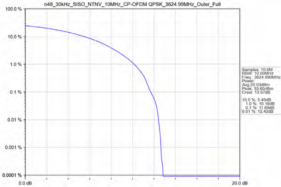
n48_30kHz_SISO_NTNV_10MHz_CP-OFDM QPSK_3624.99MHz_Outer_Full
