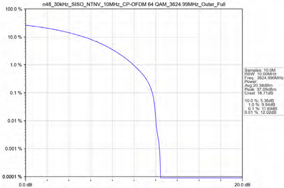
n48_30kHz_SISO_NTNV_10MHz_CP-OFDM 64 QAM_3624.99MHz_Outer_Full
