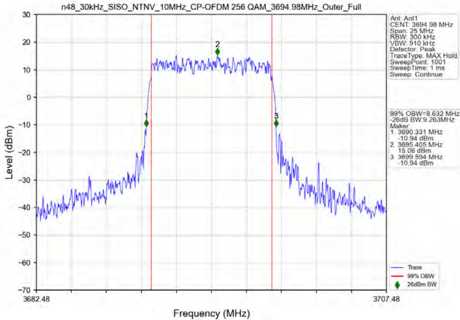
n48_30kHz_SISO_NTNV_10MHz_CP-OFDM 256 QAM_3694.98MHz_Outer_Full
