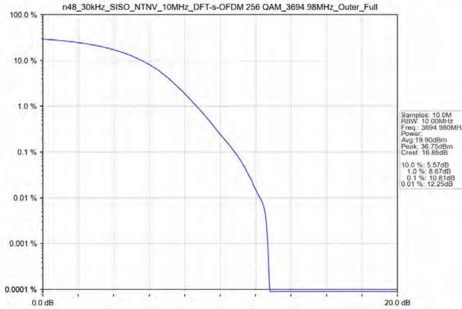
n48_30kHz_SISO_NTNV_10MHz_DFT-s-OFDM 256 QAM_3694.98MHz_Outer_Full
