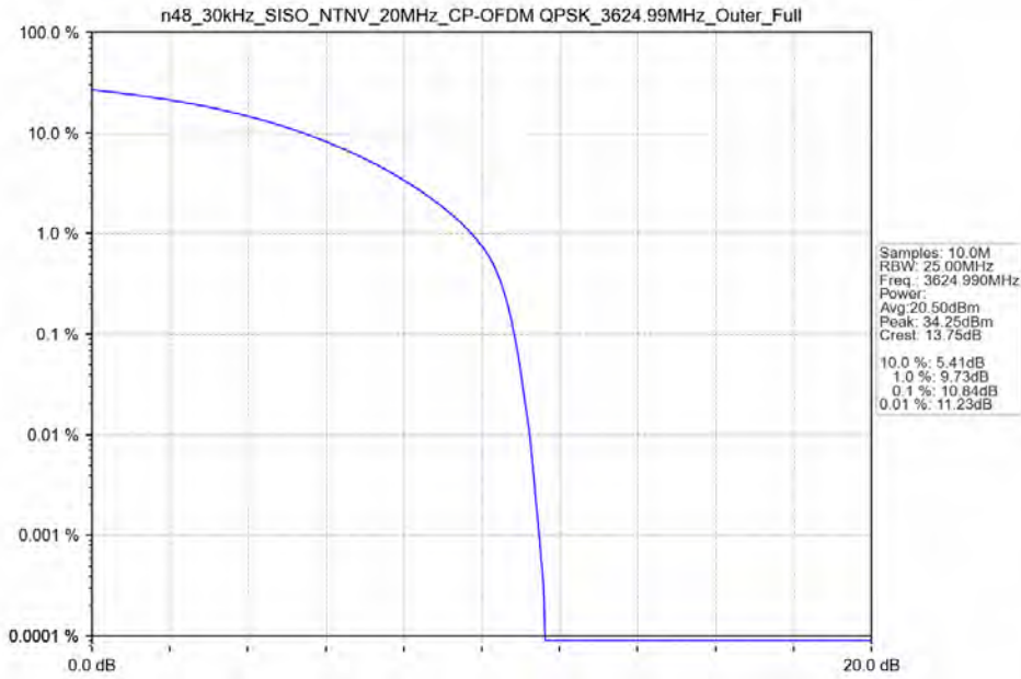
n48_30kHz_SISO_NTNV_20MHz_CP-OFDM QPSK_3624.99MHz_Outer_Full
