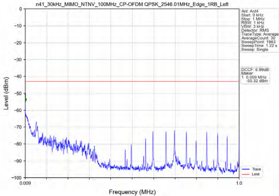
n41_30kHz_MIMO_NTNV_100MHz_CP-OFDM QPSK_2546.01MHz_Edge_1RB_Left
