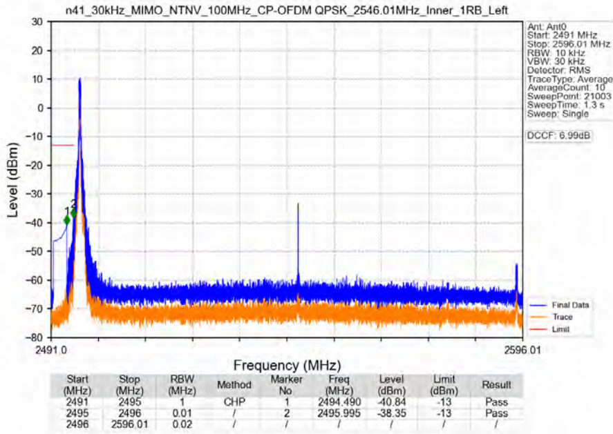
n41_30kHz_MIMO_NTNV_100MHz_CP-OFDM QPSK_2546.01MHz_Inner_1RB_Left
