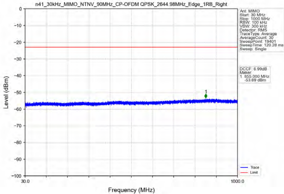
n41_30kHz_MIMO_NTNV_90MHz_CP-OFDM QPSK_2644.98MHz_Edge_1RB_Right
