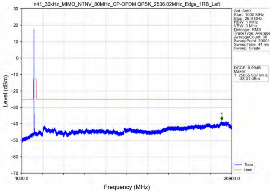
n41_30kHz_MIMO_NTNV_80MHz_CP-OFDM QPSK_2536.02MHz_Edge_1RB_Left
