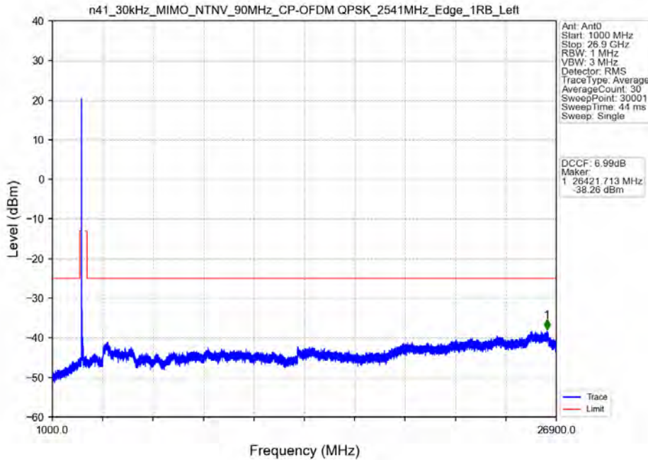
n41_30kHz_MIMO_NTNV_90MHz_CP-OFDM QPSK_2541MHz_Edge_1RB_Left
