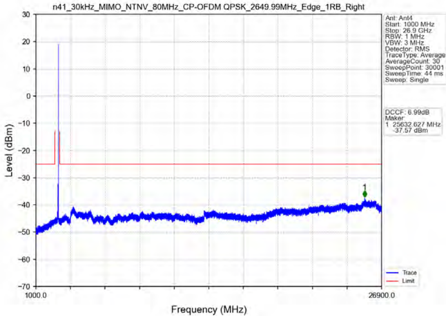
n41_30kHz_MIMO_NTNV_80MHz_CP-OFDM QPSK_2649.99MHz_Edge_1RB_Right
