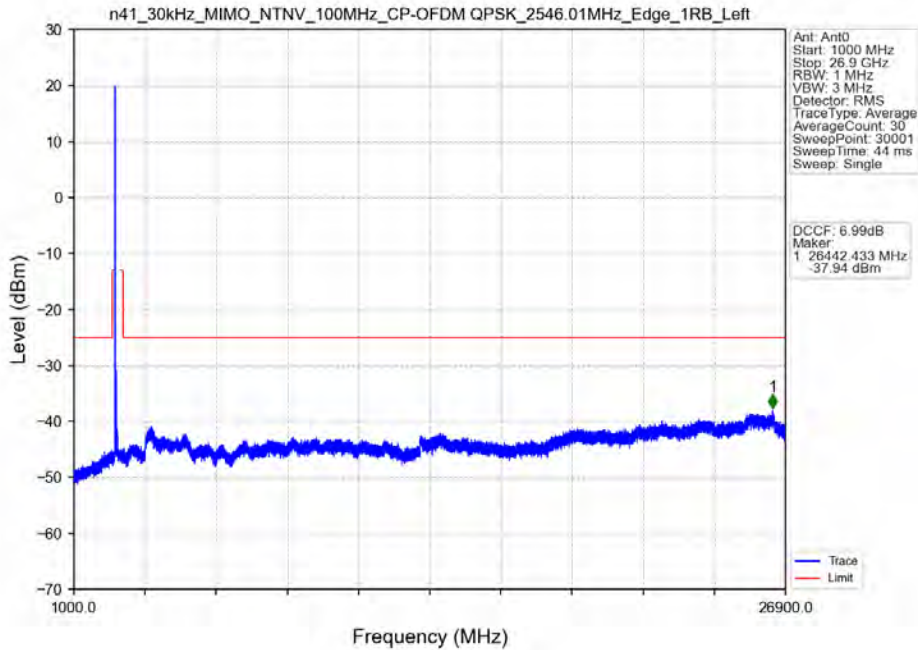
n41_30kHz_MIMO_NTNV_100MHz_CP-OFDM QPSK_2546.01MHz_Edge_1RB_Left
