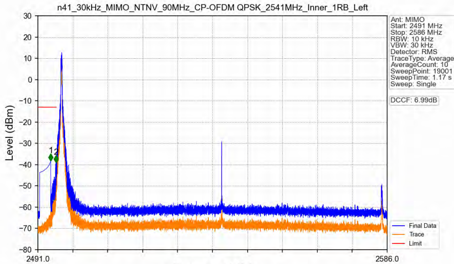
n41_30kHz_MIMO_NTNV_90MHz_CP-OFDM QPSK_2541MHz_Inner_1RB_Left
