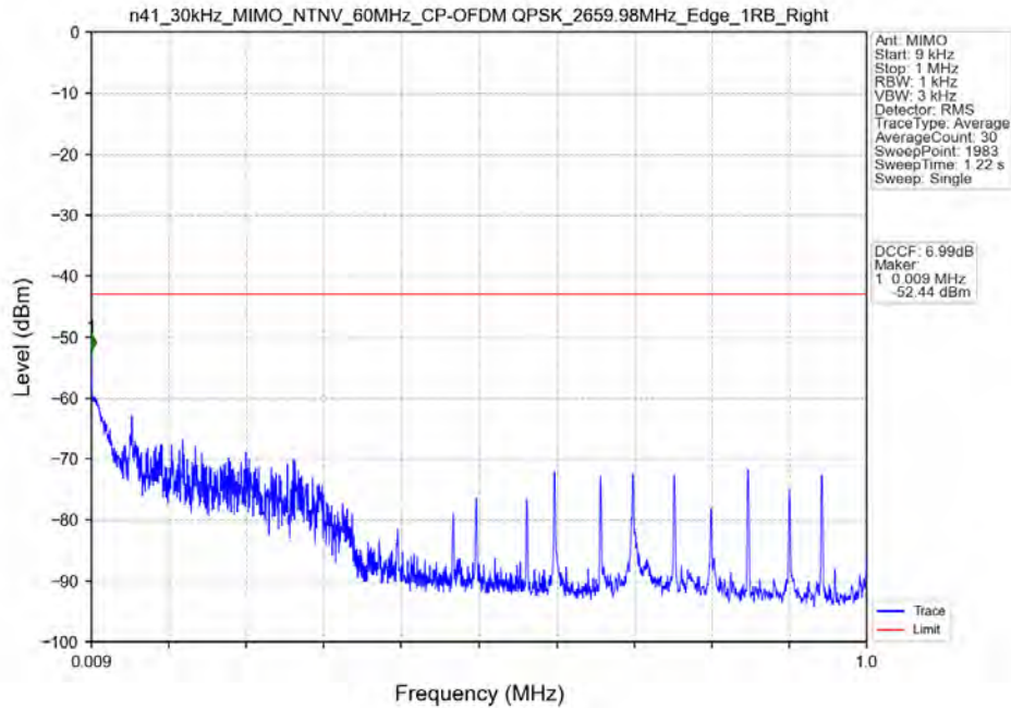
n41_30kHz_MIMO_NTNV_60MHz_CP-OFDM QPSK_2659.98MHz_Edge_1RB_Right
