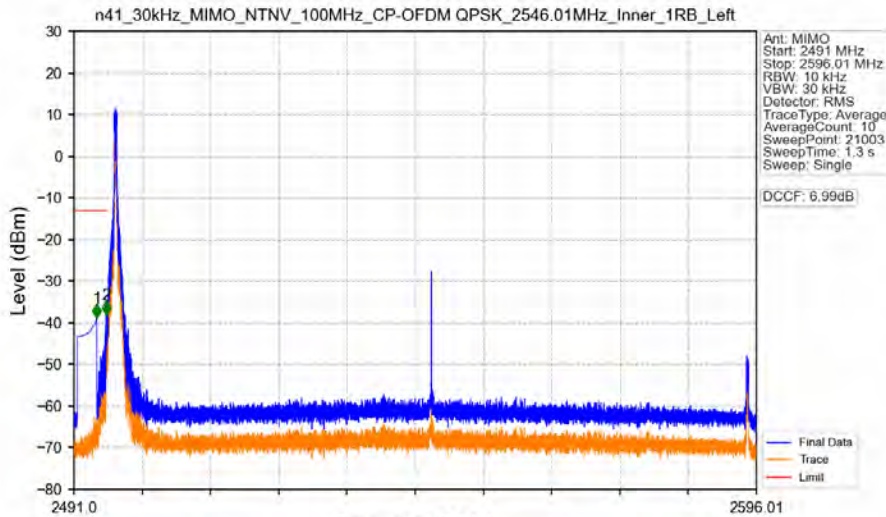
n41_30kHz_MIMO_NTNV_100MHz_CP-OFDM QPSK_2546.01MHz_Inner_1RB_Left
