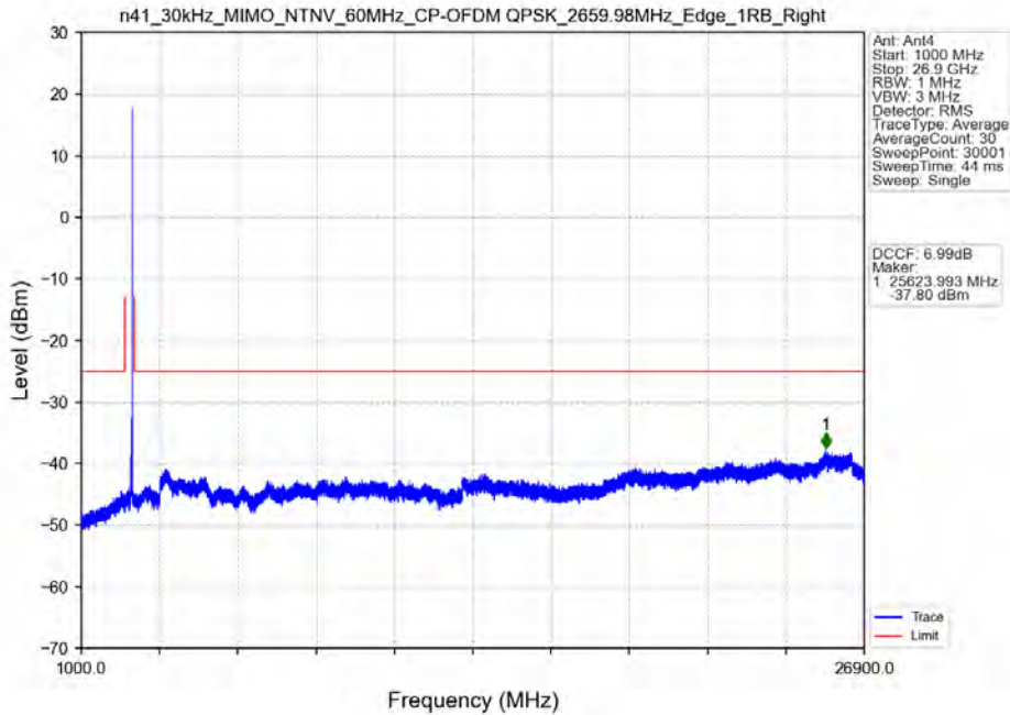
n41_30kHz_MIMO_NTNV_60MHz_CP-OFDM QPSK_2659.98MHz_Edge_1RB_Right
