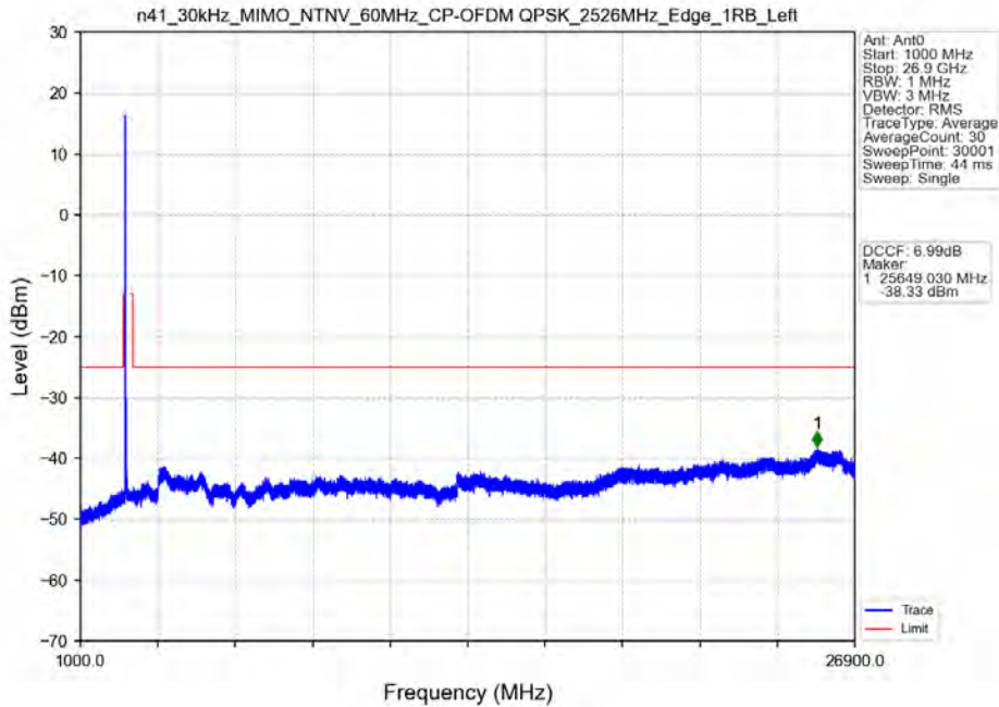
n41_30kHz_MIMO_NTNV_60MHz_CP-OFDM QPSK_2526MHz_Edge_1RB_Left
