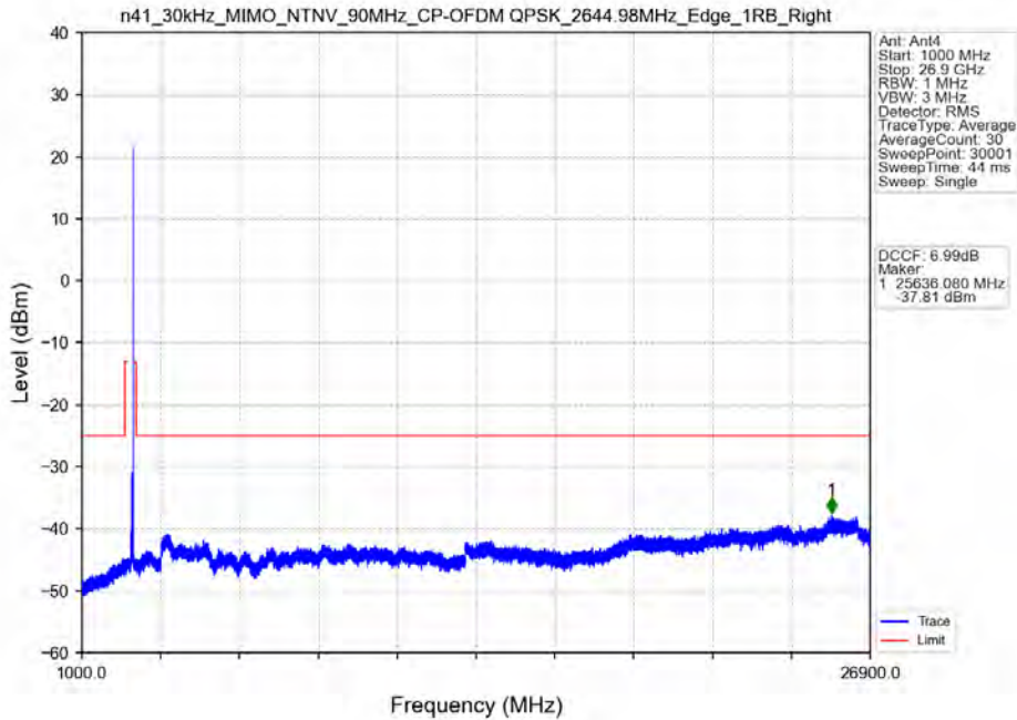
n41_30kHz_MIMO_NTNV_90MHz_CP-OFDM QPSK_2644.98MHz_Edge_1RB_Right
