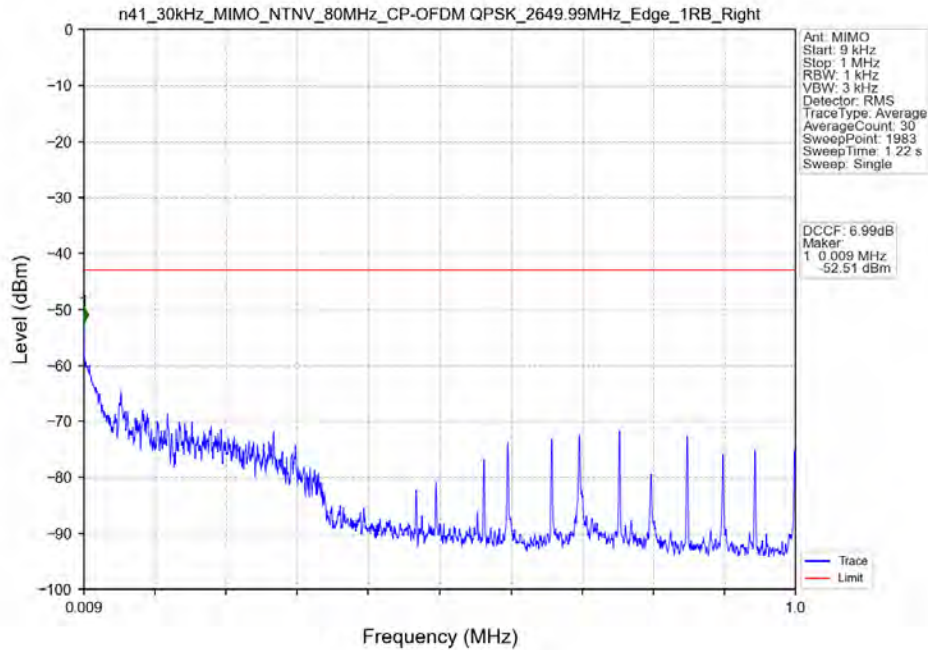
n41_30kHz_MIMO_NTNV_80MHz_CP-OFDM QPSK_2649.99MHz_Edge_1RB_Right
