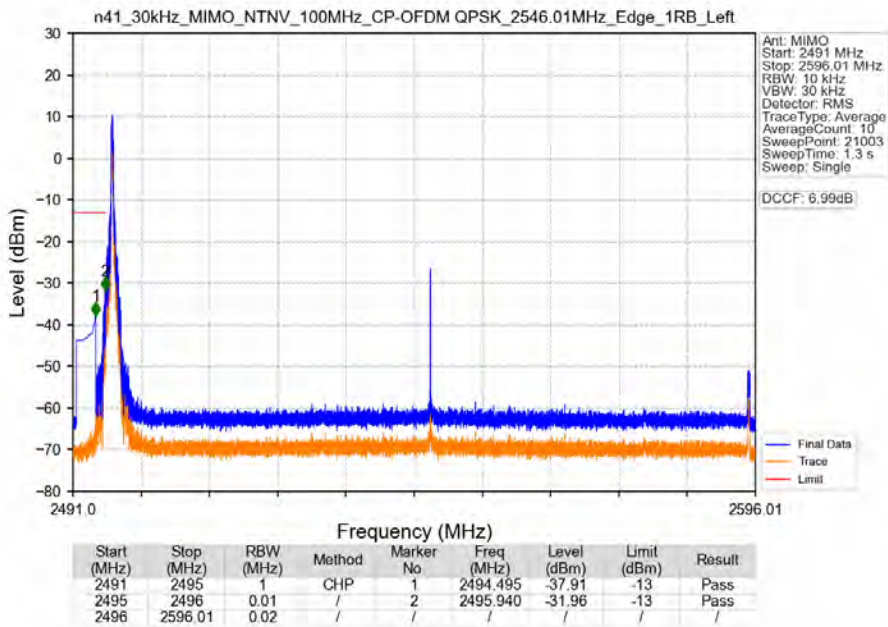
n41_30kHz_MIMO_NTNV_100MHz_CP-OFDM QPSK_2546.01MHz_Edge_1RB_Left
