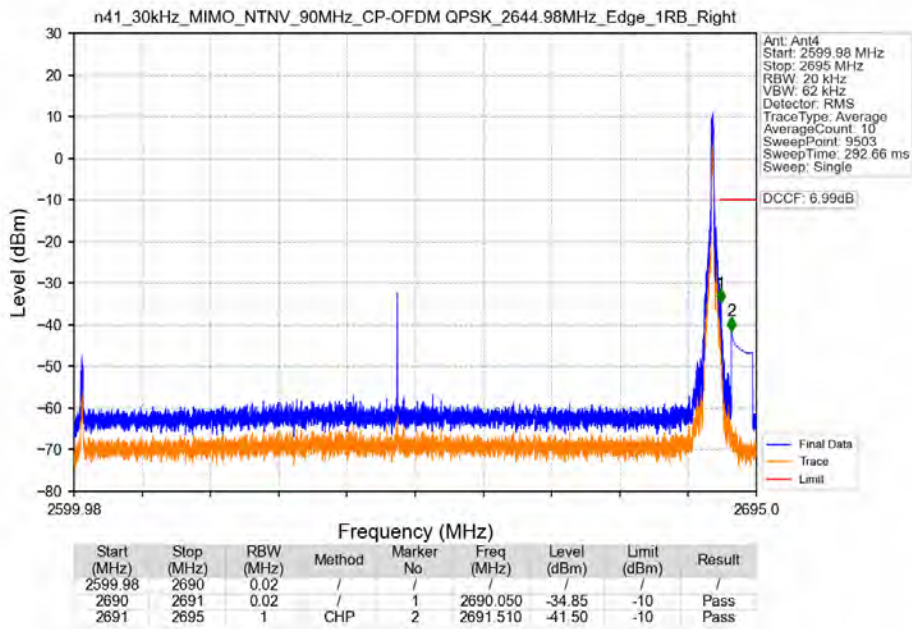
n41_30kHz_MIMO_NTNV_90MHz_CP-OFDM QPSK_2644.98MHz_Edge_1RB_Right
