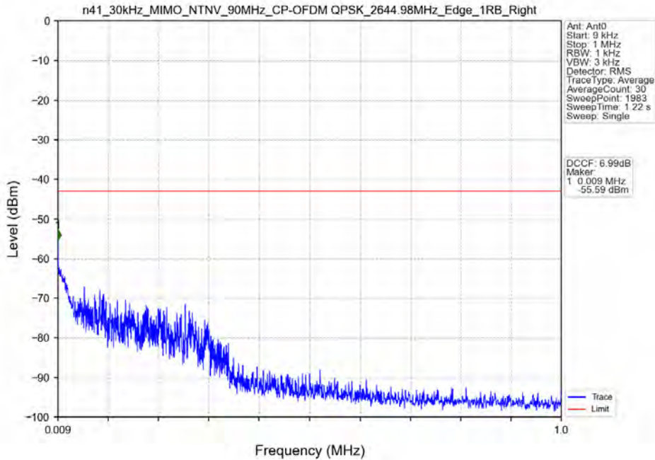
n41_30kHz_MIMO_NTNV_90MHz_CP-OFDM QPSK_2644.98MHz_Edge_1RB_Right
