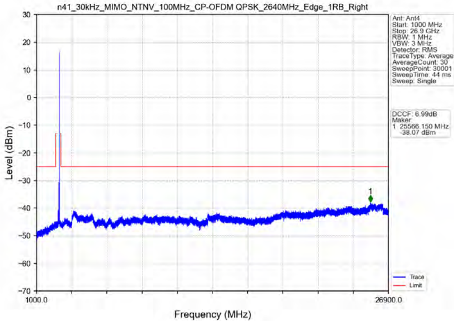
n41_30kHz_MIMO_NTNV_100MHz_CP-OFDM QPSK_2640MHz_Edge_1RB_Right
