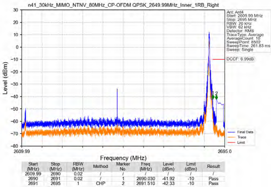
n41_30kHz_MIMO_NTNV_80MHz_CP-OFDM_QPSK_2649.99MHz_Inner_1RB_Right
