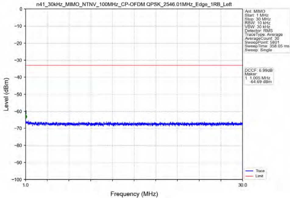
n41_30kHz_MIMO_NTNV_100MHz_CP-OFDM QPSK_2546.01MHz_Edge_1RB_Left
