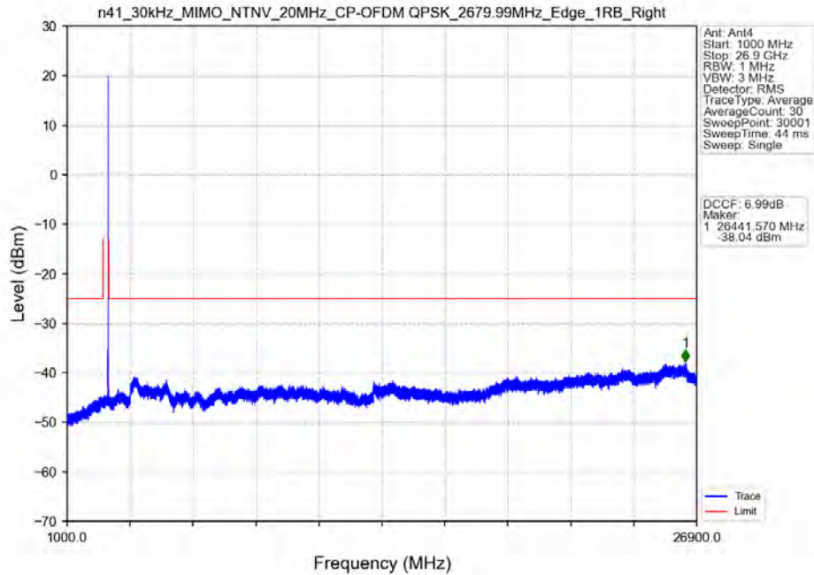
n41_30kHz_MIMO_NTNV_20MHz_CP-OFDM QPSK_2679.99MHz_Edge_1RB_Right
