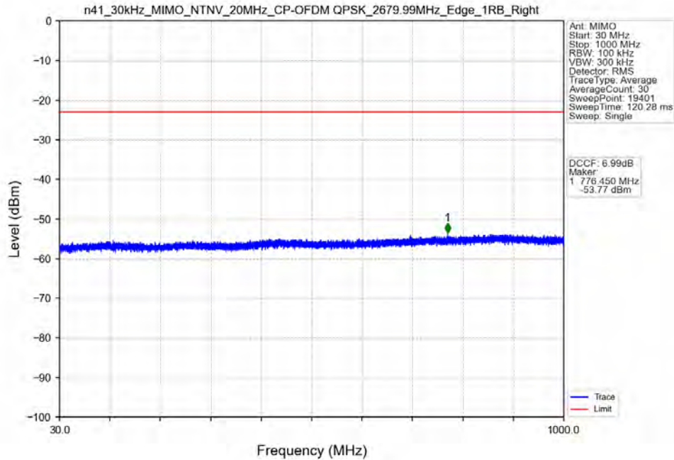
n41_30kHz_MIMO_NTNV_20MHz_CP-OFDM QPSK_2679.99MHz_Edge_1RB_Right
