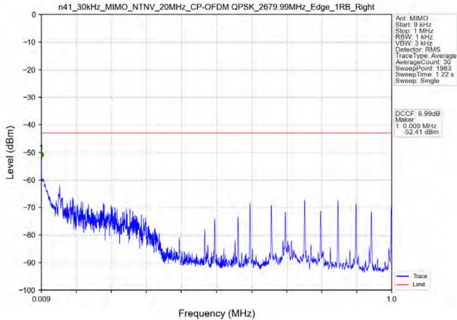
n41_30kHz_MIMO_NTNV_20MHz_CP-OFDM QPSK_2679.99MHz_Edge_1RB_Right
