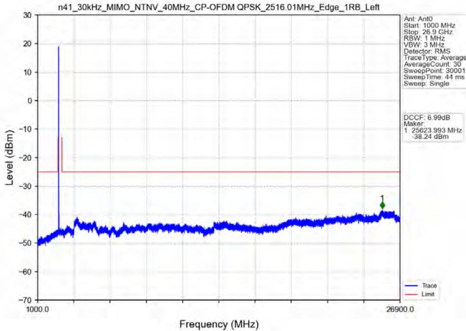
n41_30kHz_MIMO_NTNV_40MHz_CP-OFDM QPSK_2516.01MHz_Edge_1RB_Left
