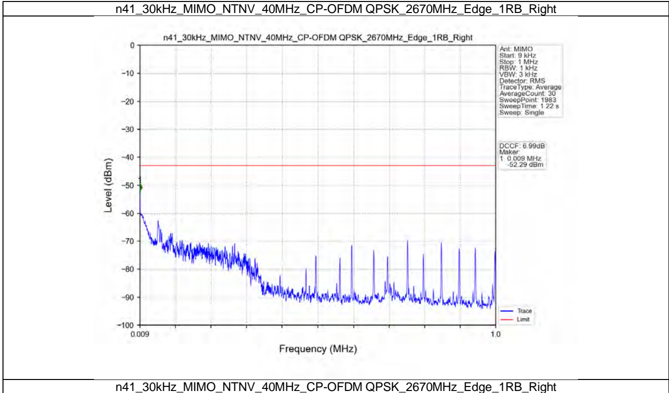
n41_30kHz_MIMO_NTNV_40MHz_CP-OFDM QPSK_2670MHz_Edge_1RB_Right
