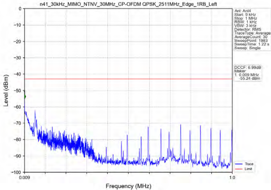
n41_30kHz_MIMO_NTNV_30MHz_CP-OFDM QPSK_2511MHz_Edge_1RB_Left
