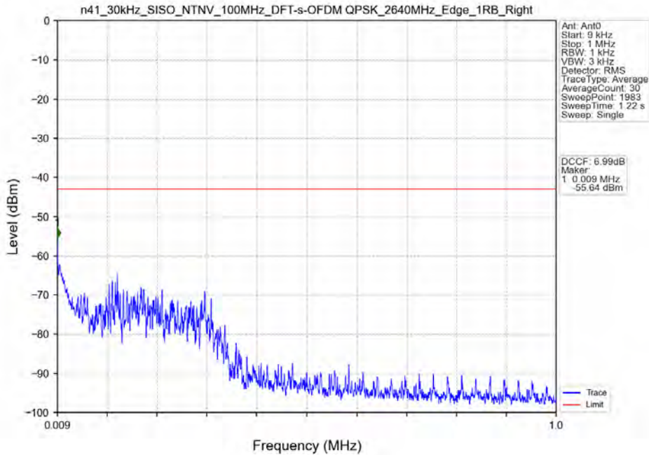
n41_30kHz_SISO_NTNV_100MHz_DFT-s-OFDM_QPSK_2640MHz_Edge_1RB_Right
