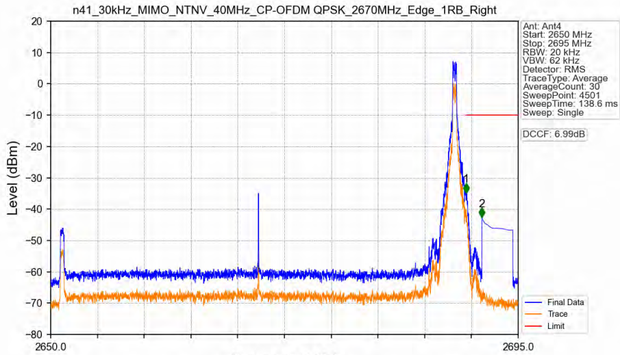
n41_30kHz_MIMO_NTNV_40MHz_CP-OFDM QPSK_2670MHz_Edge_1RB_Right
