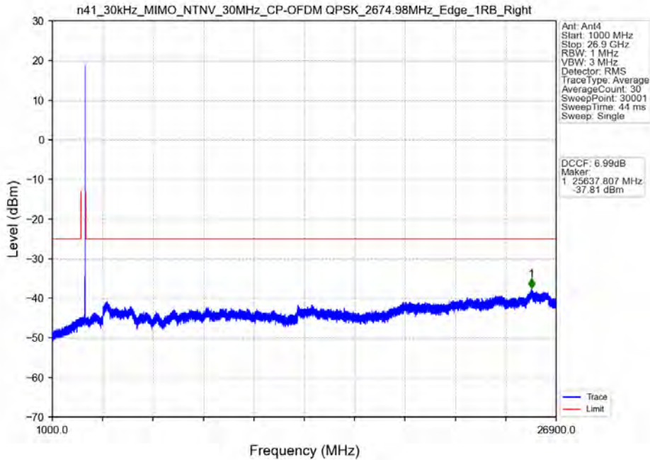
n41_30kHz_MIMO_NTNV_30MHz_CP-OFDM QPSK_2674.98MHz_Edge_1RB_Right
