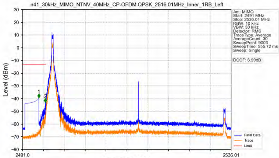
n41_30kHz_MIMO_NTNV_40MHz_CP-OFDM QPSK_2516.01MHz_Inner_1RB_Left
