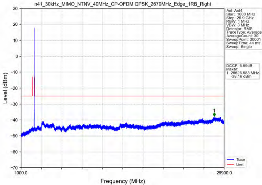
n41_30kHz_MIMO_NTNV_40MHz_CP-OFDM QPSK_2670MHz_Edge_1RB_Right
