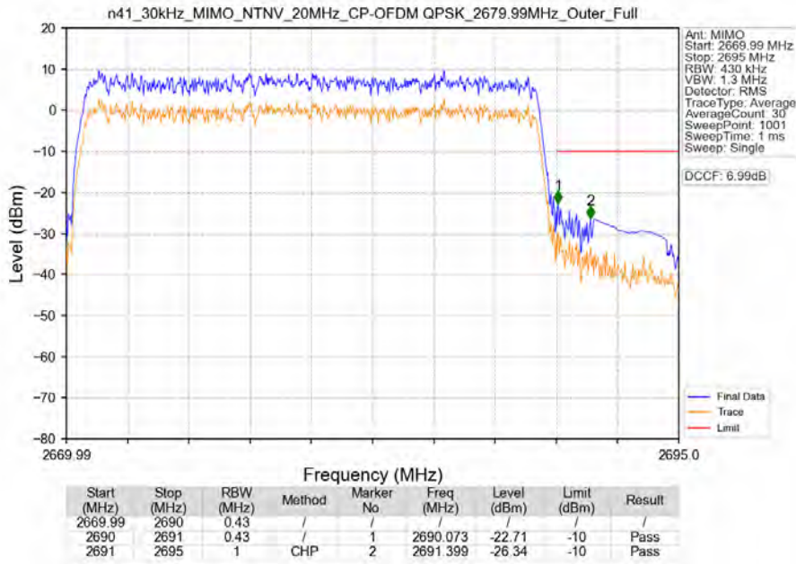
n41_30kHz_MIMO_NTNV_20MHz_CP-OFDM_QPSK_2679.99MHz_Outer_Full
