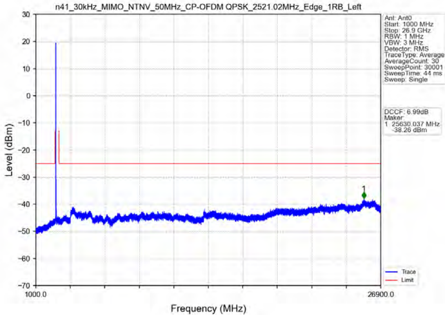
n41_30kHz_MIMO_NTNV_50MHz_CP-OFDM QPSK_2521.02MHz_Edge_1RB_Left
