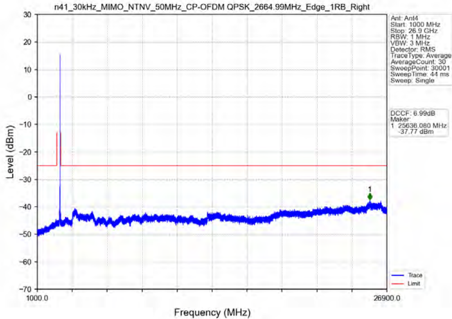
n41_30kHz_MIMO_NTNV_50MHz_CP-OFDM QPSK_2664.99MHz_Edge_1RB_Right
