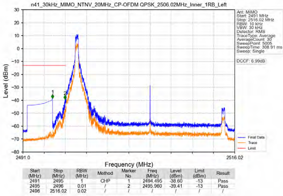
n41_30kHz_MIMO_NTNV_20MHz_CP-OFDM QPSK_2506.02MHz_Inner_1RB_Left
