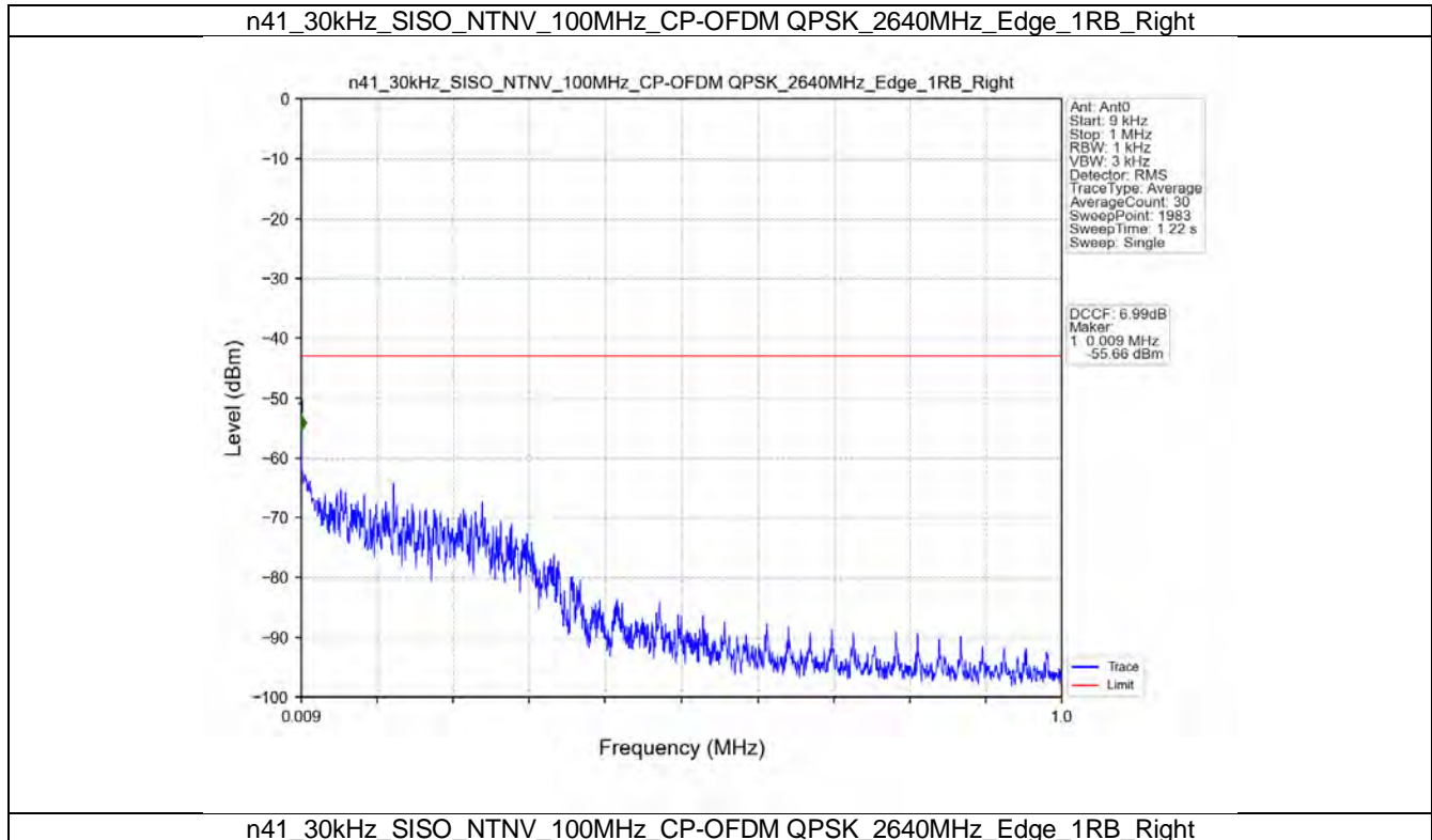
n41_30kHz_SISO_NTNV_100MHz_CP-OFDM QPSK_2640MHz_Edge_1RB_Right
