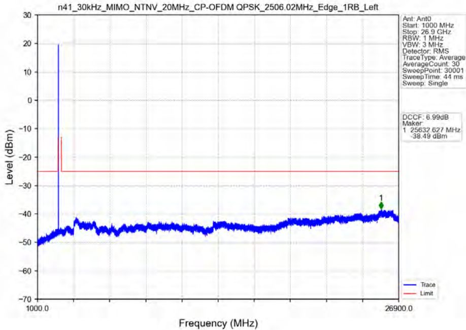
n41_30kHz_MIMO_NTNV_20MHz_CP-OFDM QPSK_2506.02MHz_Edge_1RB_Left
