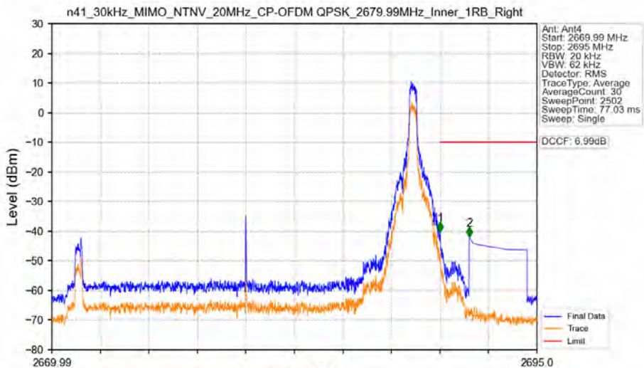
n41_30kHz_MIMO_NTNV_20MHz_CP-OFDM QPSK_2679.99MHz_Inner_1RB_Right
