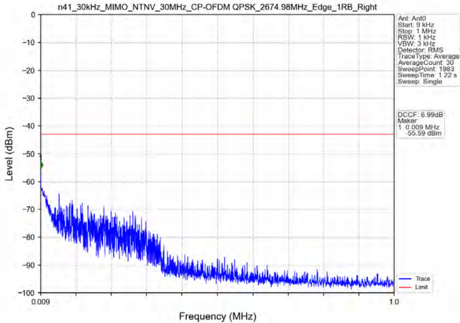
n41_30kHz_MIMO_NTNV_30MHz_CP-OFDM QPSK_2674.98MHz_Edge_1RB_Right
