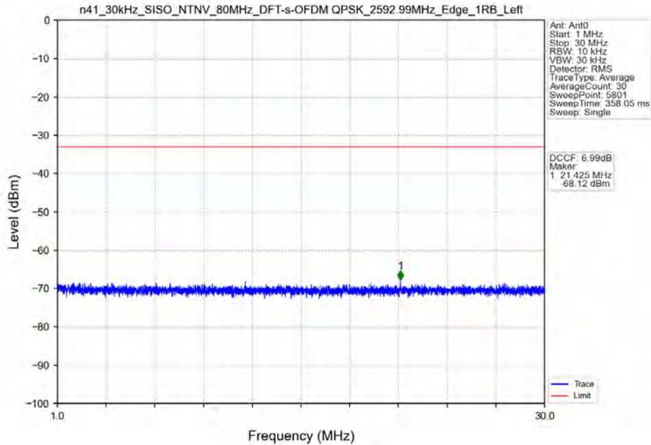
n41_30kHz_SISO_NTNV_80MHz_DFT-s-OFDM_QPSK_2592.99MHz_Edge_1RB_Left
