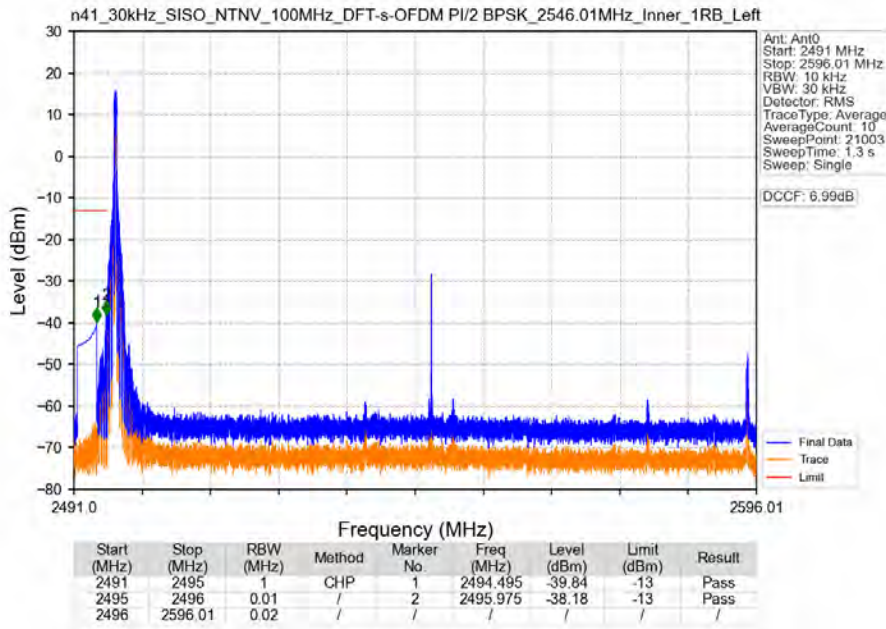
n41_30kHz_SISO_NTNV_100MHz_DFT-s-OFDM PI/2 BPSK_2546.01MHz_Inner_1RB_Left
