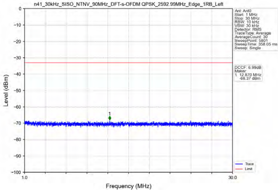
n41_30kHz_SISO_NTNV_90MHz_DFT-s-OFDM QPSK_2592.99MHz_Edge_1RB_Left
