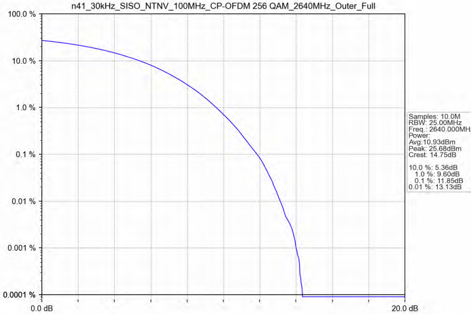
n41_30kHz_SISO_NTNV_100MHz_CP-OFDM 256 QAM_2640MHz_Outer_Full
