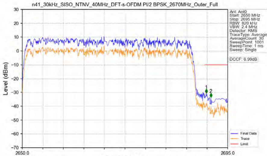
n41_30kHz_SISO_NTNV_40MHz_DFT-s-OFDM PI/2 BPSK_2670MHz_Outer_Full
