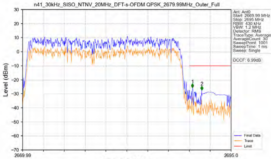
n41_30kHz_SISO_NTNV_20MHz_DFT-s-OFDM_QPSK_2679.99MHz_Outer_Full
