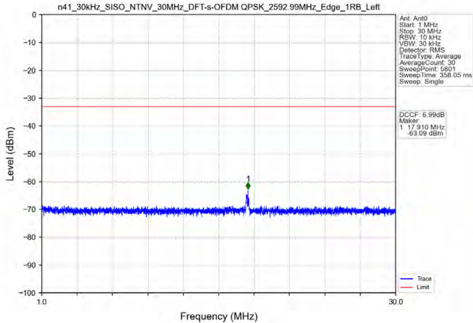
n41_30kHz_SISO_NTNV_30MHz_DFT-s-OFDM_QPSK_2592.99MHz_Edge_1RB_Left
