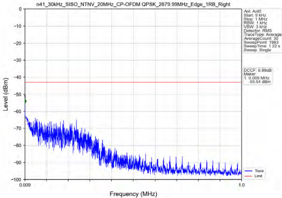
n41_30kHz_SISO_NTNV_20MHz_CP-OFDM QPSK_2679.99MHz_Edge_1RB_Right
