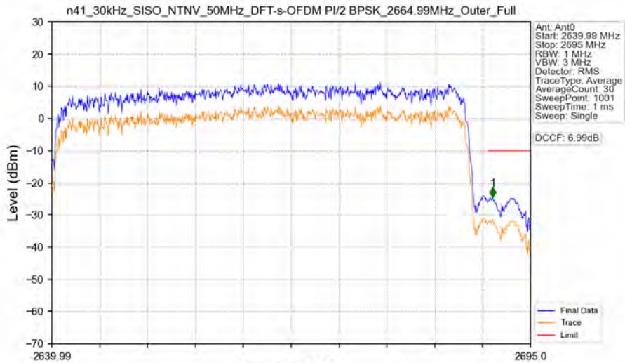
n41_30kHz_SISO_NTNV_50MHz_DFT-s-OFDM PI/2 BPSK_2664.99MHz_Outer_Full
