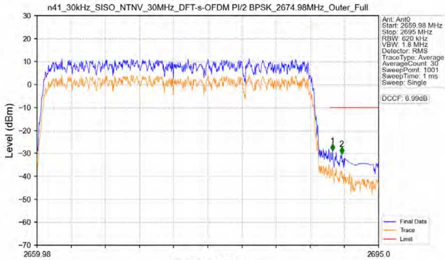
n41_30kHz_SISO_NTNV_30MHz_DFT-s-OFDM PI/2 BPSK_2674.98MHz_Outer_Full
