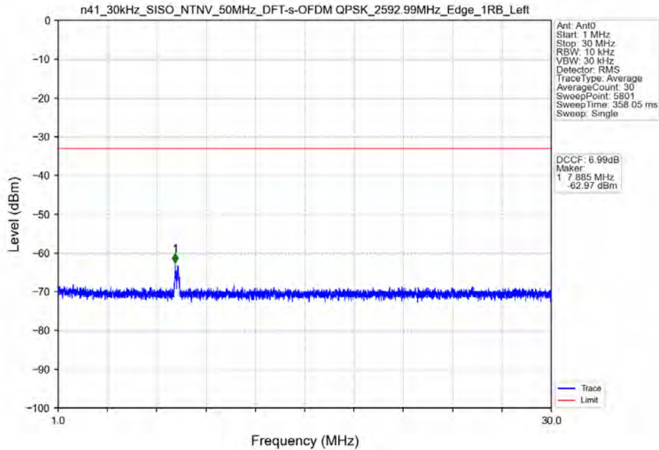
n41_30kHz_SISO_NTNV_50MHz_DFT-s-OFDM_QPSK_2592.99MHz_Edge_1RB_Left
