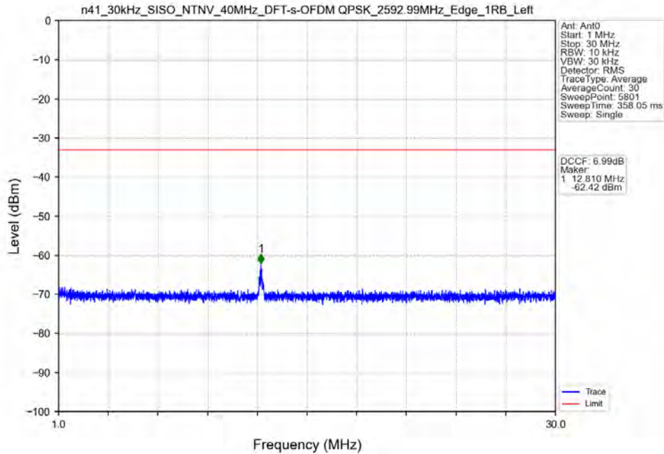
n41_30kHz_SISO_NTNV_40MHz_DFT-s-OFDM_QPSK_2592.99MHz_Edge_1RB_Left
