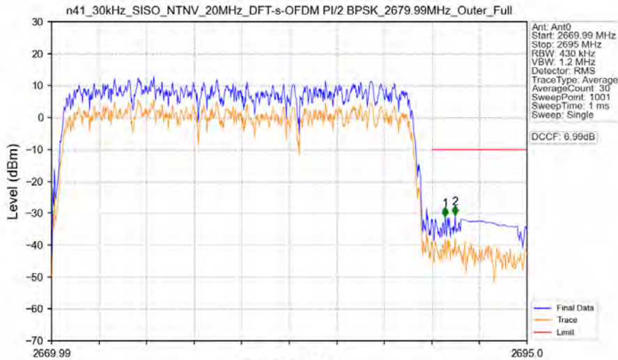
n41_30kHz_SISO_NTNV_20MHz_DFT-s-OFDM PI/2 BPSK_2679.99MHz_Outer_Full
