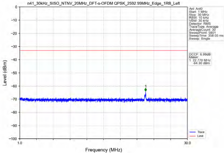
n41_30kHz_SISO_NTNV_20MHz_DFT-s-OFDM QPSK_2592.99MHz_Edge_1RB_Left
