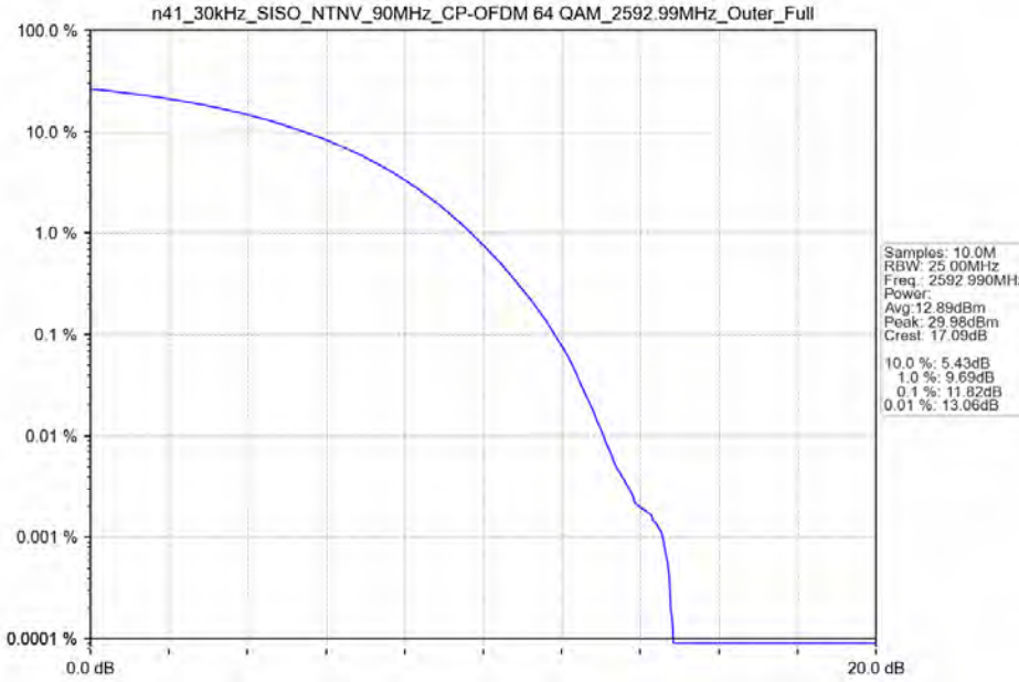
n41_30kHz_SISO_NTNV_90MHz_CP-OFDM 64 QAM_2592.99MHz_Outer_Full
