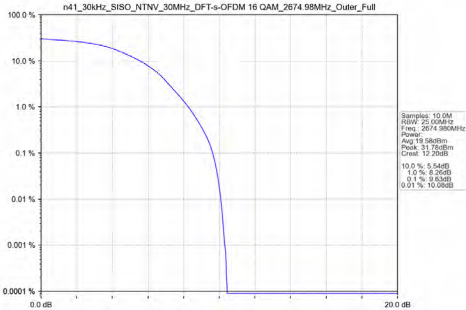
n41_30kHz_SISO_NTNV_30MHz_DFT-s-OFDM 16 QAM_2674.98MHz_Outer_Full
