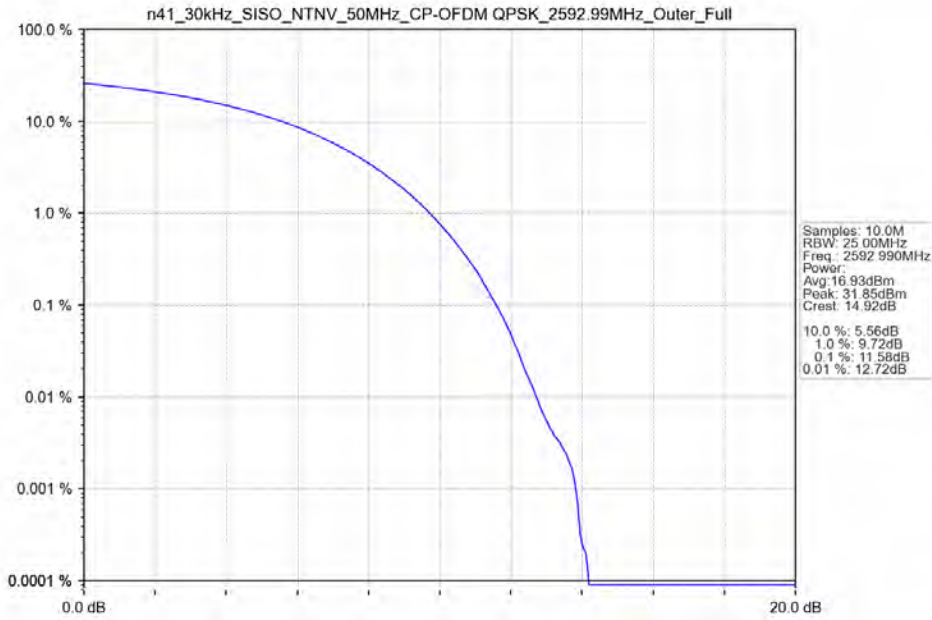
n41_30kHz_SISO_NTNV_50MHz_CP-OFDM QPSK_2592.99MHz_Outer_Full
