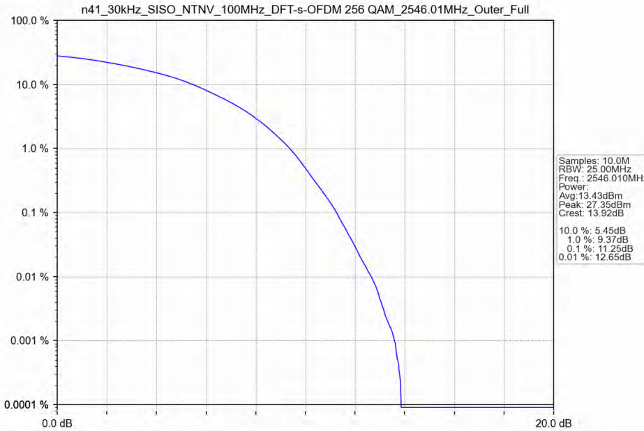
n41_30kHz_SISO_NTNV_100MHz_DFT-s-OFDM_256_QAM_2546.01MHz_Outer_Full
