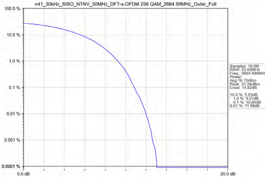
n41_30kHz_SISO_NTNV_50MHz_DFT-s-OFDM 256 QAM_2664.99MHz_Outer_Full
