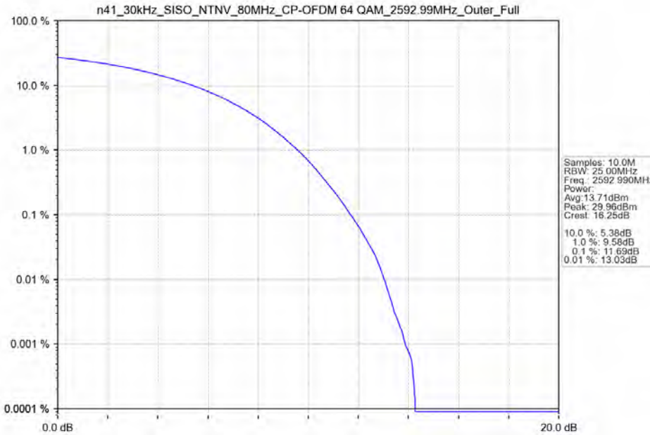
n41_30kHz_SISO_NTNV_80MHz_CP-OFDM 64 QAM_2592.99MHz_Outer_Full
