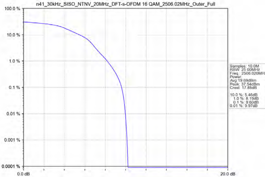
n41_30kHz_SISO_NTNV_20MHz_DFT-s-OFDM_16_QAM_2506.02MHz_Outer_Full
