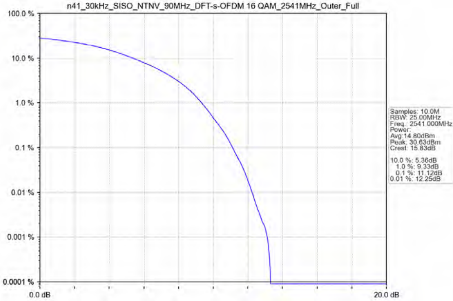
n41_30kHz_SISO_NTNV_90MHz_DFT-s-OFDM 16 QAM_2541MHz_Outer_Full
