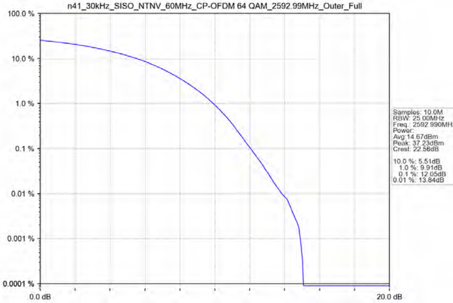
n41_30kHz_SISO_NTNV_60MHz_CP-OFDM 64 QAM_2592.99MHz_Outer_Full
