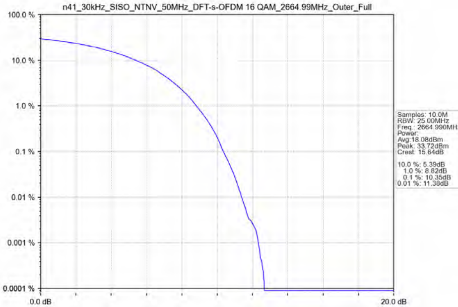
n41_30kHz_SISO_NTNV_50MHz_DFT-s-OFDM 16 QAM_2664.99MHz_Outer_Full
