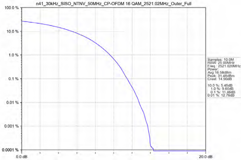
n41_30kHz_SISO_NTNV_50MHz_CP-OFDM 16 QAM_2521.02MHz_Outer_Full
