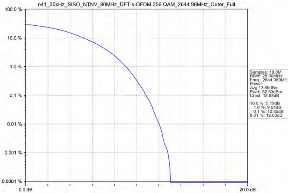
n41_30kHz_SISO_NTNV_90MHz_DFT-s-OFDM 256 QAM_2644.98MHz_Outer_Full
