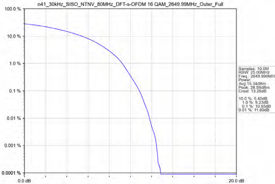
n41_30kHz_SISO_NTNV_80MHz_DFT-s-OFDM 16 QAM_2649.99MHz_Outer_Full
