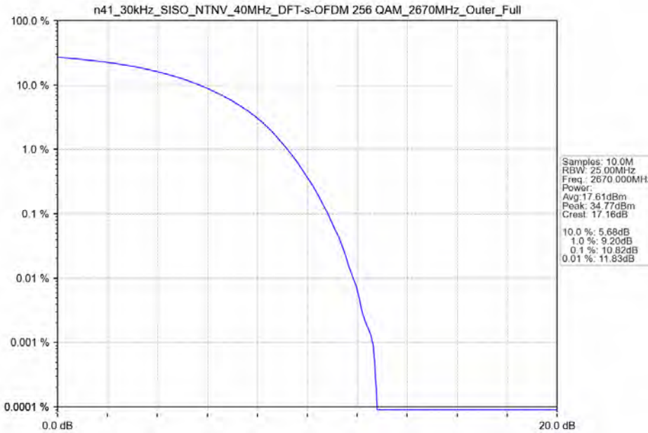
n41_30kHz_SISO_NTNV_40MHz_DFT-s-OFDM 256 QAM_2670MHz_Outer_Full
