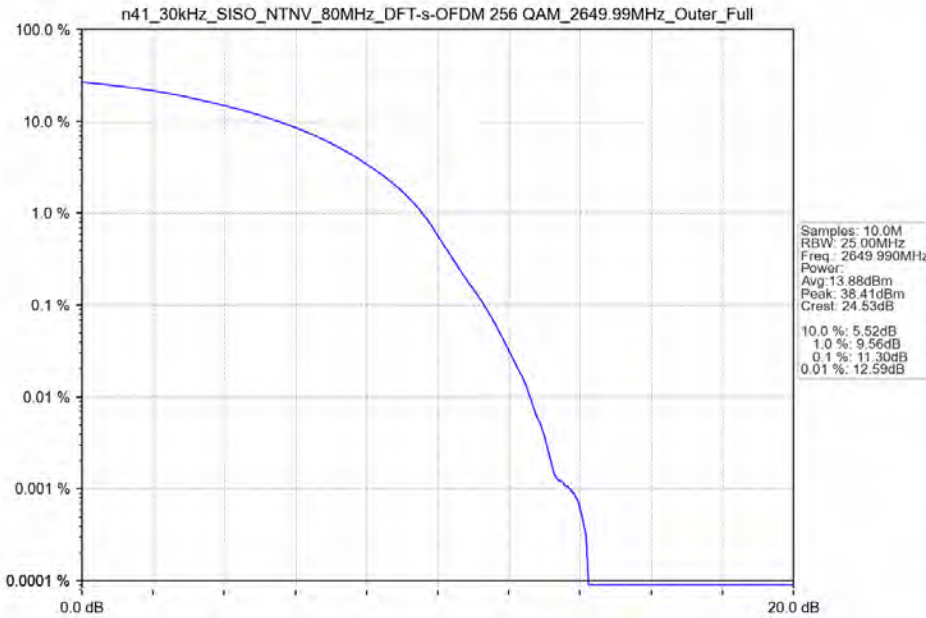
n41_30kHz_SISO_NTNV_80MHz_DFT-s-OFDM 256 QAM_2649.99MHz_Outer_Full
