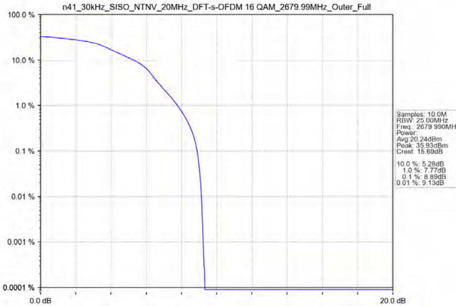
n41_30kHz_SISO_NTNV_20MHz_DFT-s-OFDM 16 QAM_2679.99MHz_Outer_Full
