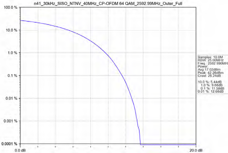
n41_30kHz_SISO_NTNV_40MHz_CP-OFDM 64 QAM_2592.99MHz_Outer_Full
