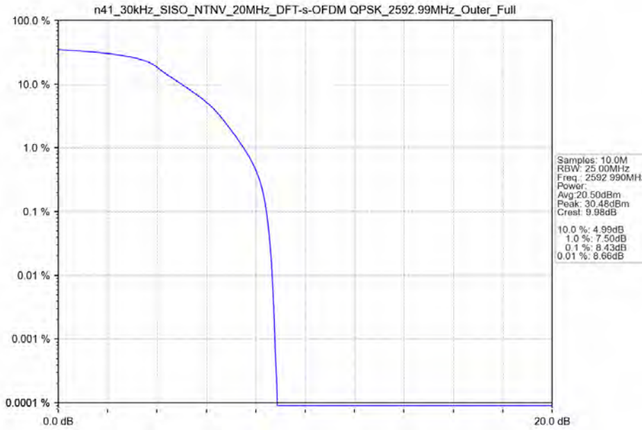
n41_30kHz_SISO_NTNV_20MHz_DFT-s-OFDM QPSK_2592.99MHz_Outer_Full
