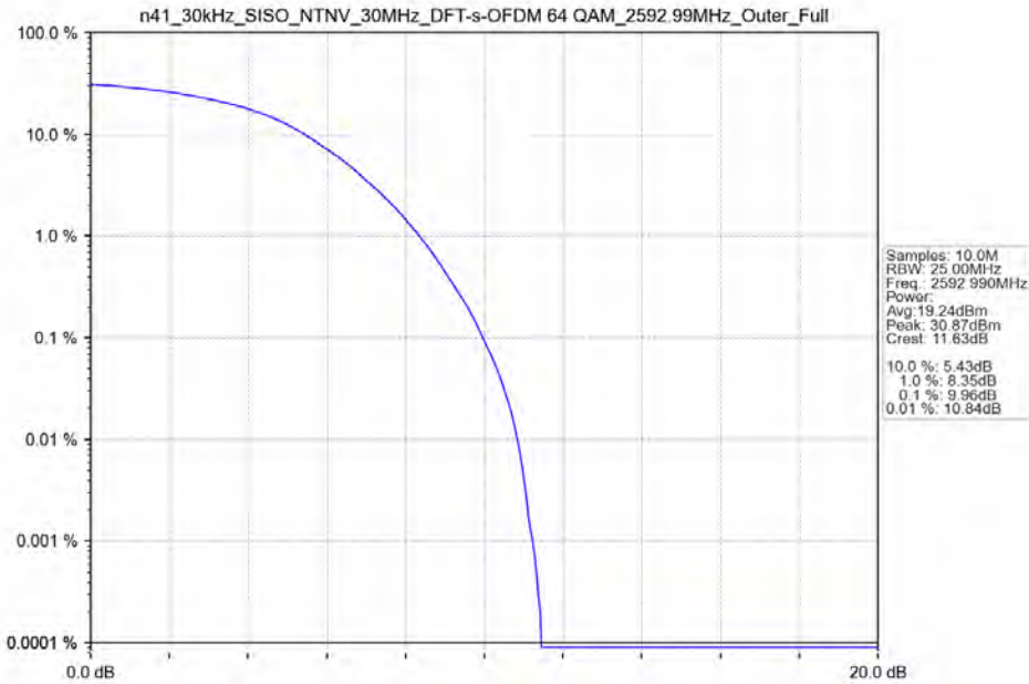
n41_30kHz_SISO_NTNV_30MHz_DFT-s-OFDM 64 QAM_2592.99MHz_Outer_Full
