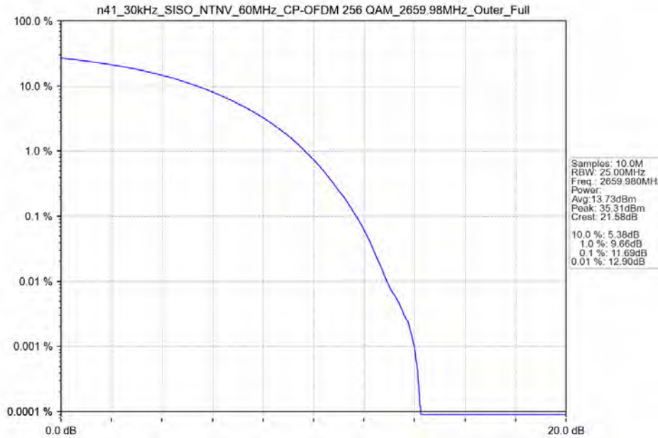
n41_30kHz_SISO_NTNV_60MHz_CP-OFDM 256 QAM_2659.98MHz_Outer_Full
