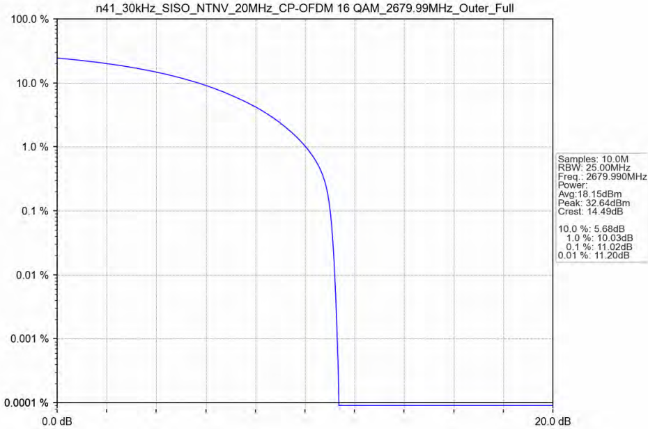
n41_30kHz_SISO_NTNV_20MHz_CP-OFDM 16 QAM_2679.99MHz_Outer_Full
