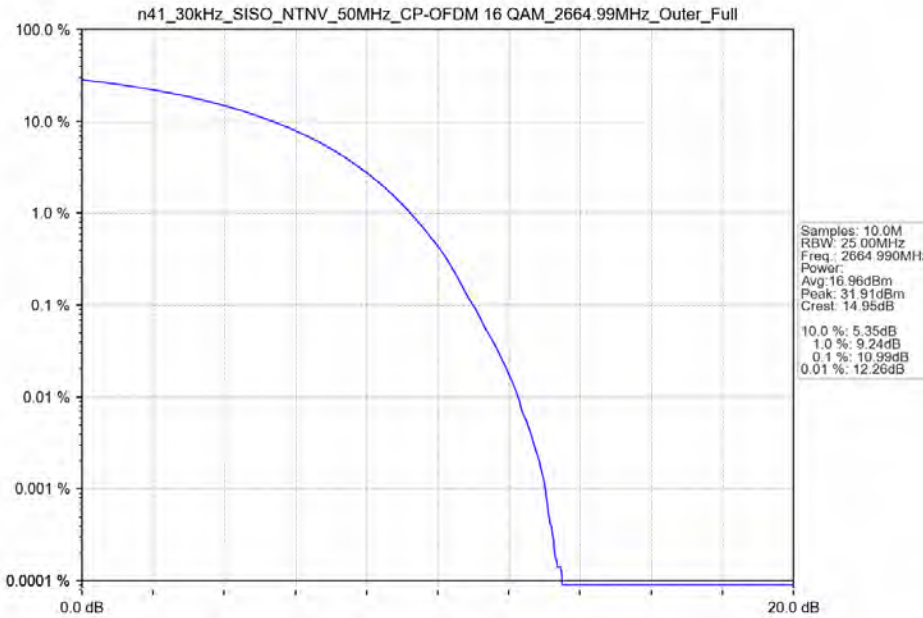
n41_30kHz_SISO_NTNV_50MHz_CP-OFDM 16 QAM_2664.99MHz_Outer_Full
