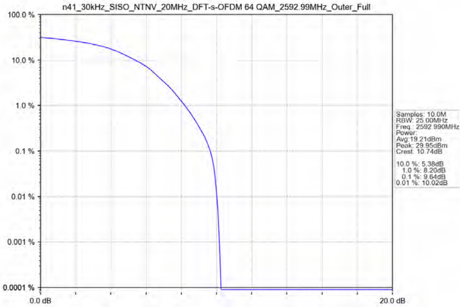
n41_30kHz_SISO_NTNV_20MHz_DFT-s-OFDM 64 QAM_2592.99MHz_Outer_Full
