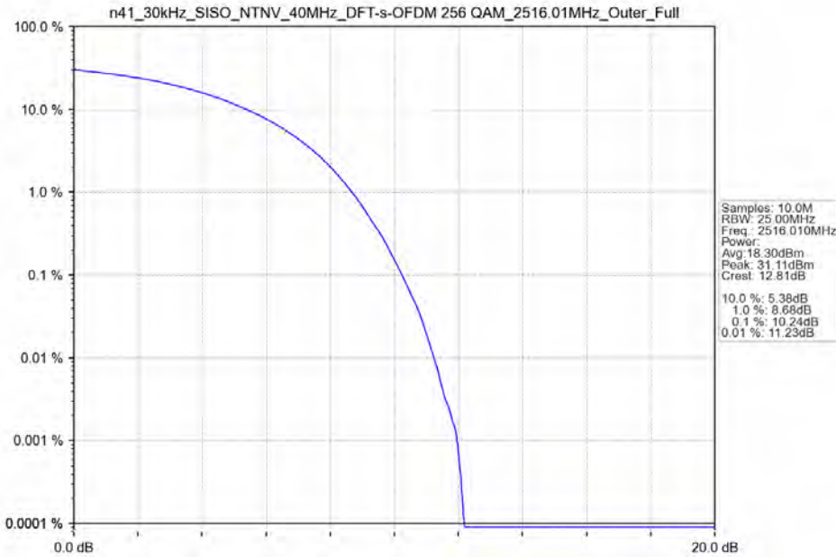
n41_30kHz_SISO_NTNV_40MHz_DFT-s-OFDM_256_QAM_2516.01MHz_Outer_Full
