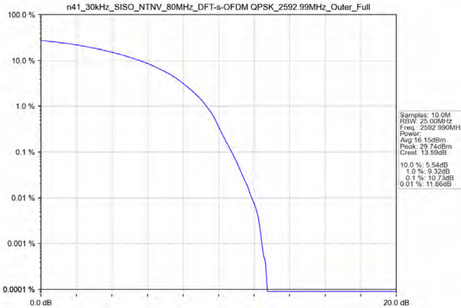
n41_30kHz_SISO_NTNV_80MHz_DFT-s-OFDM QPSK_2592.99MHz_Outer_Full
