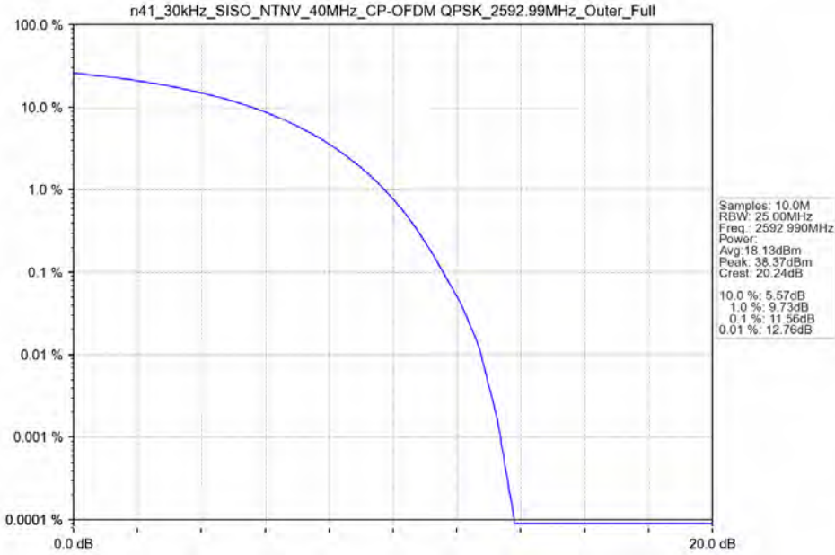
n41_30kHz_SISO_NTNV_40MHz_CP-OFDM QPSK_2592.99MHz_Outer_Full
