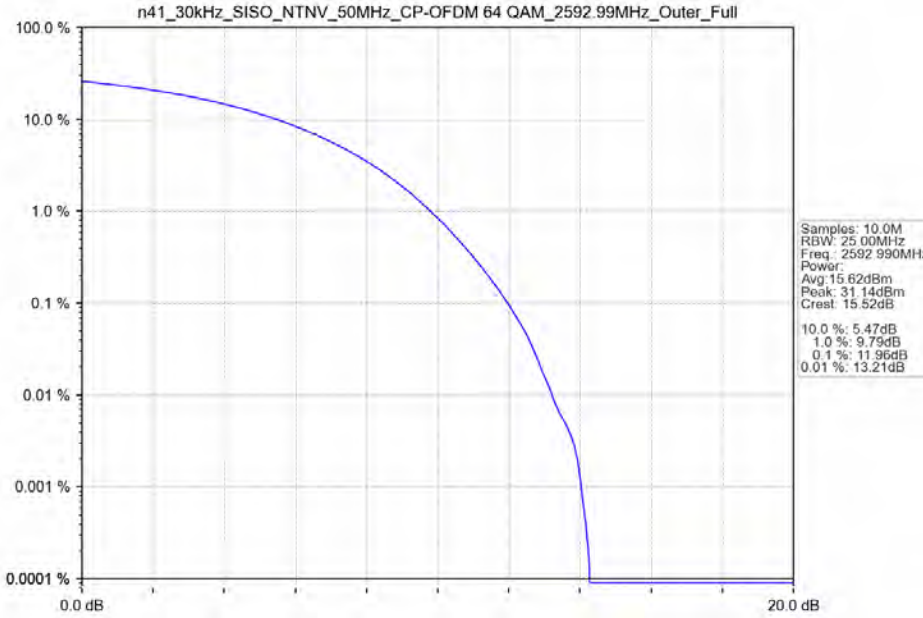
n41_30kHz_SISO_NTNV_50MHz_CP-OFDM 64 QAM_2592.99MHz_Outer_Full
