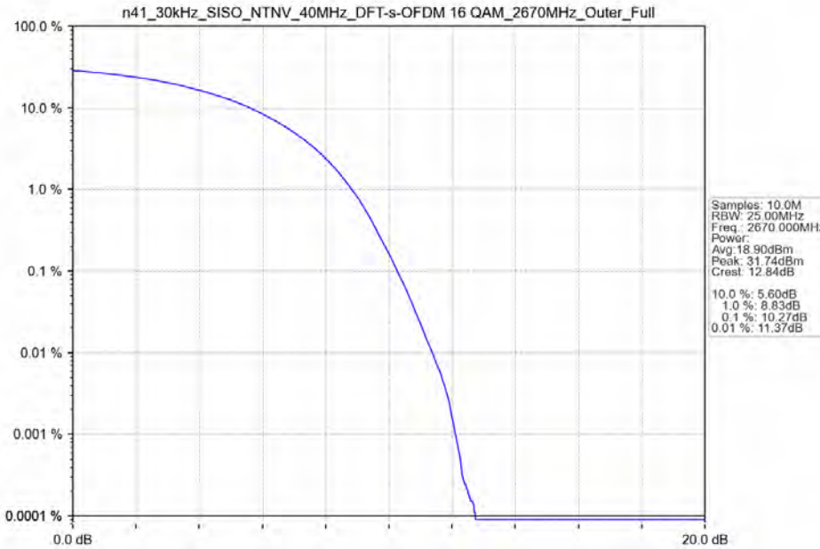
n41_30kHz_SISO_NTNV_40MHz_DFT-s-OFDM 16 QAM_2670MHz_Outer_Full
