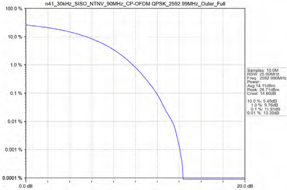
n41_30kHz_SISO_NTNV_90MHz_CP-OFDM QPSK_2592.99MHz_Outer_Full
