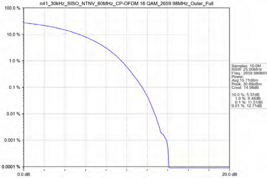
n41_30kHz_SISO_NTNV_60MHz_CP-OFDM 16 QAM_2659.98MHz_Outer_Full
