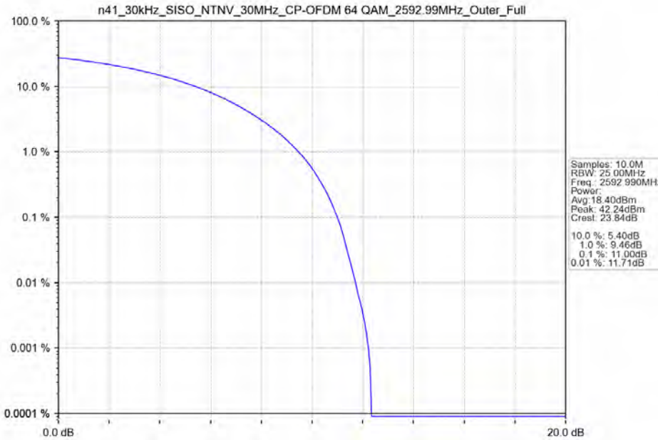
n41_30kHz_SISO_NTNV_30MHz_CP-OFDM 64 QAM_2592.99MHz_Outer_Full
