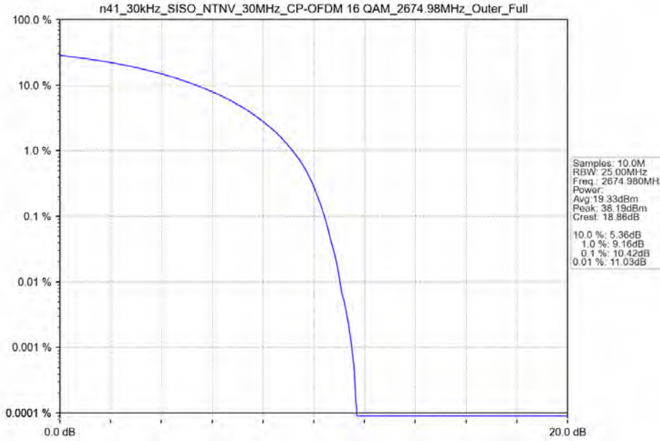
n41_30kHz_SISO_NTNV_30MHz_CP-OFDM 16 QAM_2674.98MHz_Outer_Full
