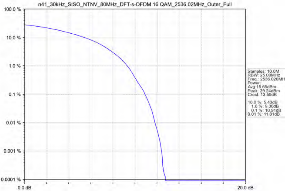
n41_30kHz_SISO_NTNV_80MHz_DFT-s-OFDM_16_QAM_2536.02MHz_Outer_Full
