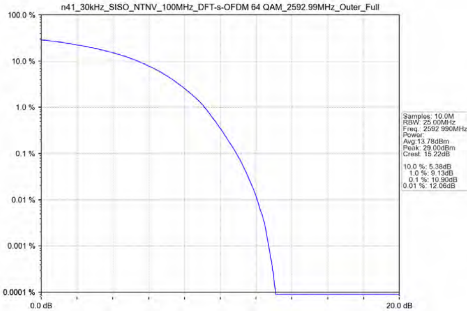
n41_30kHz_SISO_NTNV_100MHz_DFT-s-OFDM 64 QAM_2592.99MHz_Outer_Full
