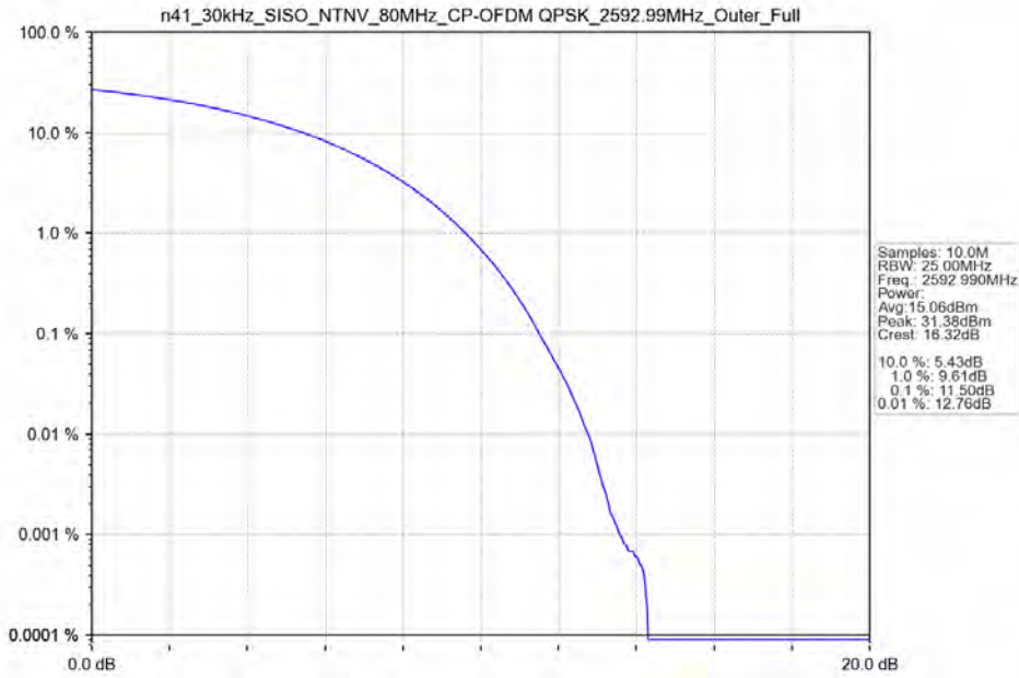
n41_30kHz_SISO_NTNV_80MHz_CP-OFDM QPSK_2592.99MHz_Outer_Full
