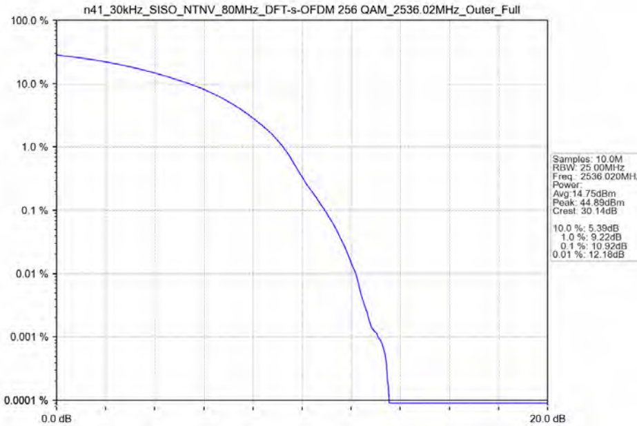
n41_30kHz_SISO_NTNV_80MHz_DFT-s-OFDM_256_QAM_2536.02MHz_Outer_Full
