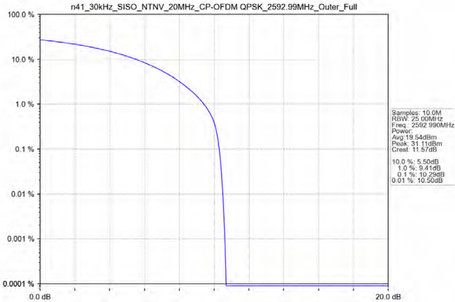
n41_30kHz_SISO_NTNV_20MHz_CP-OFDM QPSK_2592.99MHz_Outer_Full
