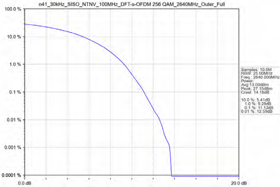
n41_30kHz_SISO_NTNV_100MHz_DFT-s-OFDM 256 QAM_2640MHz_Outer_Full
