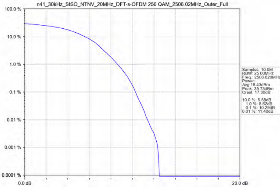
n41_30kHz_SISO_NTNV_20MHz_DFT-s-OFDM_256_QAM_2506.02MHz_Outer_Full
