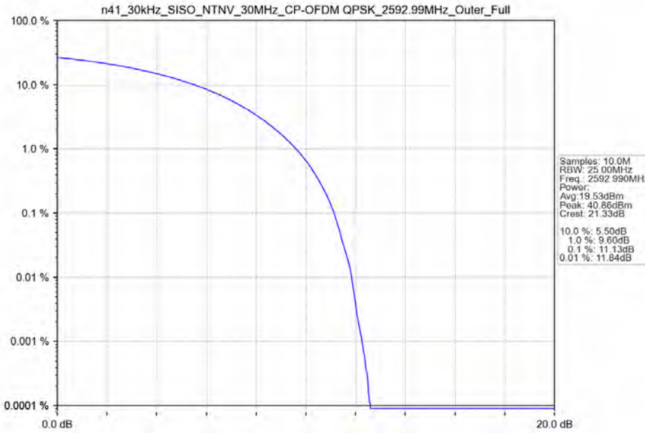
n41_30kHz_SISO_NTNV_30MHz_CP-OFDM QPSK_2592.99MHz_Outer_Full
