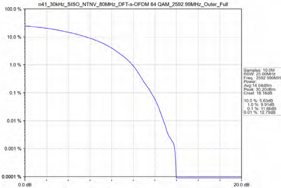
n41_30kHz_SISO_NTNV_80MHz_DFT-s-OFDM 64 QAM_2592.99MHz_Outer_Full
