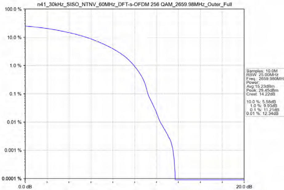
n41_30kHz_SISO_NTNV_60MHz_DFT-s-OFDM 256 QAM_2659.98MHz_Outer_Full
