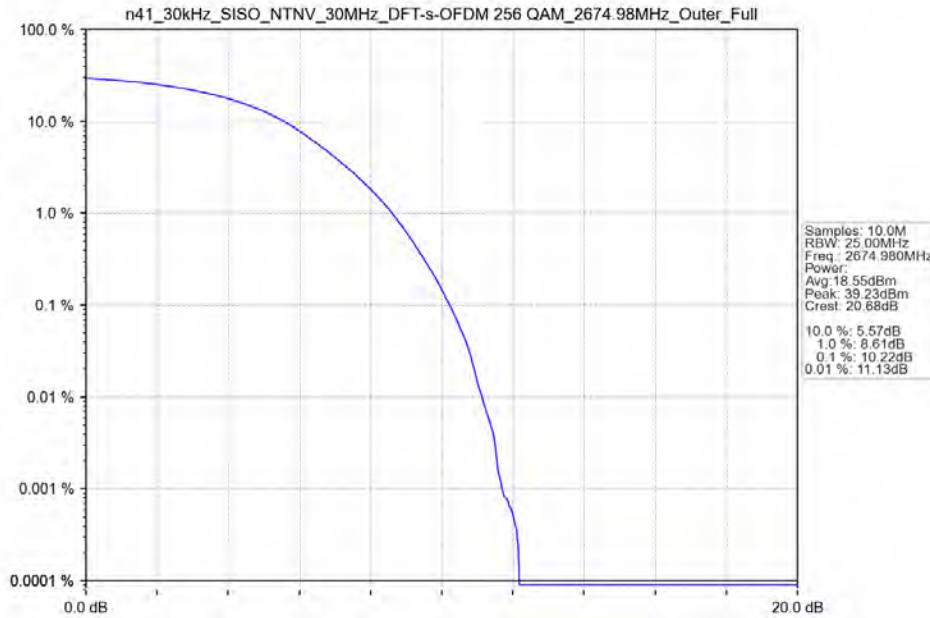
n41_30kHz_SISO_NTNV_30MHz_DFT-s-OFDM 256 QAM_2674.98MHz_Outer_Full
