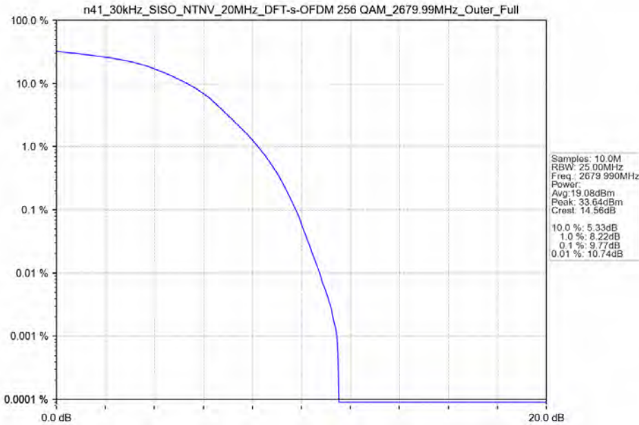
n41_30kHz_SISO_NTNV_20MHz_DFT-s-OFDM 256 QAM_2679.99MHz_Outer_Full
