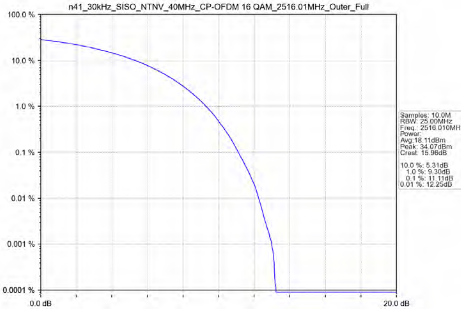
n41_30kHz_SISO_NTNV_40MHz_CP-OFDM 16 QAM_2516.01MHz_Outer_Full
