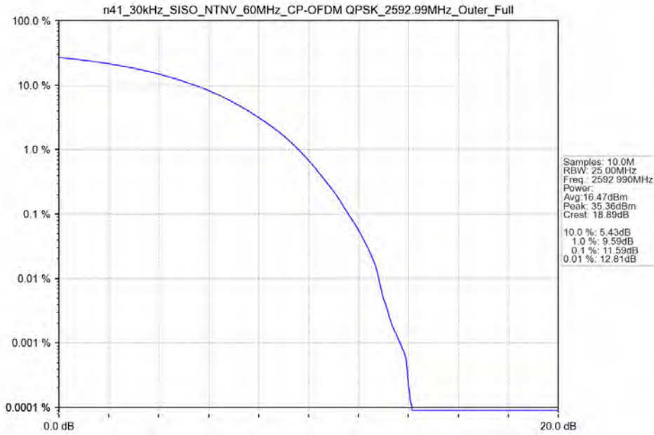
n41_30kHz_SISO_NTNV_60MHz_CP-OFDM QPSK_2592.99MHz_Outer_Full
