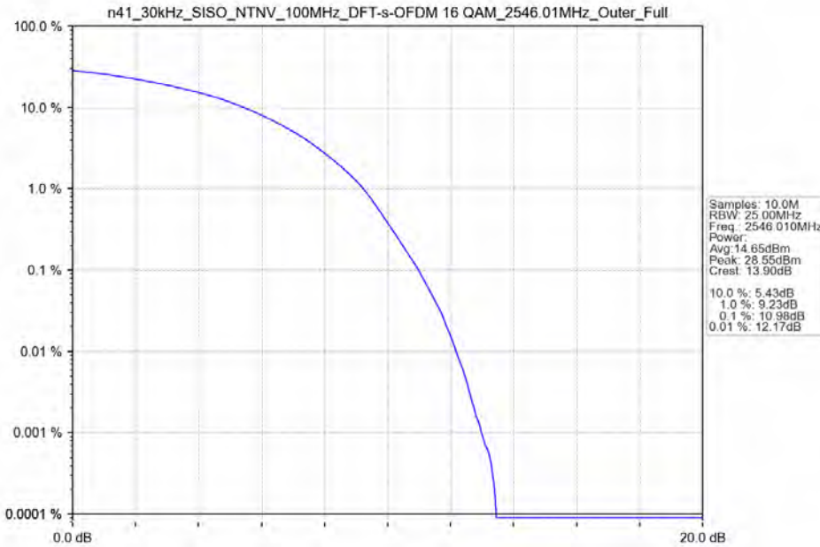
n41_30kHz_SISO_NTNV_100MHz_DFT-s-OFDM_16_QAM_2546.01MHz_Outer_Full
