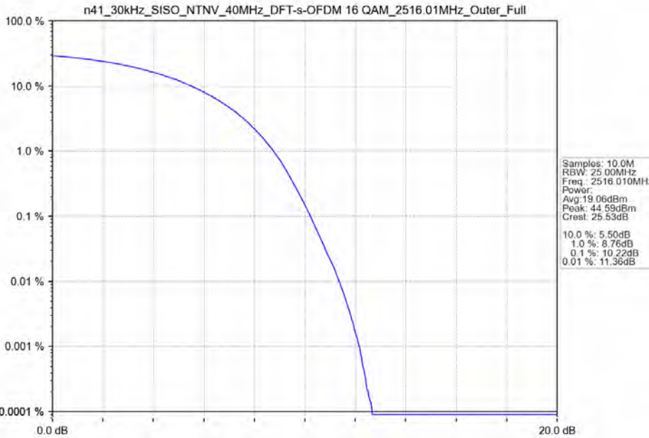
n41_30kHz_SISO_NTNV_40MHz_DFT-s-OFDM_16_QAM_2516.01MHz_Outer_Full
