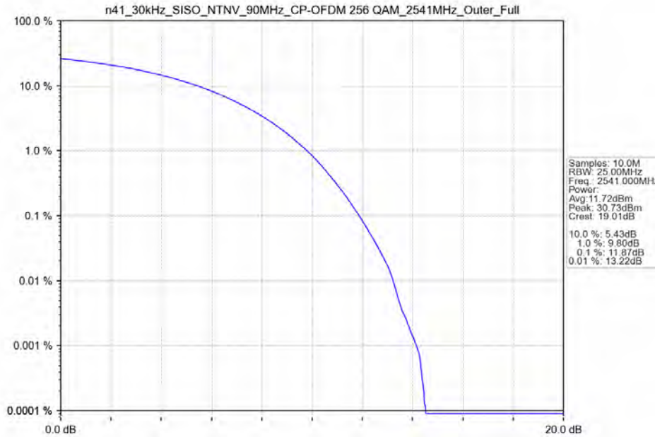
n41_30kHz_SISO_NTNV_90MHz_CP-OFDM 256 QAM_2541MHz_Outer_Full
