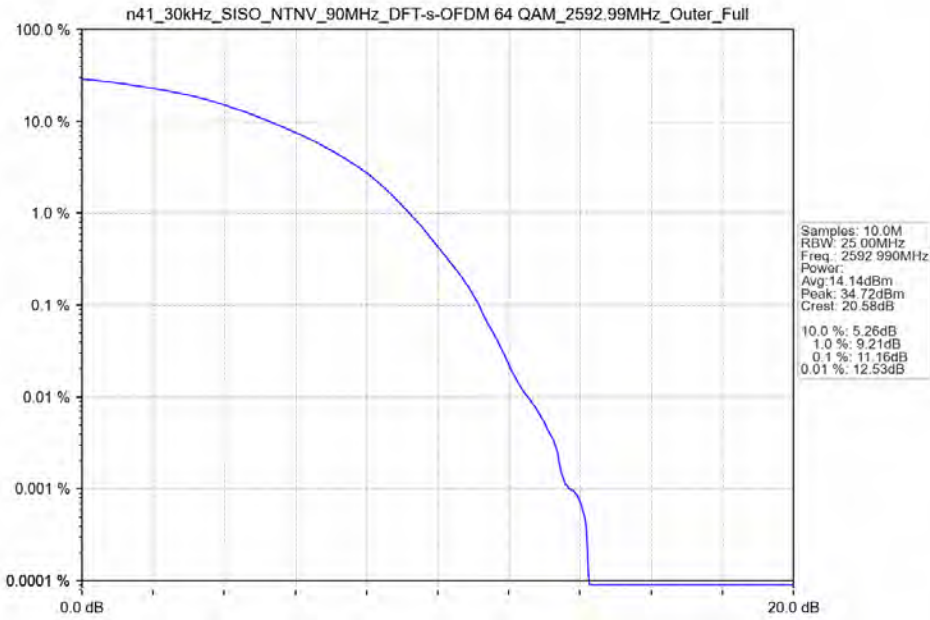
n41_30kHz_SISO_NTNV_90MHz_DFT-s-OFDM 64 QAM_2592.99MHz_Outer_Full
