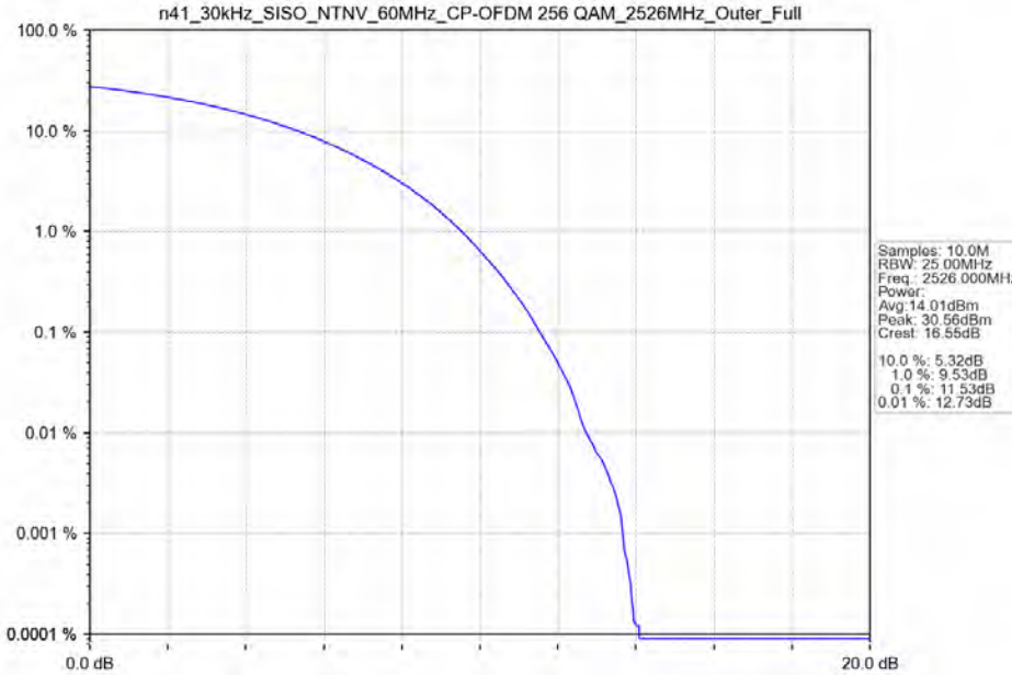
n41_30kHz_SISO_NTNV_60MHz_CP-OFDM 256 QAM_2526MHz_Outer_Full
