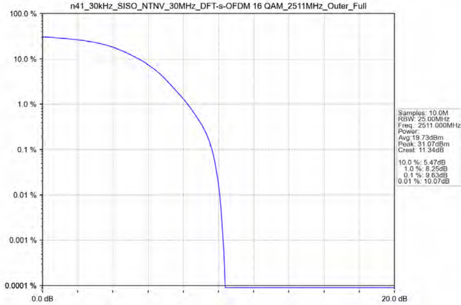
n41_30kHz_SISO_NTNV_30MHz_DFT-s-OFDM 16 QAM_2511MHz_Outer_Full
