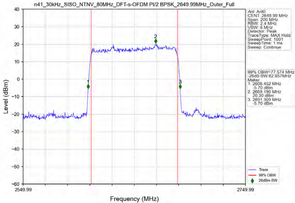
n41_30kHz_SISO_NTNV_80MHz_DFT-s-OFDM QPSK_2536.02MHz_Outer_Full
