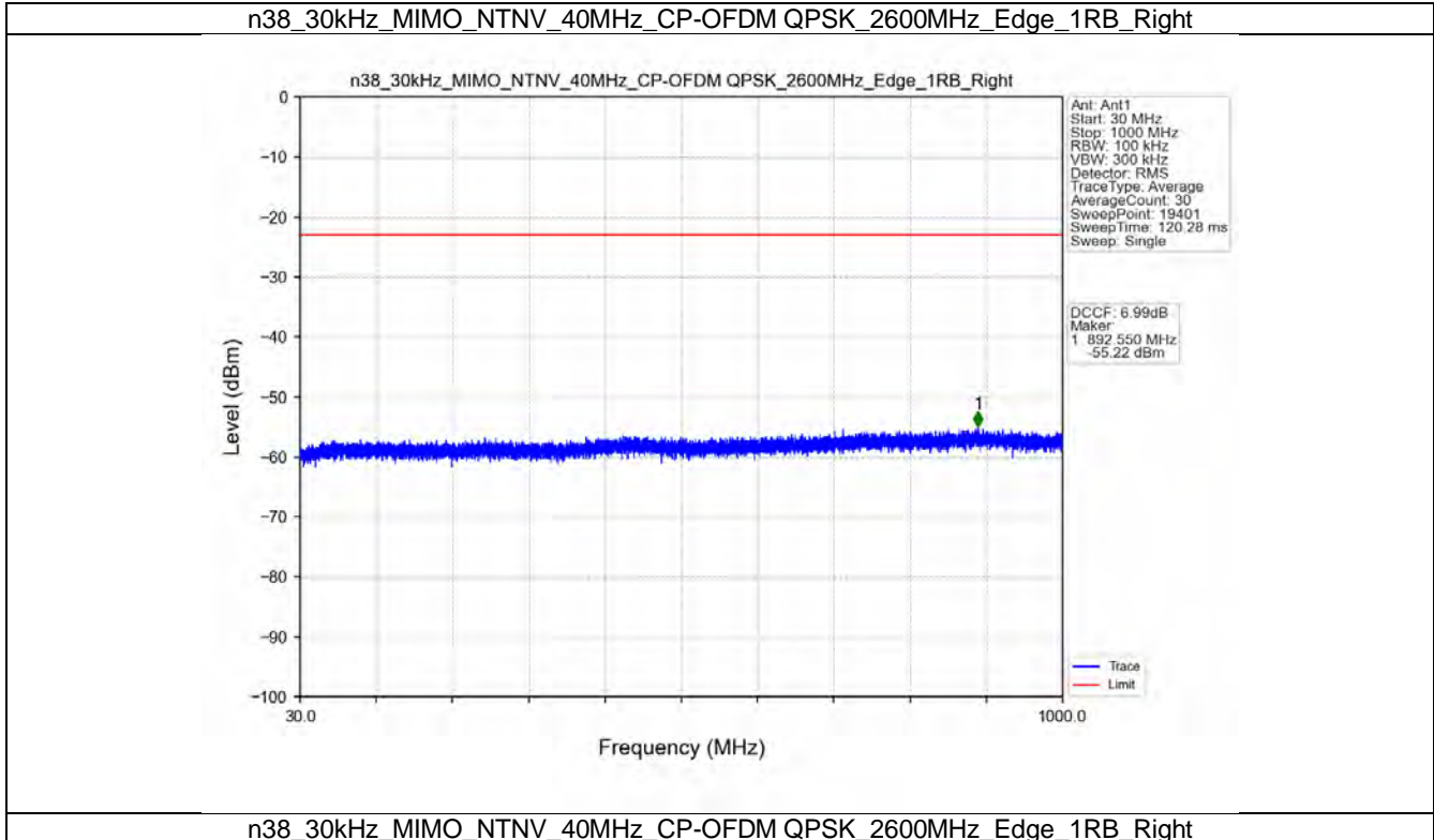
n38_30kHz_MIMO_NTNV_40MHz_CP-OFDM QPSK_2600MHz_Edge_1RB_Right
