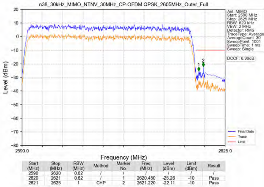
n38_30kHz_MIMO_NTNV_30MHz_CP-OFDM QPSK_2605MHz_Outer_Full
