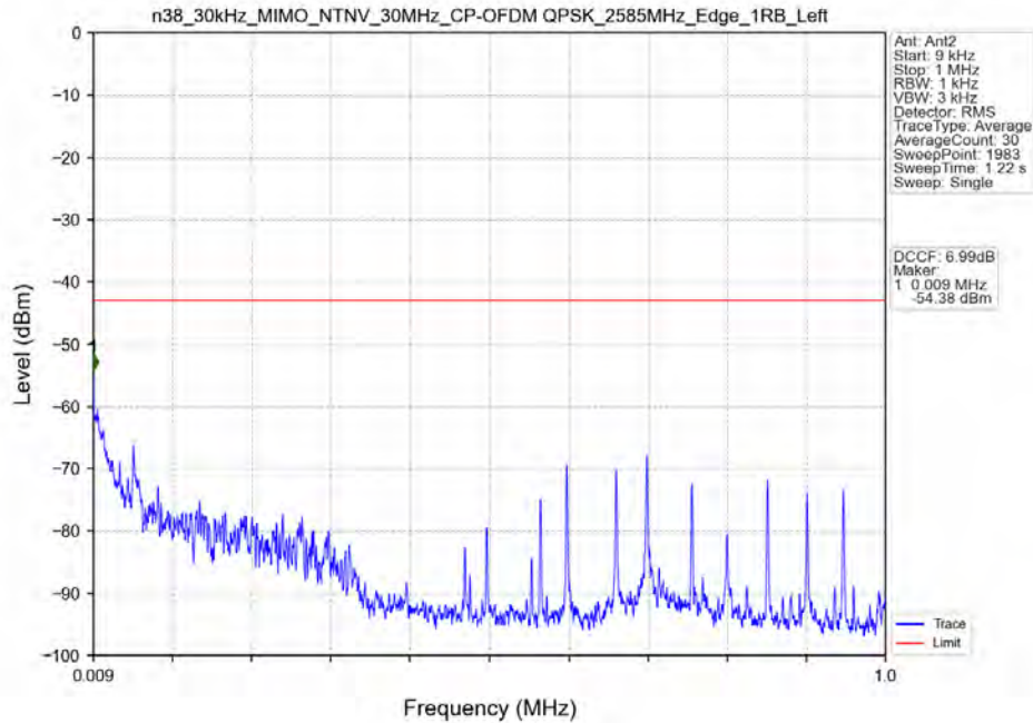
n38_30kHz_MIMO_NTNV_30MHz_CP-OFDM QPSK_2585MHz_Edge_1RB_Left
