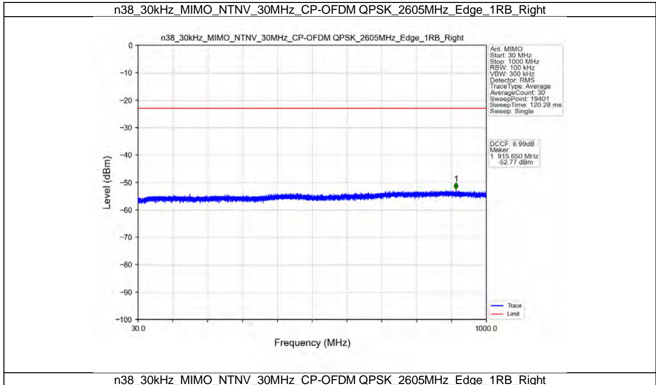
n38_30kHz_MIMO_NTNV_30MHz_CP-OFDM_QPSK_2605MHz_Edge_1RB_Right
