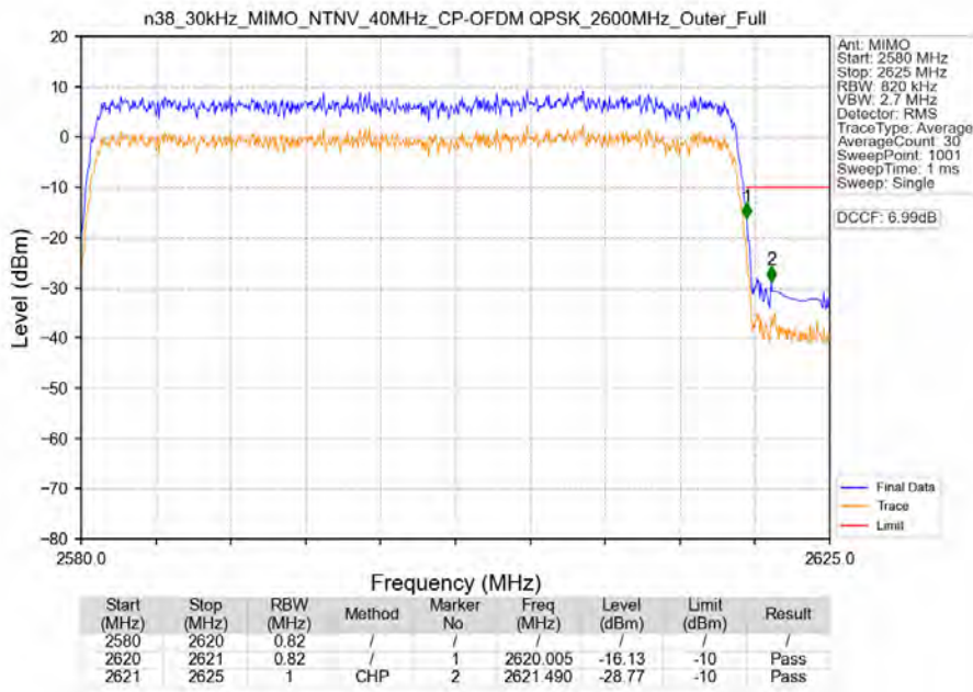
n38_30kHz_MIMO_NTNV_40MHz_CP-OFDM QPSK_2600MHz_Outer_Full
