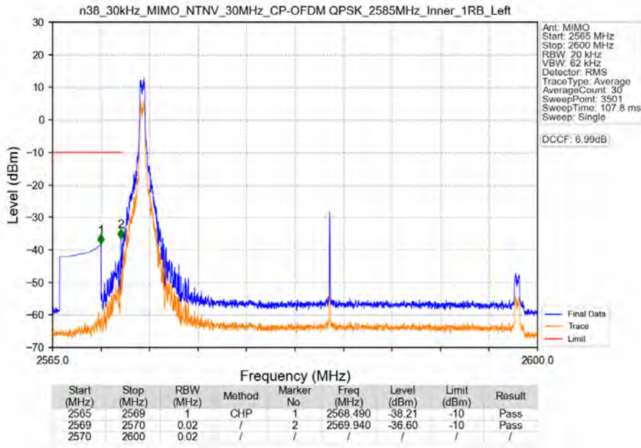
n38_30kHz_MIMO_NTNV_30MHz_CP-OFDM QPSK_2585MHz_Inner_1RB_Left
