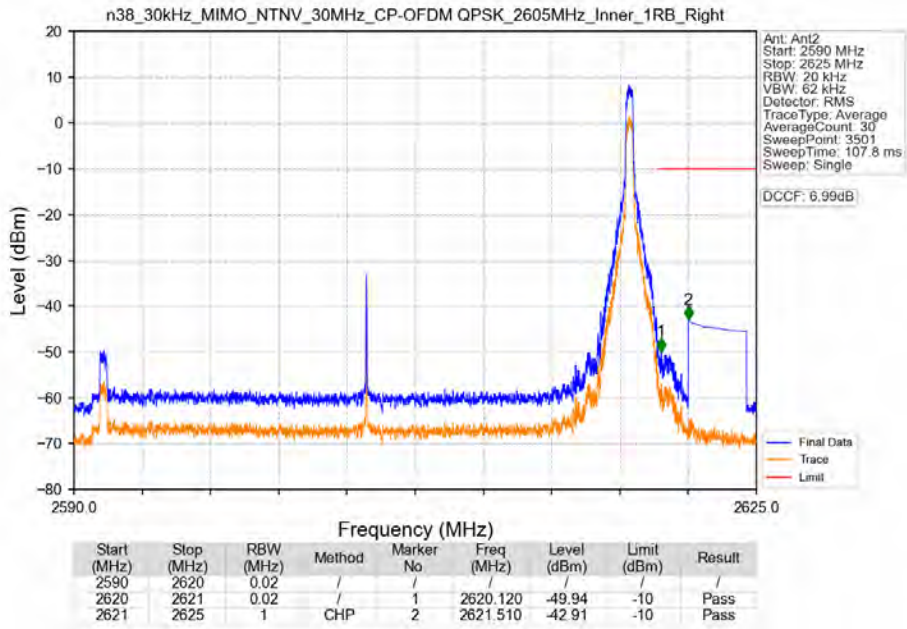
n38_30kHz_MIMO_NTNV_30MHz_CP-OFDM QPSK_2605MHz_Inner_1RB_Right
