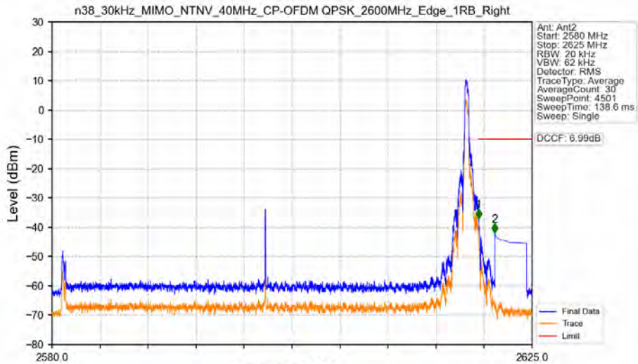
n38_30kHz_MIMO_NTNV_40MHz_CP-OFDM QPSK_2600MHz_Edge_1RB_Right
