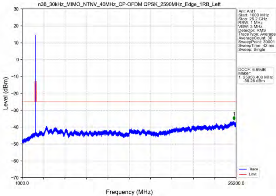
n38_30kHz_MIMO_NTNV_40MHz_CP-OFDM QPSK_2590MHz_Edge_1RB_Left
