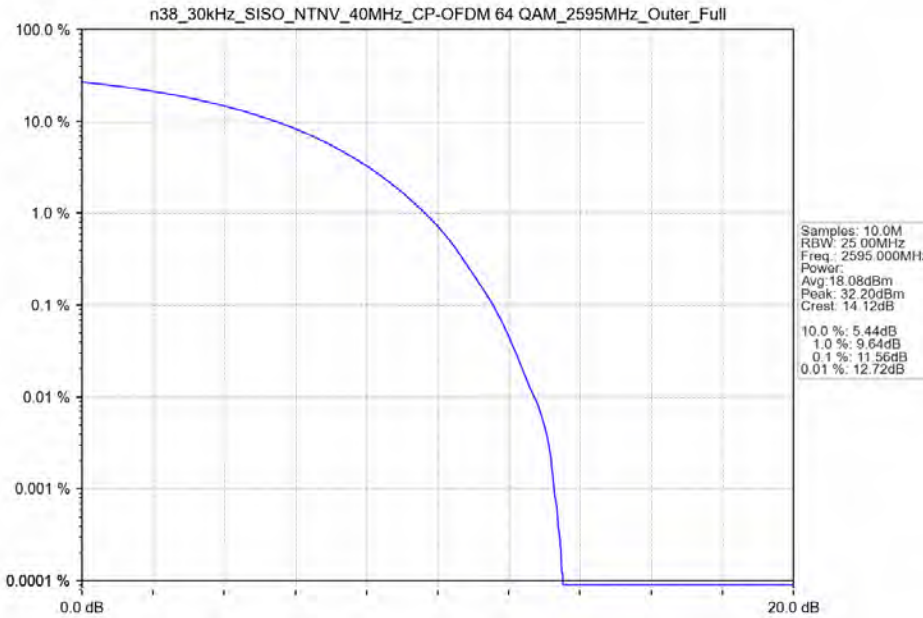
n38_30kHz_SISO_NTNV_40MHz_CP-OFDM 64 QAM_2595MHz_Outer_Full
