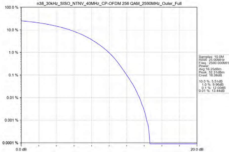
n38_30kHz_SISO_NTNV_40MHz_CP-OFDM 256 QAM_2590MHz_Outer_Full
