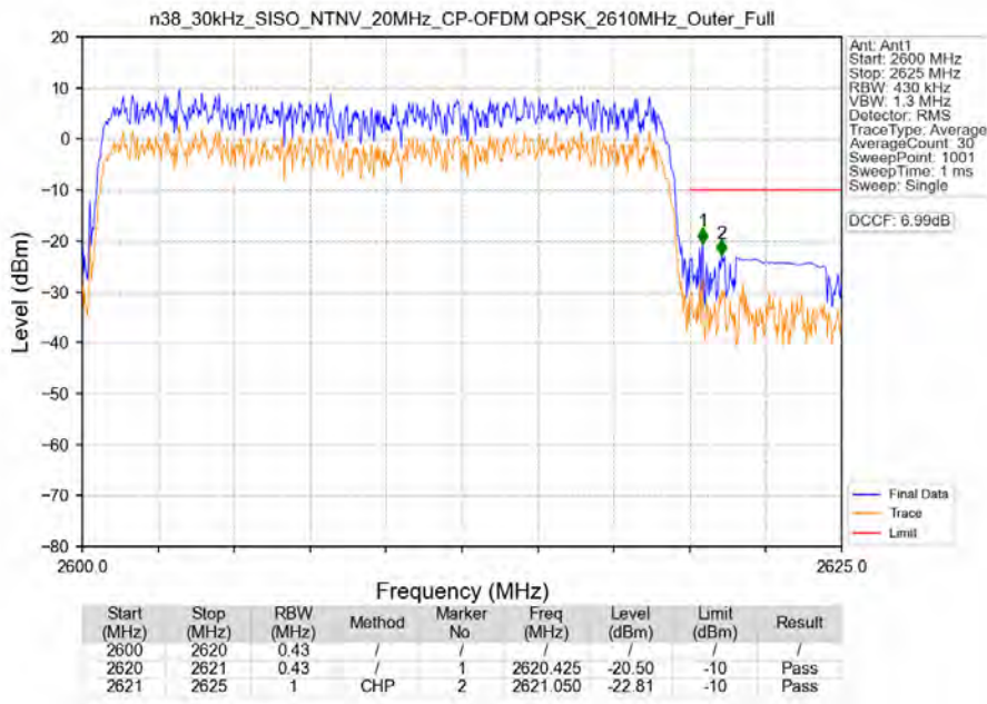
n38_30kHz_SISO_NTNV_20MHz_CP-OFDM QPSK_2610MHz_Outer_Full
