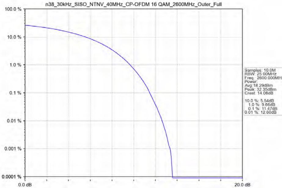
n38_30kHz_SISO_NTNV_40MHz_CP-OFDM 16 QAM_2600MHz_Outer_Full
