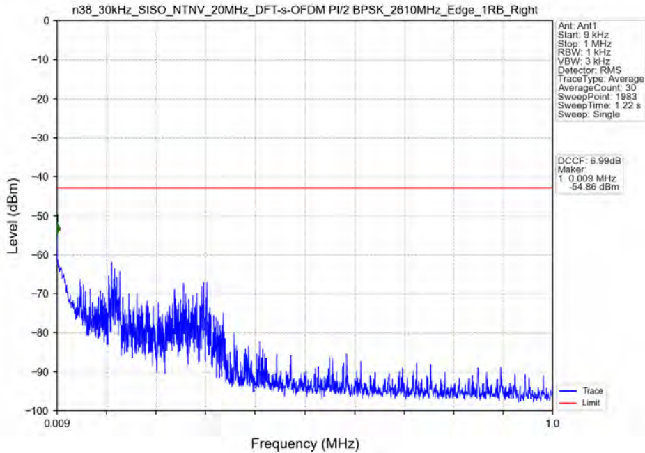
n38_30kHz_SISO_NTNV_20MHz_DFT-s-OFDM PI/2 BPSK_2610MHz_Edge_1RB_Right
