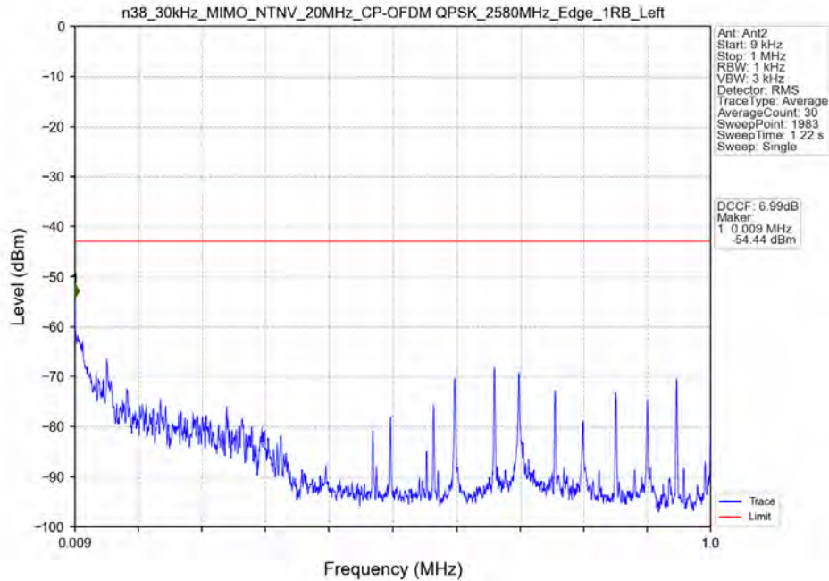
n38_30kHz_MIMO_NTNV_20MHz_CP-OFDM QPSK_2580MHz_Edge_1RB_Left
