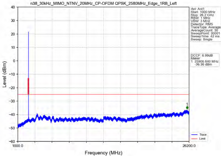
n38_30kHz_MIMO_NTNV_20MHz_CP-OFDM QPSK_2580MHz_Edge_1RB_Left
