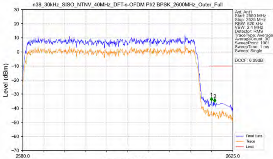
n38_30kHz_SISO_NTNV_40MHz_DFT-s-OFDM PI/2 BPSK_2600MHz_Outer_Full
