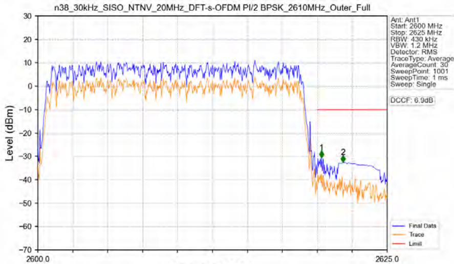
n38_30kHz_SISO_NTNV_20MHz_DFT-s-OFDM PI/2 BPSK_2610MHz_Outer_Full
