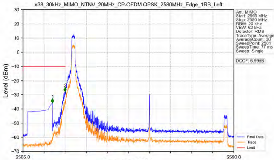
n38_30kHz_MIMO_NTNV_20MHz_CP-OFDM QPSK_2580MHz_Edge_1RB_Left
