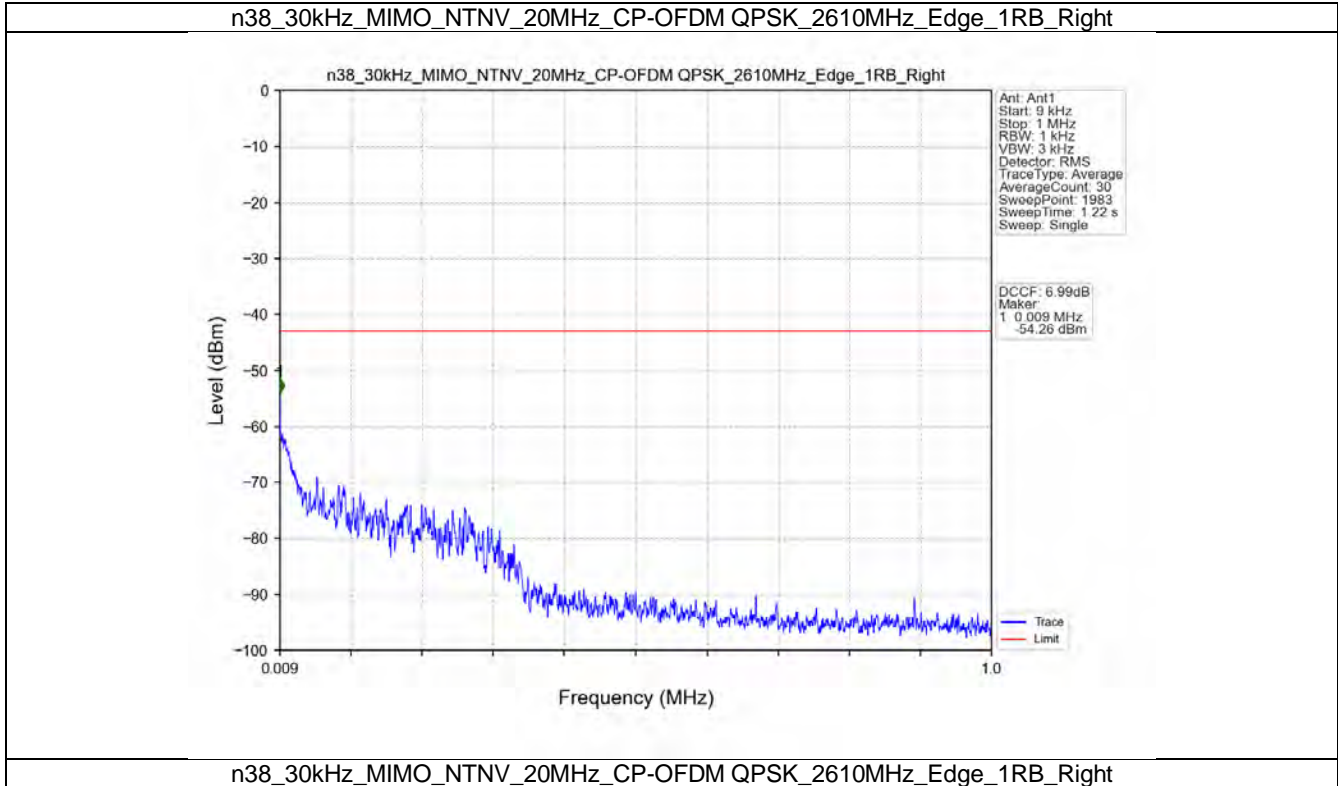
n38_30kHz_MIMO_NTNV_20MHz_CP-OFDM QPSK_2610MHz_Edge_1RB_Right
