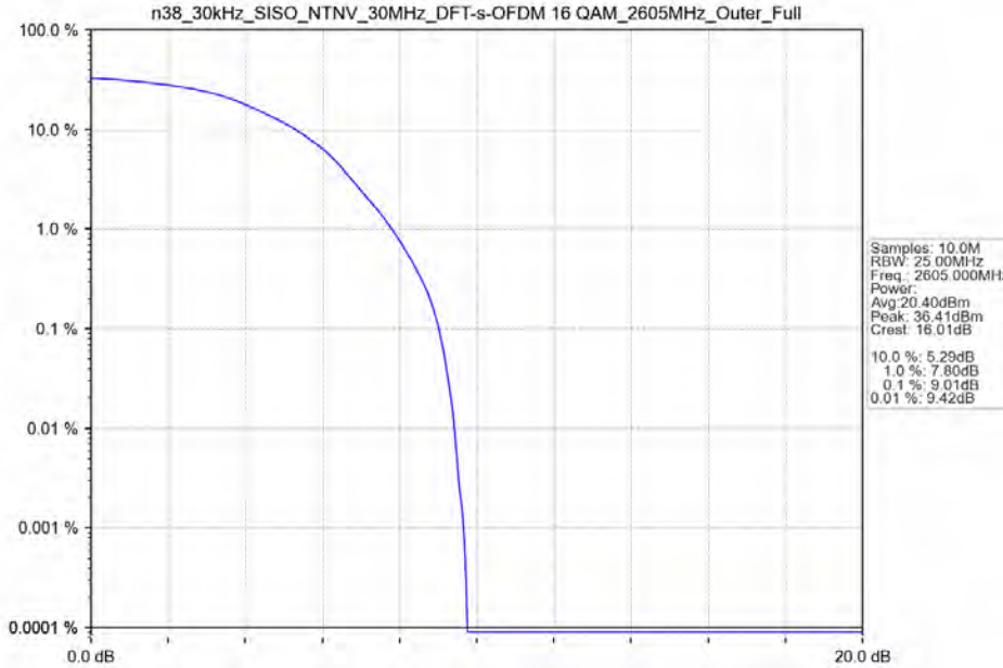
n38_30kHz_SISO_NTNV_30MHz_DFT-s-OFDM 16 QAM_2605MHz_Outer_Full
