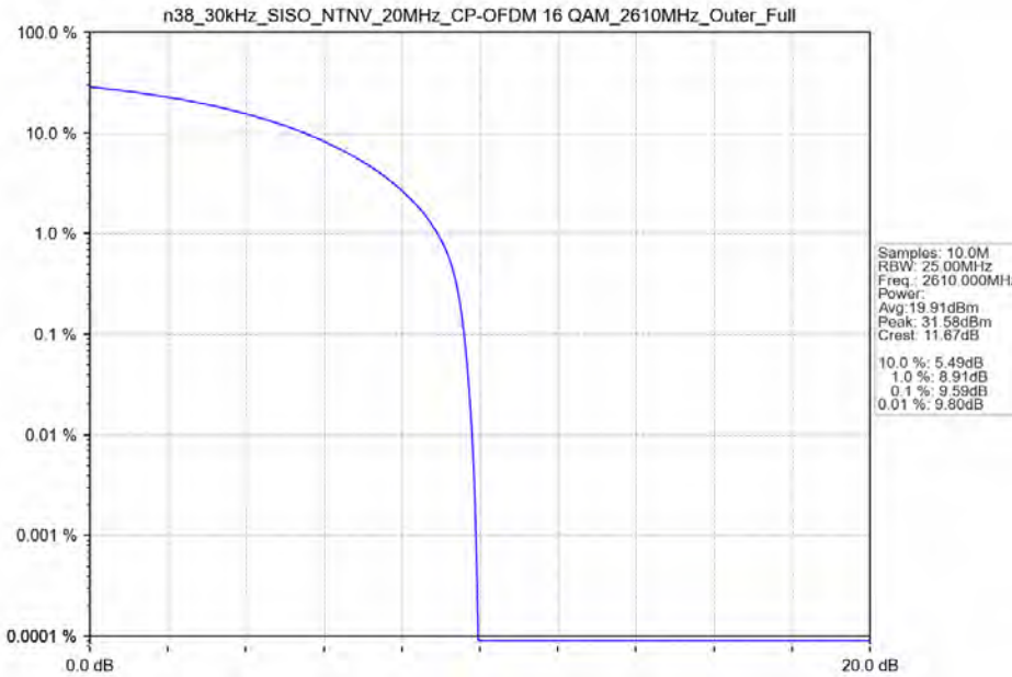
n38_30kHz_SISO_NTNV_20MHz_CP-OFDM 16 QAM_2610MHz_Outer_Full
