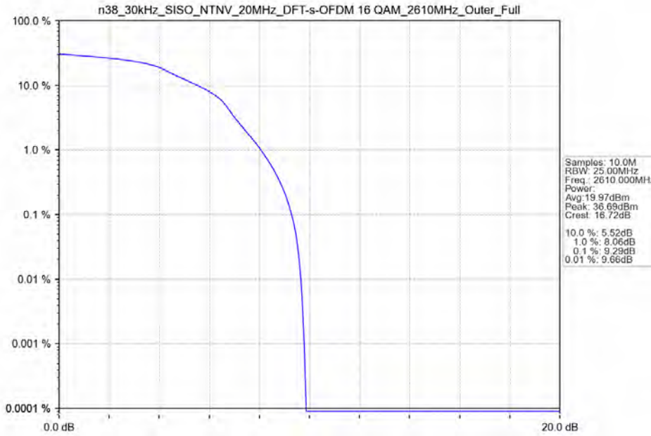
n38_30kHz_SISO_NTNV_20MHz_DFT-s-OFDM 16 QAM_2610MHz_Outer_Full
