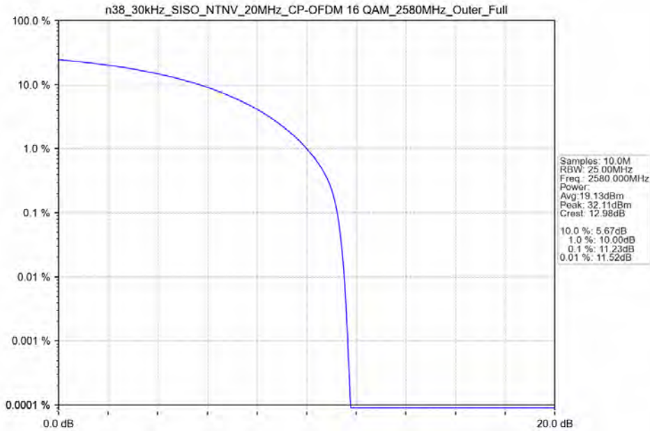
n38_30kHz_SISO_NTNV_20MHz_CP-OFDM 16 QAM_2580MHz_Outer_Full
