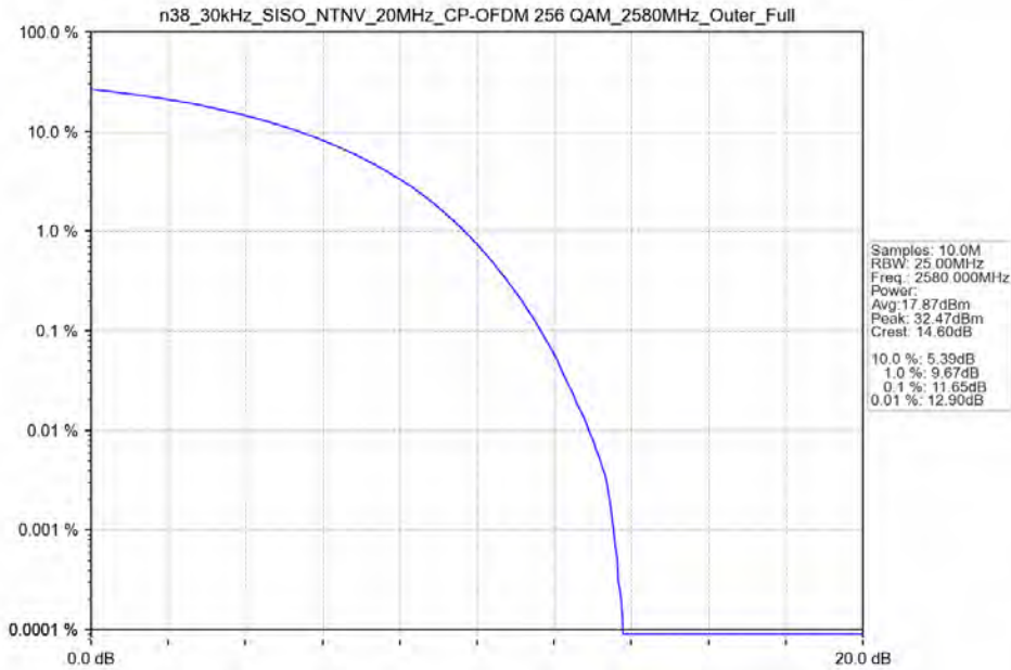
n38_30kHz_SISO_NTNV_20MHz_CP-OFDM 256 QAM_2580MHz_Outer_Full
