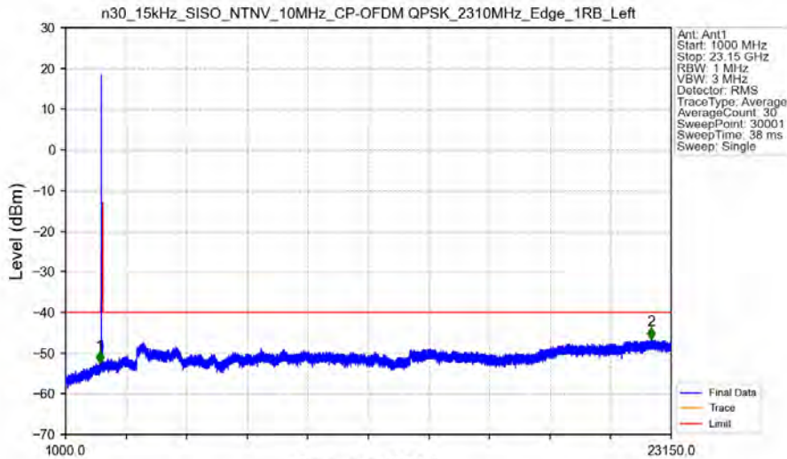
n30_15kHz_SISO_NTNV_10MHz_CP-OFDM QPSK_2310MHz_Edge_1RB_Left
