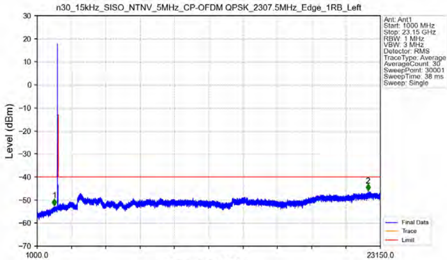
n30_15kHz_SISO_NTNV_5MHz_CP-OFDM QPSK_2307.5MHz_Edge_1RB_Left
