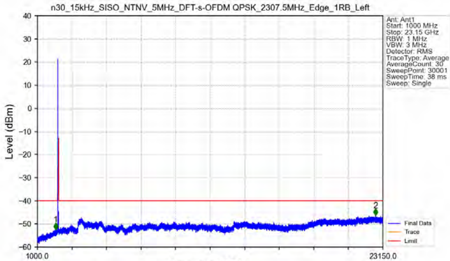
n30_15kHz_SISO_NTNV_5MHz_DFT-s-OFDM QPSK_2307.5MHz_Edge_1RB_Left
