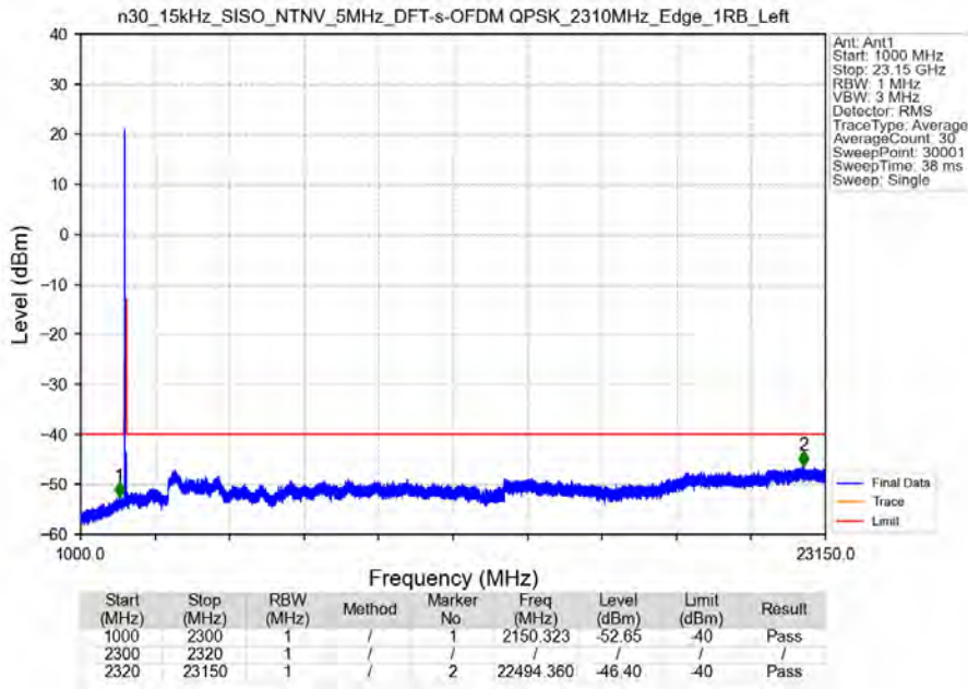
n30_15kHz_SISO_NTNV_5MHz_DFT-s-OFDM_QPSK_2310MHz_Edge_1RB_Left
