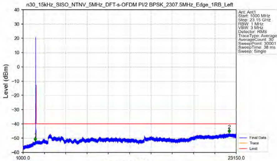
n30_15kHz_SISO_NTNV_5MHz_DFT-s-OFDM PI/2 BPSK_2307.5MHz_Edge_1RB_Left
