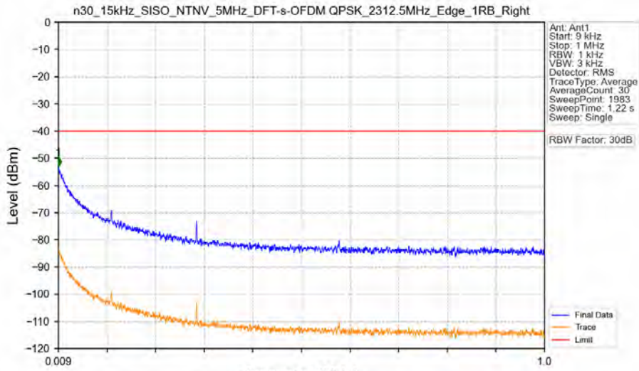
n30_15kHz_SISO_NTNV_5MHz_DFT-s-OFDM QPSK_2312.5MHz_Edge_1RB_Right
