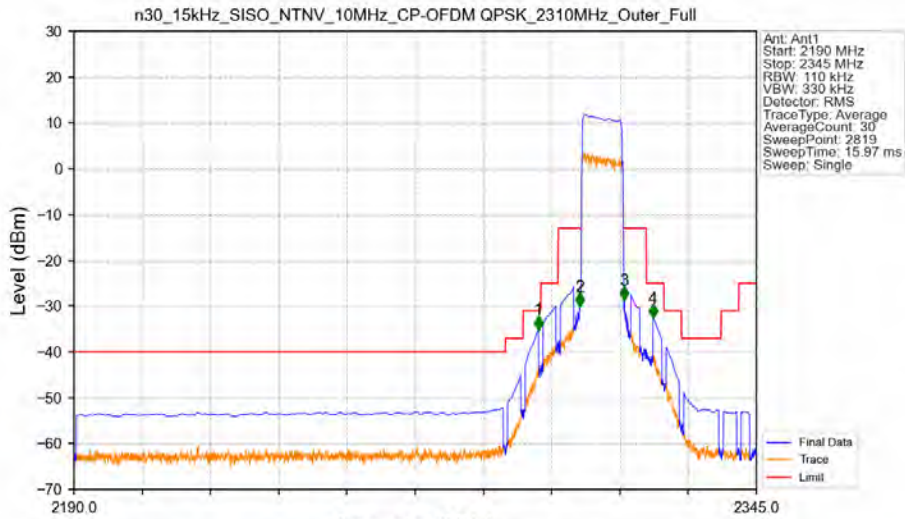
n30_15kHz_SISO_NTNV_10MHz_CP-OFDM QPSK_2310MHz_Outer_Full
