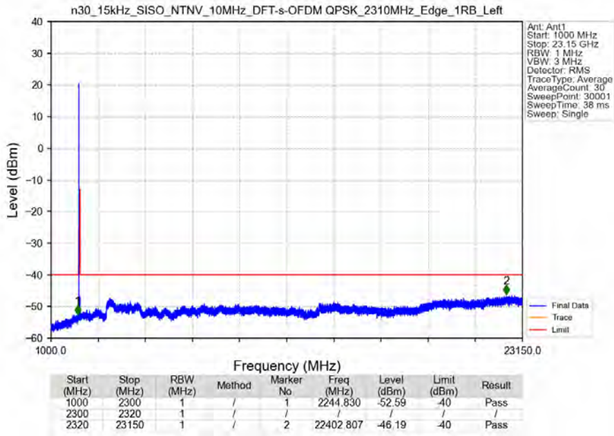
n30_15kHz_SISO_NTNV_10MHz_DFT-s-OFDM QPSK_2310MHz_Edge_1RB_Left
