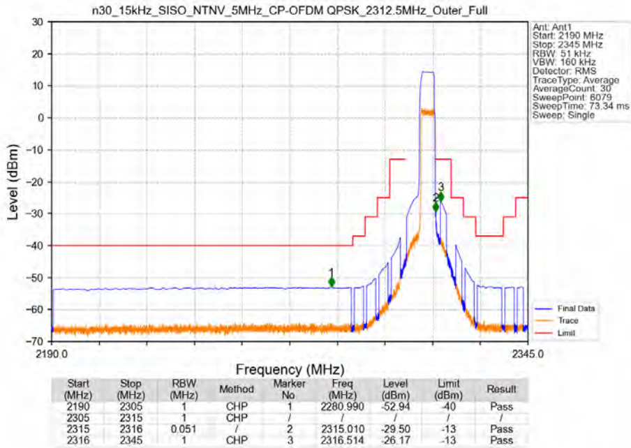
n30_15kHz_SISO_NTNV_5MHz_CP-OFDM QPSK_2312.5MHz_Outer_Full
