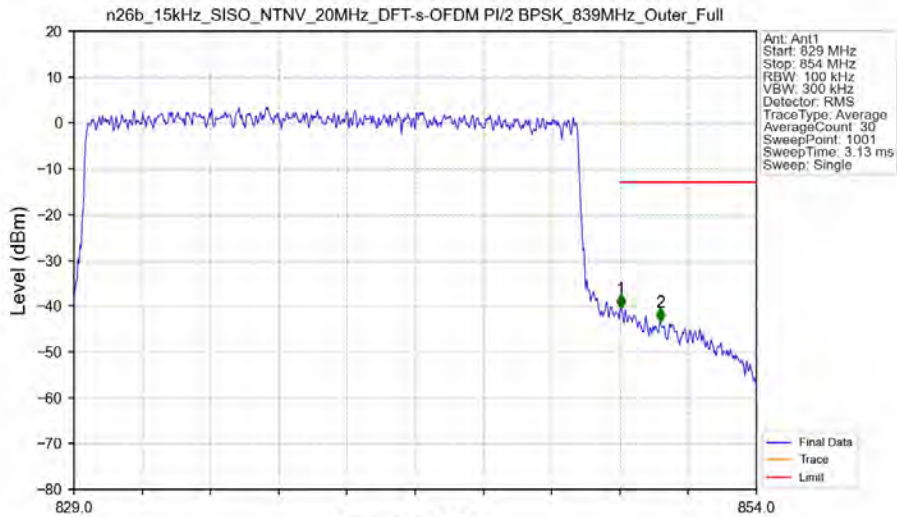
n26b_15kHz_SISO_NTNV_20MHz_DFT-s-OFDM PI/2 BPSK_839MHz_Outer_Full
