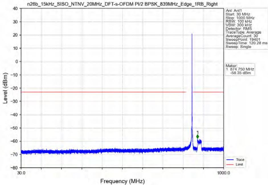
n26b_15kHz_SISO_NTNV_20MHz_DFT-s-OFDM PI/2 BPSK_839MHz_Edge_1RB_Right
