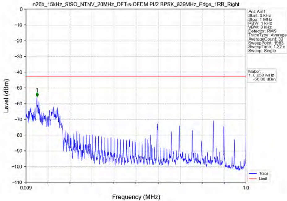
n26b_15kHz_SISO_NTNV_20MHz_DFT-s-OFDM PI/2 BPSK_839MHz_Edge_1RB_Right
