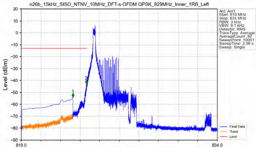
n26b_15kHz_SISO_NTNV_10MHz_DFT-s-OFDM_QPSK_829MHz_Inner_1RB_Left
