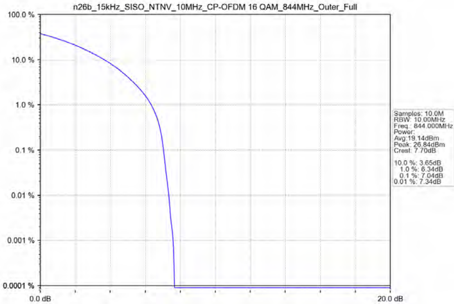
n26b_15kHz_SISO_NTNV_10MHz_CP-OFDM 16 QAM_844MHz_Outer_Full
