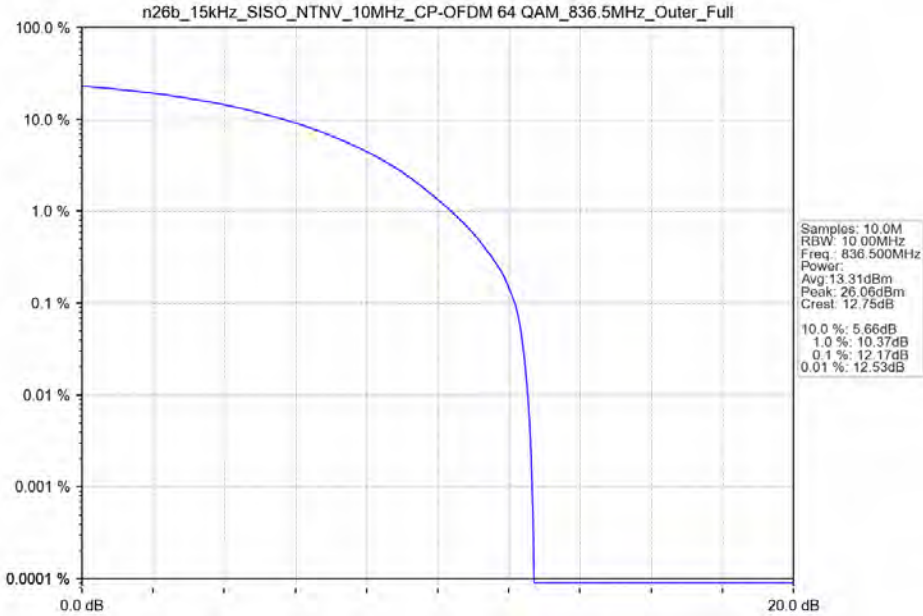
n26b_15kHz_SISO_NTNV_10MHz_CP-OFDM 64 QAM_836.5MHz_Outer_Full
