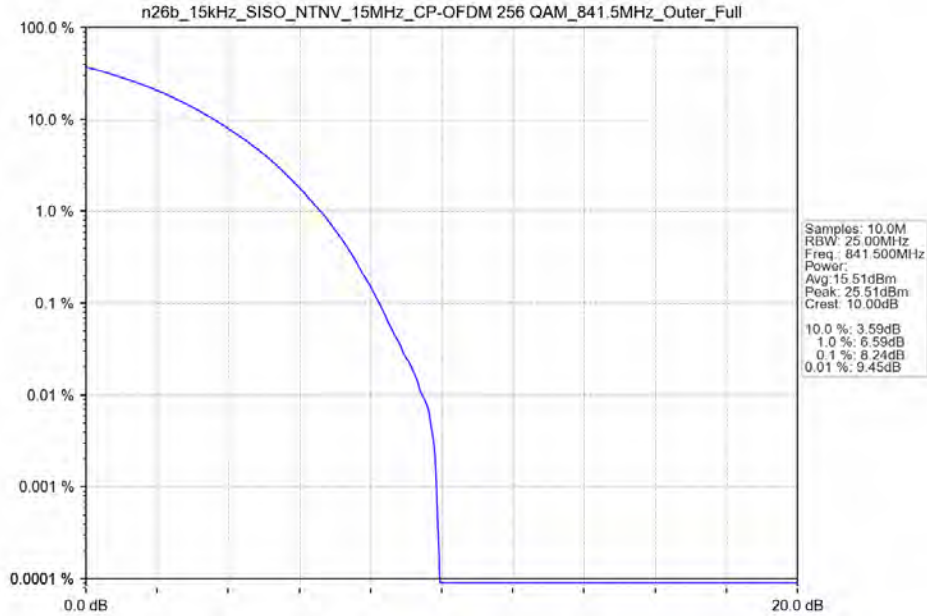
n26b_15kHz_SISO_NTNV_15MHz_CP-OFDM 256 QAM_841.5MHz_Outer_Full
