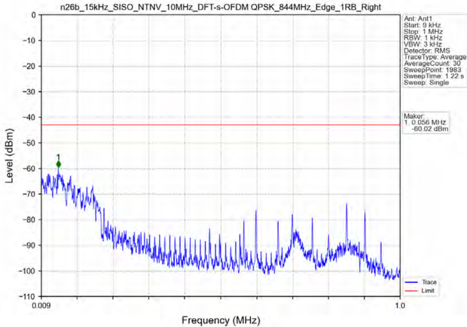
n26b_15kHz_SISO_NTNV_10MHz_DFT-s-OFDM_QPSK_844MHz_Edge_1RB_Right
