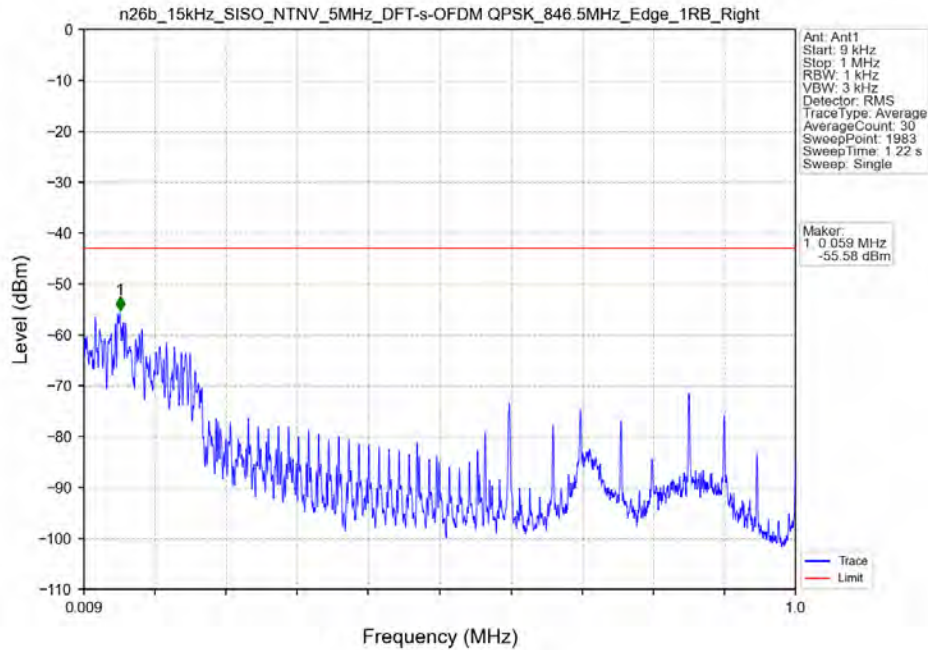
n26b_15kHz_SISO_NTNV_5MHz_DFT-s-OFDM QPSK_846.5MHz_Edge_1RB_Right
