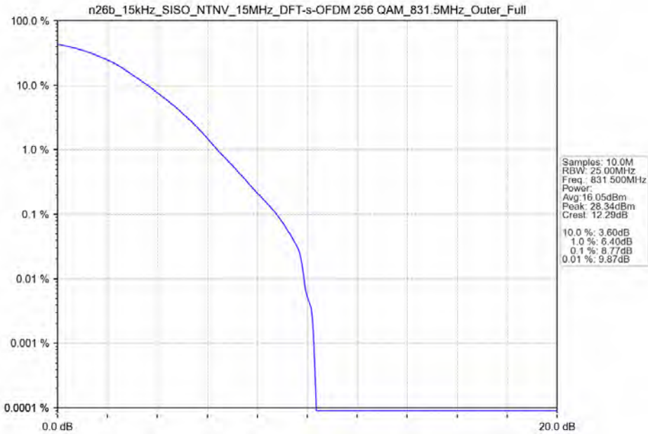
n26b_15kHz_SISO_NTNV_15MHz_DFT-s-OFDM 256 QAM_831.5MHz_Outer_Full
