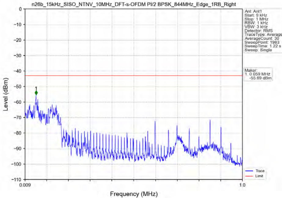
n26b_15kHz_SISO_NTNV_10MHz_DFT-s-OFDM PI/2 BPSK_844MHz_Edge_1RB_Right
