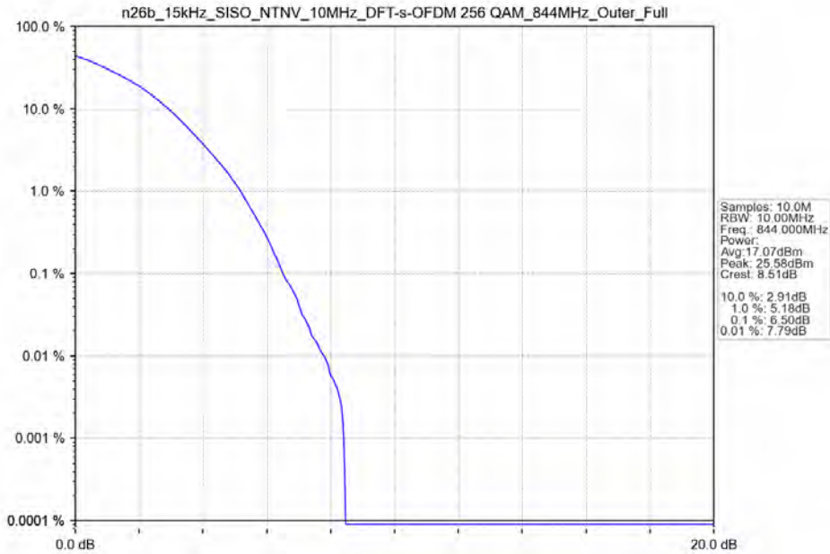
n26b_15kHz_SISO_NTNV_10MHz_DFT-s-OFDM 256 QAM_844MHz_Outer_Full
