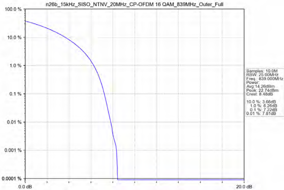
n26b_15kHz_SISO_NTNV_20MHz_CP-OFDM 16 QAM_839MHz_Outer_Full
