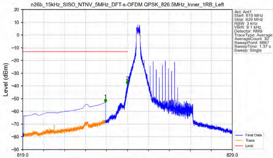
n26b_15kHz_SISO_NTNV_5MHz_DFT-s-OFDM_QPSK_826.5MHz_Inner_1RB_Left
