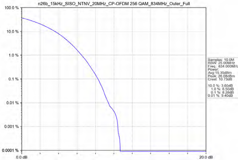
n26b_15kHz_SISO_NTNV_20MHz_CP-OFDM_256_QAM_834MHz_Outer_Full
