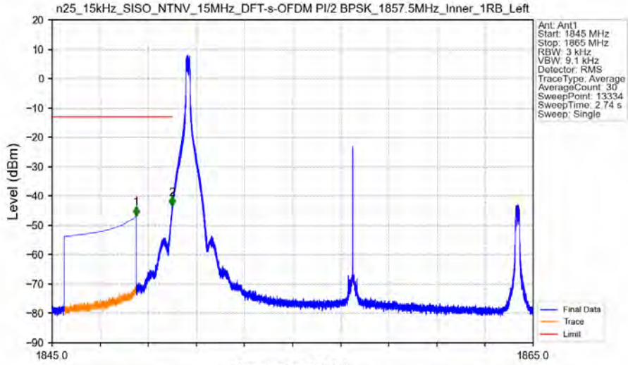
n25_15kHz_SISO_NTNV_15MHz_DFT-s-OFDM PI/2 BPSK_1857.5MHz_Inner_1RB_Left
