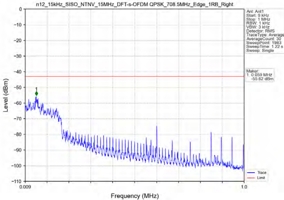
n12_15kHz_SISO_NTNV_15MHz_DFT-s-OFDM QPSK_708.5MHz_Edge_1RB_Right
