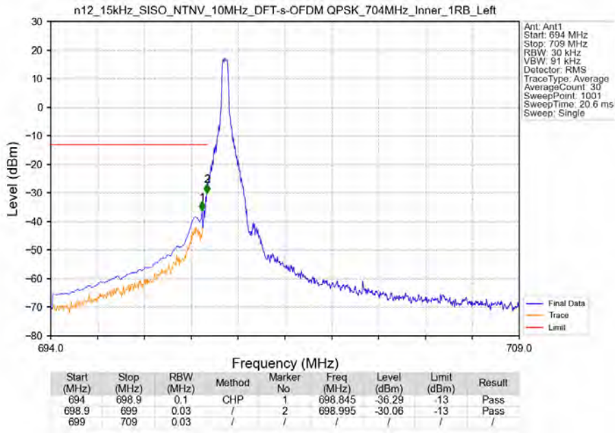
n12_15kHz_SISO_NTNV_10MHz_DFT-s-OFDM QPSK_704MHz_Inner_1RB_Left
