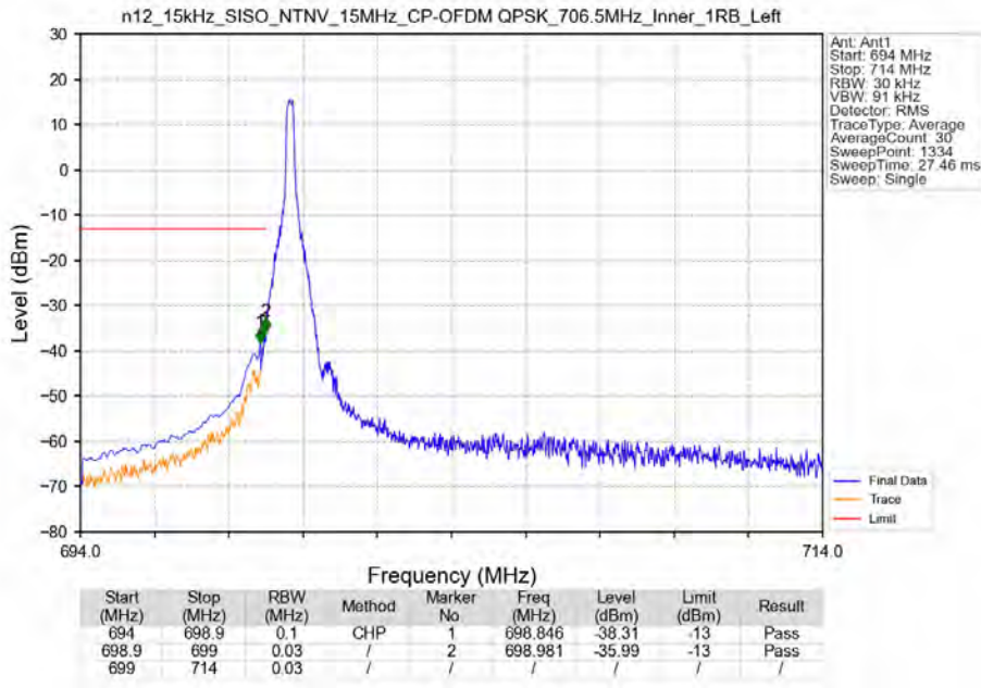
n12_15kHz_SISO_NTNV_15MHz_CP-OFDM QPSK_706.5MHz_Inner_1RB_Left
