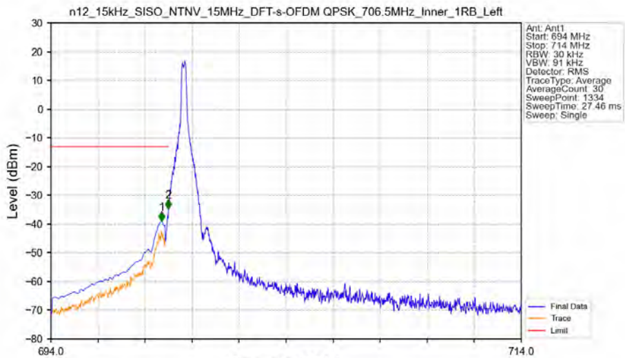
n12_15kHz_SISO_NTNV_15MHz_DFT-s-OFDM QPSK_706.5MHz_Inner_1RB_Left
