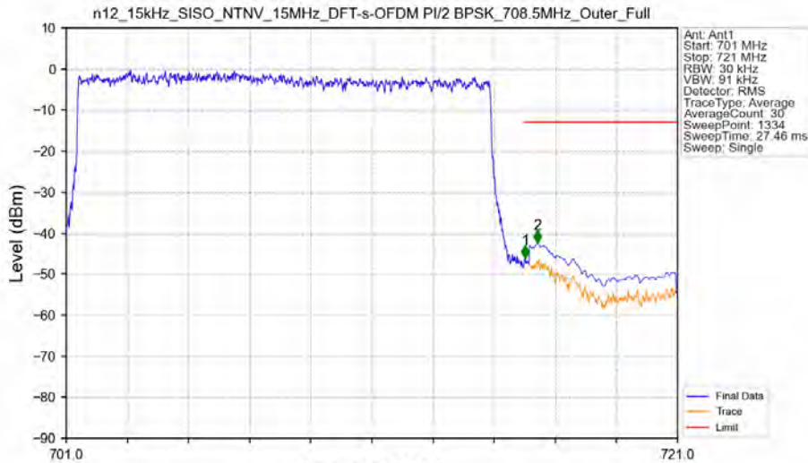
n12_15kHz_SISO_NTNV_15MHz_DFT-s-OFDM PI/2 BPSK_708.5MHz_Outer_Full
