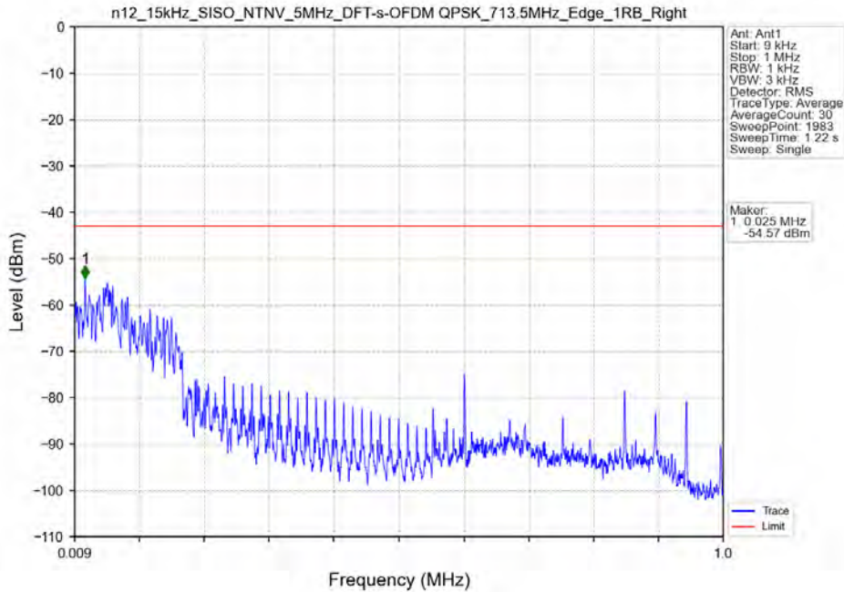
n12_15kHz_SISO_NTNV_5MHz_DFT-s-OFDM QPSK_713.5MHz_Edge_1RB_Right
