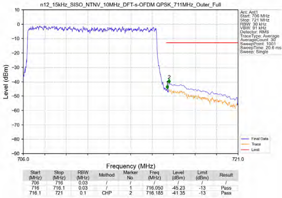
n12_15kHz_SISO_NTNV_10MHz_DFT-s-OFDM QPSK_711MHz_Outer_Full
