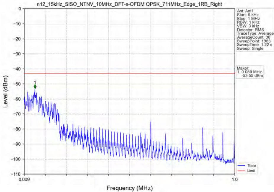
n12_15kHz_SISO_NTNV_10MHz_DFT-s-OFDM QPSK_711MHz_Edge_1RB_Right
