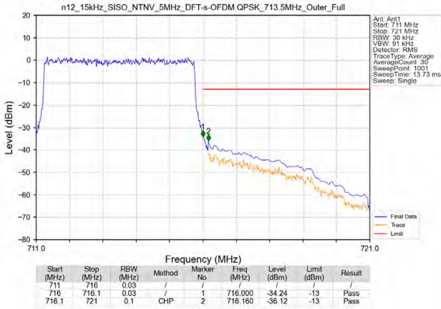
n12_15kHz_SISO_NTNV_5MHz_DFT-s-OFDM QPSK_713.5MHz_Outer_Full
