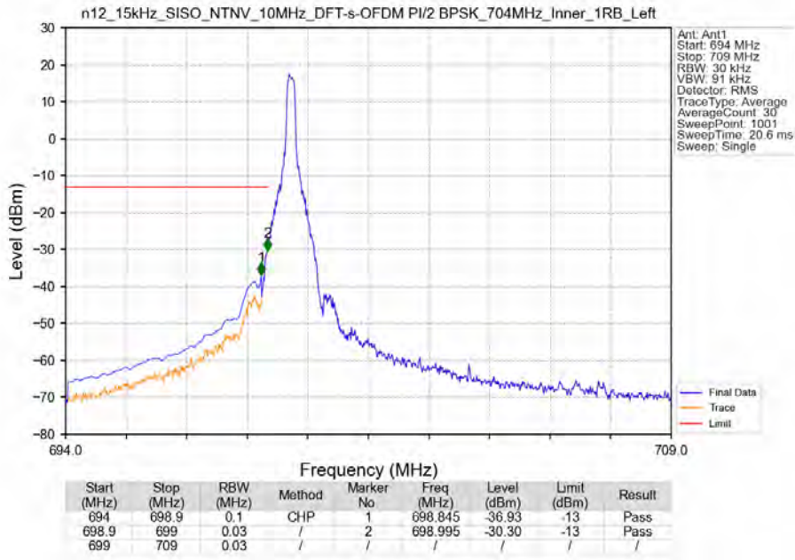
n12_15kHz_SISO_NTNV_10MHz_DFT-s-OFDM PI/2 BPSK_704MHz_Inner_1RB_Left
