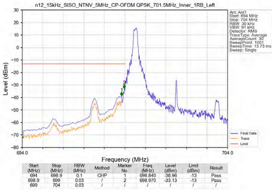
n12_15kHz_SISO_NTNV_5MHz_CP-OFDM QPSK_701.5MHz_Inner_1RB_Left
