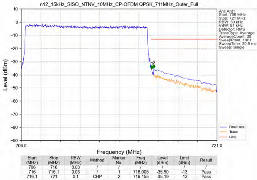
n12_15kHz_SISO_NTNV_10MHz_CP-OFDM QPSK_711MHz_Outer_Full
