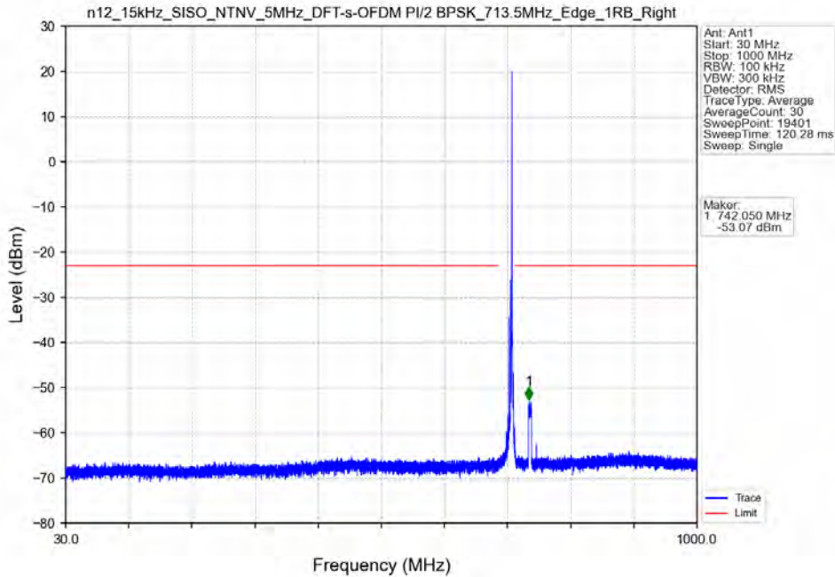
n12_15kHz_SISO_NTNV_5MHz_DFT-s-OFDM PI/2 BPSK_713.5MHz_Edge_1RB_Right
