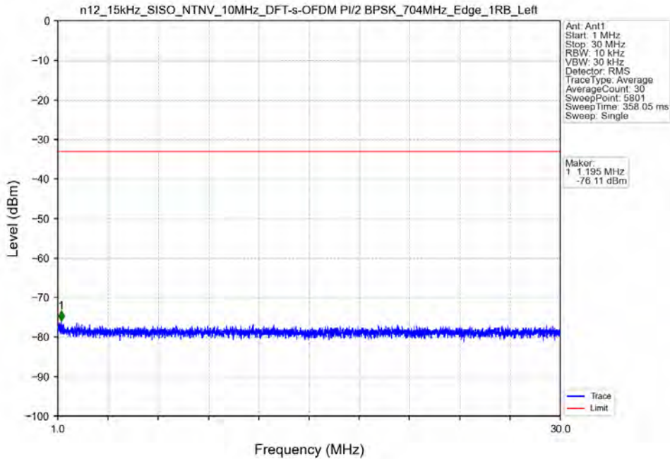
n12_15kHz_SISO_NTNV_10MHz_DFT-s-OFDM PI/2 BPSK_704MHz_Edge_1RB_Left
