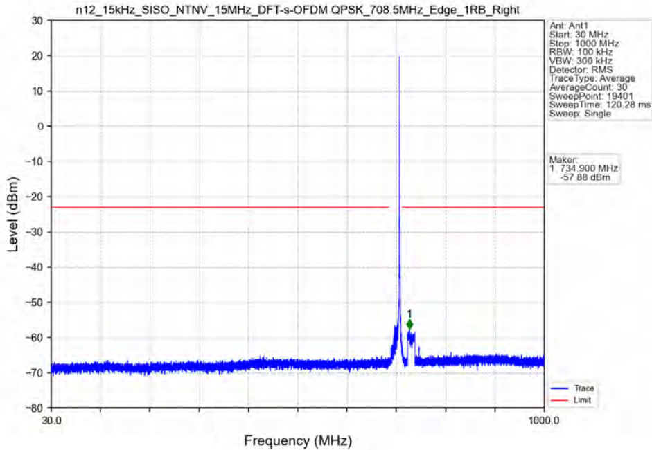
n12_15kHz_SISO_NTNV_15MHz_DFT-s-OFDM QPSK_708.5MHz_Edge_1RB_Right
