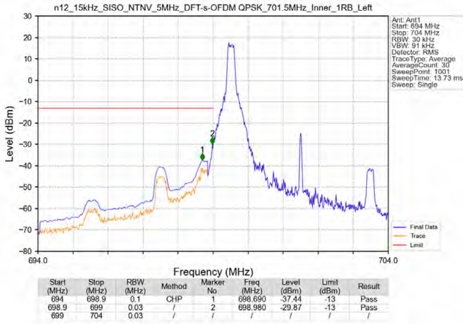
n12_15kHz_SISO_NTNV_5MHz_DFT-s-OFDM_QPSK_701.5MHz_Inner_1RB_Left
