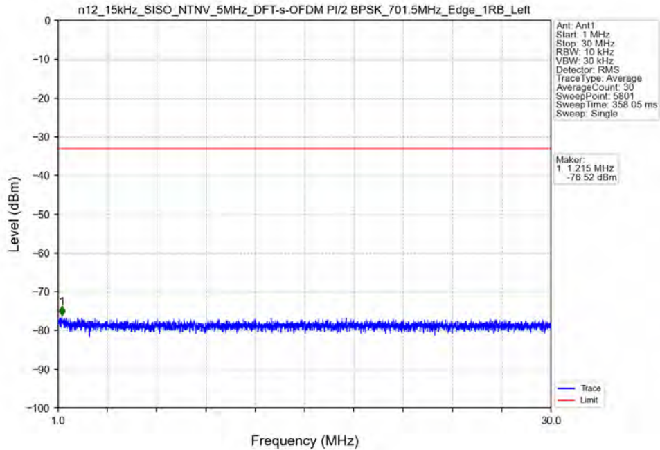
n12_15kHz_SISO_NTNV_5MHz_DFT-s-OFDM PI/2 BPSK_701.5MHz_Edge_1RB_Left
