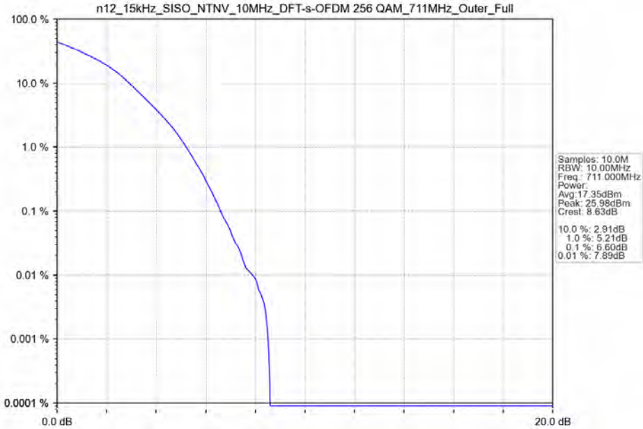
n12_15kHz_SISO_NTNV_10MHz_DFT-s-OFDM 256 QAM_711MHz_Outer_Full
