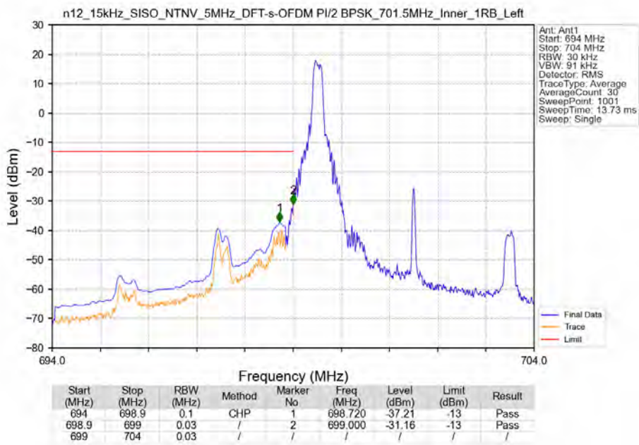
n12_15kHz_SISO_NTNV_5MHz_DFT-s-OFDM PI/2 BPSK_701.5MHz_Inner_1RB_Left
