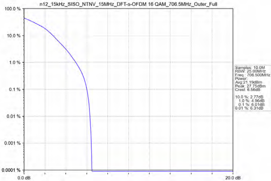
n12_15kHz_SISO_NTNV_15MHz_DFT-s-OFDM_16_QAM_706.5MHz_Outer_Full
