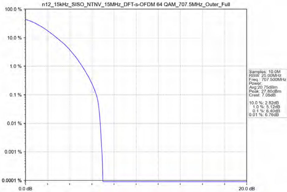
n12_15kHz_SISO_NTNV_15MHz_DFT-s-OFDM 64 QAM_707.5MHz_Outer_Full
