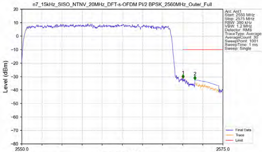
n7_15kHz_SISO_NTNV_20MHz_DFT-s-OFDM PI/2 BPSK_2560MHz_Outer_Full
