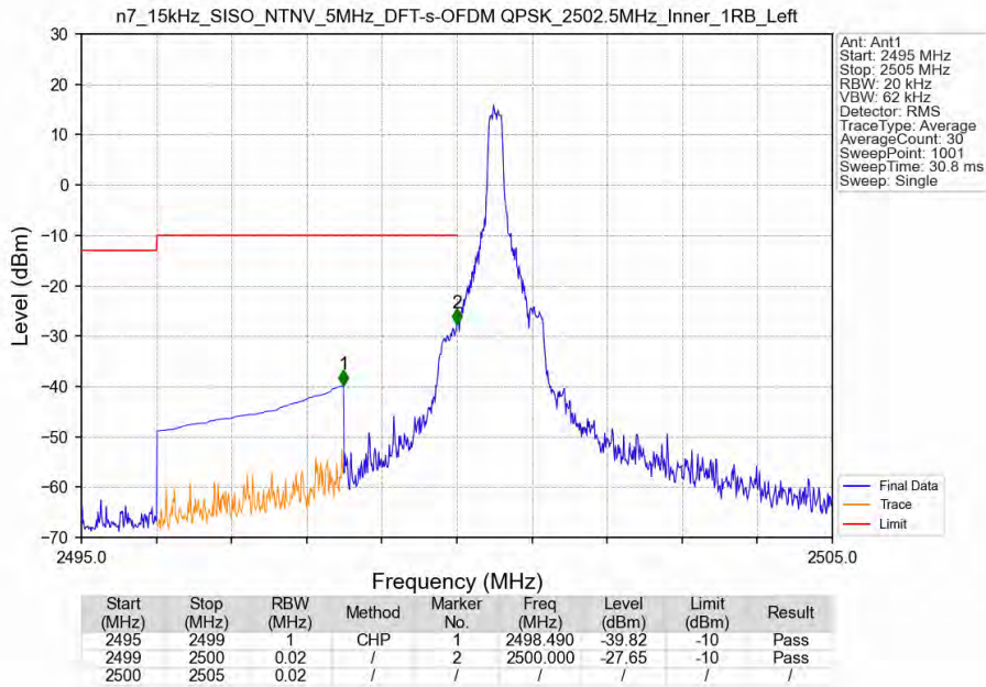
n7_15kHz_SISO_NTNV_5MHz_DFT-s-OFDM QPSK_2502.5MHz_Inner_1RB_Left
