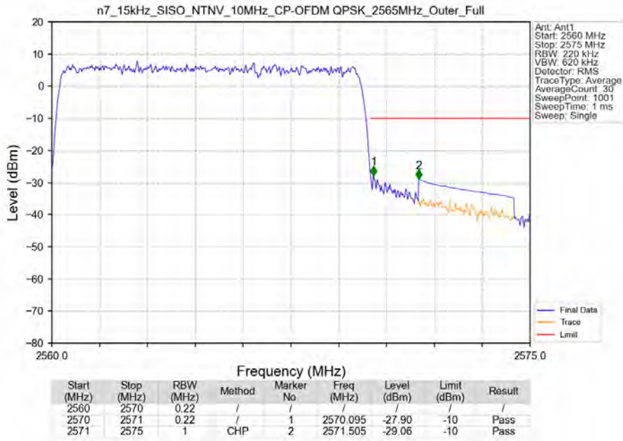
n7_15kHz_SISO_NTNV_10MHz_CP-OFDM QPSK_2565MHz_Outer_Full
