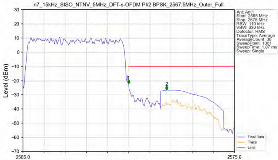
n7_15kHz_SISO_NTNV_5MHz_DFT-s-OFDM PI/2 BPSK_2567.5MHz_Outer_Full
