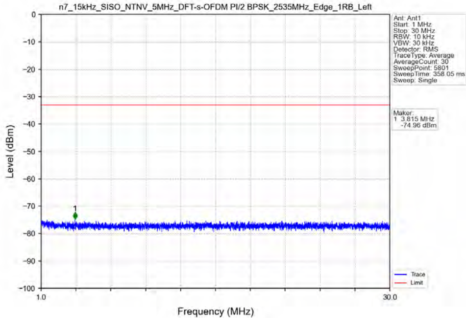
n7_15kHz_SISO_NTNV_5MHz_DFT-s-OFDM PI/2 BPSK_2535MHz_Edge_1RB_Left
