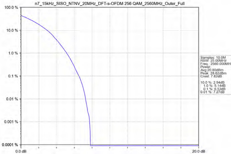
n7_15kHz_SISO_NTNV_20MHz_DFT-s-OFDM 256 QAM_2560MHz_Outer_Full
