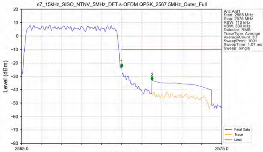
n7_15kHz_SISO_NTNV_5MHz_DFT-s-OFDM QPSK_2567.5MHz_Outer_Full
