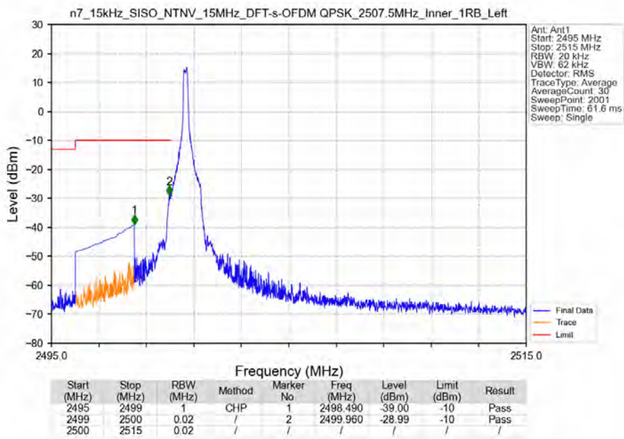
n7_15kHz_SISO_NTNV_15MHz_DFT-s-OFDM QPSK_2507.5MHz_Inner_1RB_Left
