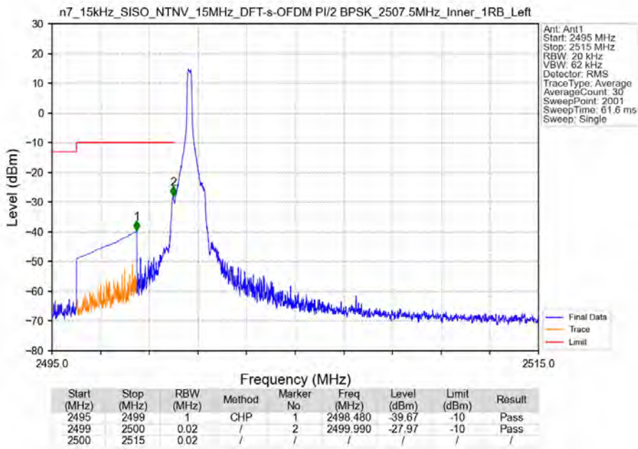
n7_15kHz_SISO_NTNV_15MHz_DFT-s-OFDM PI/2 BPSK_2507.5MHz_Inner_1RB_Left
