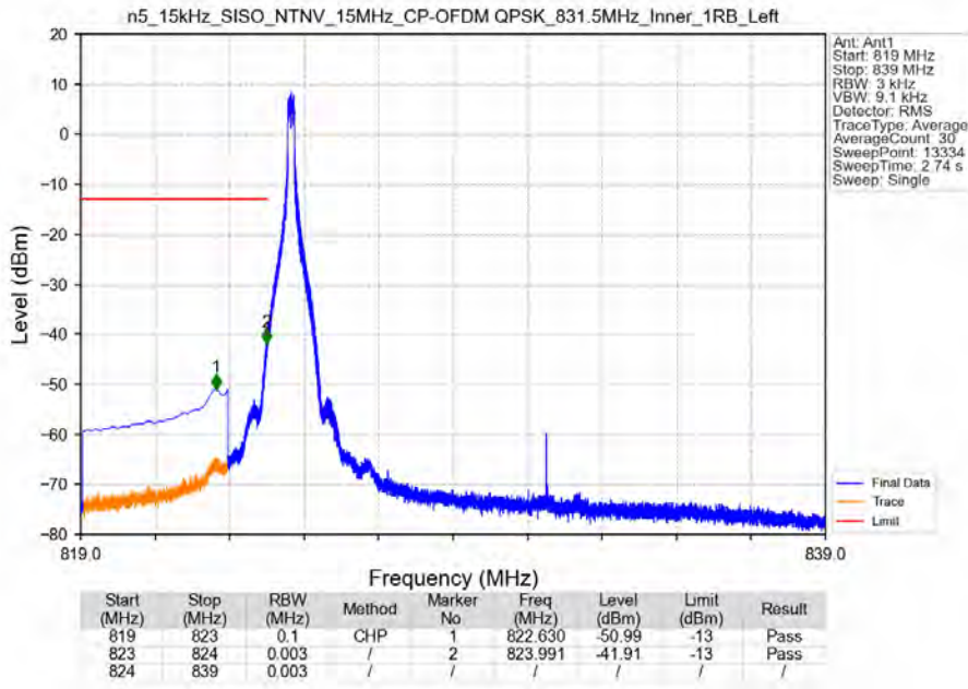
n5_15kHz_SISO_NTNV_15MHz_CP-OFDM QPSK_831.5MHz_Inner_1RB_Left
