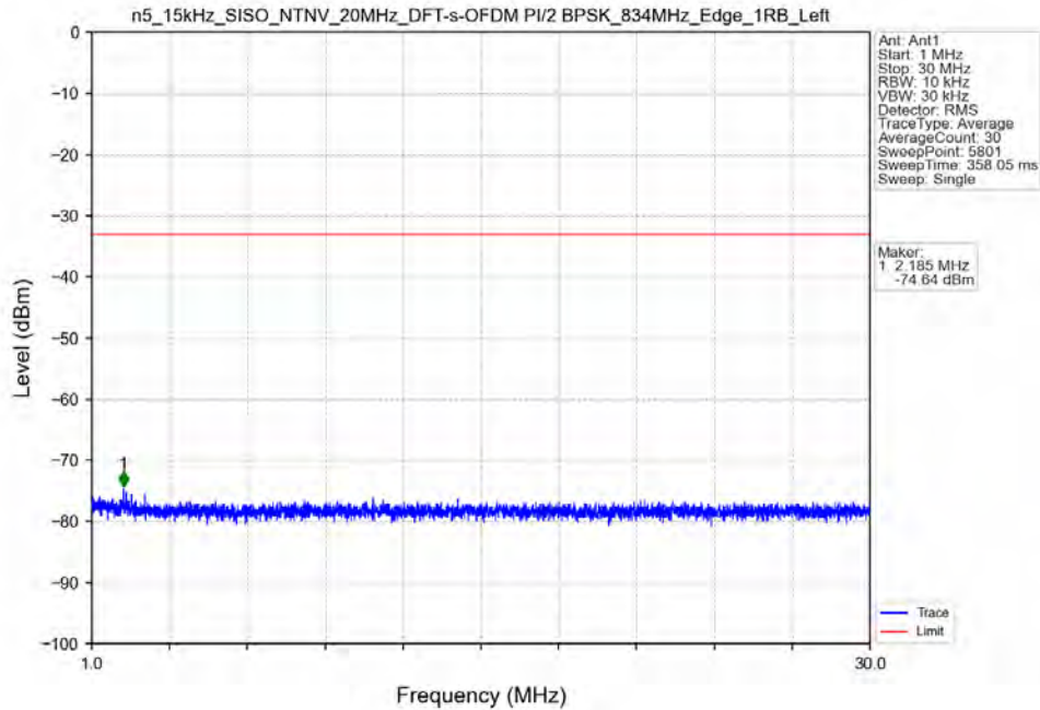
n5_15kHz_SISO_NTNV_20MHz_DFT-s-OFDM PI/2 BPSK_834MHz_Edge_1RB_Left
