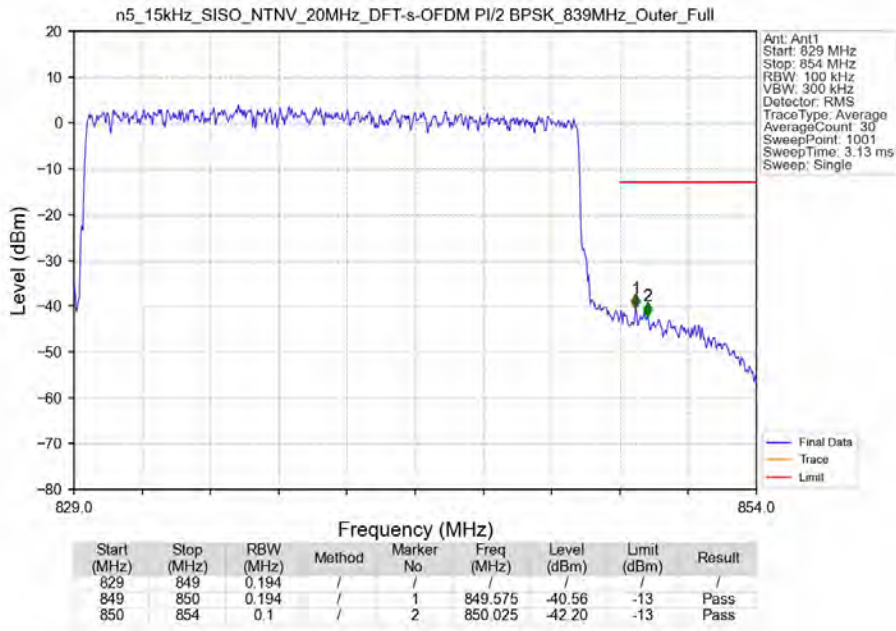
n5_15kHz_SISO_NTNV_20MHz_DFT-s-OFDM PI/2 BPSK_839MHz_Outer_Full
