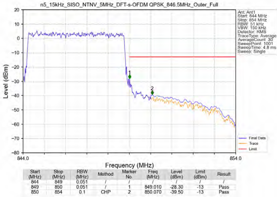
n5_15kHz_SISO_NTNV_5MHz_DFT-s-OFDM QPSK_846.5MHz_Outer_Full
