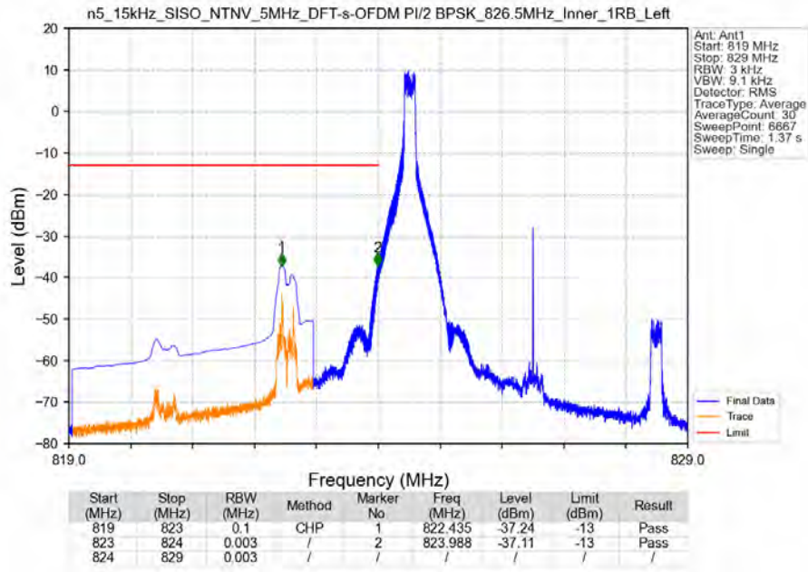
n5_15kHz_SISO_NTNV_5MHz_DFT-s-OFDM PI/2 BPSK_826.5MHz_Inner_1RB_Left
