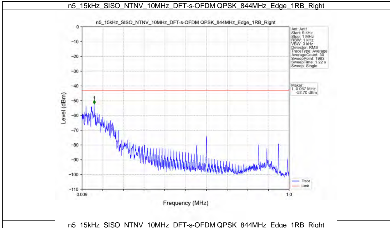
n5_15kHz_SISO_NTNV_10MHz_DFT-s-OFDM_QPSK_844MHz_Edge_1RB_Right
