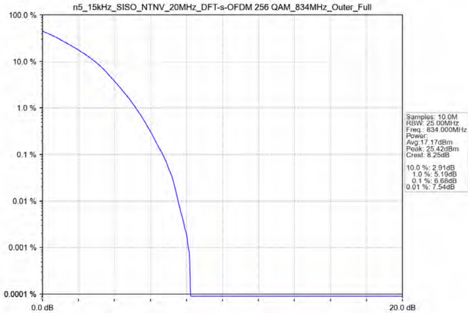
n5_15kHz_SISO_NTNV_20MHz_DFT-s-OFDM 256 QAM_834MHz_Outer_Full
