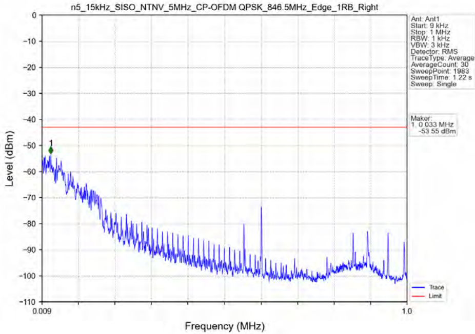
n5_15kHz_SISO_NTNV_5MHz_CP-OFDM QPSK_846.5MHz_Edge_1RB_Right
