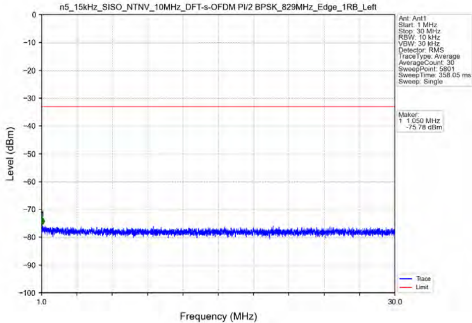
n5_15kHz_SISO_NTNV_10MHz_DFT-s-OFDM PI/2 BPSK_829MHz_Edge_1RB_Left
