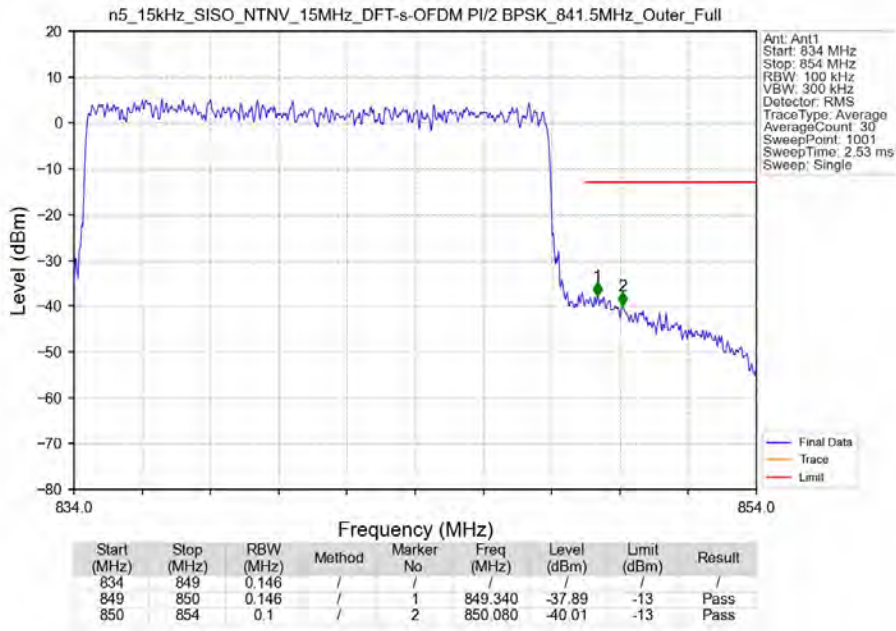
n5_15kHz_SISO_NTNV_15MHz_DFT-s-OFDM PI/2 BPSK_841.5MHz_Outer_Full
