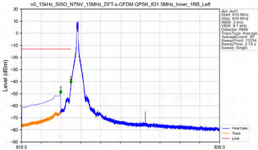
n5_15kHz_SISO_NTNV_15MHz_DFT-s-OFDM_QPSK_831.5MHz_Inner_1RB_Left
