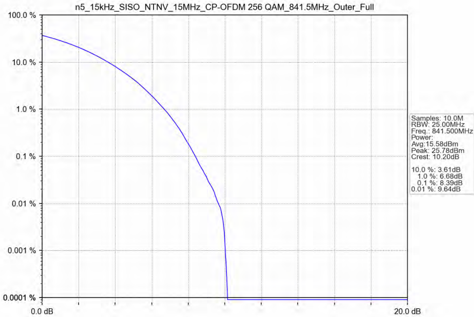
n5_15kHz_SISO_NTNV_15MHz_CP-OFDM 256 QAM_841.5MHz_Outer_Full
