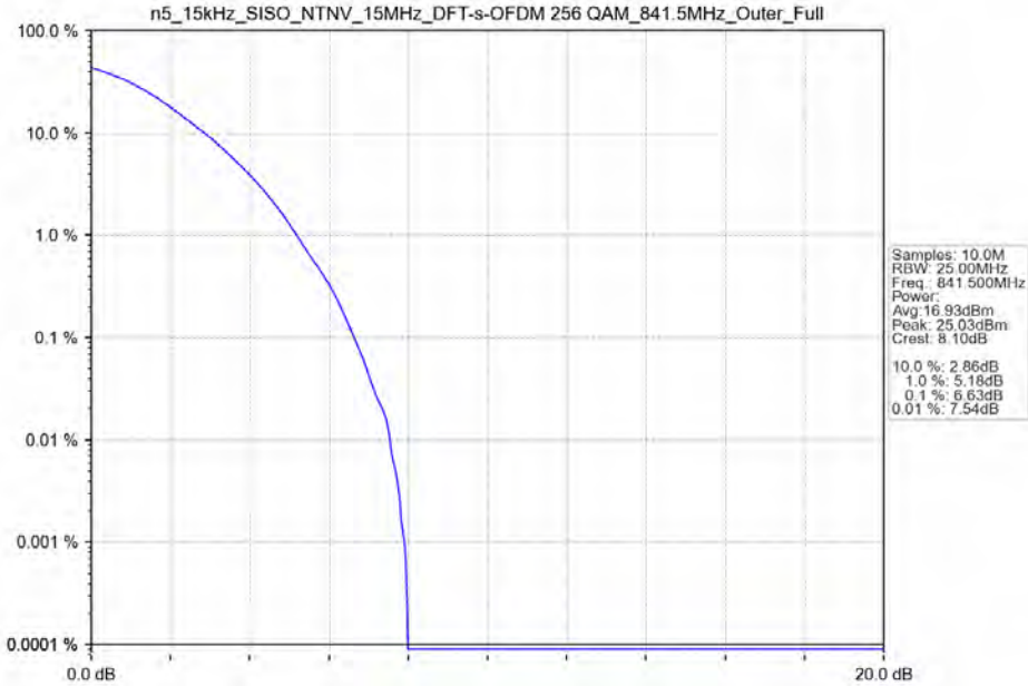
n5_15kHz_SISO_NTNV_15MHz_DFT-s-OFDM 256 QAM_841.5MHz_Outer_Full
