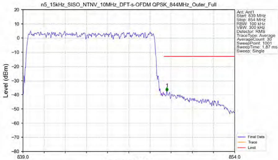
n5_15kHz_SISO_NTNV_10MHz_DFT-s-OFDM_QPSK_844MHz_Outer_Full
