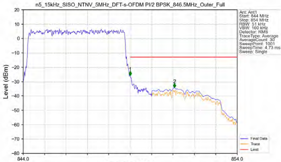
n5_15kHz_SISO_NTNV_5MHz_DFT-s-OFDM PI/2 BPSK_846.5MHz_Outer_Full
