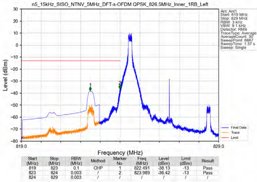
n5_15kHz_SISO_NTNV_5MHz_DFT-s-OFDM QPSK_826.5MHz_Inner_1RB_Left
