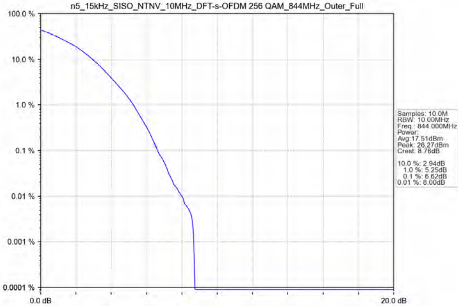
n5_15kHz_SISO_NTNV_10MHz_DFT-s-OFDM 256 QAM_844MHz_Outer_Full
