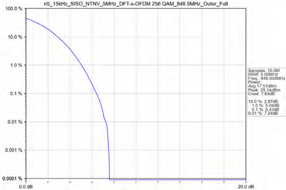
n5_15kHz_SISO_NTNV_5MHz_DFT-s-OFDM 256 QAM_846.5MHz_Outer_Full
