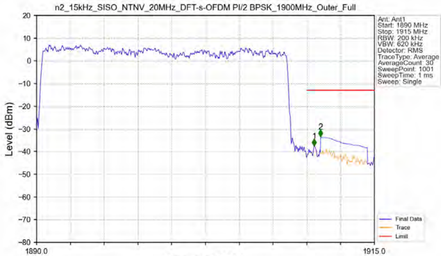
n2_15kHz_SISO_NTNV_20MHz_DFT-s-OFDM PI/2 BPSK_1900MHz_Outer_Full
