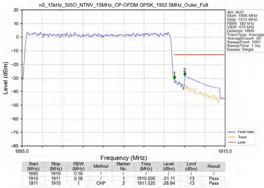
n2_15kHz_SISO_NTNV_15MHz_CP-OFDM QPSK_1902.5MHz_Outer_Full
