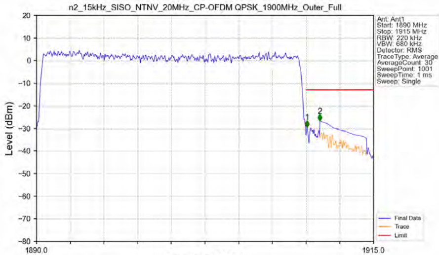
n2_15kHz_SISO_NTNV_20MHz_CP-OFDM QPSK_1900MHz_Outer_Full
