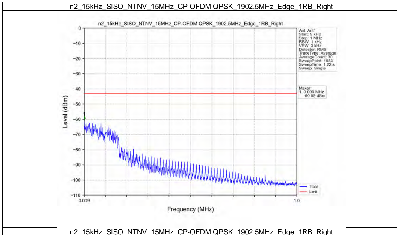
n2_15kHz_SISO_NTNV_15MHz_CP-OFDM QPSK_1902.5MHz_Edge_1RB_Right
