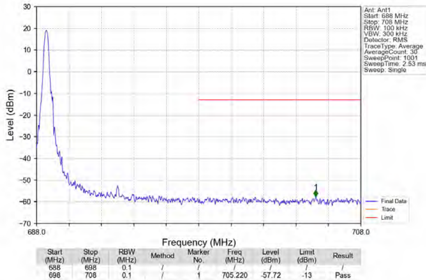
Band71_10MHz_64QAM_HCH_693MHz_RB_50_0_NTV
