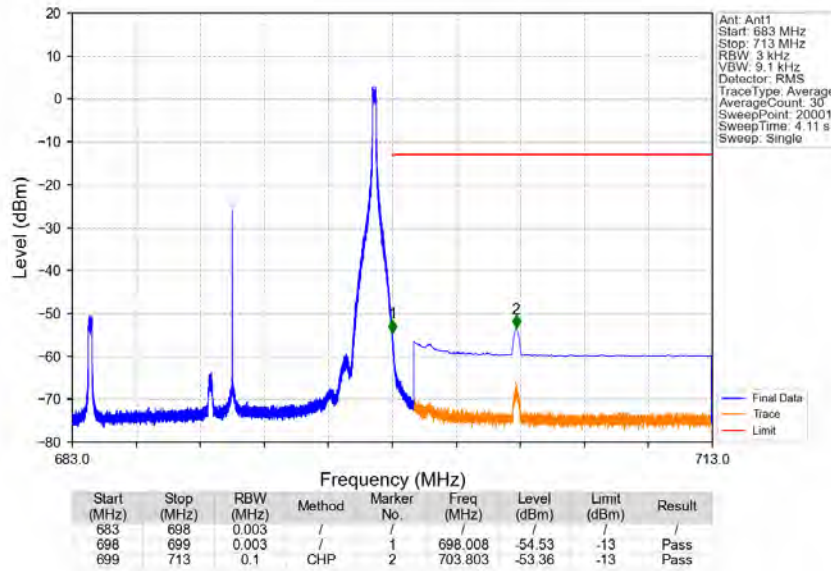
Band71_15MHz_256QAM_HCH_690.5MHz_RB_1_74_NTNV
