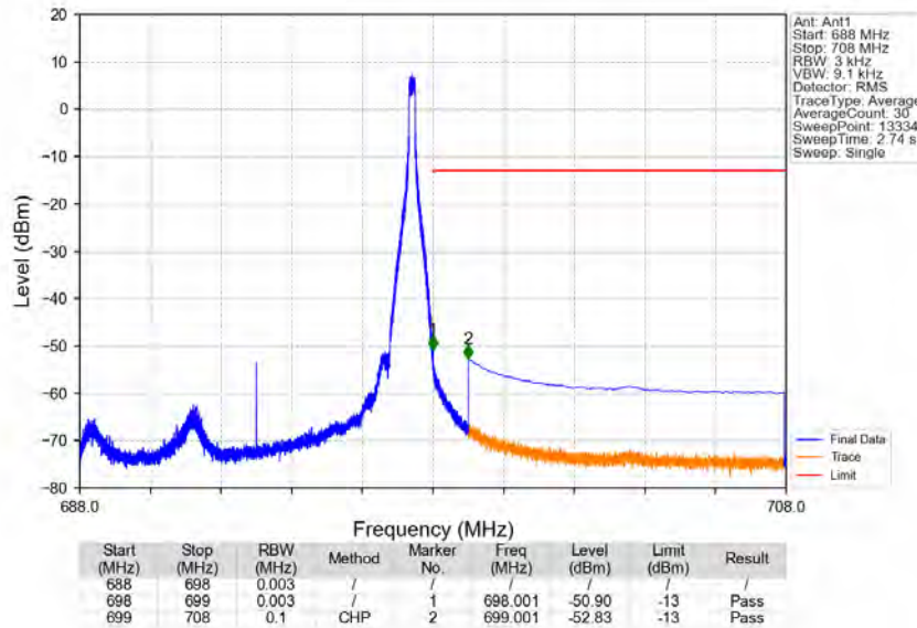
Band71_10MHz_16QAM_HCH_693MHz_RB_1_49_NTV
