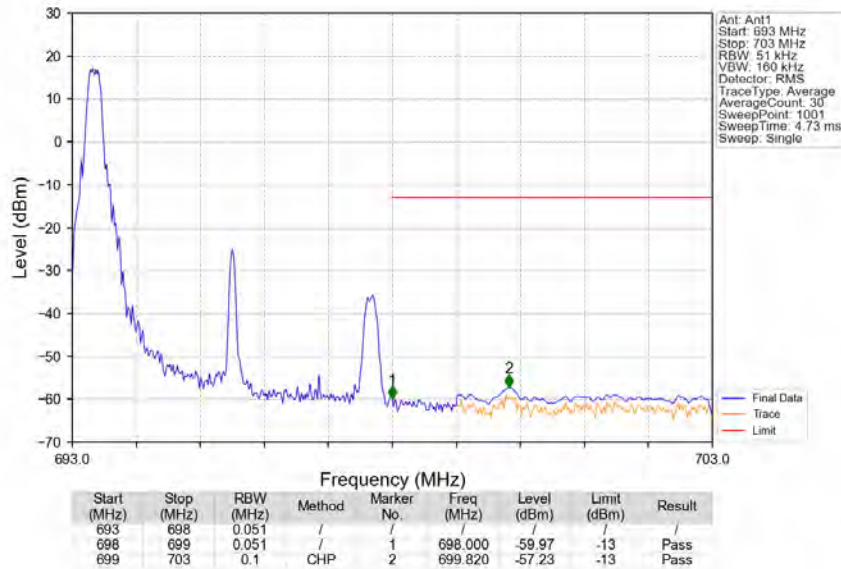
Band71_5MHz_64QAM_HCH_695.5MHz_RB_25_0_NTV
