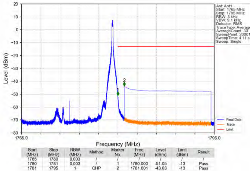
Band66_15MHz_16QAM_HCH_1772.5MHz_RB_1_74_NTNV
