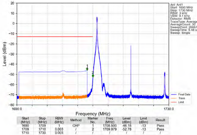
Band66_20MHz_64QAM_LCH_1720MHz_RB_1_0_NTNV
