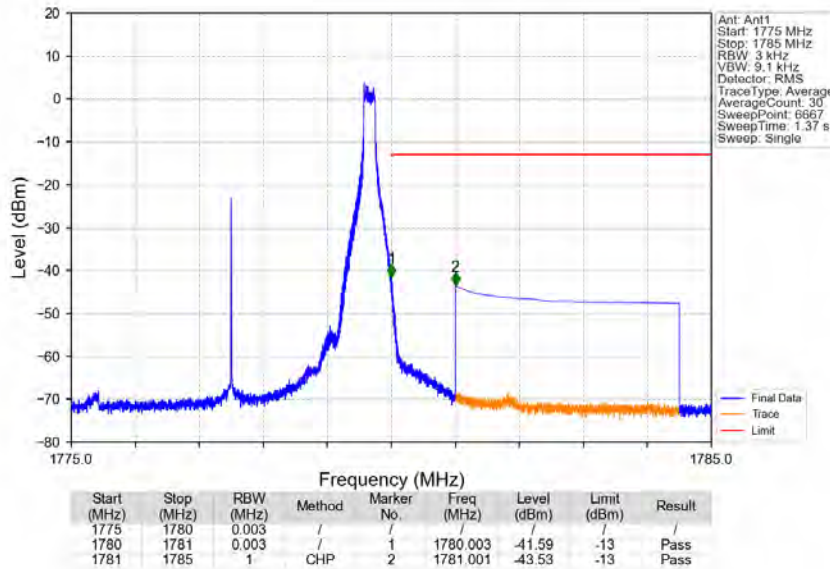
Band66_5MHz_256QAM_HCH_1777.5MHz_RB_1_24_NTNV
