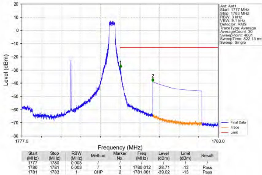
Band66_3MHz_QPSK_HCH_1778.5MHz_RB_1_14_NTNV
