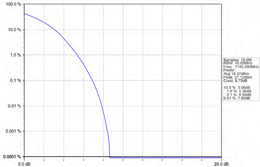
Band66_10MHz_256QAM_MCH_1745MHz_RB_50_0_NTNV
