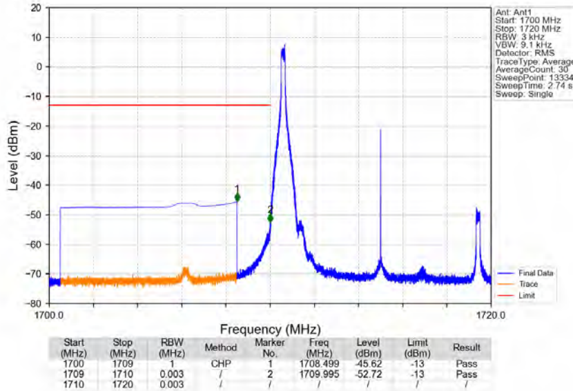
Band66_10MHz_64QAM_LCH_1715MHz_RB_1_0_NTNV
