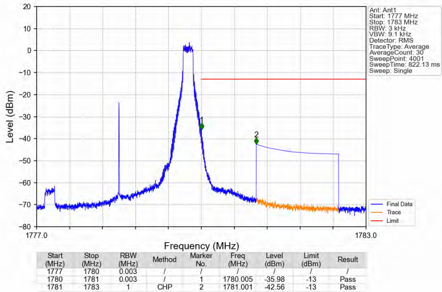
Band66_3MHz_256QAM_HCH_1778.5MHz_RB_1_14_NTNV
