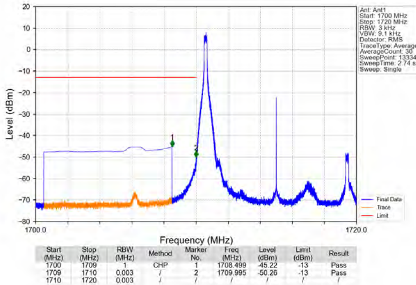
Band66_10MHz_16QAM_LCH_1715MHz_RB_1_0_NTNV
