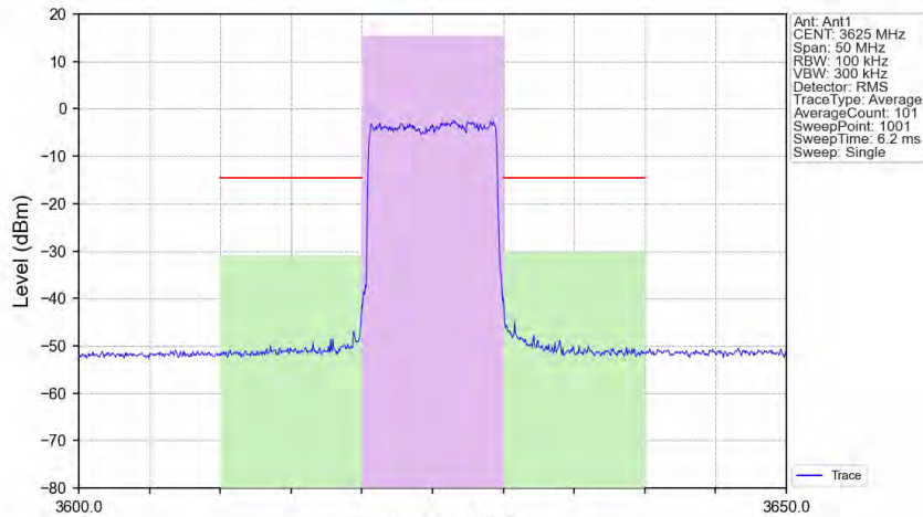
Band48_10MHz_256QAM_MCH_3625MHz_RB_50_0_NTNV
