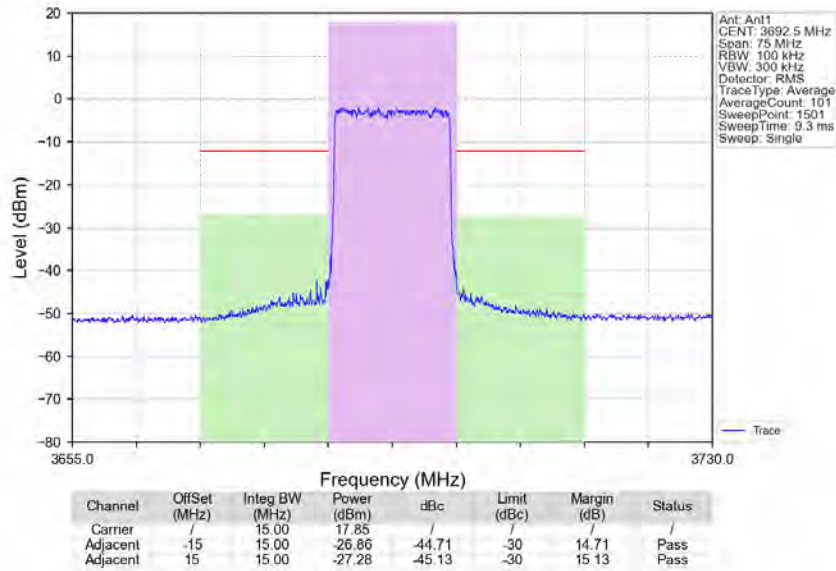
Band48_15MHz_64QAM_HCH_3692.5MHz_RB_75_0_NTNV
