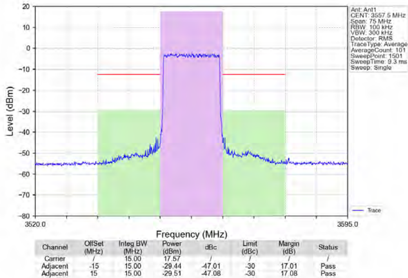
Band48_15MHz_64QAM_LCH_3557.5MHz_RB_75_0_NTNV
