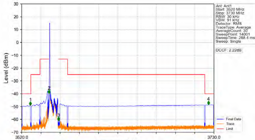
Band48_10MHz_64QAM_LCH_3555MHz_RB_1_0_NTNV
