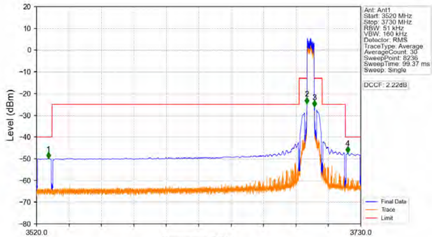
Band48_5MHz_QPSK_HCH_3697.5MHz_RB_25_0_NTNV
