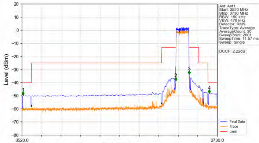
Band48_15MHz_64QAM_HCH_3692.5MHz_RB_75_0_NTNV
