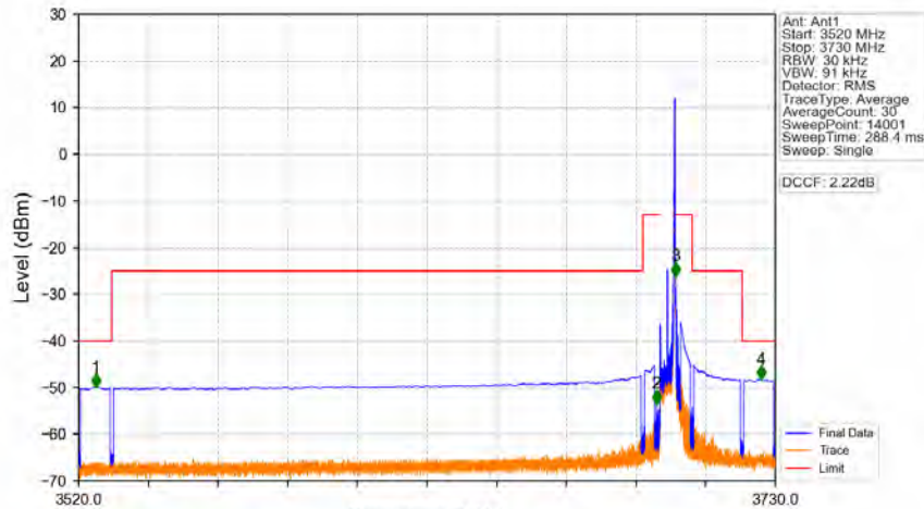
Band48_5MHz_256QAM_HCH_3697.5MHz_RB_1_24_NTNV
