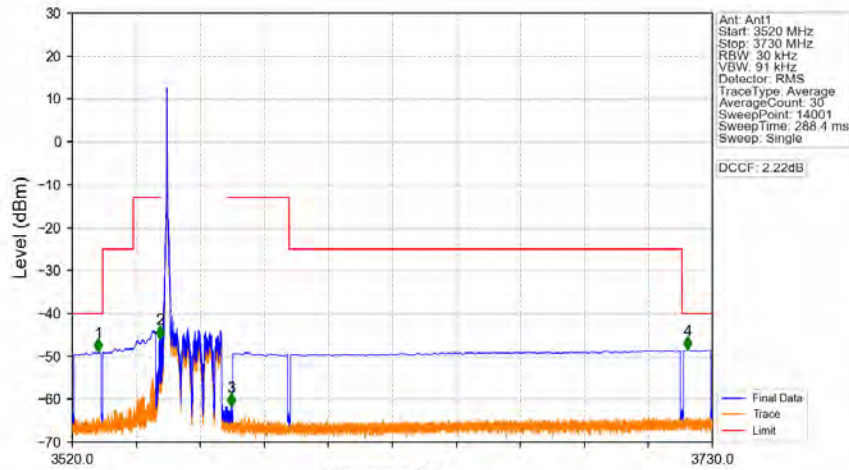
Band48_20MHz_64QAM_LCH_3560MHz_RB_1_0_NTNV
