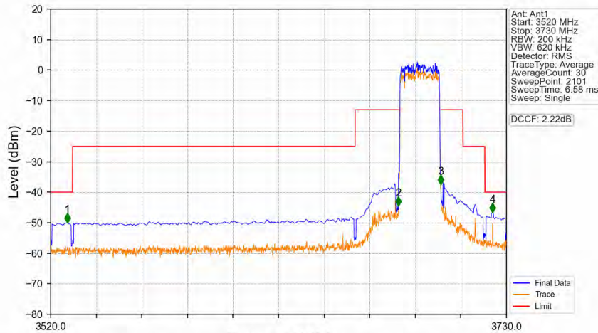
Band48_20MHz_64QAM_HCH_3690MHz_RB_100_0_NTNV
