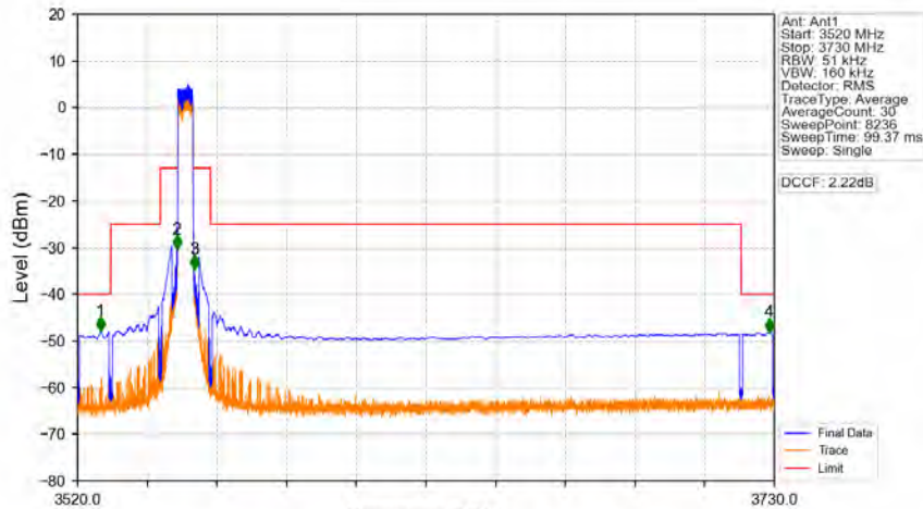
Band48_5MHz_QPSK_LCH_3552.5MHz_RB_25_0_NTNV
