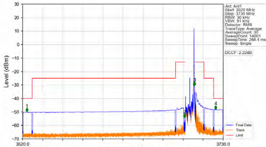
Band48_10MHz_256QAM_HCH_3695MHz_RB_1_49_NTNV
