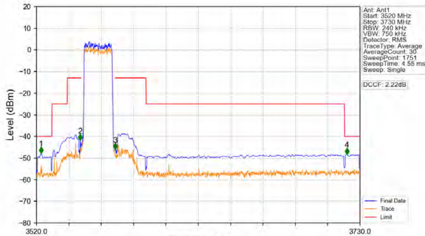
Band48_20MHz_64QAM_LCH_3560MHz_RB_100_0_NTNV
