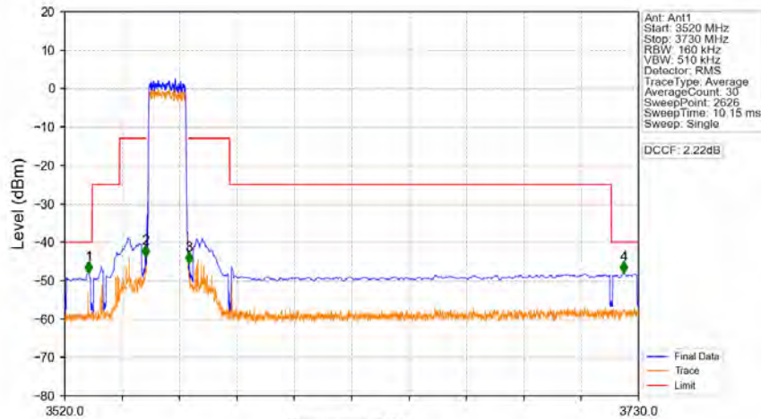
Band48_15MHz_64QAM_LCH_3557.5MHz_RB_75_0_NTNV
