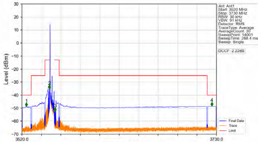
Band48_5MHz_64QAM_LCH_3552.5MHz_RB_1_0_NTNV
