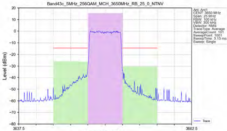
Band43c_5MHz_256QAM_MCH_3650MHz_RB_25_0_NTNV
