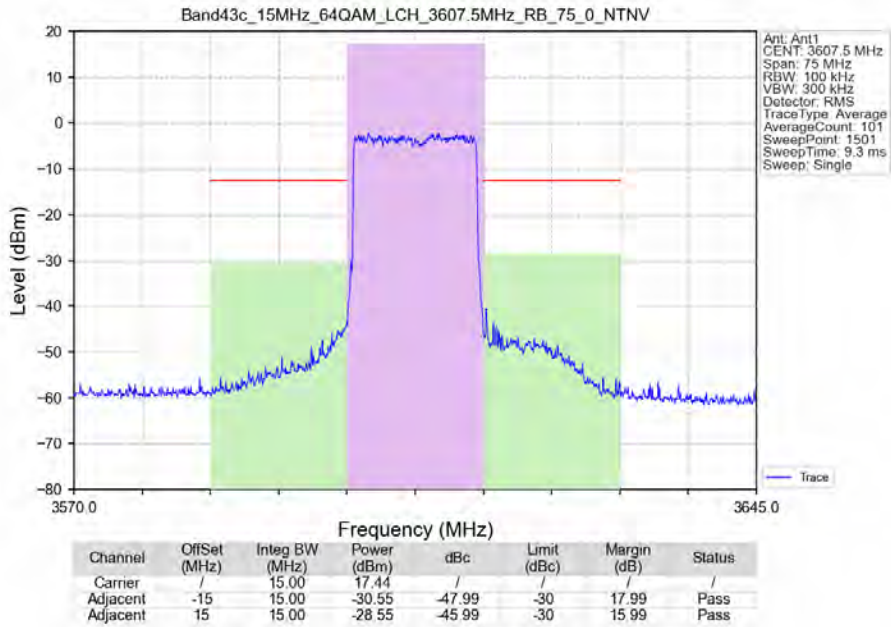
Band43c_15MHz_64QAM_LCH_3607.5MHz_RB_75_0_NTNV
