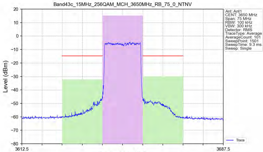
Band43c_15MHz_256QAM_MCH_3650MHz_RB_75_0_NTNV
