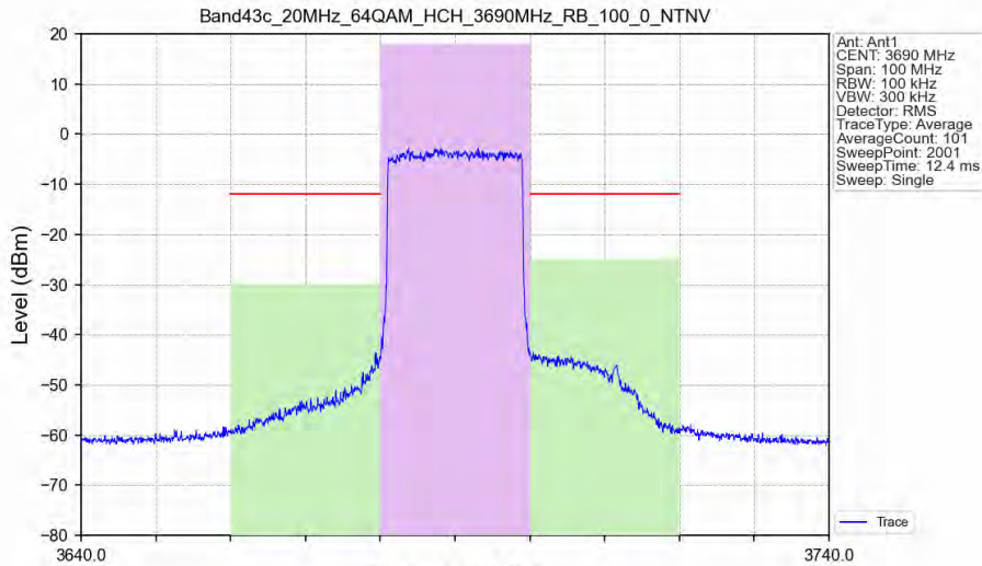
Band43c_20MHz_64QAM_HCH_3690MHz_RB_100_0_NTNV
