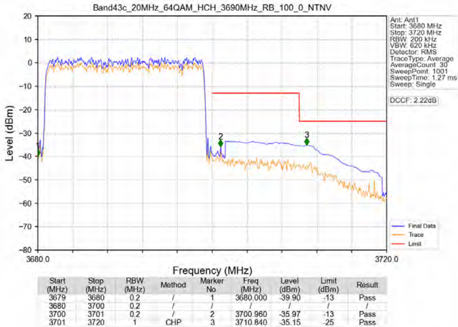
Band43c_20MHz_64QAM_HCH_3690MHz_RB_100_0_NTNV
