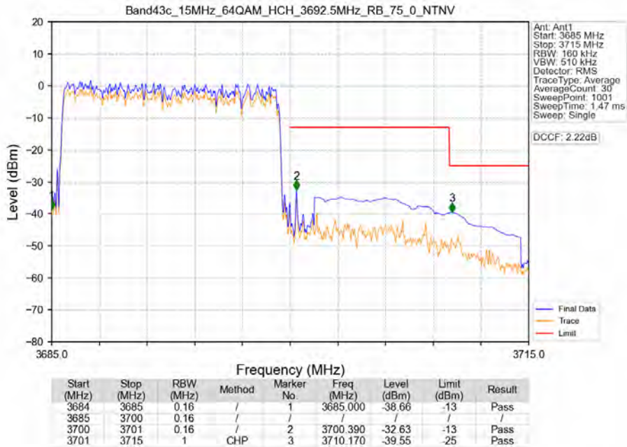
Band43c_15MHz_64QAM_HCH_3692.5MHz_RB_75_0_NTNV
