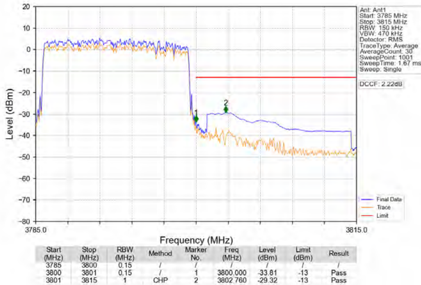
Band43d_15MHz_QPSK_HCH_3792.5MHz_RB_75_0_NTNV
