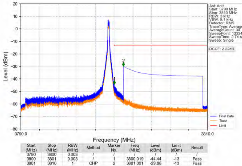
Band43d_10MHz_16QAM_HCH_3795MHz_RB_1_49_NTNV
