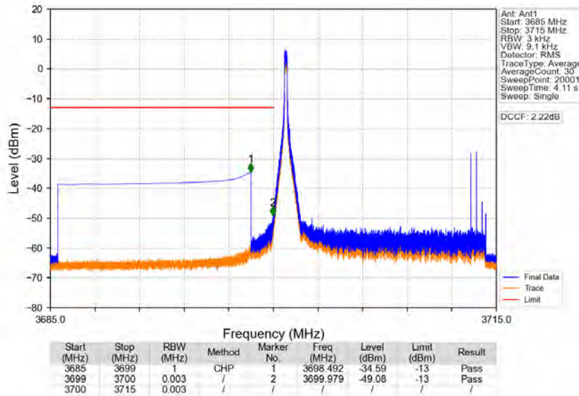
Band43d_15MHz_64QAM_LCH_3707.5MHz_RB_1_0_NTNV
