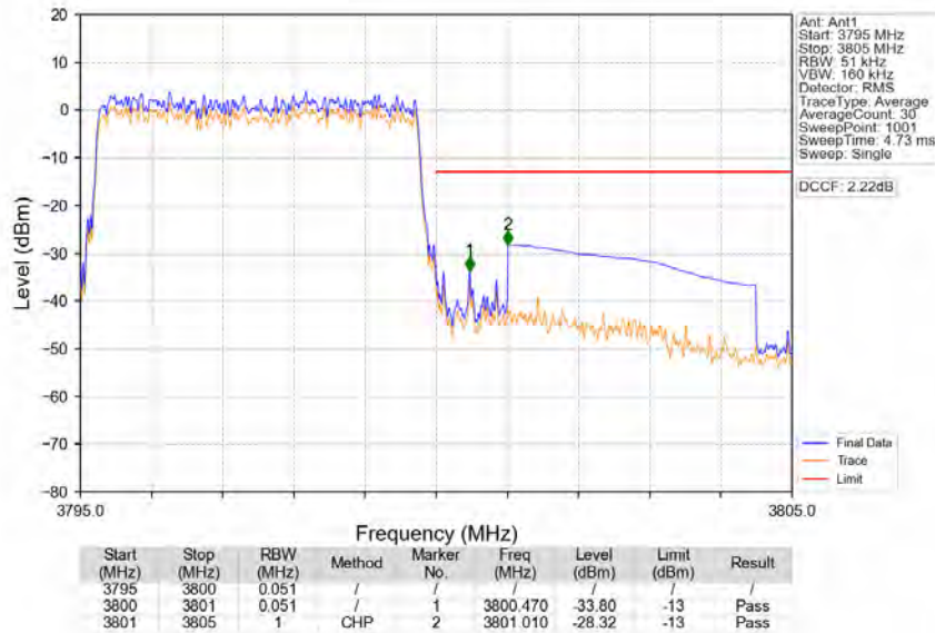
Band43d_5MHz_64QAM_HCH_3797.5MHz_RB_25_0_NTNV
