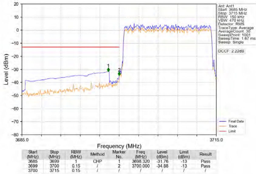
Band43d_15MHz_QPSK_LCH_3707.5MHz_RB_75_0_NTNV
