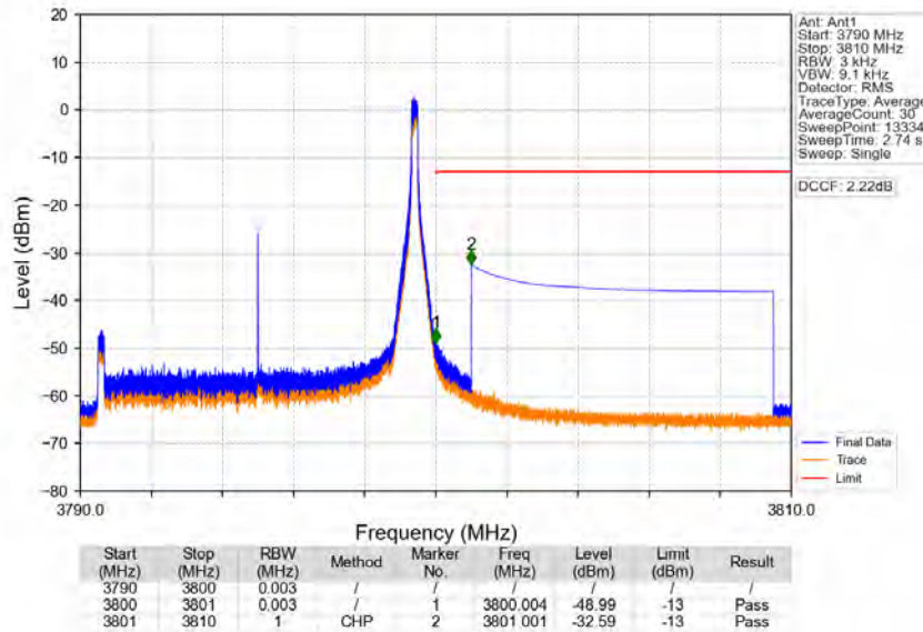
Band43d_10MHz_256QAM_HCH_3795MHz_RB_1_49_NTNV
