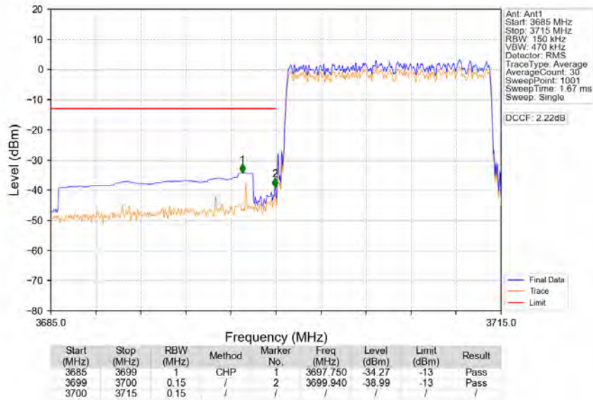
Band43d_15MHz_64QAM_LCH_3707.5MHz_RB_75_0_NTNV
