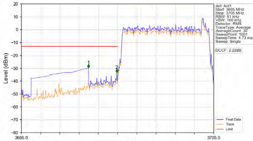
Band43d_5MHz_64QAM_LCH_3702.5MHz_RB_25_0_NTNV
