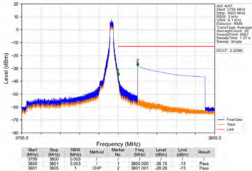
Band43d_5MHz_16QAM_HCH_3797.5MHz_RB_1_24_NTNV
