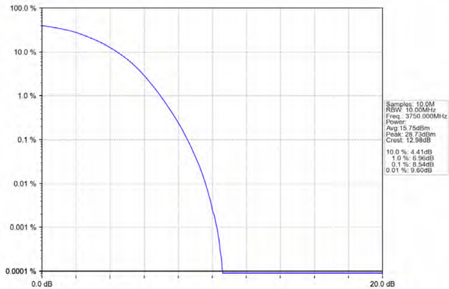
Band43d_10MHz_256QAM_MCH_3750MHz_RB_50_0_NTNV
