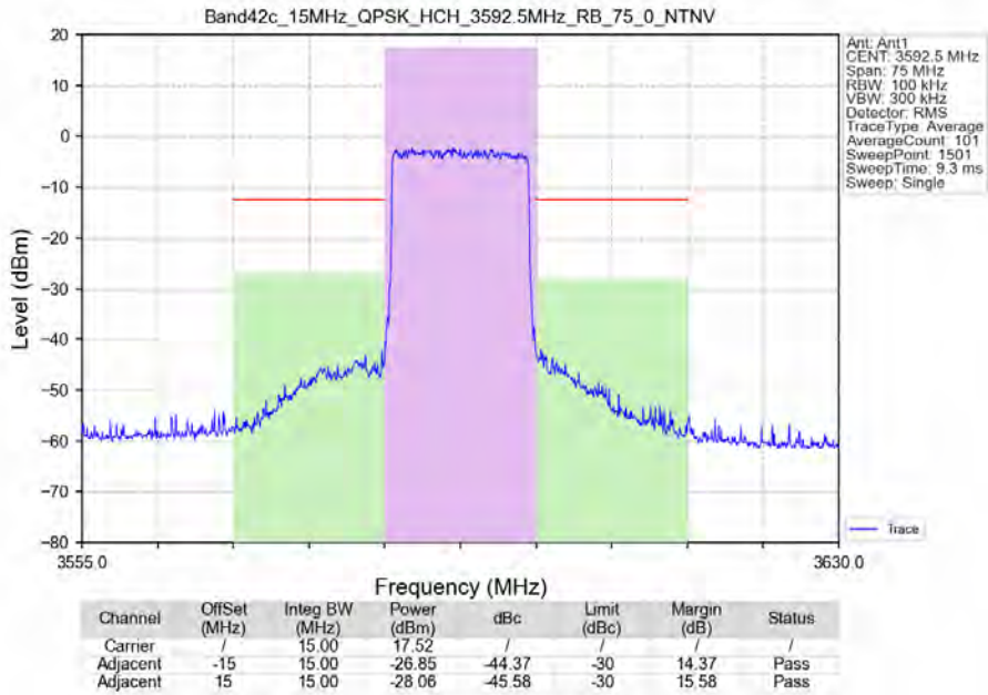
Band42c_15MHz_QPSK_HCH_3592.5MHz_RB_75_0_NTNV
