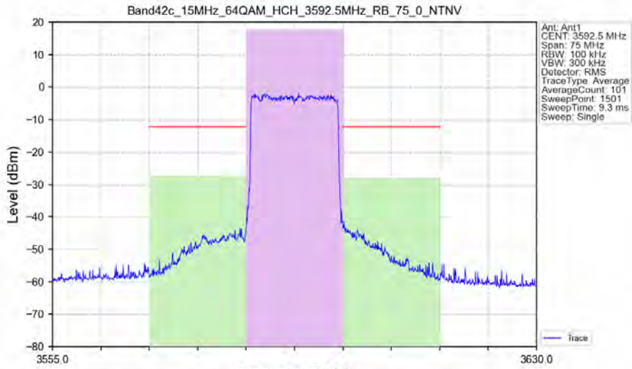
Band42c_15MHz_64QAM_HCH_3592.5MHz_RB_75_0_NTNV
