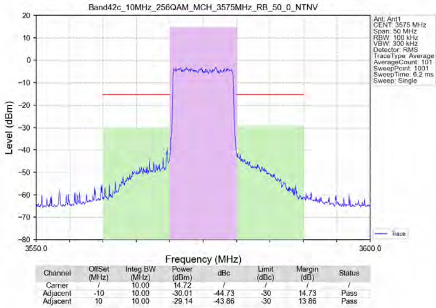
Band42c_10MHz_256QAM_MCH_3575MHz_RB_50_0_NTNV
