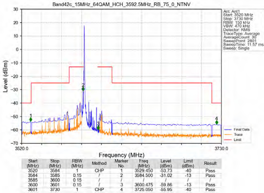
Band42c 15MHz 64QAM HCH 3592.5MHz RB 75 0 NTV
