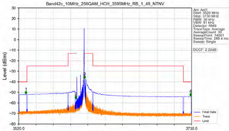
Band42c_10MHz_256QAM_HCH_3595MHz_RB_1_49_NTNV
