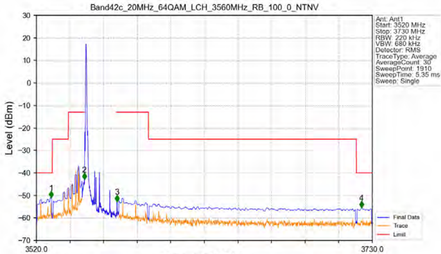
Band42c_20MHz_64QAM_LCH_3560MHz_RB_100_0_NTNV
