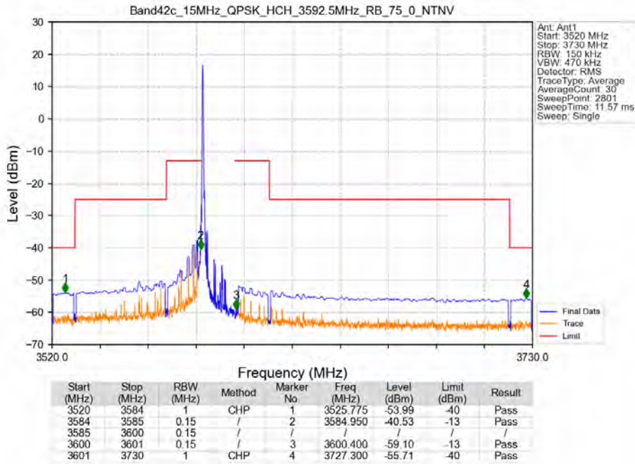
Band42c_15MHz_QPSK_HCH_3592.5MHz_RB_75_0_NTNV
